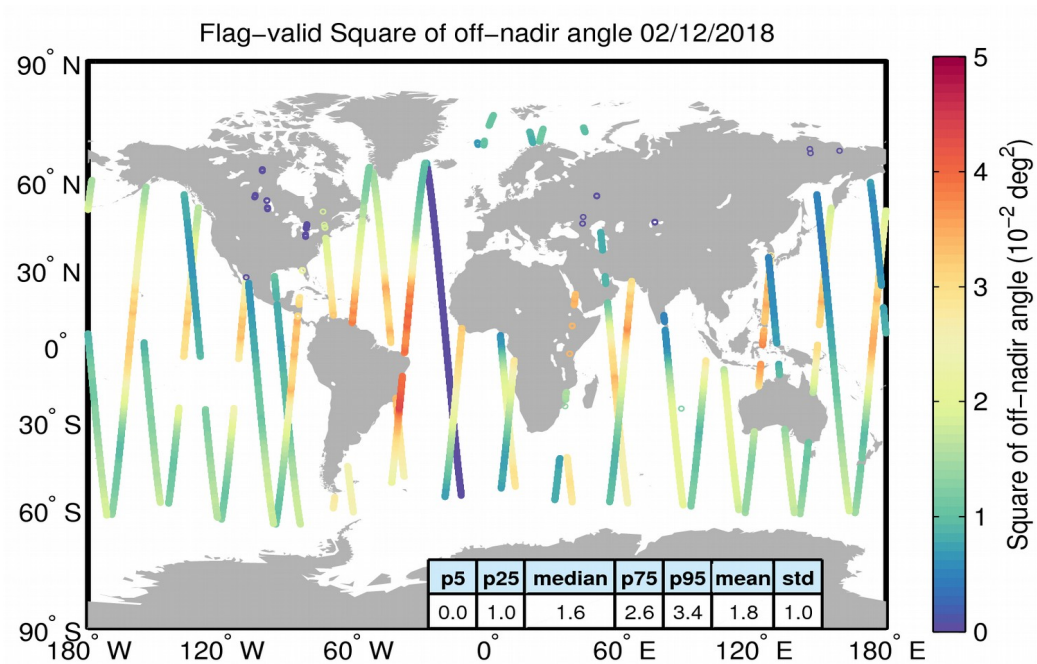
Figure 37. Geographical distribution of flag-valid mispointing data over oceans and lakes for 02/12/2018. The statistical values shown in the table refer to the mispointing in 10^{-2} \text{ deg}^2 and are calculated over all measurements shown in the figure.
