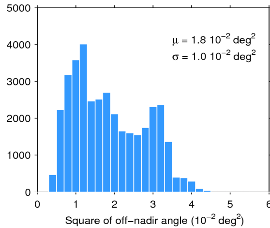
Figure 39. Histogram of flag-valid mispointing over oceans and lakes for 02/12/2018. The mean ( \mu ) and standard deviation ( \sigma ) are also shown. Note that values larger than 6 \cdot 10^{-2} \text{ deg}^2 are excluded from the histogram for the sake of readability but not from the computation of \mu and \sigma .
