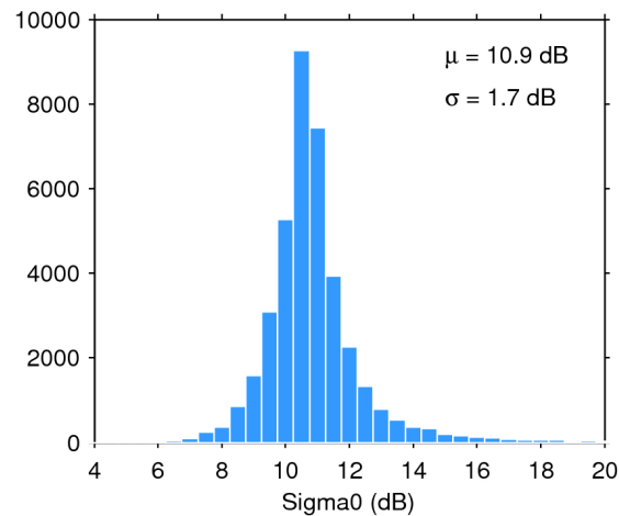
Figure 25. Histogram of flag-valid sigma0 over oceans and lakes for 02/12/2018. The mean ( \mu ) and standard deviation ( \sigma ) are also shown. Note that values outside [4 20] dB are excluded from the histogram for the sake of readability but not from the computation of \mu and \sigma .
