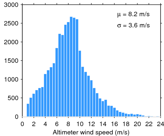
Figure 33. Histogram of flag-valid wind over oceans and lakes for 02/12/2018. The mean ( \mu ) and standard deviation ( \sigma ) are also shown. Note that values larger than 24 m/s are excluded from the histogram for the sake of readability but not from the computation of \mu and \sigma .
