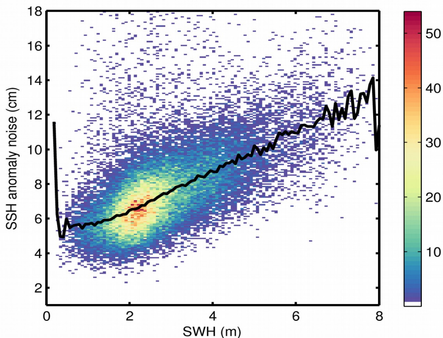
Figure 9. 2D histogram showing flag-valid SSH anomaly noise as a function of SWH for 02/12/2018. The black line denotes the median SSH anomaly noise as a function of SWH.
