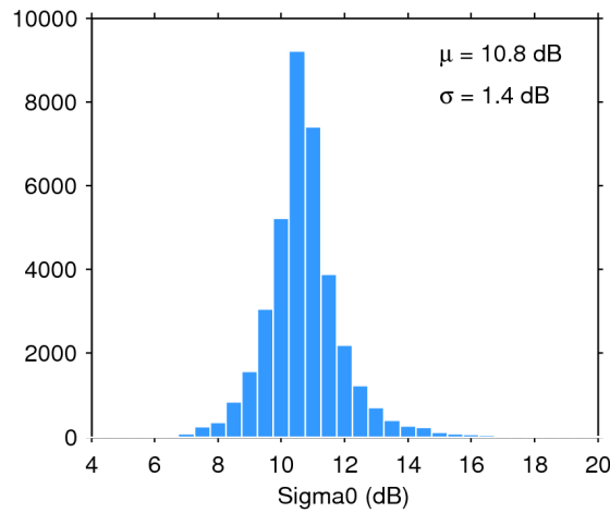
Figure 28. Histogram of science-valid sigma0 over oceans and lakes for 02/12/2018. The mean ( \mu ) and standard deviation ( \sigma ) are also shown. Note that values outside [4 20] dB are excluded from the histogram for the sake of readability but not from the computation of \mu and \sigma .
