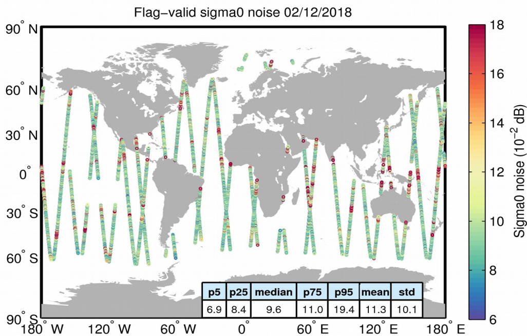
Figure 26. Geographical distribution of flag-valid 20-Hz sigma0 measurement noise over oceans and lakes for 02/12/2018. The statistical values shown in the table refer to the sigma0 noise and are calculated over all measurements shown in the figure.
