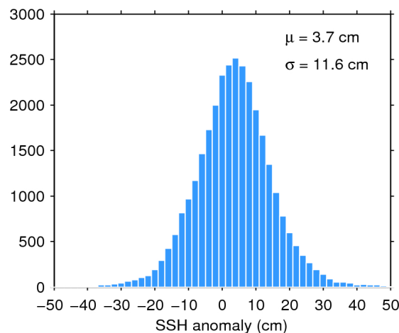
Figure 11. Histogram of science-valid SSH anomaly over oceans and lakes for 02/12/2018. The mean ( \mu ) and standard deviation ( \sigma ) are also shown. Note that values outside [-50 50] cm are excluded from the histogram for the sake of readability but not from the computation of \mu and \sigma .
