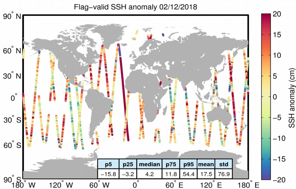
Figure 5. Geographical distribution of flag-valid 1-Hz SSH anomaly data over oceans and lakes for 02/12/2018. The statistical values shown in the table refer to the SSH anomaly in cm and are calculated over all measurements shown in the figure.
