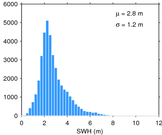
Figure 20. Histogram of science-valid SWH over oceans and lakes for 02/12/2018. The mean ( \mu ) and standard deviation ( \sigma ) are also shown. Note that values larger than 12 m are excluded from the histogram for the sake of readability but not from the computation of \mu and \sigma .
