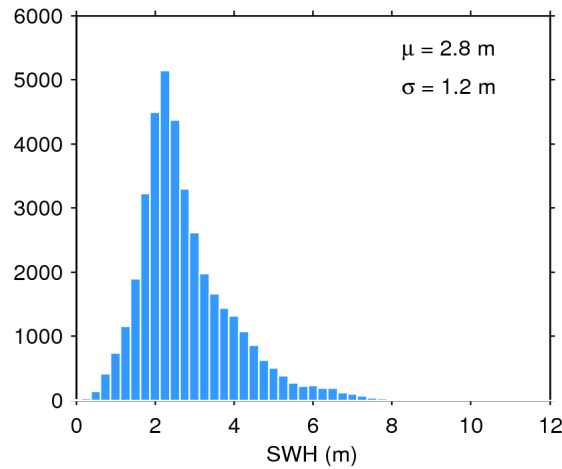
Figure 17. Histogram of flag-valid SWH over oceans and lakes for 02/12/2018. The mean ( \mu ) and standard deviation ( \sigma ) are also shown. Note that values larger than 12 m are excluded from the histogram for the sake of readability but not from the computation of \mu and \sigma .
