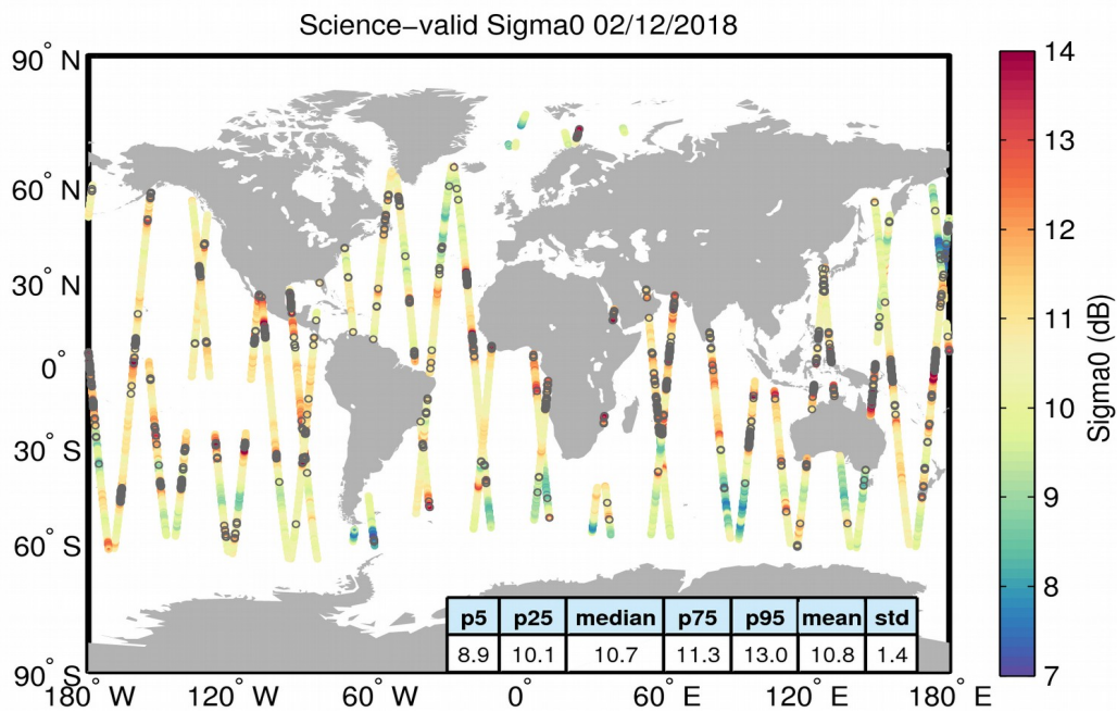
Figure 27. Geographical distribution of science-valid sigma0 data over oceans and lakes for 02/12/2018. The statistical values shown in the table refer to the sigma0 in dB and are calculated over all measurements shown in the figure. Gray circles denote records that have been rejected based on the editing criteria described in Table 4.
