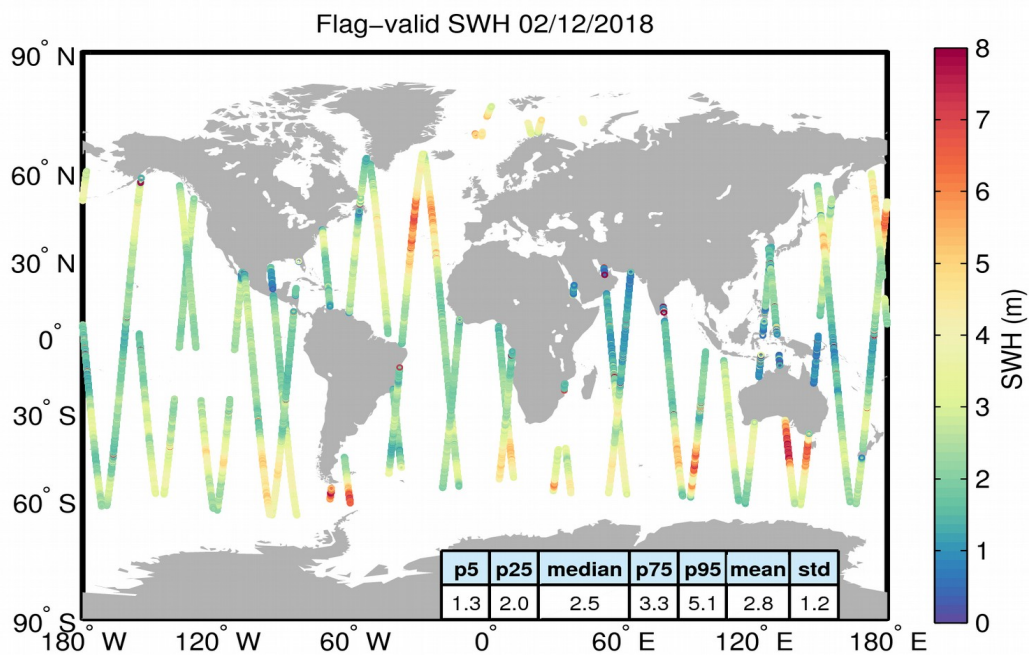
Figure 15. Geographical distribution of flag-valid SWH data over oceans and lakes for 02/12/2018. The statistical values shown in the table refer to the SWH in m and are calculated over all measurements shown in the figure.
