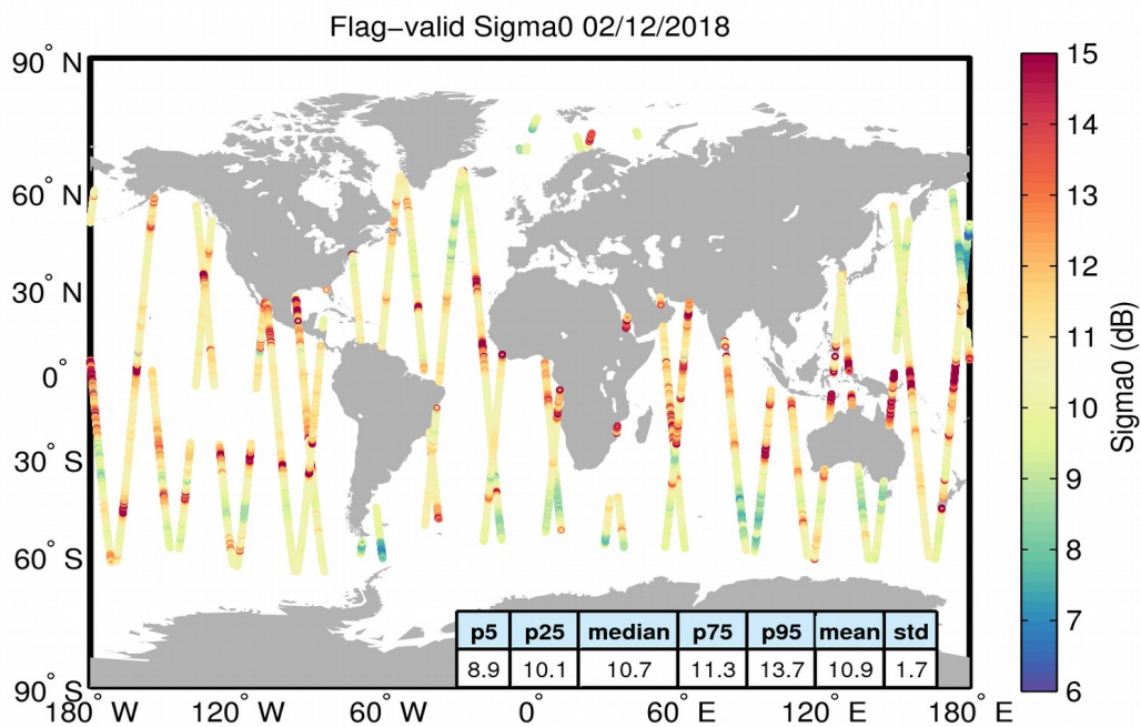
Figure 23. Geographical distribution of flag-valid sigma0 data over oceans and lakes for 02/12/2018. The statistical values shown in the table refer to the sigma0 in dB and are calculated over all measurements shown in the figure.
