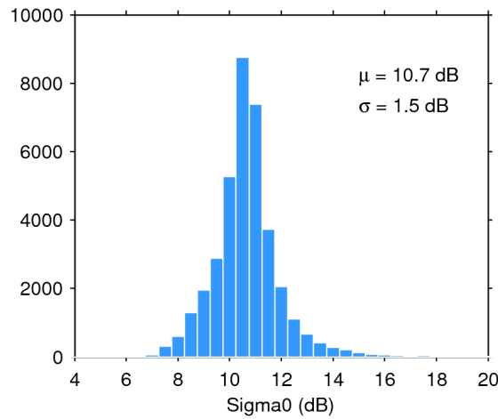
Figure 28. Histogram of science-valid sigma0 over oceans and lakes for 01/12/2018. The mean ( \mu ) and standard deviation ( \sigma ) are also shown. Note that values outside [4 20] dB are excluded from the histogram for the sake of readability but not from the computation of \mu and \sigma .
