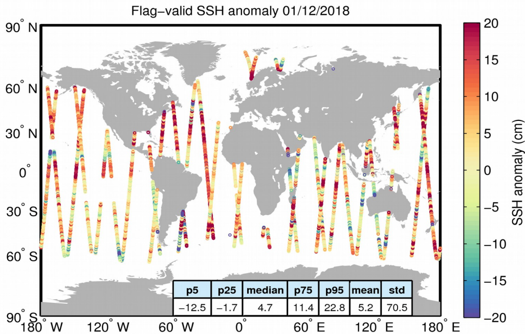
Figure 5. Geographical distribution of flag-valid 1-Hz SSH anomaly data over oceans and lakes for 01/12/2018. The statistical values shown in the table refer to the SSH anomaly in cm and are calculated over all measurements shown in the figure.
