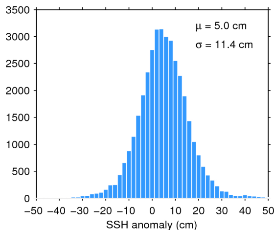
Figure 11. Histogram of science-valid SSH anomaly over oceans and lakes for 01/12/2018. The mean ( \mu ) and standard deviation ( \sigma ) are also shown. Note that values outside [-50 50] cm are excluded from the histogram for the sake of readability but not from the computation of \mu and \sigma .
