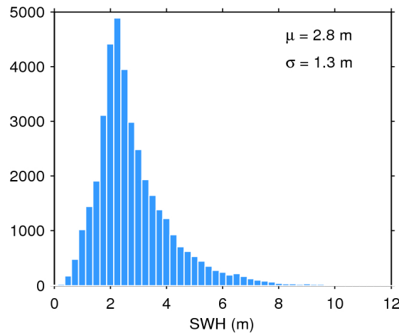
Figure 20. Histogram of science-valid SWH over oceans and lakes for 01/12/2018. The mean ( \mu ) and standard deviation ( \sigma ) are also shown. Note that values larger than 12 m are excluded from the histogram for the sake of readability but not from the computation of \mu and \sigma .
