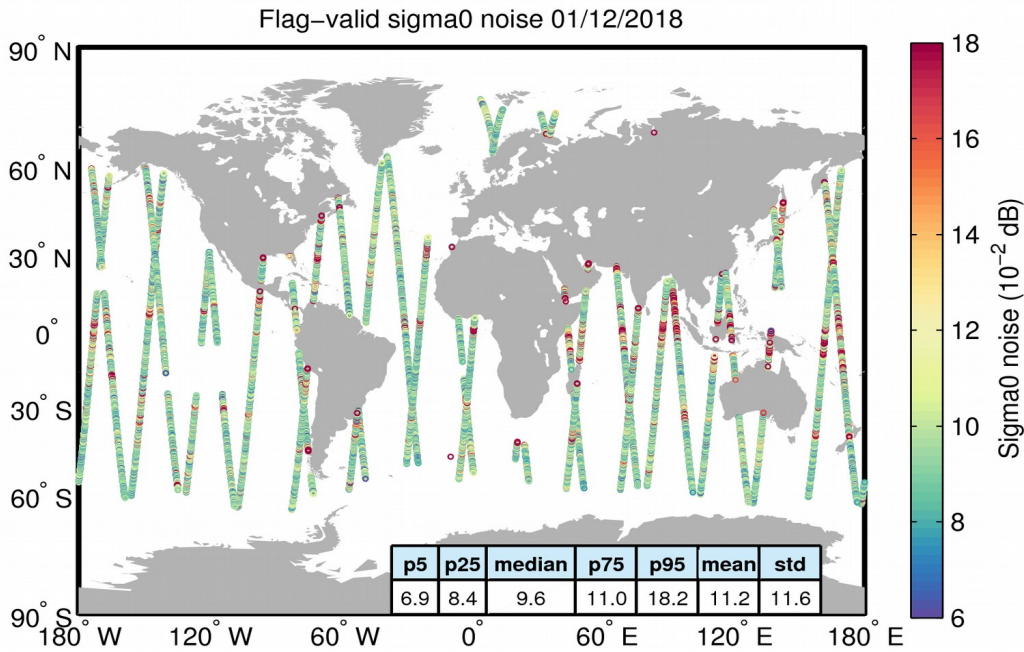
Figure 26. Geographical distribution of flag-valid 20-Hz sigma0 measurement noise over oceans and lakes for 01/12/2018. The statistical values shown in the table refer to the sigma0 noise and are calculated over all measurements shown in the figure.
