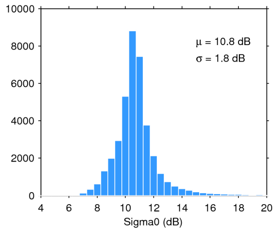
Figure 25. Histogram of flag-valid sigma0 over oceans and lakes for 01/12/2018. The mean ( \mu ) and standard deviation ( \sigma ) are also shown. Note that values outside [4 20] dB are excluded from the histogram for the sake of readability but not from the computation of \mu and \sigma .
