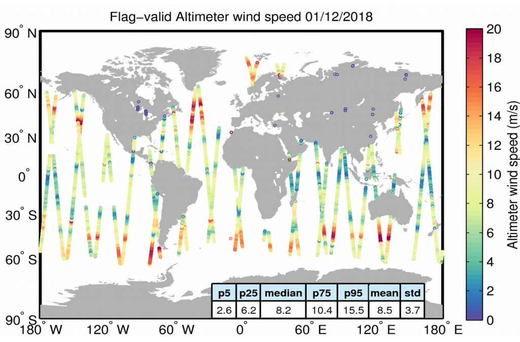
Figure 31. Geographical distribution of flag-valid wind data over oceans and lakes for 01/12/2018. The statistical values shown in the table refer to the wind in m/s and are calculated over all measurements shown in the figure.
