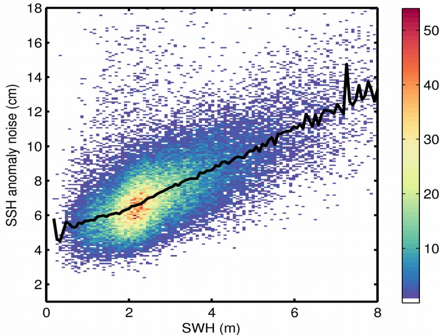
Figure 9. 2D histogram showing flag-valid SSH anomaly noise as a function of SWH for 01/12/2018. The black line denotes the median SSH anomaly noise as a function of SWH.
