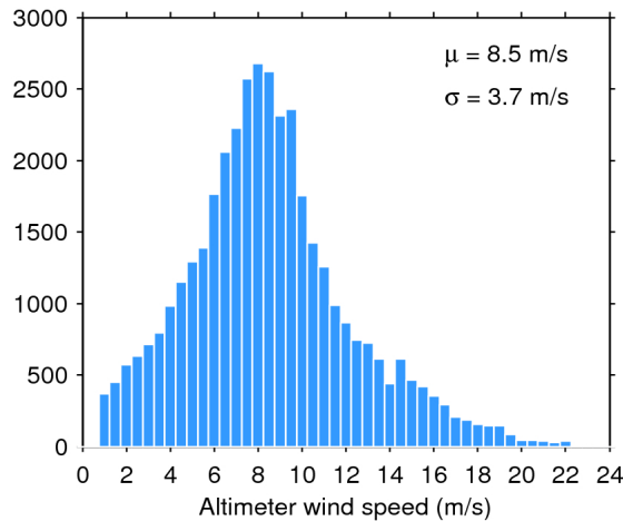
Figure 33. Histogram of flag-valid wind over oceans and lakes for 01/12/2018. The mean ( \mu ) and standard deviation ( \sigma ) are also shown. Note that values larger than 24 m/s are excluded from the histogram for the sake of readability but not from the computation of \mu and \sigma .
