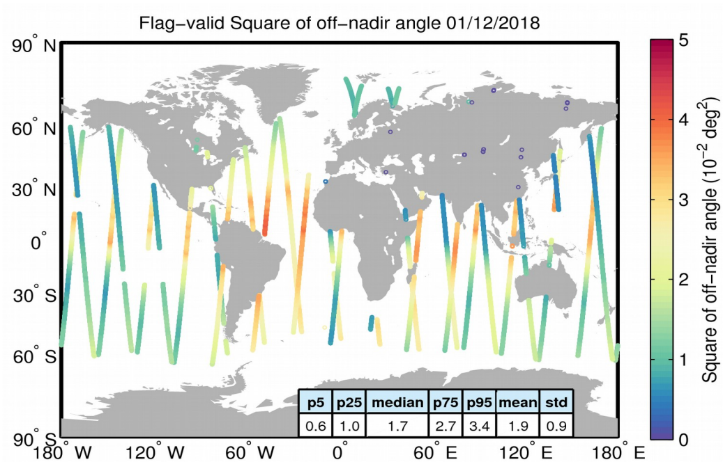
Figure 37. Geographical distribution of flag-valid mispointing data over oceans and lakes for 01/12/2018. The statistical values shown in the table refer to the mispointing in 10^{-2} \text{ deg}^2 and are calculated over all measurements shown in the figure.
