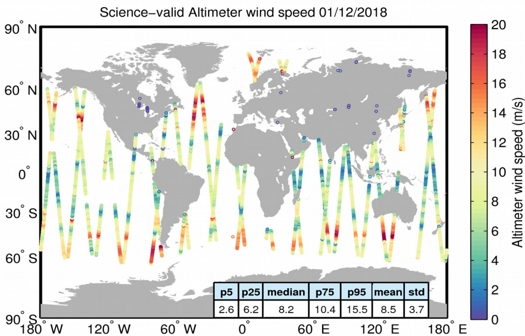
Figure 34. Geographical distribution of science-valid wind data over oceans and lakes for 01/12/2018. The statistical values shown in the table refer to the wind in m/s and are calculated over all measurements shown in the figure. Gray circles denote records that have been rejected based on the editing criteria described in Table 5.
