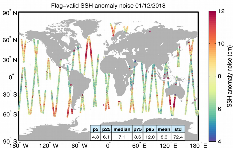
Figure 8. Geographical distribution of flag-valid 20-Hz SSH anomaly measurement noise over oceans and lakes for 01/12/2018. The statistical values shown in the table refer to the SSH anomaly noise and are calculated over all measurements shown in the figure.
