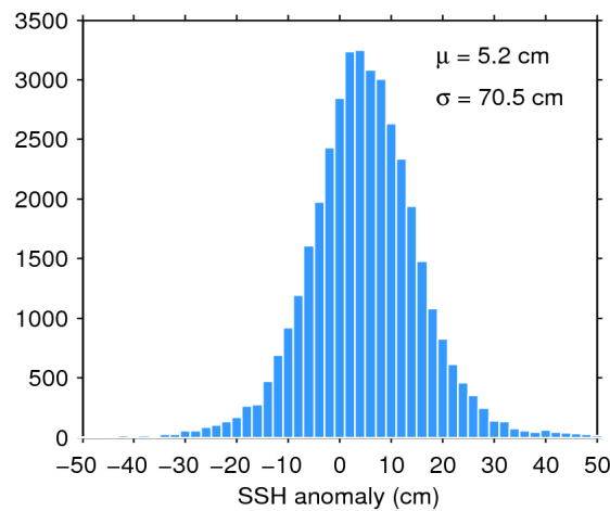
Figure 7. Histogram of flag-valid SSH anomaly over oceans and lakes for 01/12/2018. The mean ( \mu ) and standard deviation ( \sigma ) are also shown. Note that values outside [-50\ 50] cm are excluded from the histogram for the sake of readability but not from the computation of \mu and \sigma .
