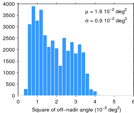
Figure 39. Histogram of flag-valid mispointing over oceans and lakes for 01/12/2018. The mean ( \mu ) and standard deviation ( \sigma ) are also shown. Note that values larger than 6 \cdot 10^{-2} \text{ deg}^2 are excluded from the histogram for the sake of readability but not from the computation of \mu and \sigma .
