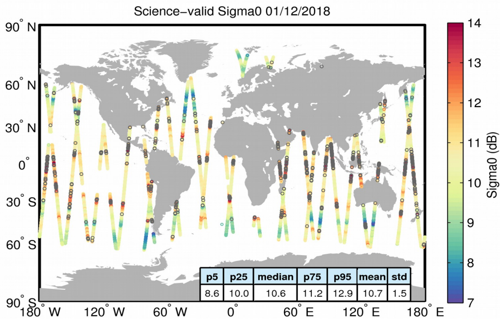
Figure 27. Geographical distribution of science-valid sigma0 data over oceans and lakes for 01/12/2018. The statistical values shown in the table refer to the sigma0 in dB and are calculated over all measurements shown in the figure. Gray circles denote records that have been rejected based on the editing criteria described in Table 4.
