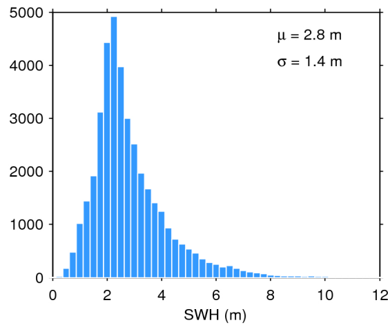
Figure 17. Histogram of flag-valid SWH over oceans and lakes for 01/12/2018. The mean ( \mu ) and standard deviation ( \sigma ) are also shown. Note that values larger than 12 m are excluded from the histogram for the sake of readability but not from the computation of \mu and \sigma .
