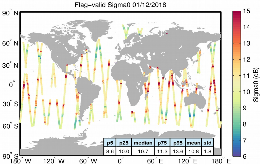
Figure 23. Geographical distribution of flag-valid sigma0 data over oceans and lakes for 01/12/2018. The statistical values shown in the table refer to the sigma0 in dB and are calculated over all measurements shown in the figure.
