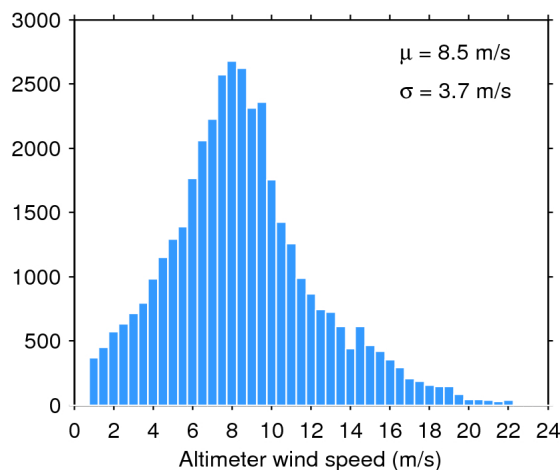
Figure 35. Histogram of science-valid wind over oceans and lakes for 01/12/2018. The mean ( \mu ) and standard deviation ( \sigma ) are also shown. Note that values larger than 24 m/s are excluded from the histogram for the sake of readability but not from the computation of \mu and \sigma .
