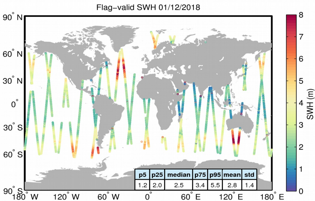
Figure 15. Geographical distribution of flag-valid SWH data over oceans and lakes for 01/12/2018. The statistical values shown in the table refer to the SWH in m and are calculated over all measurements shown in the figure.
