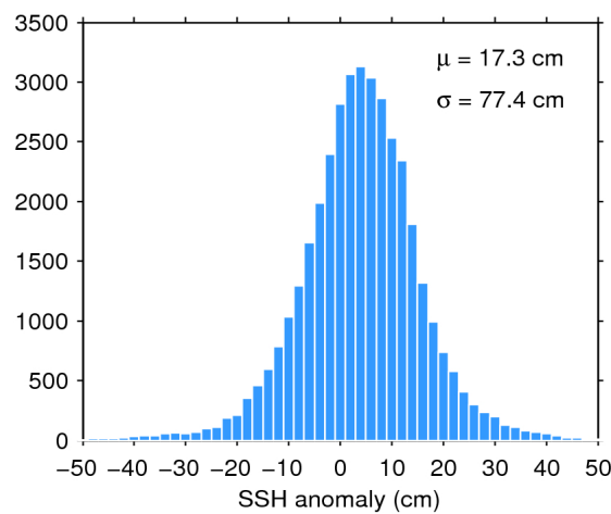
Figure 7. Histogram of flag-valid SSH anomaly over oceans and lakes for 30/11/2018. The mean ( \mu ) and standard deviation ( \sigma ) are also shown. Note that values outside [-50 \ 50] cm are excluded from the histogram for the sake of readability but not from the computation of \mu and \sigma .
