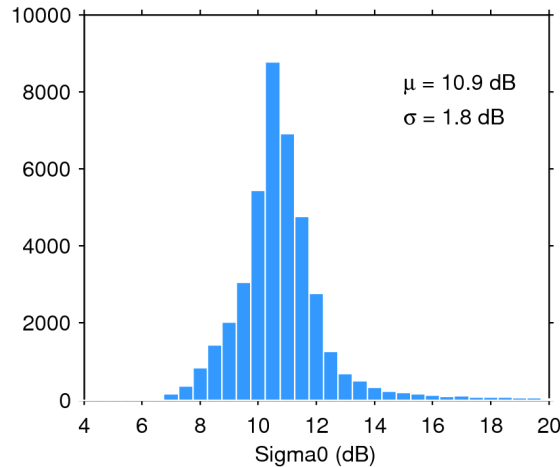
Figure 25. Histogram of flag-valid sigma0 over oceans and lakes for 30/11/2018. The mean ( \mu ) and standard deviation ( \sigma ) are also shown. Note that values outside [4 20] dB are excluded from the histogram for the sake of readability but not from the computation of \mu and \sigma .
