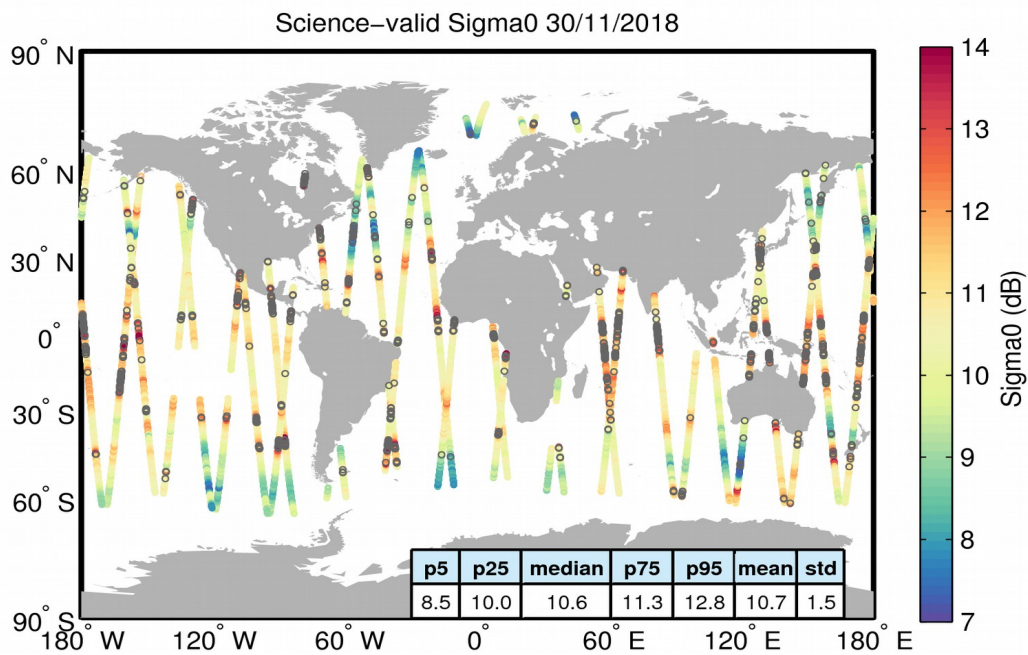
Figure 27. Geographical distribution of science-valid sigma0 data over oceans and lakes for 30/11/2018. The statistical values shown in the table refer to the sigma0 in dB and are calculated over all measurements shown in the figure. Gray circles denote records that have been rejected based on the editing criteria described in Table 4.
