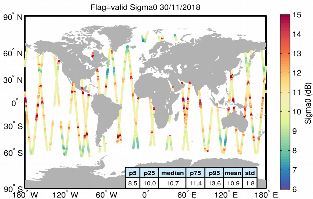
Figure 23. Geographical distribution of flag-valid sigma0 data over oceans and lakes for 30/11/2018. The statistical values shown in the table refer to the sigma0 in dB and are calculated over all measurements shown in the figure.
