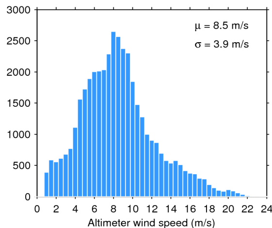
Figure 35. Histogram of science-valid wind over oceans and lakes for 30/11/2018. The mean ( \mu ) and standard deviation ( \sigma ) are also shown. Note that values larger than 24 m/s are excluded from the histogram for the sake of readability but not from the computation of \mu and \sigma .
