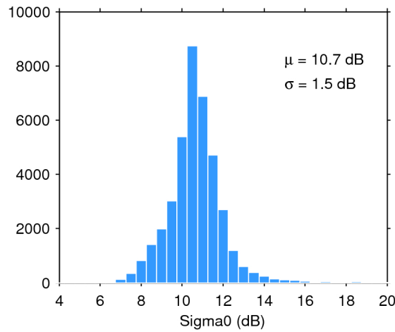
Figure 28. Histogram of science-valid sigma0 over oceans and lakes for 30/11/2018. The mean ( \mu ) and standard deviation ( \sigma ) are also shown. Note that values outside [4 20] dB are excluded from the histogram for the sake of readability but not from the computation of \mu and \sigma .
