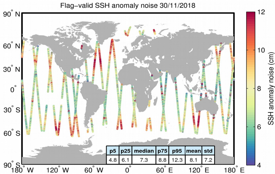
Figure 8. Geographical distribution of flag-valid 20-Hz SSH anomaly measurement noise over oceans and lakes for 30/11/2018. The statistical values shown in the table refer to the SSH anomaly noise and are calculated over all measurements shown in the figure.
