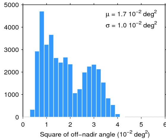
Figure 39. Histogram of flag-valid mispointing over oceans and lakes for 30/11/2018. The mean ( \mu ) and standard deviation ( \sigma ) are also shown. Note that values larger than 6 \cdot 10^{-2} \text{ deg}^2 are excluded from the histogram for the sake of readability but not from the computation of \mu and \sigma .
