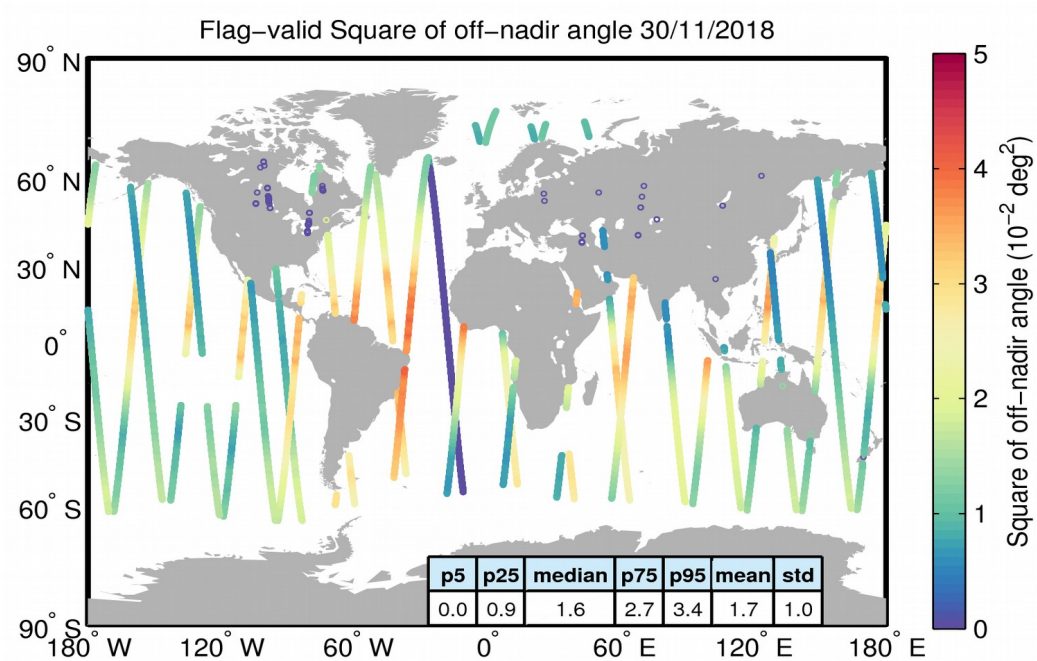
Figure 37. Geographical distribution of flag-valid mispointing data over oceans and lakes for 30/11/2018. The statistical values shown in the table refer to the mispointing in 10^{-2} deg 2 and are calculated over all measurements shown in the figure.
