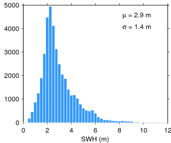
Figure 20. Histogram of science-valid SWH over oceans and lakes for 30/11/2018. The mean ( \mu ) and standard deviation ( \sigma ) are also shown. Note that values larger than 12 m are excluded from the histogram for the sake of readability but not from the computation of \mu and \sigma .
