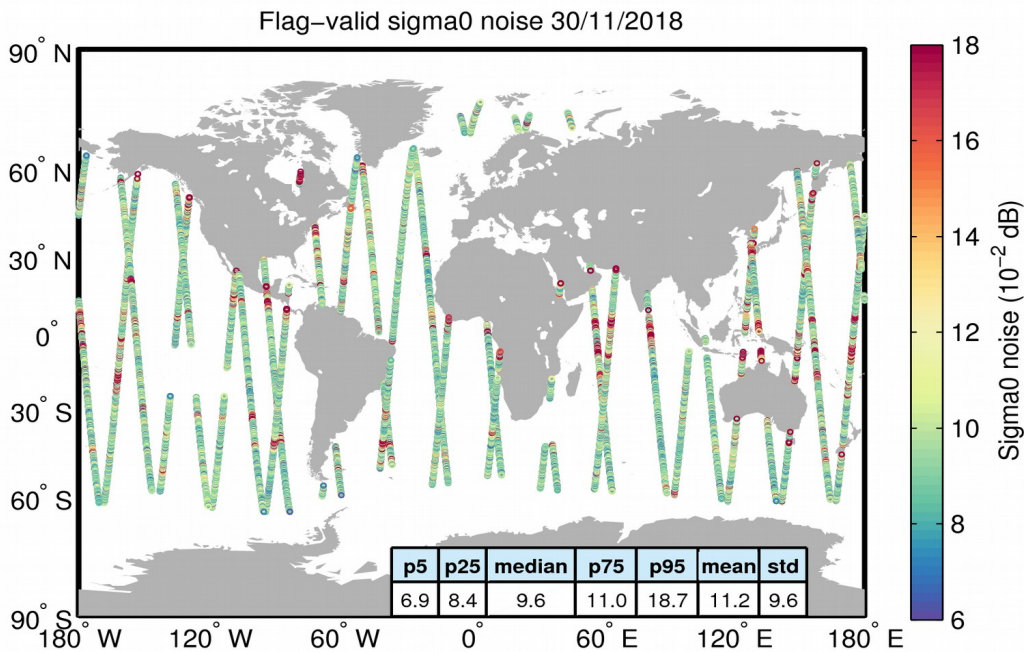
Figure 26. Geographical distribution of flag-valid 20-Hz sigma0 measurement noise over oceans and lakes for 30/11/2018. The statistical values shown in the table refer to the sigma0 noise and are calculated over all measurements shown in the figure.
