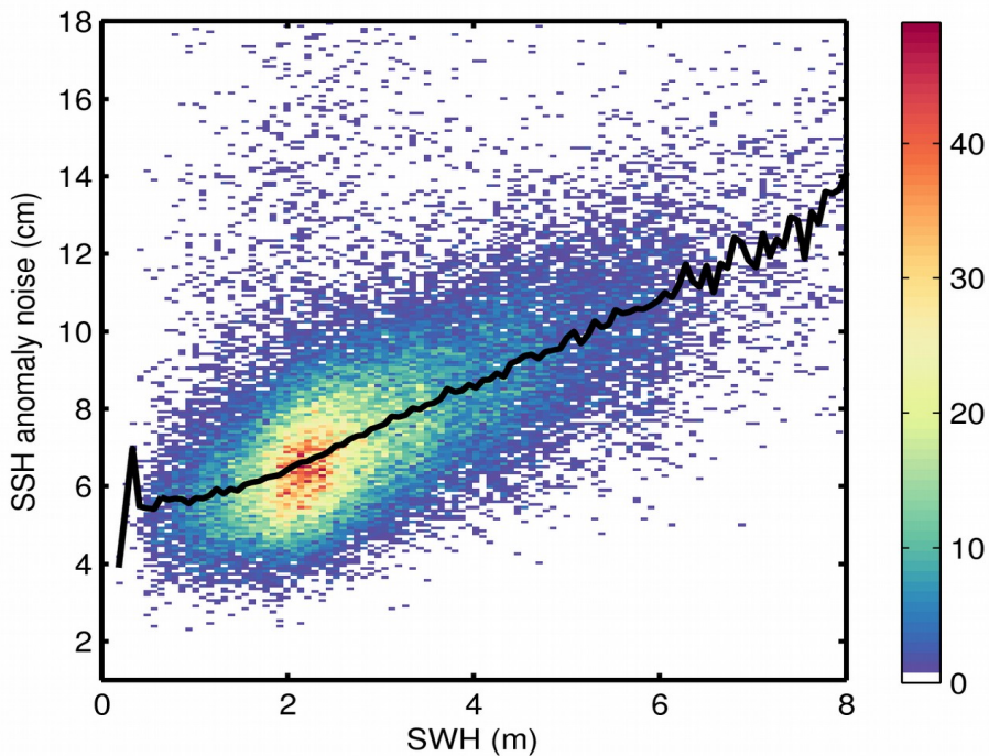
Figure 9. 2D histogram showing flag-valid SSH anomaly noise as a function of SWH for 30/11/2018. The black line denotes the median SSH anomaly noise as a function of SWH.
