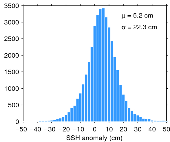
Figure 7. Histogram of flag-valid SSH anomaly over oceans and lakes for 29/11/2018. The mean ( \mu ) and standard deviation ( \sigma ) are also shown. Note that values outside [-50\ 50] cm are excluded from the histogram for the sake of readability but not from the computation of \mu and \sigma .
