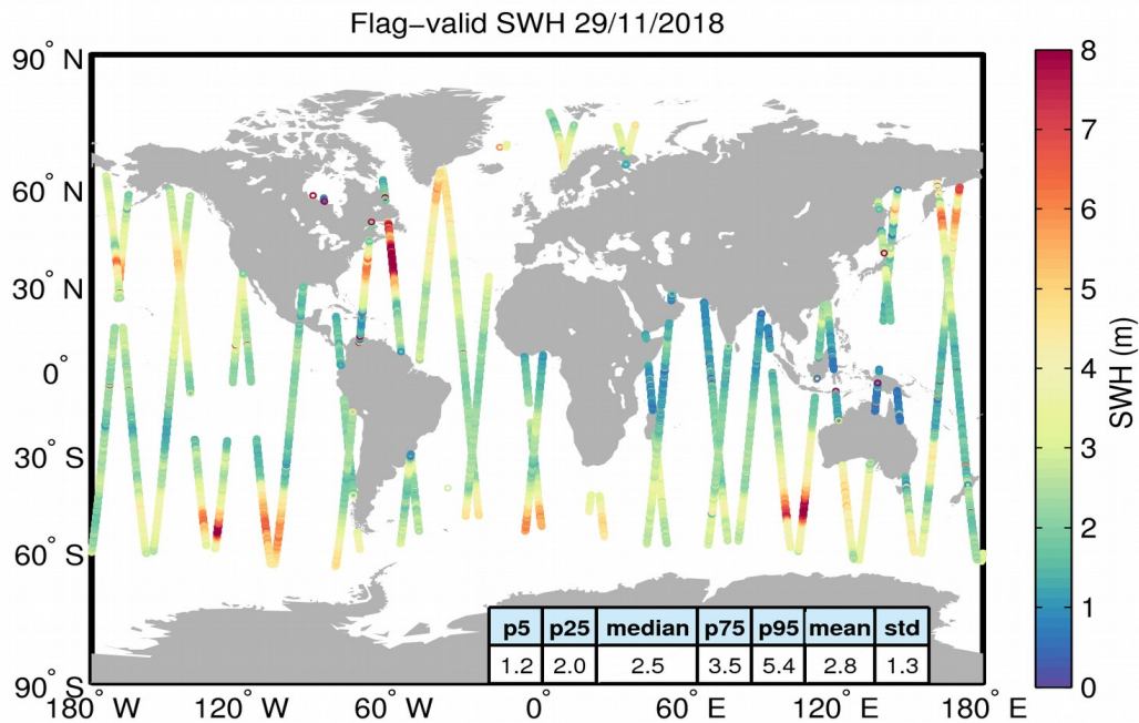
Figure 15. Geographical distribution of flag-valid SWH data over oceans and lakes for 29/11/2018. The statistical values shown in the table refer to the SWH in m and are calculated over all measurements shown in the figure.
