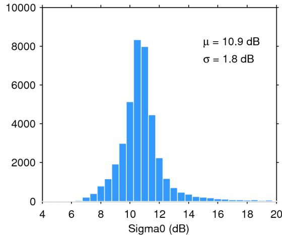
Figure 25. Histogram of flag-valid sigma0 over oceans and lakes for 29/11/2018. The mean ( \mu ) and standard deviation ( \sigma ) are also shown. Note that values outside [4 20] dB are excluded from the histogram for the sake of readability but not from the computation of \mu and \sigma .
