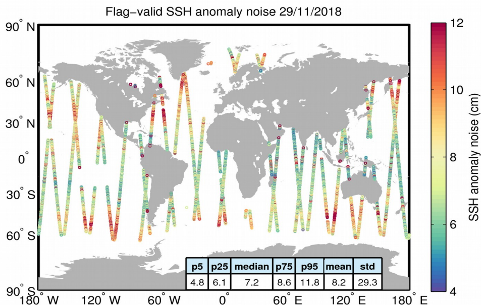
Figure 8. Geographical distribution of flag-valid 20-Hz SSH anomaly measurement noise over oceans and lakes for 29/11/2018. The statistical values shown in the table refer to the SSH anomaly noise and are calculated over all measurements shown in the figure.
