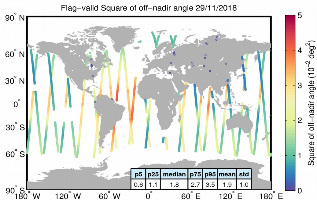
Figure 37. Geographical distribution of flag-valid mispointing data over oceans and lakes for 29/11/2018. The statistical values shown in the table refer to the mispointing in 10^{-2} \text{ deg}^2 and are calculated over all measurements shown in the figure.
