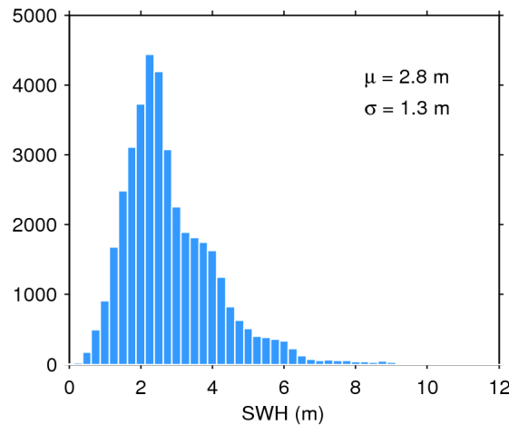
Figure 20. Histogram of science-valid SWH over oceans and lakes for 29/11/2018. The mean ( \mu ) and standard deviation ( \sigma ) are also shown. Note that values larger than 12 m are excluded from the histogram for the sake of readability but not from the computation of \mu and \sigma .
