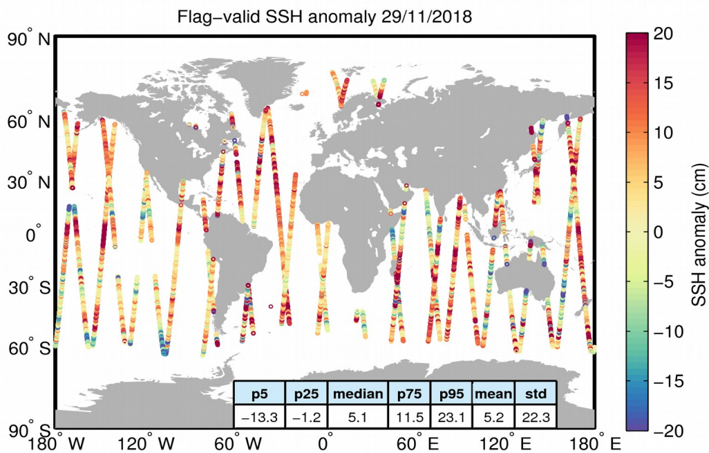
Figure 5. Geographical distribution of flag-valid 1-Hz SSH anomaly data over oceans and lakes for 29/11/2018. The statistical values shown in the table refer to the SSH anomaly in cm and are calculated over all measurements shown in the figure.
