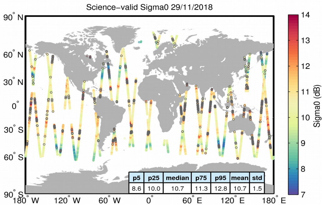
Figure 27. Geographical distribution of science-valid sigma0 data over oceans and lakes for 29/11/2018. The statistical values shown in the table refer to the sigma0 in dB and are calculated over all measurements shown in the figure. Gray circles denote records that have been rejected based on the editing criteria described in Table 4.
