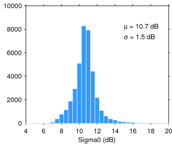
Figure 28. Histogram of science-valid sigma0 over oceans and lakes for 29/11/2018. The mean ( \mu ) and standard deviation ( \sigma ) are also shown. Note that values outside [4 20] dB are excluded from the histogram for the sake of readability but not from the computation of \mu and \sigma .
