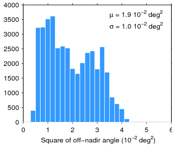
Figure 39. Histogram of flag-valid mispointing over oceans and lakes for 29/11/2018. The mean ( \mu ) and standard deviation ( \sigma ) are also shown. Note that values larger than 6 \cdot 10^{-2} \text{ deg}^2 are excluded from the histogram for the sake of readability but not from the computation of \mu and \sigma .
