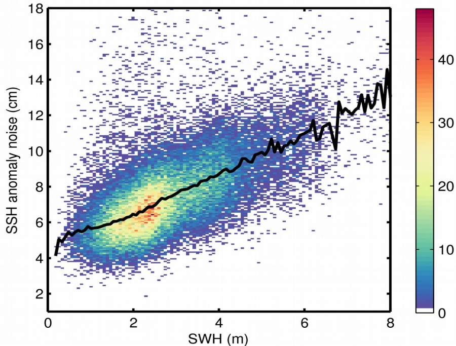
Figure 9. 2D histogram showing flag-valid SSH anomaly noise as a function of SWH for 29/11/2018. The black line denotes the median SSH anomaly noise as a function of SWH.
