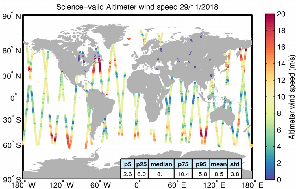
Figure 34. Geographical distribution of science-valid wind data over oceans and lakes for 29/11/2018. The statistical values shown in the table refer to the wind in m/s and are calculated over all measurements shown in the figure. Gray circles denote records that have been rejected based on the editing criteria described in Table 5.
