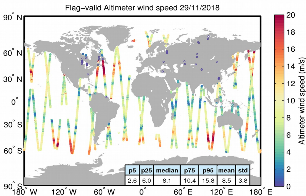
Figure 31. Geographical distribution of flag-valid wind data over oceans and lakes for 29/11/2018. The statistical values shown in the table refer to the wind in m/s and are calculated over all measurements shown in the figure.
