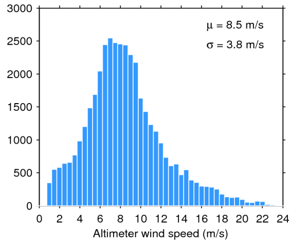
Figure 33. Histogram of flag-valid wind over oceans and lakes for 29/11/2018. The mean ( \mu ) and standard deviation ( \sigma ) are also shown. Note that values larger than 24 m/s are excluded from the histogram for the sake of readability but not from the computation of \mu and \sigma .
