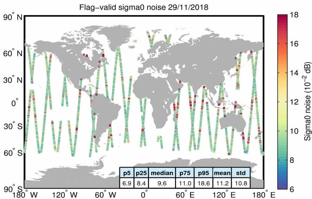
Figure 26. Geographical distribution of flag-valid 20-Hz sigma0 measurement noise over oceans and lakes for 29/11/2018. The statistical values shown in the table refer to the sigma0 noise and are calculated over all measurements shown in the figure.
