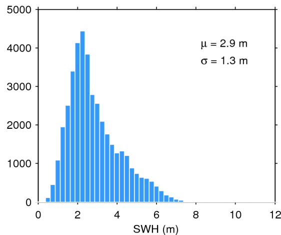
Figure 17. Histogram of flag-valid SWH over oceans and lakes for 28/11/2018. The mean ( \mu ) and standard deviation ( \sigma ) are also shown. Note that values larger than 12 m are excluded from the histogram for the sake of readability but not from the computation of \mu and \sigma .
