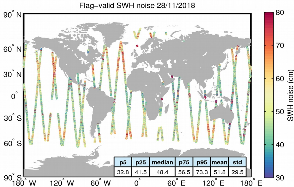
Figure 18. Geographical distribution of flag-valid 20-Hz SWH measurement noise over oceans and lakes for 28/11/2018. The statistical values shown in the figure refer to the SWH noise and are calculated over all measurements shown in the figure.
