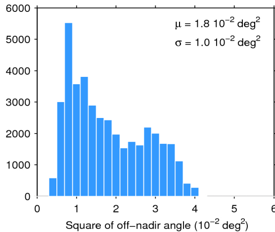
Figure 39. Histogram of flag-valid mispointing over oceans and lakes for 28/11/2018. The mean ( \mu ) and standard deviation ( \sigma ) are also shown. Note that values larger than 6 \cdot 10^{-2} \text{ deg}^2 are excluded from the histogram for the sake of readability but not from the computation of \mu and \sigma .
