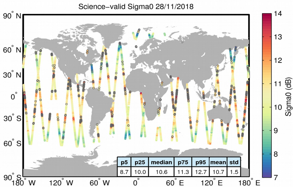
Figure 27. Geographical distribution of science-valid sigma0 data over oceans and lakes for 28/11/2018. The statistical values shown in the table refer to the sigma0 in dB and are calculated over all measurements shown in the figure. Gray circles denote records that have been rejected based on the editing criteria described in Table 4.
