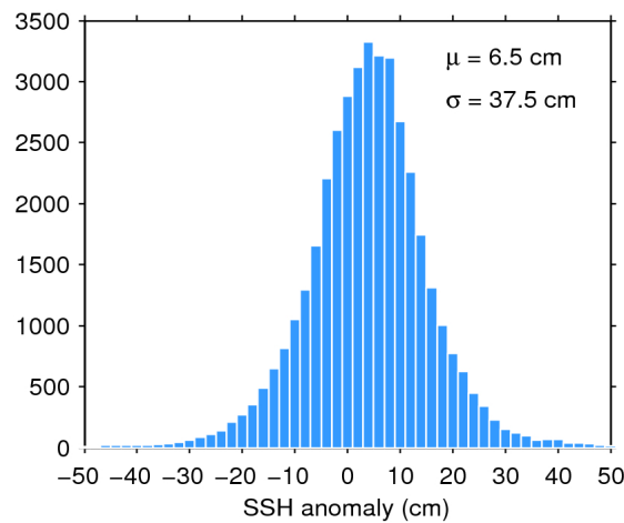
Figure 7. Histogram of flag-valid SSH anomaly over oceans and lakes for 28/11/2018. The mean ( \mu ) and standard deviation ( \sigma ) are also shown. Note that values outside [-50\ 50] cm are excluded from the histogram for the sake of readability but not from the computation of \mu and \sigma .
