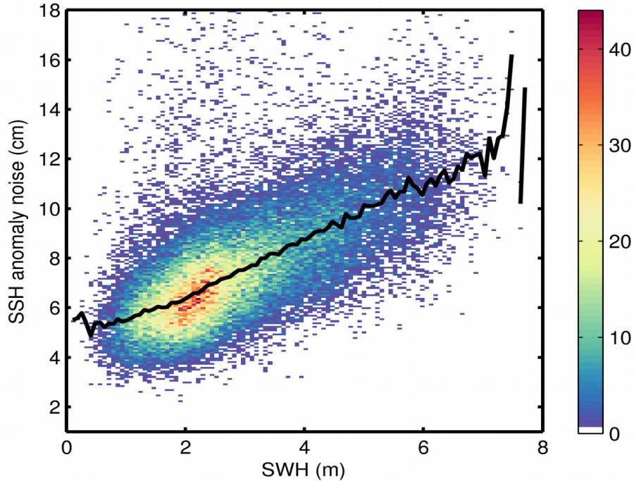
Figure 9. 2D histogram showing flag-valid SSH anomaly noise as a function of SWH for 28/11/2018. The black line denotes the median SSH anomaly noise as a function of SWH.
