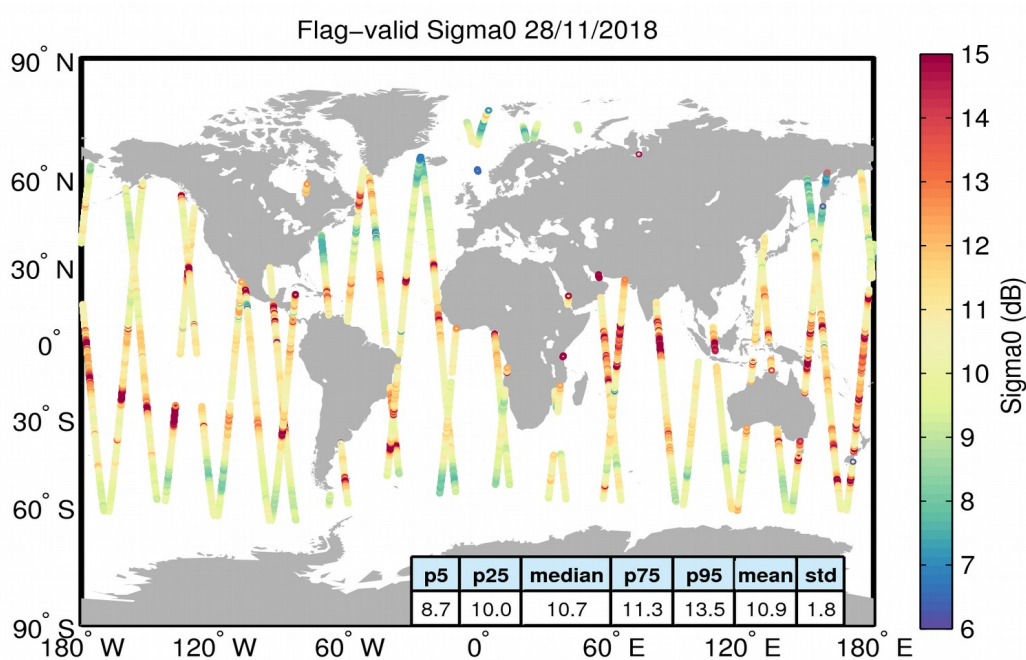
Figure 23. Geographical distribution of flag-valid sigma0 data over oceans and lakes for 28/11/2018. The statistical values shown in the table refer to the sigma0 in dB and are calculated over all measurements shown in the figure.
