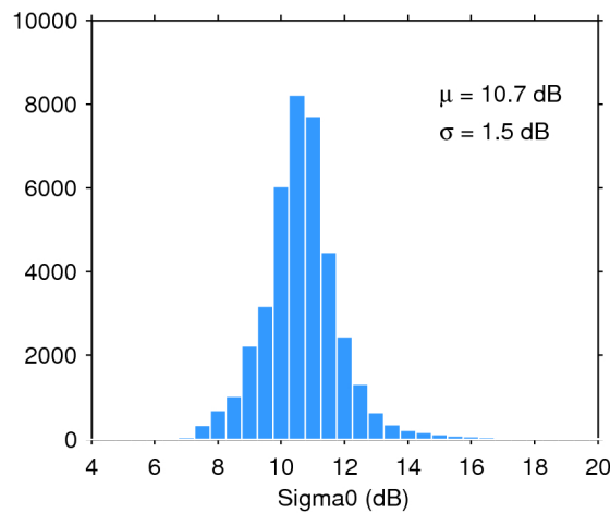
Figure 28. Histogram of science-valid sigma0 over oceans and lakes for 28/11/2018. The mean ( \mu ) and standard deviation ( \sigma ) are also shown. Note that values outside [4 20] dB are excluded from the histogram for the sake of readability but not from the computation of \mu and \sigma .
