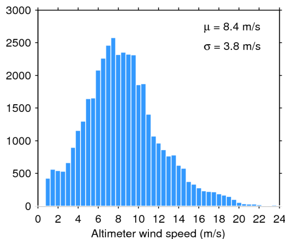
Figure 35. Histogram of science-valid wind over oceans and lakes for 28/11/2018. The mean ( \mu ) and standard deviation ( \sigma ) are also shown. Note that values larger than 24 m/s are excluded from the histogram for the sake of readability but not from the computation of \mu and \sigma .
