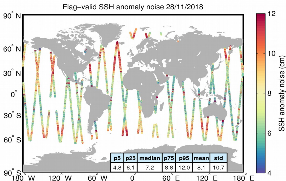
Figure 8. Geographical distribution of flag-valid 20-Hz SSH anomaly measurement noise over oceans and lakes for 28/11/2018. The statistical values shown in the table refer to the SSH anomaly noise and are calculated over all measurements shown in the figure.
