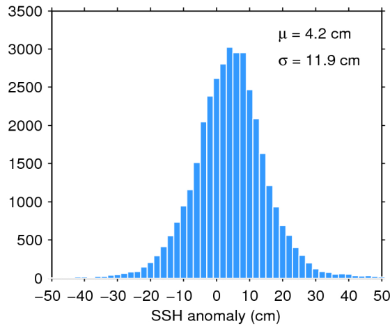
Figure 11. Histogram of science-valid SSH anomaly over oceans and lakes for 28/11/2018. The mean ( \mu ) and standard deviation ( \sigma ) are also shown. Note that values outside [-50 50] cm are excluded from the histogram for the sake of readability but not from the computation of \mu and \sigma .
