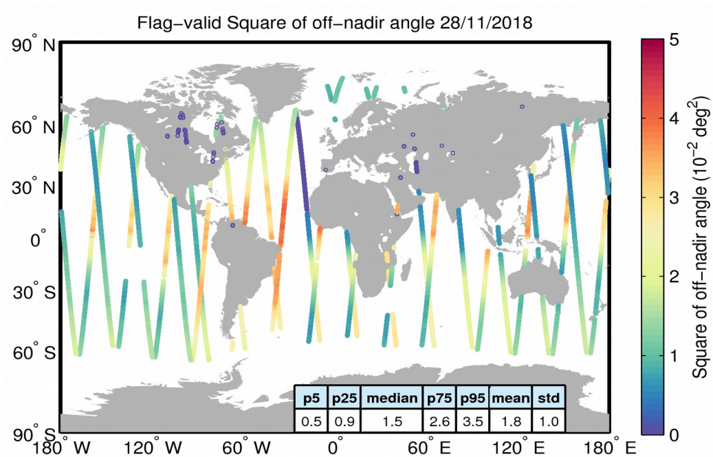
Figure 37. Geographical distribution of flag-valid mispointing data over oceans and lakes for 28/11/2018. The statistical values shown in the table refer to the mispointing in 10^{-2} \text{deg}^2 and are calculated over all measurements shown in the figure.
