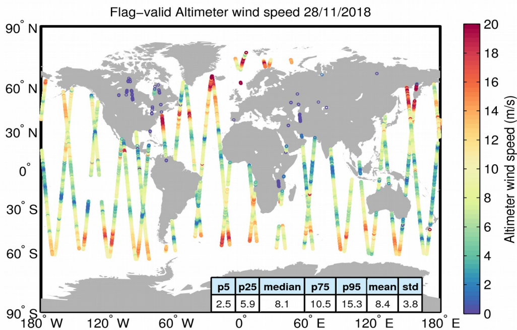
Figure 31. Geographical distribution of flag-valid wind data over oceans and lakes for 28/11/2018. The statistical values shown in the table refer to the wind in m/s and are calculated over all measurements shown in the figure.
