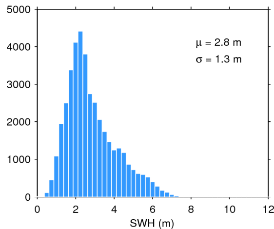
Figure 20. Histogram of science-valid SWH over oceans and lakes for 28/11/2018. The mean ( \mu ) and standard deviation ( \sigma ) are also shown. Note that values larger than 12 m are excluded from the histogram for the sake of readability but not from the computation of \mu and \sigma .
