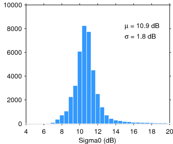
Figure 25. Histogram of flag-valid sigma0 over oceans and lakes for 28/11/2018. The mean ( \mu ) and standard deviation ( \sigma ) are also shown. Note that values outside [4 20] dB are excluded from the histogram for the sake of readability but not from the computation of \mu and \sigma .
