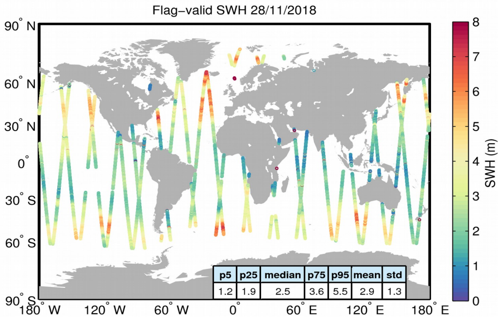
Figure 15. Geographical distribution of flag-valid SWH data over oceans and lakes for 28/11/2018. The statistical values shown in the table refer to the SWH in m and are calculated over all measurements shown in the figure.
