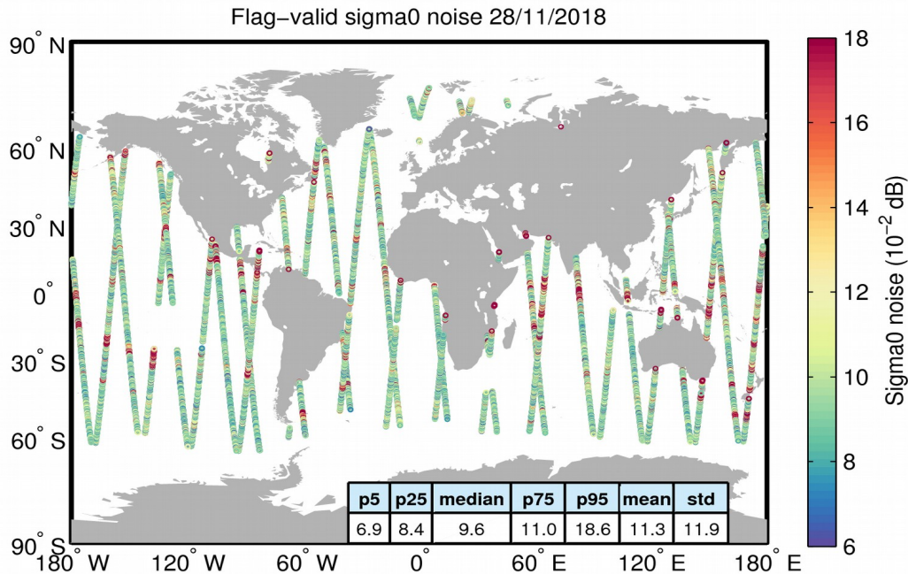
Figure 26. Geographical distribution of flag-valid 20-Hz sigma0 measurement noise over oceans and lakes for 28/11/2018. The statistical values shown in the table refer to the sigma0 noise and are calculated over all measurements shown in the figure.
