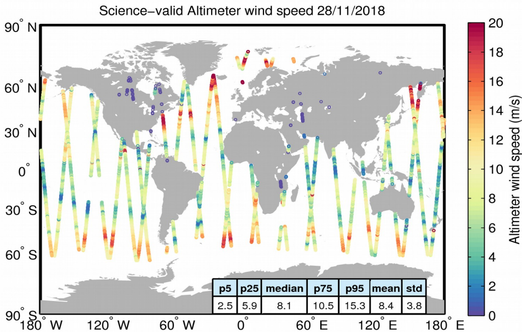
Figure 34. Geographical distribution of science-valid wind data over oceans and lakes for 28/11/2018. The statistical values shown in the table refer to the wind in m/s and are calculated over all measurements shown in the figure. Gray circles denote records that have been rejected based on the editing criteria described in Table 5.
