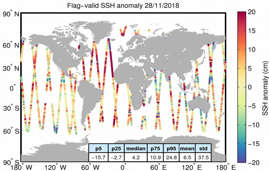
Figure 5. Geographical distribution of flag-valid 1-Hz SSH anomaly data over oceans and lakes for 28/11/2018. The statistical values shown in the table refer to the SSH anomaly in cm and are calculated over all measurements shown in the figure.
