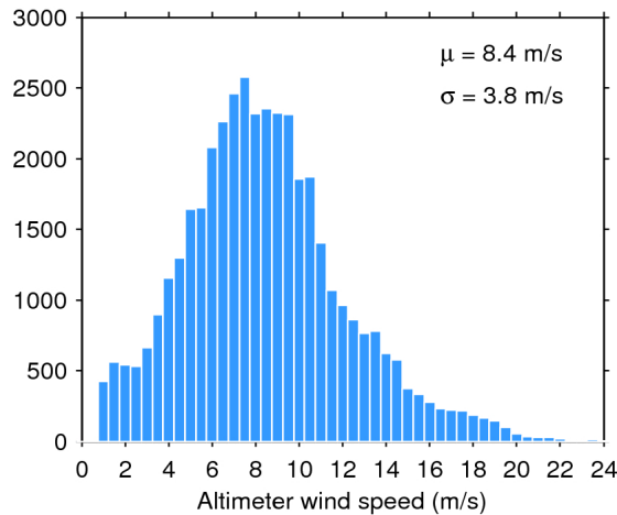
Figure 33. Histogram of flag-valid wind over oceans and lakes for 28/11/2018. The mean ( \mu ) and standard deviation ( \sigma ) are also shown. Note that values larger than 24 m/s are excluded from the histogram for the sake of readability but not from the computation of \mu and \sigma .
