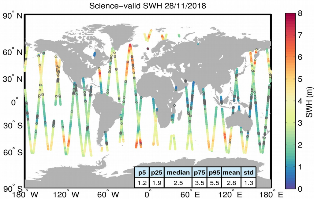
Figure 19. Geographical distribution of science-valid SWH data over oceans and lakes for 28/11/2018. The statistical values shown in the table refer to the SWH in m and are calculated over all measurements shown in the figure. Gray circles denote records that have been rejected based on the editing criteria described in Table 3.
