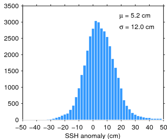
Figure 11. Histogram of science-valid SSH anomaly over oceans and lakes for 27/11/2018. The mean ( \mu ) and standard deviation ( \sigma ) are also shown. Note that values outside [-50 50] cm are excluded from the histogram for the sake of readability but not from the computation of \mu and \sigma .
