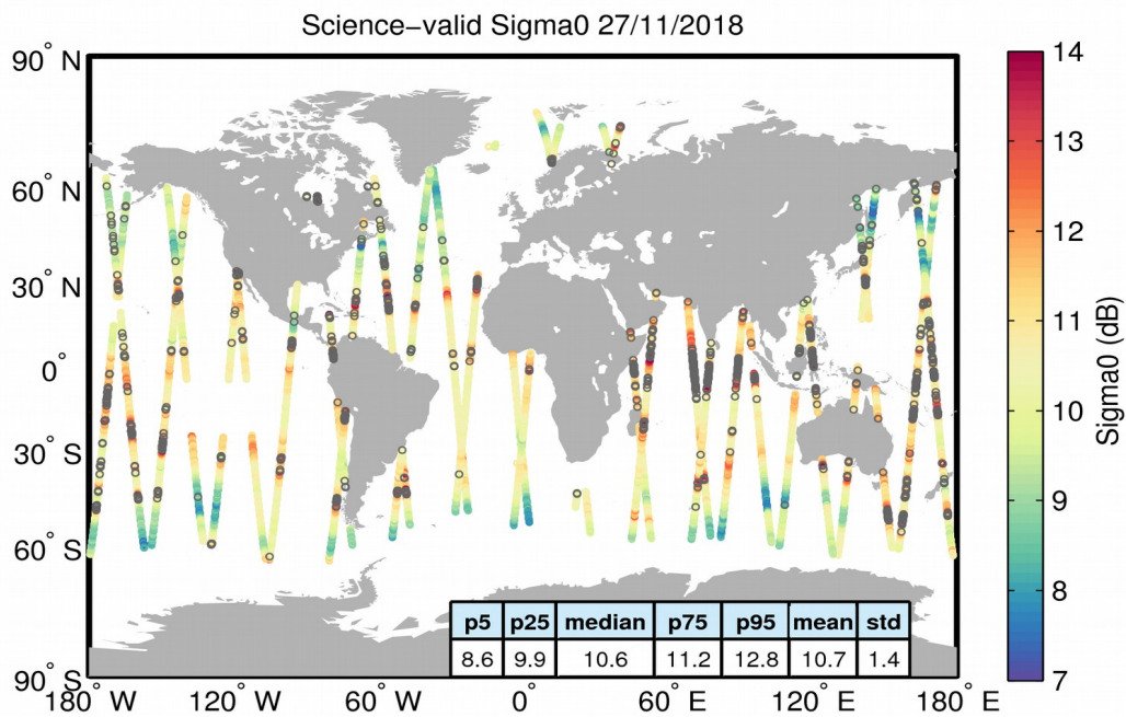
Figure 27. Geographical distribution of science-valid sigma0 data over oceans and lakes for 27/11/2018. The statistical values shown in the table refer to the sigma0 in dB and are calculated over all measurements shown in the figure. Gray circles denote records that have been rejected based on the editing criteria described in Table 4.
