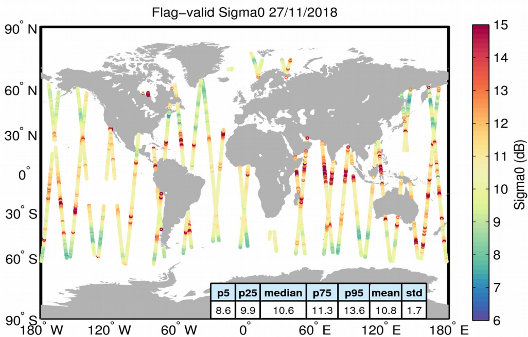
Figure 23. Geographical distribution of flag-valid sigma0 data over oceans and lakes for 27/11/2018. The statistical values shown in the table refer to the sigma0 in dB and are calculated over all measurements shown in the figure.
