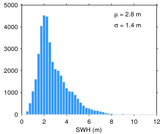
Figure 17. Histogram of flag-valid SWH over oceans and lakes for 27/11/2018. The mean ( \mu ) and standard deviation ( \sigma ) are also shown. Note that values larger than 12 m are excluded from the histogram for the sake of readability but not from the computation of \mu and \sigma .
