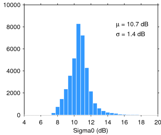
Figure 28. Histogram of science-valid sigma0 over oceans and lakes for 27/11/2018. The mean ( \mu ) and standard deviation ( \sigma ) are also shown. Note that values outside [4 20] dB are excluded from the histogram for the sake of readability but not from the computation of \mu and \sigma .
