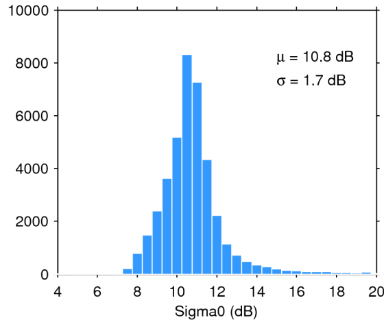
Figure 25. Histogram of flag-valid sigma0 over oceans and lakes for 27/11/2018. The mean ( \mu ) and standard deviation ( \sigma ) are also shown. Note that values outside [4 20] dB are excluded from the histogram for the sake of readability but not from the computation of \mu and \sigma .
