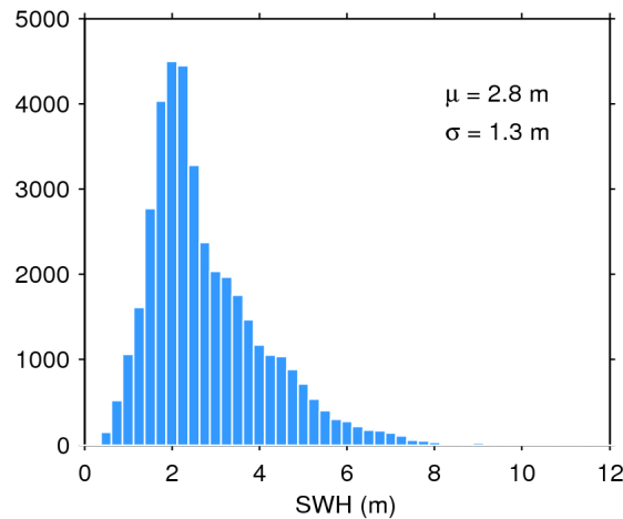
Figure 20. Histogram of science-valid SWH over oceans and lakes for 27/11/2018. The mean ( \mu ) and standard deviation ( \sigma ) are also shown. Note that values larger than 12 m are excluded from the histogram for the sake of readability but not from the computation of \mu and \sigma .
