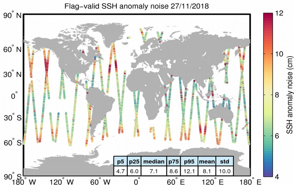
Figure 8. Geographical distribution of flag-valid 20-Hz SSH anomaly measurement noise over oceans and lakes for 27/11/2018. The statistical values shown in the table refer to the SSH anomaly noise and are calculated over all measurements shown in the figure.
