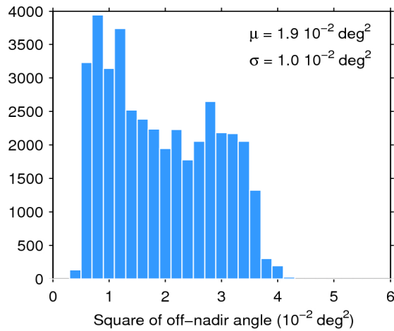
Figure 39. Histogram of flag-valid mispointing over oceans and lakes for 27/11/2018. The mean ( \mu ) and standard deviation ( \sigma ) are also shown. Note that values larger than 6 \cdot 10^{-2} \text{ deg}^2 are excluded from the histogram for the sake of readability but not from the computation of \mu and \sigma .
