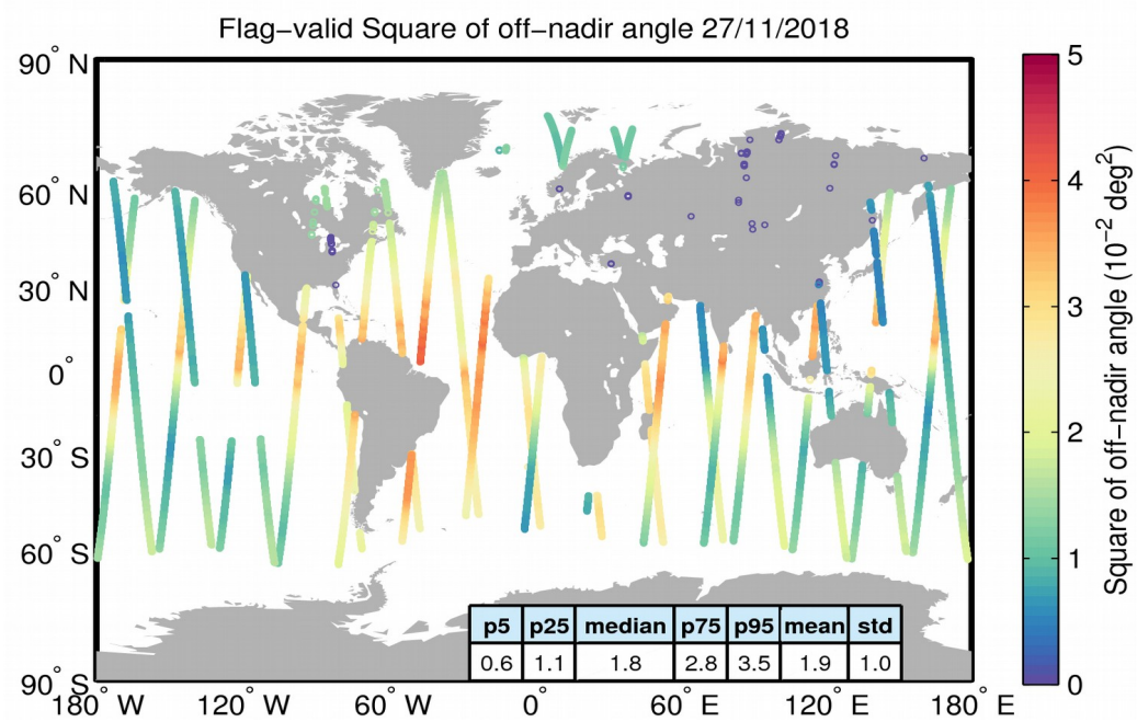
Figure 37. Geographical distribution of flag-valid mispointing data over oceans and lakes for 27/11/2018. The statistical values shown in the table refer to the mispointing in 10^{-2} \text{ deg}^2 and are calculated over all measurements shown in the figure.
