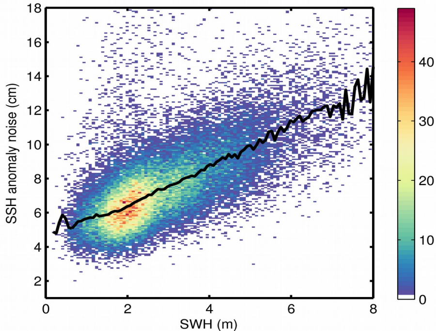
Figure 9. 2D histogram showing flag-valid SSH anomaly noise as a function of SWH for 27/11/2018. The black line denotes the median SSH anomaly noise as a function of SWH.
