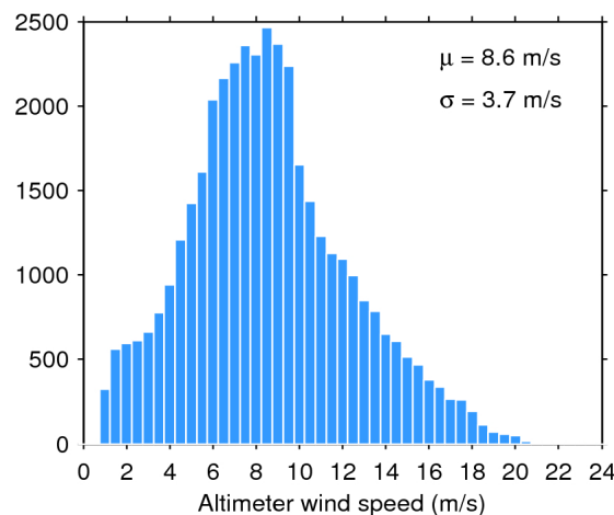
Figure 35. Histogram of science-valid wind over oceans and lakes for 27/11/2018. The mean ( \mu ) and standard deviation ( \sigma ) are also shown. Note that values larger than 24 m/s are excluded from the histogram for the sake of readability but not from the computation of \mu and \sigma .
