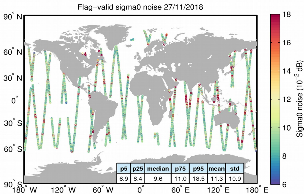
Figure 26. Geographical distribution of flag-valid 20-Hz sigma0 measurement noise over oceans and lakes for 27/11/2018. The statistical values shown in the table refer to the sigma0 noise and are calculated over all measurements shown in the figure.
