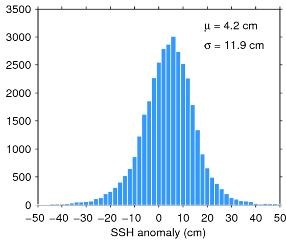
Figure 11. Histogram of science-valid SSH anomaly over oceans and lakes for 26/11/2018. The mean ( \mu ) and standard deviation ( \sigma ) are also shown. Note that values outside [-50 50] cm are excluded from the histogram for the sake of readability but not from the computation of \mu and \sigma .
