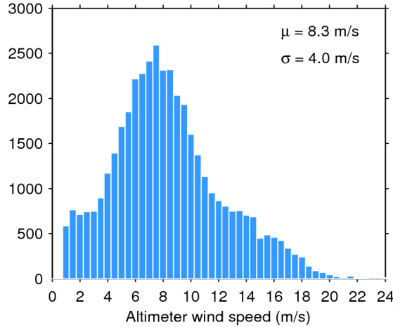
Figure 33. Histogram of flag-valid wind over oceans and lakes for 26/11/2018. The mean ( \mu ) and standard deviation ( \sigma ) are also shown. Note that values larger than 24 m/s are excluded from the histogram for the sake of readability but not from the computation of \mu and \sigma .
