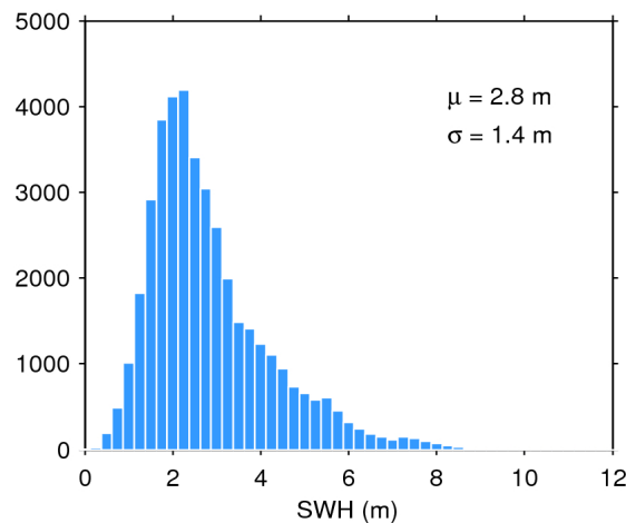
Figure 20. Histogram of science-valid SWH over oceans and lakes for 26/11/2018. The mean ( \mu ) and standard deviation ( \sigma ) are also shown. Note that values larger than 12 m are excluded from the histogram for the sake of readability but not from the computation of \mu and \sigma .
