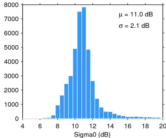
Figure 25. Histogram of flag-valid sigma0 over oceans and lakes for 26/11/2018. The mean ( \mu ) and standard deviation ( \sigma ) are also shown. Note that values outside [4 20] dB are excluded from the histogram for the sake of readability but not from the computation of \mu and \sigma .
