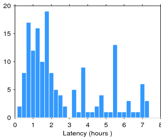
Figure 2. Histogram of the data latency for 26/11/2018. The y-axis denotes the number of files that are made available with a delay of x-hours with respect to the mean time of the records stored in the file.
