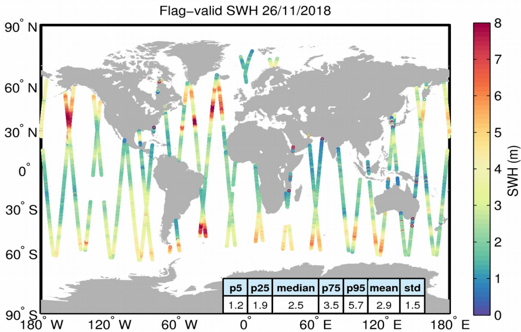
Figure 15. Geographical distribution of flag-valid SWH data over oceans and lakes for 26/11/2018. The statistical values shown in the table refer to the SWH in m and are calculated over all measurements shown in the figure.
