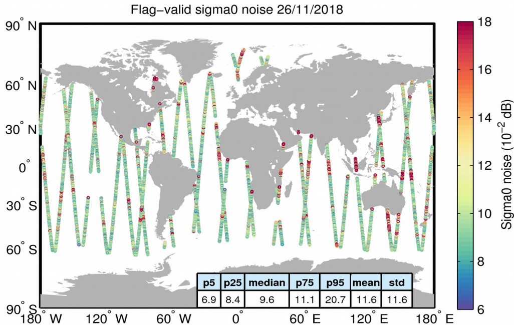
Figure 26. Geographical distribution of flag-valid 20-Hz sigma0 measurement noise over oceans and lakes for 26/11/2018. The statistical values shown in the table refer to the sigma0 noise and are calculated over all measurements shown in the figure.
