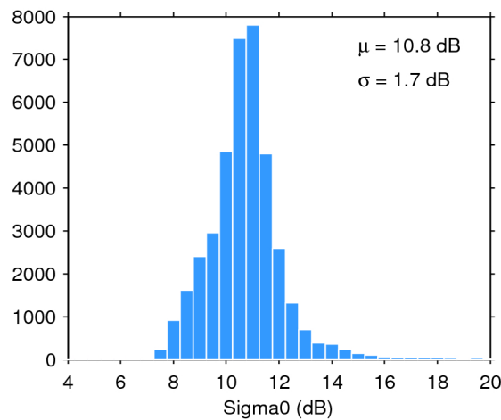
Figure 28. Histogram of science-valid sigma0 over oceans and lakes for 26/11/2018. The mean ( \mu ) and standard deviation ( \sigma ) are also shown. Note that values outside [4 20] dB are excluded from the histogram for the sake of readability but not from the computation of \mu and \sigma .
