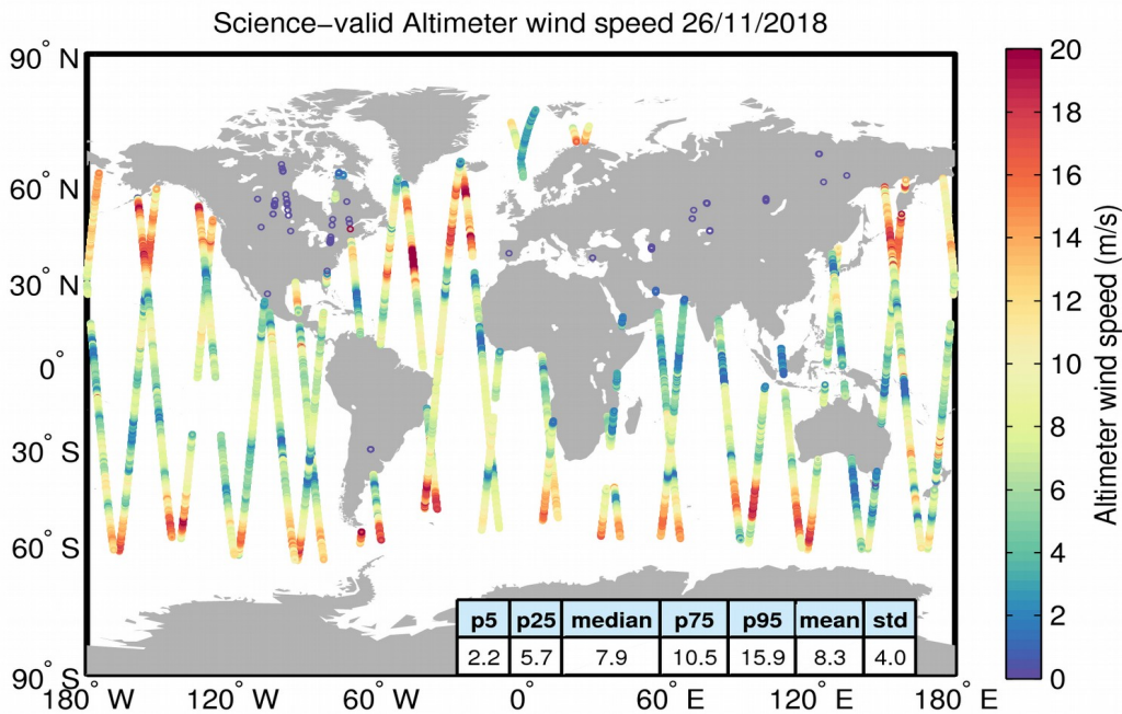
Figure 34. Geographical distribution of science-valid wind data over oceans and lakes for 26/11/2018. The statistical values shown in the table refer to the wind in m/s and are calculated over all measurements shown in the figure. Gray circles denote records that have been rejected based on the editing criteria described in Table 5.
