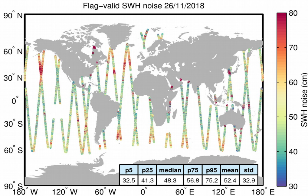
Figure 18. Geographical distribution of flag-valid 20-Hz SWH measurement noise over oceans and lakes for 26/11/2018. The statistical values shown in the figure refer to the SWH noise and are calculated over all measurements shown in the figure.
