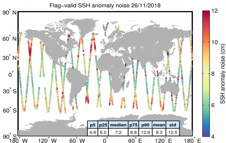
Figure 8. Geographical distribution of flag-valid 20-Hz SSH anomaly measurement noise over oceans and lakes for 26/11/2018. The statistical values shown in the table refer to the SSH anomaly noise and are calculated over all measurements shown in the figure.
