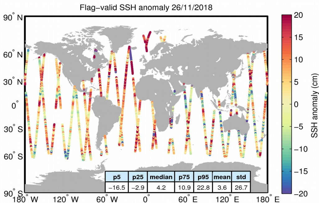
Figure 5. Geographical distribution of flag-valid 1-Hz SSH anomaly data over oceans and lakes for 26/11/2018. The statistical values shown in the table refer to the SSH anomaly in cm and are calculated over all measurements shown in the figure.
