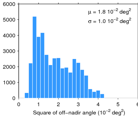
Figure 39. Histogram of flag-valid mispointing over oceans and lakes for 26/11/2018. The mean ( \mu ) and standard deviation ( \sigma ) are also shown. Note that values larger than 6 \cdot 10^{-2} \text{ deg}^2 are excluded from the histogram for the sake of readability but not from the computation of \mu and \sigma .
