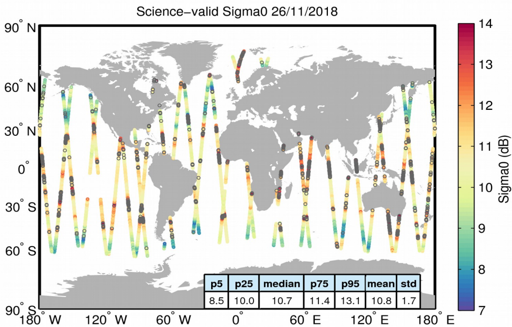
Figure 27. Geographical distribution of science-valid sigma0 data over oceans and lakes for 26/11/2018. The statistical values shown in the table refer to the sigma0 in dB and are calculated over all measurements shown in the figure. Gray circles denote records that have been rejected based on the editing criteria described in Table 4.
