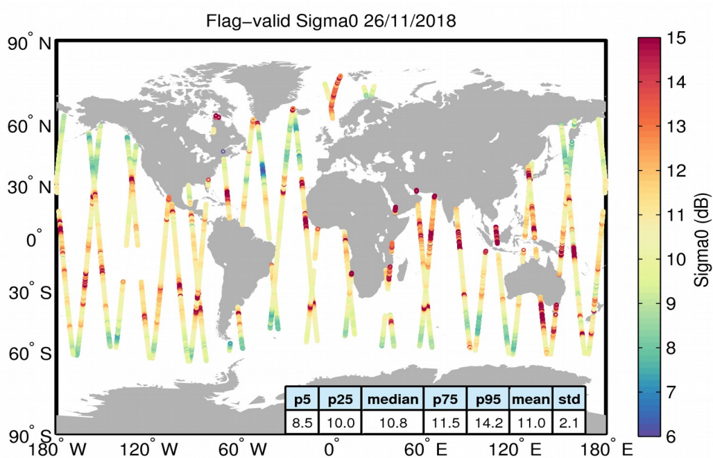
Figure 23. Geographical distribution of flag-valid sigma0 data over oceans and lakes for 26/11/2018. The statistical values shown in the table refer to the sigma0 in dB and are calculated over all measurements shown in the figure.
