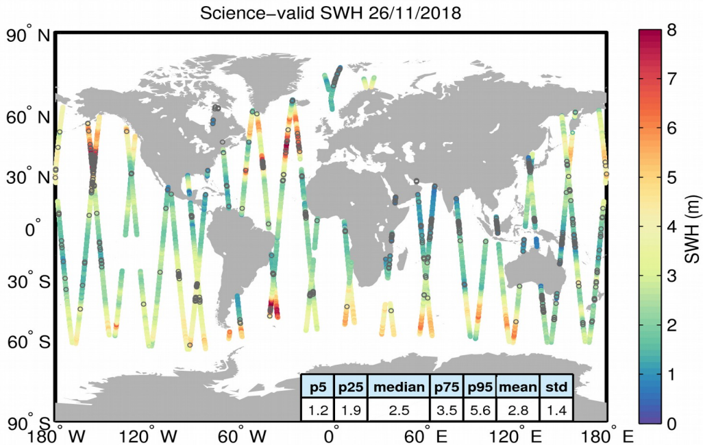
Figure 19. Geographical distribution of science-valid SWH data over oceans and lakes for 26/11/2018. The statistical values shown in the table refer to the SWH in m and are calculated over all measurements shown in the figure. Gray circles denote records that have been rejected based on the editing criteria described in Table 3.
