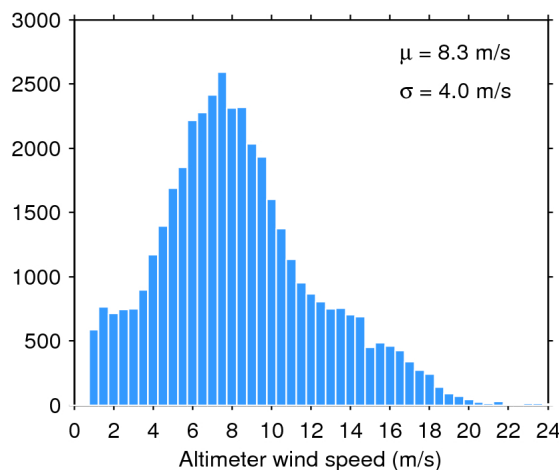
Figure 35. Histogram of science-valid wind over oceans and lakes for 26/11/2018. The mean ( \mu ) and standard deviation ( \sigma ) are also shown. Note that values larger than 24 m/s are excluded from the histogram for the sake of readability but not from the computation of \mu and \sigma .
