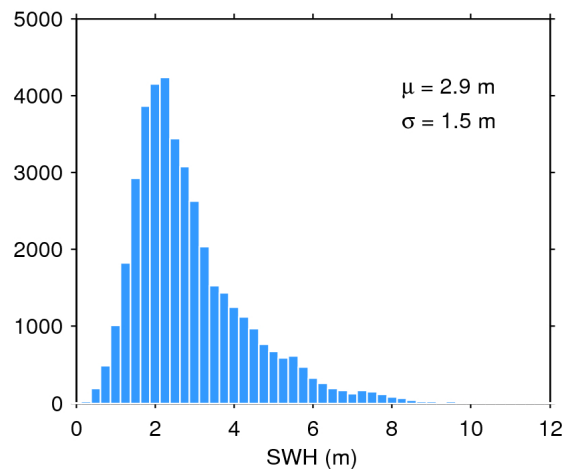
Figure 17. Histogram of flag-valid SWH over oceans and lakes for 26/11/2018. The mean ( \mu ) and standard deviation ( \sigma ) are also shown. Note that values larger than 12 m are excluded from the histogram for the sake of readability but not from the computation of \mu and \sigma .
