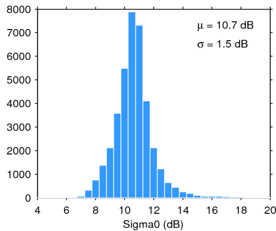
Figure 28. Histogram of science-valid sigma0 over oceans and lakes for 25/11/2018. The mean ( \mu ) and standard deviation ( \sigma ) are also shown. Note that values outside [4 20] dB are excluded from the histogram for the sake of readability but not from the computation of \mu and \sigma .
