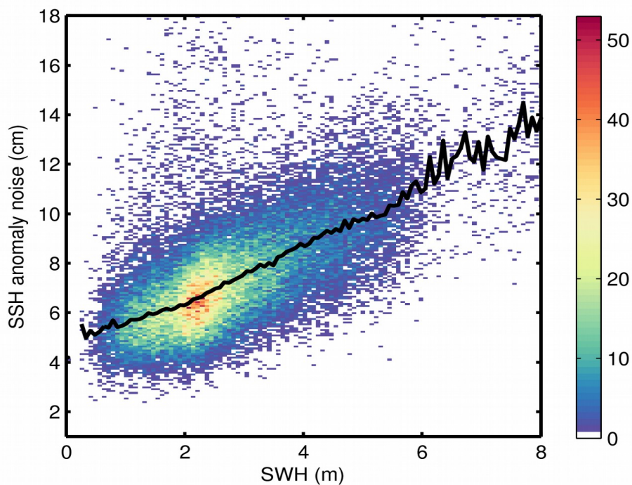
Figure 9. 2D histogram showing flag-valid SSH anomaly noise as a function of SWH for 25/11/2018. The black line denotes the median SSH anomaly noise as a function of SWH.
