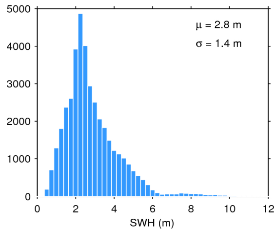
Figure 17. Histogram of flag-valid SWH over oceans and lakes for 25/11/2018. The mean ( \mu ) and standard deviation ( \sigma ) are also shown. Note that values larger than 12 m are excluded from the histogram for the sake of readability but not from the computation of \mu and \sigma .
