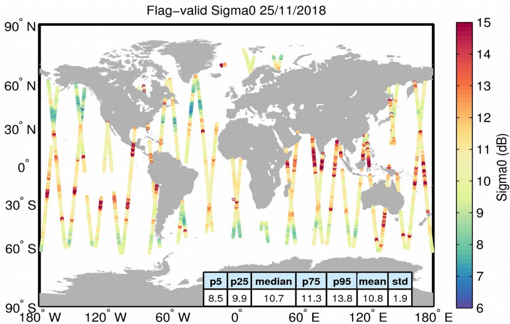
Figure 23. Geographical distribution of flag-valid sigma0 data over oceans and lakes for 25/11/2018. The statistical values shown in the table refer to the sigma0 in dB and are calculated over all measurements shown in the figure.
