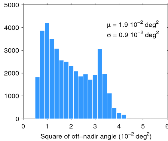
Figure 39. Histogram of flag-valid mispointing over oceans and lakes for 25/11/2018. The mean ( \mu ) and standard deviation ( \sigma ) are also shown. Note that values larger than 6 \cdot 10^{-2} \text{ deg}^2 are excluded from the histogram for the sake of readability but not from the computation of \mu and \sigma .
