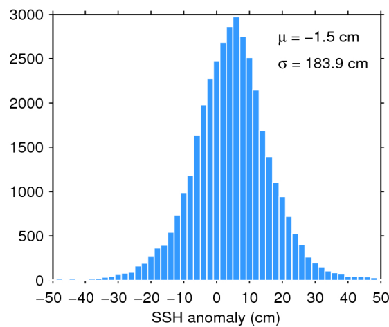
Figure 7. Histogram of flag-valid SSH anomaly over oceans and lakes for 25/11/2018. The mean ( \mu ) and standard deviation ( \sigma ) are also shown. Note that values outside [-50 50] cm are excluded from the histogram for the sake of readability but not from the computation of \mu and \sigma .
