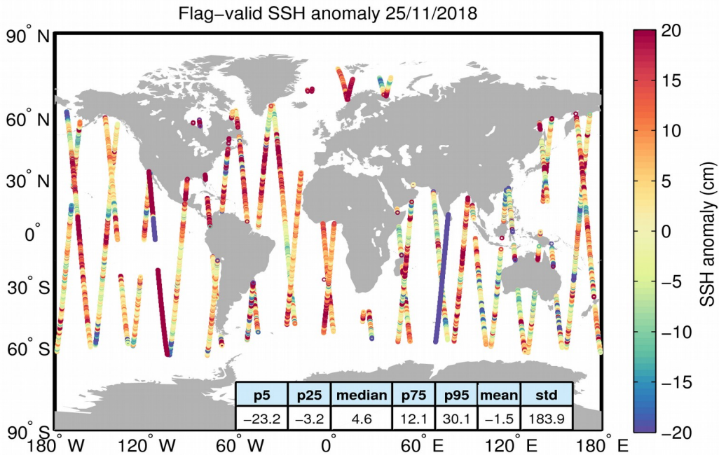
Figure 5. Geographical distribution of flag-valid 1-Hz SSH anomaly data over oceans and lakes for 25/11/2018. The statistical values shown in the table refer to the SSH anomaly in cm and are calculated over all measurements shown in the figure.
