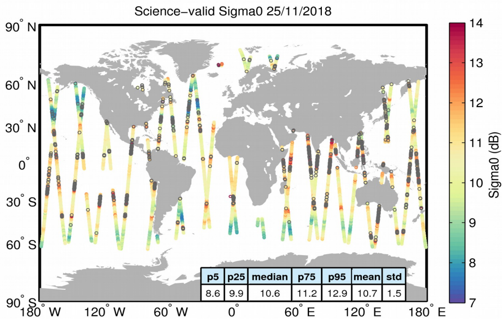
Figure 27. Geographical distribution of science-valid sigma0 data over oceans and lakes for 25/11/2018. The statistical values shown in the table refer to the sigma0 in dB and are calculated over all measurements shown in the figure. Gray circles denote records that have been rejected based on the editing criteria described in Table 4.
