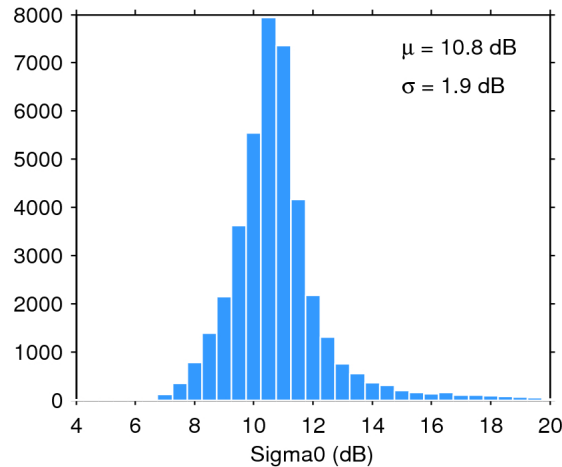
Figure 25. Histogram of flag-valid sigma0 over oceans and lakes for 25/11/2018. The mean ( \mu ) and standard deviation ( \sigma ) are also shown. Note that values outside [4 20] dB are excluded from the histogram for the sake of readability but not from the computation of \mu and \sigma .
