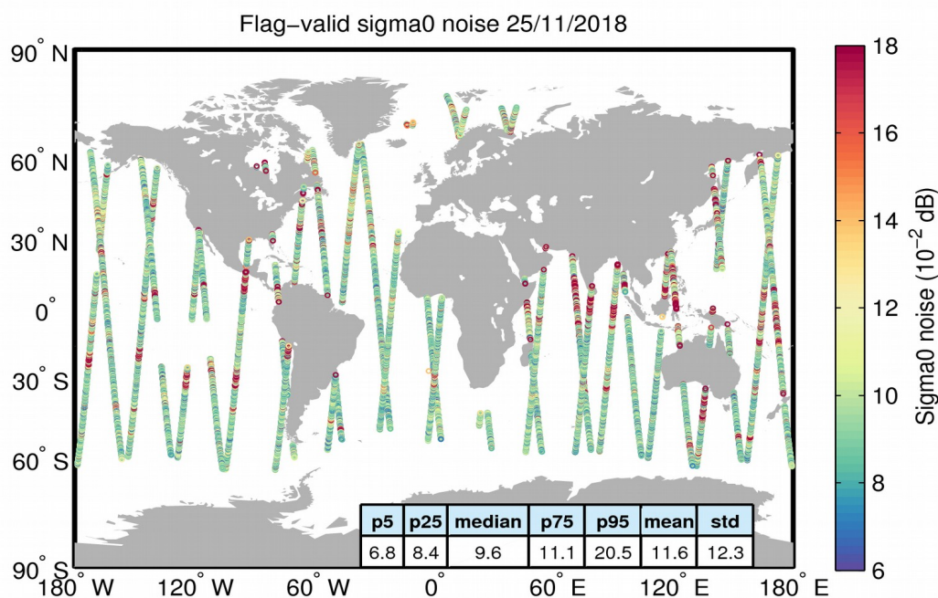
Figure 26. Geographical distribution of flag-valid 20-Hz sigma0 measurement noise over oceans and lakes for 25/11/2018. The statistical values shown in the table refer to the sigma0 noise and are calculated over all measurements shown in the figure.
