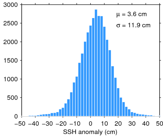
Figure 11. Histogram of science-valid SSH anomaly over oceans and lakes for 24/11/2018. The mean ( \mu ) and standard deviation ( \sigma ) are also shown. Note that values outside [-50 50] cm are excluded from the histogram for the sake of readability but not from the computation of \mu and \sigma .
