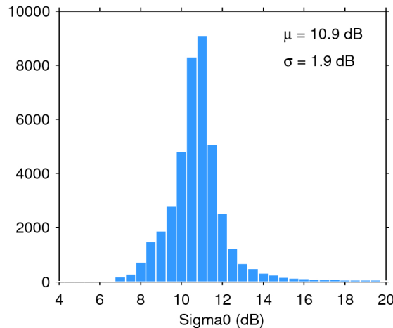
Figure 25. Histogram of flag-valid sigma0 over oceans and lakes for 24/11/2018. The mean ( \mu ) and standard deviation ( \sigma ) are also shown. Note that values outside [4 20] dB are excluded from the histogram for the sake of readability but not from the computation of \mu and \sigma .
