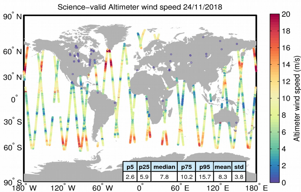
Figure 34. Geographical distribution of science-valid wind data over oceans and lakes for 24/11/2018. The statistical values shown in the table refer to the wind in m/s and are calculated over all measurements shown in the figure. Gray circles denote records that have been rejected based on the editing criteria described in Table 5.
