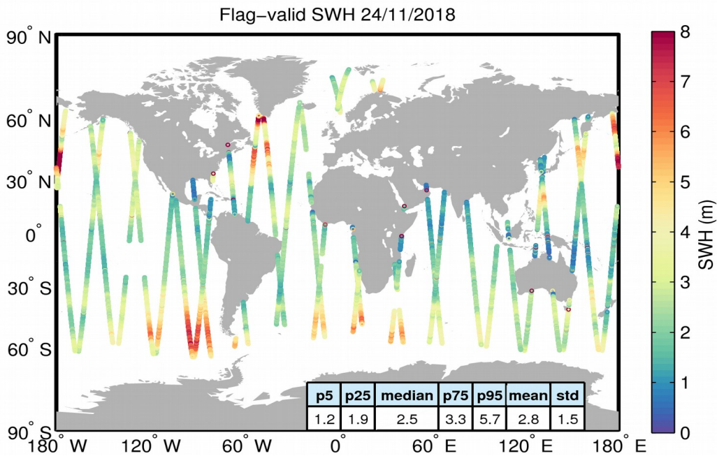
Figure 15. Geographical distribution of flag-valid SWH data over oceans and lakes for 24/11/2018. The statistical values shown in the table refer to the SWH in m and are calculated over all measurements shown in the figure.
