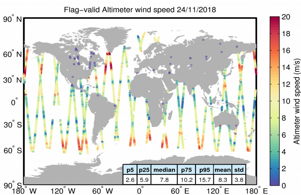
Figure 31. Geographical distribution of flag-valid wind data over oceans and lakes for 24/11/2018. The statistical values shown in the figure refer to the wind in m/s and are calculated over all measurements shown in the figure.
