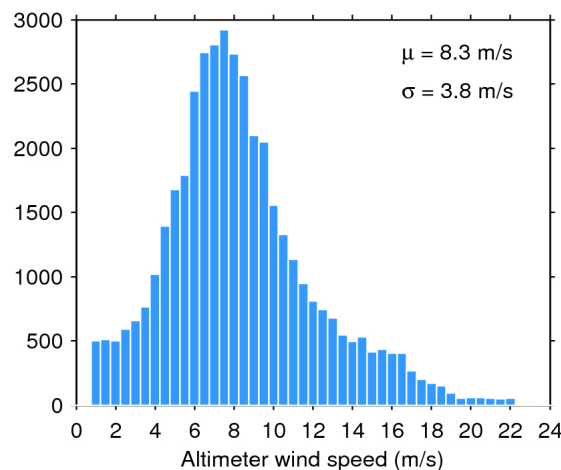
Figure 35. Histogram of science-valid wind over oceans and lakes for 24/11/2018. The mean ( \mu ) and standard deviation ( \sigma ) are also shown. Note that values larger than 24 m/s are excluded from the histogram for the sake of readability but not from the computation of \mu and \sigma .
