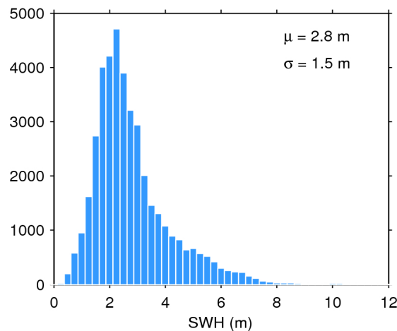
Figure 17. Histogram of flag-valid SWH over oceans and lakes for 24/11/2018. The mean ( \mu ) and standard deviation ( \sigma ) are also shown. Note that values larger than 12 m are excluded from the histogram for the sake of readability but not from the computation of \mu and \sigma .
