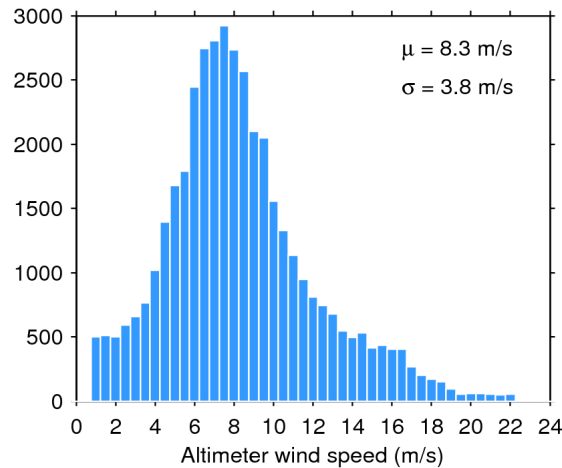
Figure 33. Histogram of flag-valid wind over oceans and lakes for 24/11/2018. The mean ( \mu ) and standard deviation ( \sigma ) are also shown. Note that values larger than 24 m/s are excluded from the histogram for the sake of readability but not from the computation of \mu and \sigma .
