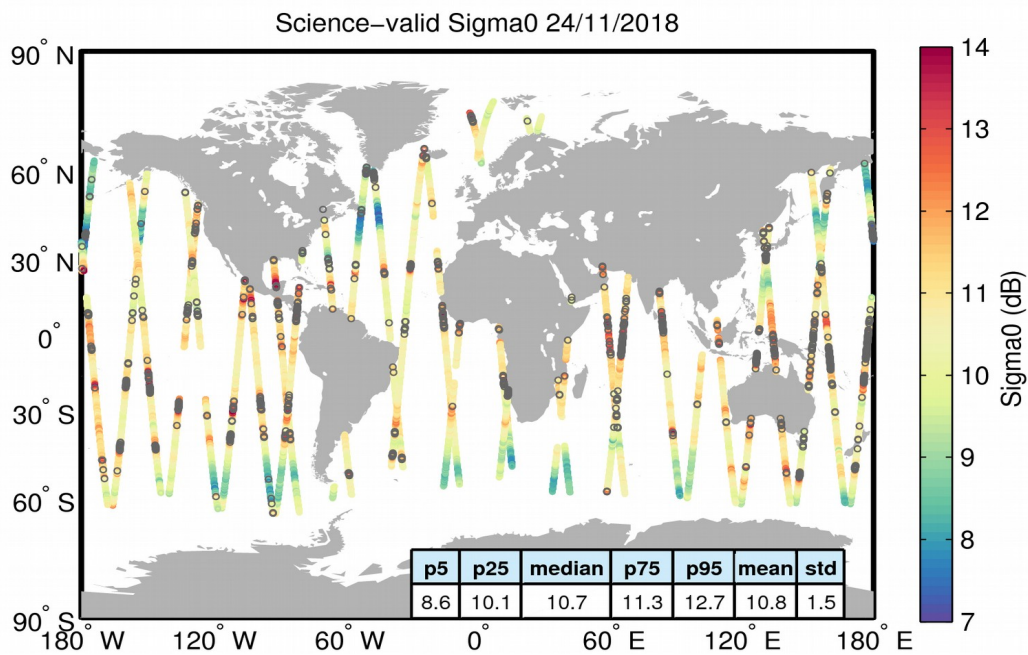
Figure 27. Geographical distribution of science-valid sigma0 data over oceans and lakes for 24/11/2018. The statistical values shown in the table refer to the sigma0 in dB and are calculated over all measurements shown in the figure. Gray circles denote records that have been rejected based on the editing criteria described in Table 4.
