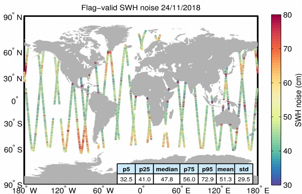
Figure 18. Geographical distribution of flag-valid 20-Hz SWH measurement noise over oceans and lakes for 24/11/2018. The statistical values shown in the figure refer to the SWH noise and are calculated over all measurements shown in the figure.
