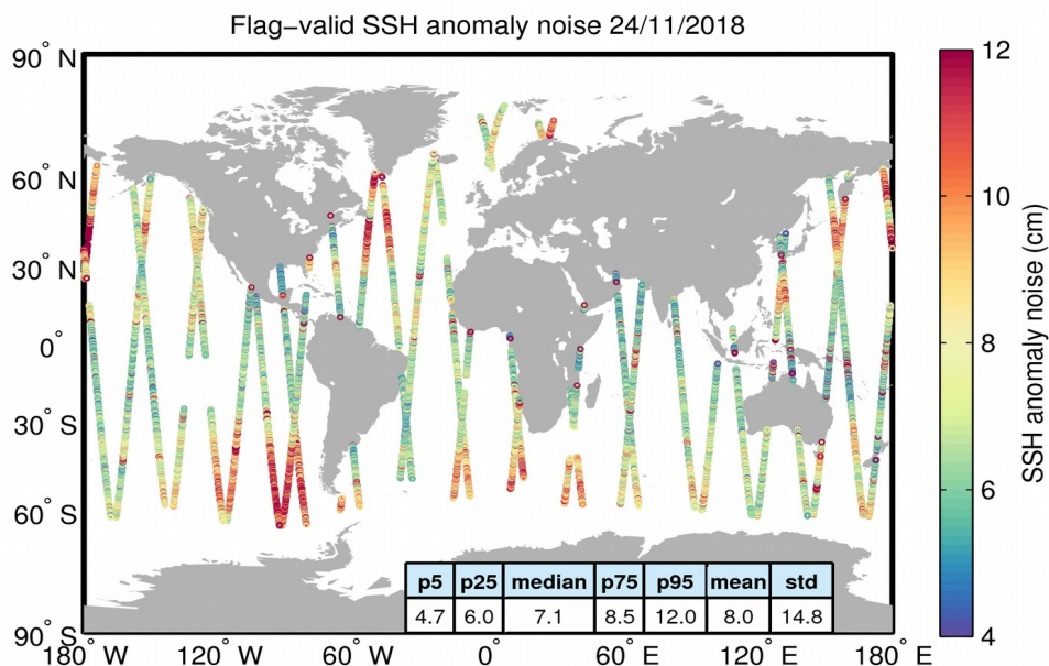
Figure 8. Geographical distribution of flag-valid 20-Hz SSH anomaly measurement noise over oceans and lakes for 24/11/2018. The statistical values shown in the table refer to the SSH anomaly noise and are calculated over all measurements shown in the figure.
