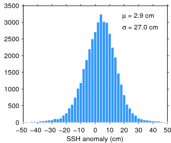
Figure 7. Histogram of flag-valid SSH anomaly over oceans and lakes for 24/11/2018. The mean ( \mu ) and standard deviation ( \sigma ) are also shown. Note that values outside [-50\ 50] cm are excluded from the histogram for the sake of readability but not from the computation of \mu and \sigma .
