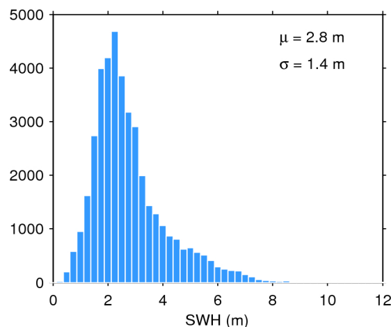
Figure 20. Histogram of science-valid SWH over oceans and lakes for 24/11/2018. The mean ( \mu ) and standard deviation ( \sigma ) are also shown. Note that values larger than 12 m are excluded from the histogram for the sake of readability but not from the computation of \mu and \sigma .
