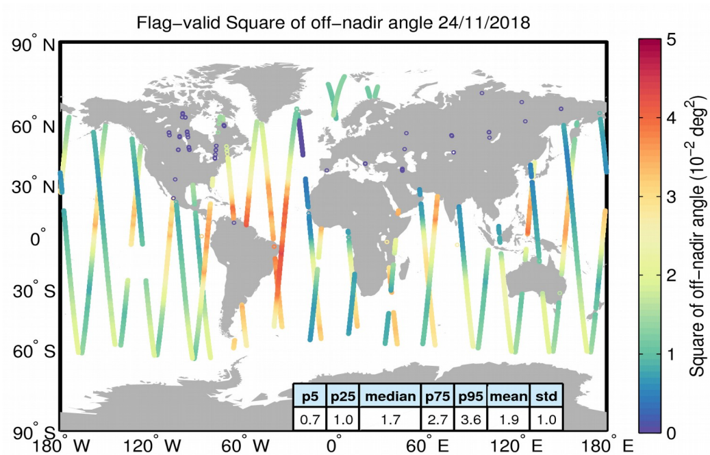
Figure 37. Geographical distribution of flag-valid mispointing data over oceans and lakes for 24/11/2018. The statistical values shown in the table refer to the mispointing in 10^{-2} deg 2 and are calculated over all measurements shown in the figure.
