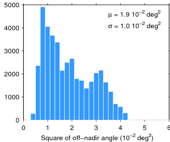
Figure 39. Histogram of flag-valid mispointing over oceans and lakes for 24/11/2018. The mean ( \mu ) and standard deviation ( \sigma ) are also shown. Note that values larger than 6 \cdot 10^{-2} \text{ deg}^2 are excluded from the histogram for the sake of readability but not from the computation of \mu and \sigma .
