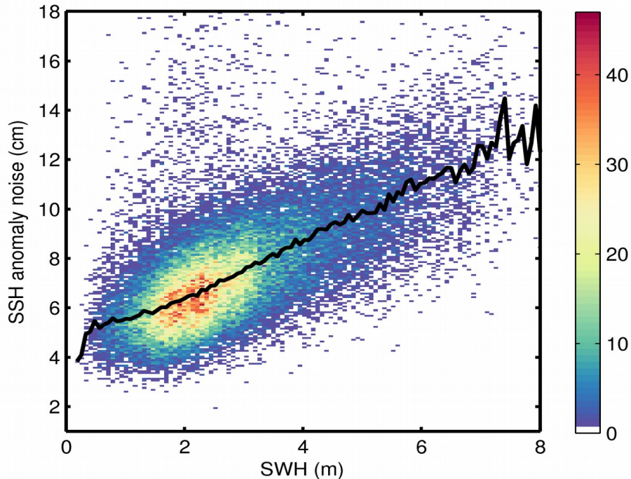
Figure 9. 2D histogram showing flag-valid SSH anomaly noise as a function of SWH for 24/11/2018. The black line denotes the median SSH anomaly noise as a function of SWH.
