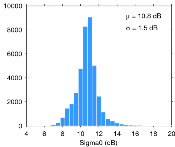
Figure 28. Histogram of science-valid sigma0 over oceans and lakes for 24/11/2018. The mean ( \mu ) and standard deviation ( \sigma ) are also shown. Note that values outside [4 20] dB are excluded from the histogram for the sake of readability but not from the computation of \mu and \sigma .
