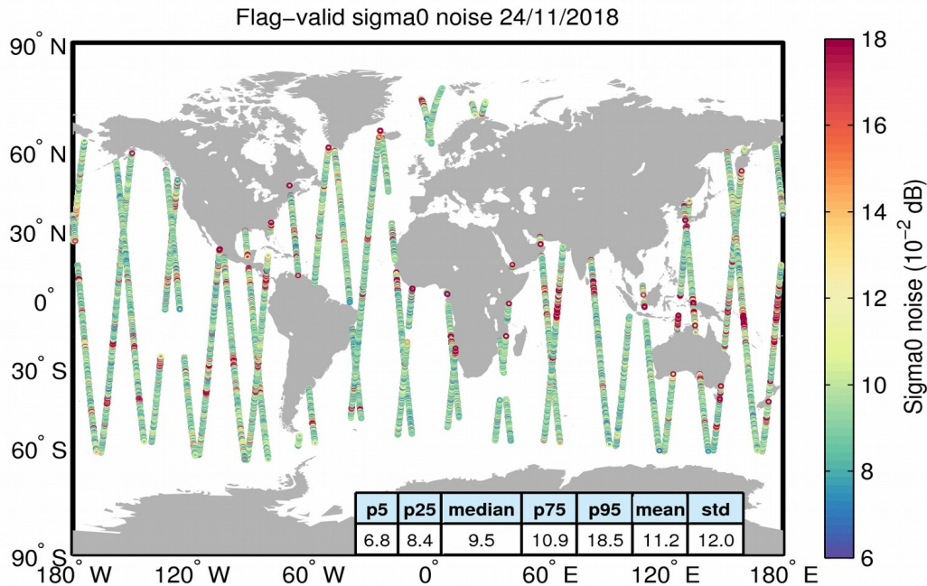
Figure 26. Geographical distribution of flag-valid 20-Hz sigma0 measurement noise over oceans and lakes for 24/11/2018. The statistical values shown in the table refer to the sigma0 noise and are calculated over all measurements shown in the figure.
