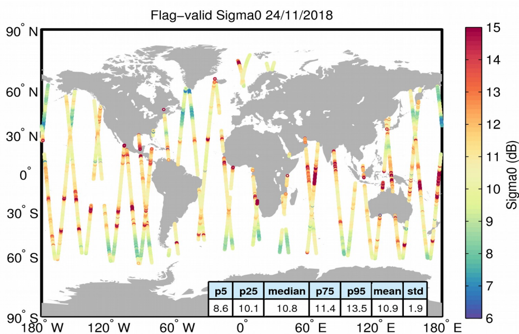
Figure 23. Geographical distribution of flag-valid sigma0 data over oceans and lakes for 24/11/2018. The statistical values shown in the table refer to the sigma0 in dB and are calculated over all measurements shown in the figure.
