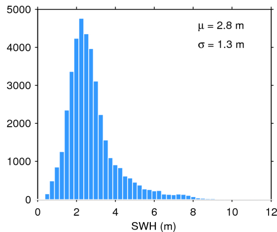
Figure 20. Histogram of science-valid SWH over oceans and lakes for 23/11/2018. The mean ( \mu ) and standard deviation ( \sigma ) are also shown. Note that values larger than 12 m are excluded from the histogram for the sake of readability but not from the computation of \mu and \sigma .
