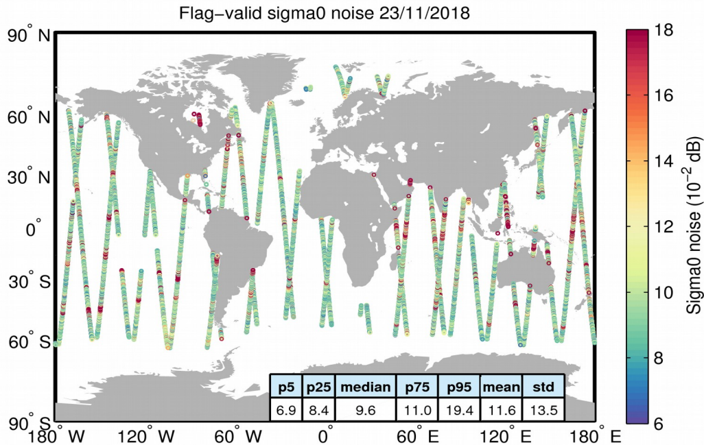
Figure 26. Geographical distribution of flag-valid 20-Hz sigma0 measurement noise over oceans and lakes for 23/11/2018. The statistical values shown in the table refer to the sigma0 noise and are calculated over all measurements shown in the figure.
