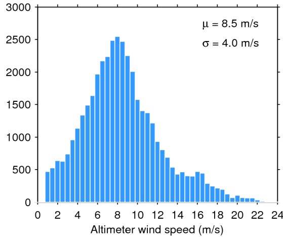
Figure 33. Histogram of flag-valid wind over oceans and lakes for 23/11/2018. The mean ( \mu ) and standard deviation ( \sigma ) are also shown. Note that values larger than 24 m/s are excluded from the histogram for the sake of readability but not from the computation of \mu and \sigma .
