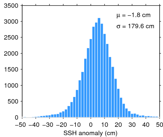
Figure 7. Histogram of flag-valid SSH anomaly over oceans and lakes for 23/11/2018. The mean ( \mu ) and standard deviation ( \sigma ) are also shown. Note that values outside [-50\ 50] cm are excluded from the histogram for the sake of readability but not from the computation of \mu and \sigma .
