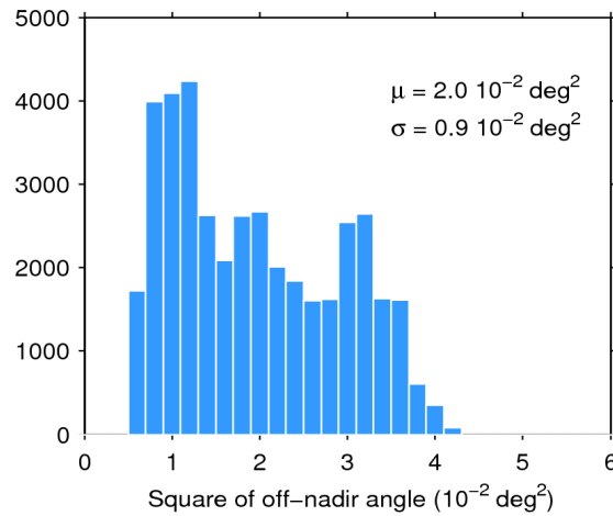
Figure 39. Histogram of flag-valid mispointing over oceans and lakes for 23/11/2018. The mean ( \mu ) and standard deviation ( \sigma ) are also shown. Note that values larger than 6 \cdot 10^{-2} \text{ deg}^2 are excluded from the histogram for the sake of readability but not from the computation of \mu and \sigma .
