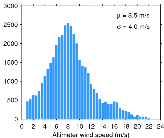
Figure 35. Histogram of science-valid wind over oceans and lakes for 23/11/2018. The mean ( \mu ) and standard deviation ( \sigma ) are also shown. Note that values larger than 24 m/s are excluded from the histogram for the sake of readability but not from the computation of \mu and \sigma .
