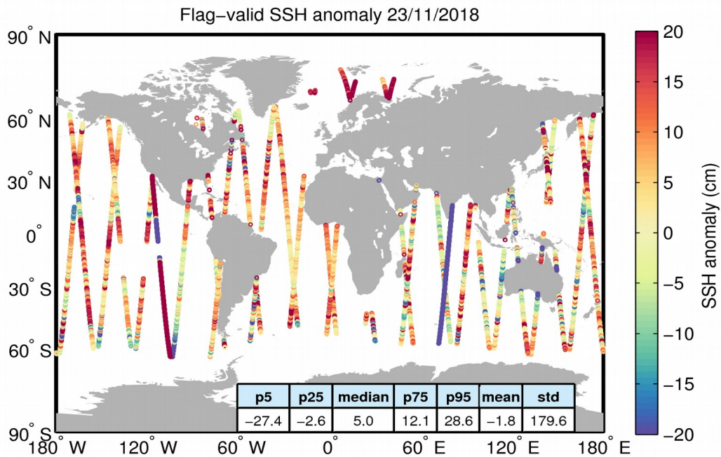
Figure 5. Geographical distribution of flag-valid 1-Hz SSH anomaly data over oceans and lakes for 23/11/2018. The statistical values shown in the table refer to the SSH anomaly in cm and are calculated over all measurements shown in the figure.
