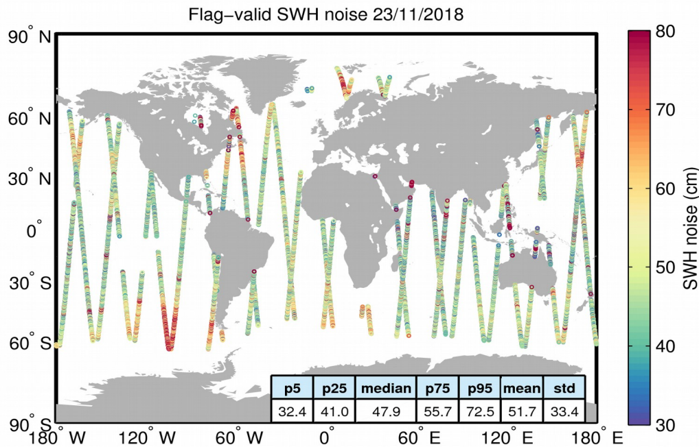
Figure 18. Geographical distribution of flag-valid 20-Hz SWH measurement noise over oceans and lakes for 23/11/2018. The statistical values shown in the figure refer to the SWH noise and are calculated over all measurements shown in the figure.
