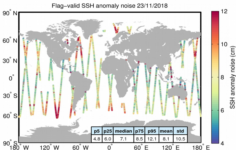
Figure 8. Geographical distribution of flag-valid 20-Hz SSH anomaly measurement noise over oceans and lakes for 23/11/2018. The statistical values shown in the table refer to the SSH anomaly noise and are calculated over all measurements shown in the figure.
