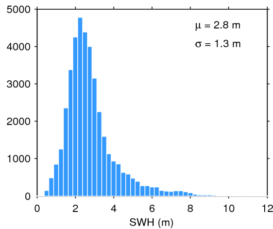
Figure 17. Histogram of flag-valid SWH over oceans and lakes for 23/11/2018. The mean ( \mu ) and standard deviation ( \sigma ) are also shown. Note that values larger than 12 m are excluded from the histogram for the sake of readability but not from the computation of \mu and \sigma .
