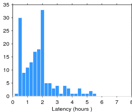
Figure 2. Histogram of the data latency for 23/11/2018. The y-axis denotes the number of files that are made available with a delay of x-hours with respect to the mean time of the records stored in the file.
