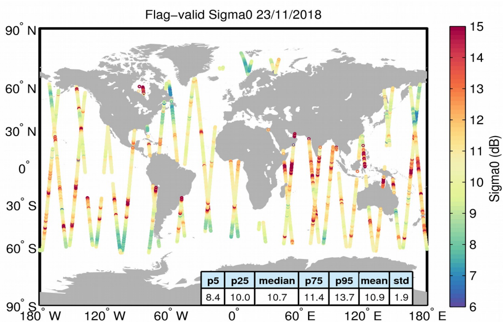
Figure 23. Geographical distribution of flag-valid sigma0 data over oceans and lakes for 23/11/2018. The statistical values shown in the table refer to the sigma0 in dB and are calculated over all measurements shown in the figure.
