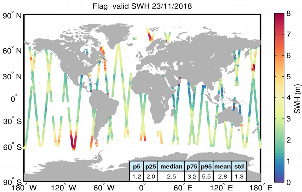
Figure 15. Geographical distribution of flag-valid SWH data over oceans and lakes for 23/11/2018. The statistical values shown in the table refer to the SWH in m and are calculated over all measurements shown in the figure.
