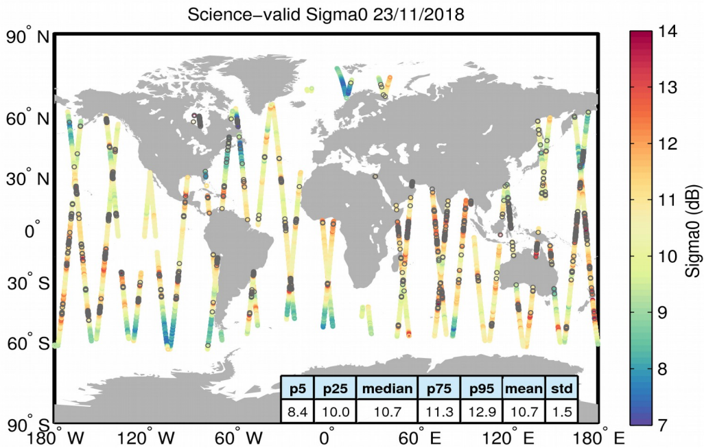
Figure 27. Geographical distribution of science-valid sigma0 data over oceans and lakes for 23/11/2018. The statistical values shown in the table refer to the sigma0 in dB and are calculated over all measurements shown in the figure. Gray circles denote records that have been rejected based on the editing criteria described in Table 4.
