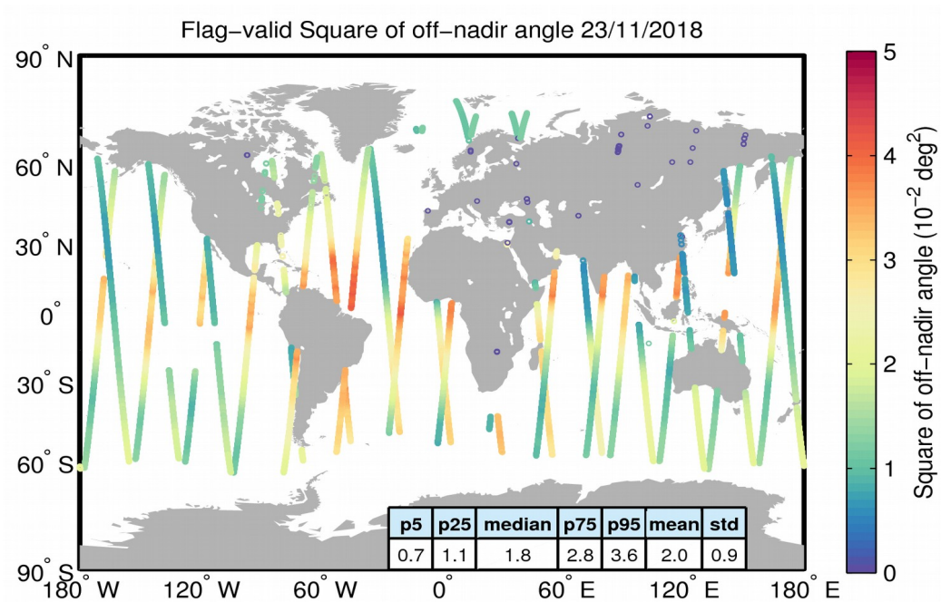
Figure 37. Geographical distribution of flag-valid mispointing data over oceans and lakes for 23/11/2018. The statistical values shown in the table refer to the mispointing in 10^{-2} deg 2 and are calculated over all measurements shown in the figure.
