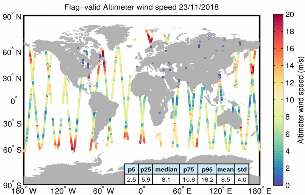
Figure 31. Geographical distribution of flag-valid wind data over oceans and lakes for 23/11/2018. The statistical values shown in the table refer to the wind in m/s and are calculated over all measurements shown in the figure.
