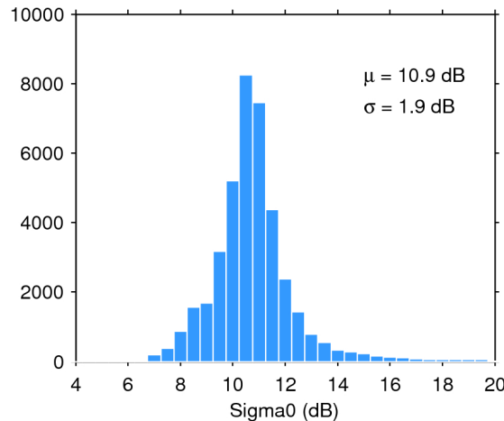
Figure 25. Histogram of flag-valid sigma0 over oceans and lakes for 23/11/2018. The mean ( \mu ) and standard deviation ( \sigma ) are also shown. Note that values outside [4 20] dB are excluded from the histogram for the sake of readability but not from the computation of \mu and \sigma .
