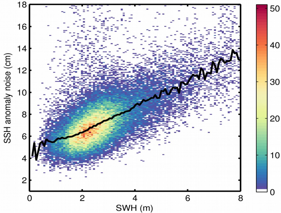
Figure 9. 2D histogram showing flag-valid SSH anomaly noise as a function of SWH for 23/11/2018. The black line denotes the median SSH anomaly noise as a function of SWH.
