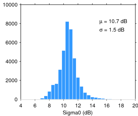
Figure 28. Histogram of science-valid sigma0 over oceans and lakes for 23/11/2018. The mean ( \mu ) and standard deviation ( \sigma ) are also shown. Note that values outside [4 20] dB are excluded from the histogram for the sake of readability but not from the computation of \mu and \sigma .
