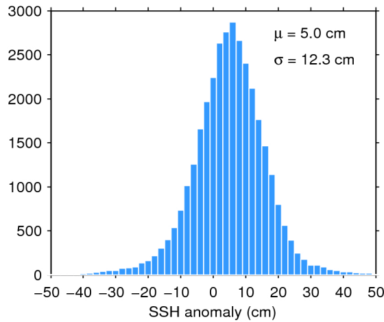
Figure 11. Histogram of science-valid SSH anomaly over oceans and lakes for 23/11/2018. The mean ( \mu ) and standard deviation ( \sigma ) are also shown. Note that values outside [-50 50] cm are excluded from the histogram for the sake of readability but not from the computation of \mu and \sigma .
