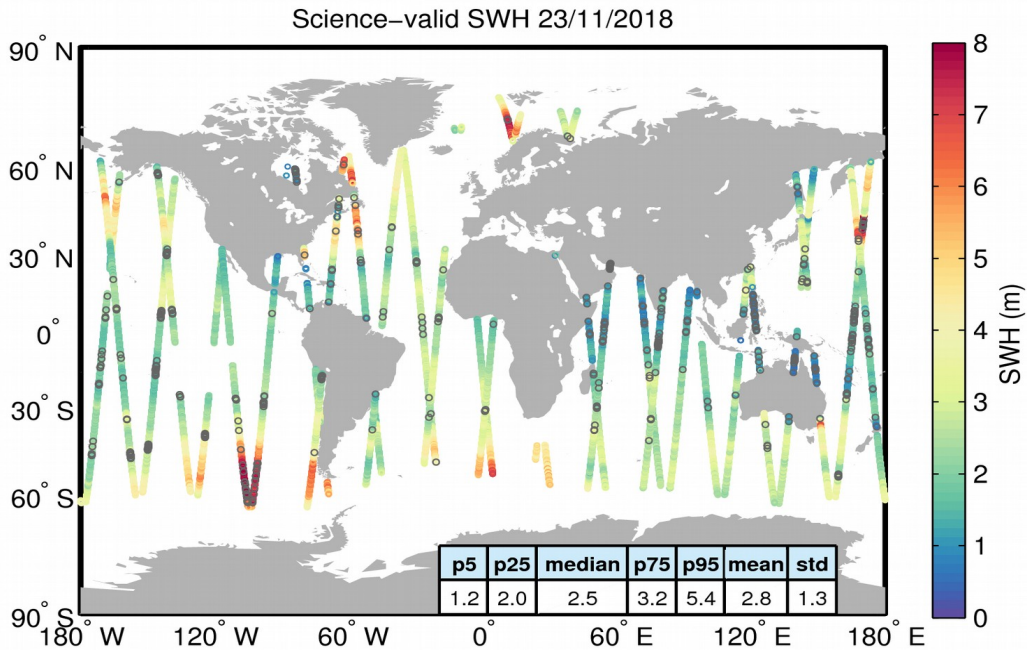
Figure 19. Geographical distribution of science-valid SWH data over oceans and lakes for 23/11/2018. The statistical values shown in the table refer to the SWH in m and are calculated over all measurements shown in the figure. Gray circles denote records that have been rejected based on the editing criteria described in Table 3.
