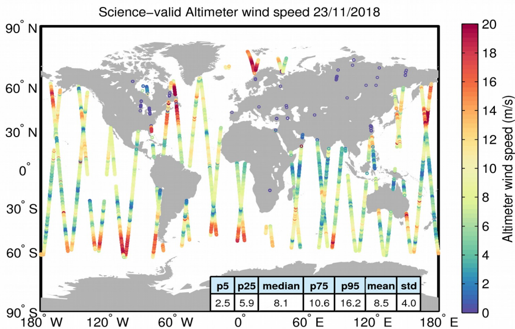
Figure 34. Geographical distribution of science-valid wind data over oceans and lakes for 23/11/2018. The statistical values shown in the table refer to the wind in m/s and are calculated over all measurements shown in the figure. Gray circles denote records that have been rejected based on the editing criteria described in Table 5.
