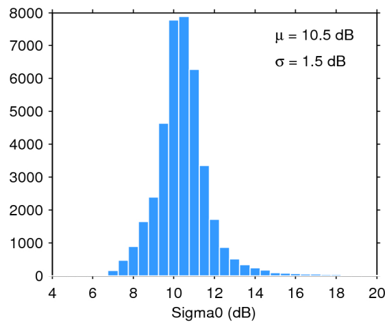
Figure 28. Histogram of science-valid sigma0 over oceans and lakes for 22/11/2018. The mean ( \mu ) and standard deviation ( \sigma ) are also shown. Note that values outside [4 20] dB are excluded from the histogram for the sake of readability but not from the computation of \mu and \sigma .
