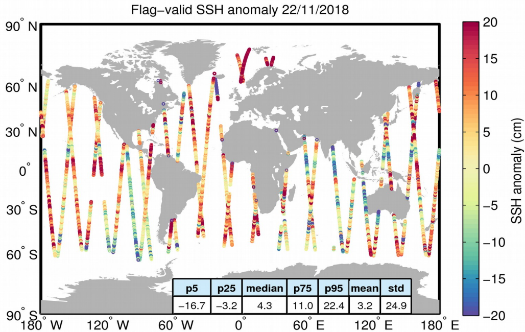
Figure 5. Geographical distribution of flag-valid 1-Hz SSH anomaly data over oceans and lakes for 22/11/2018. The statistical values shown in the table refer to the SSH anomaly in cm and are calculated over all measurements shown in the figure.
