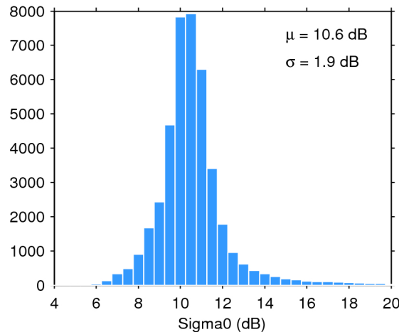
Figure 25. Histogram of flag-valid sigma0 over oceans and lakes for 22/11/2018. The mean ( \mu ) and standard deviation ( \sigma ) are also shown. Note that values outside [4 20] dB are excluded from the histogram for the sake of readability but not from the computation of \mu and \sigma .
