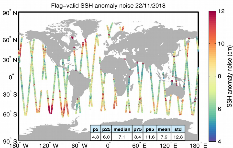
Figure 8. Geographical distribution of flag-valid 20-Hz SSH anomaly measurement noise over oceans and lakes for 22/11/2018. The statistical values shown in the table refer to the SSH anomaly noise and are calculated over all measurements shown in the figure.
