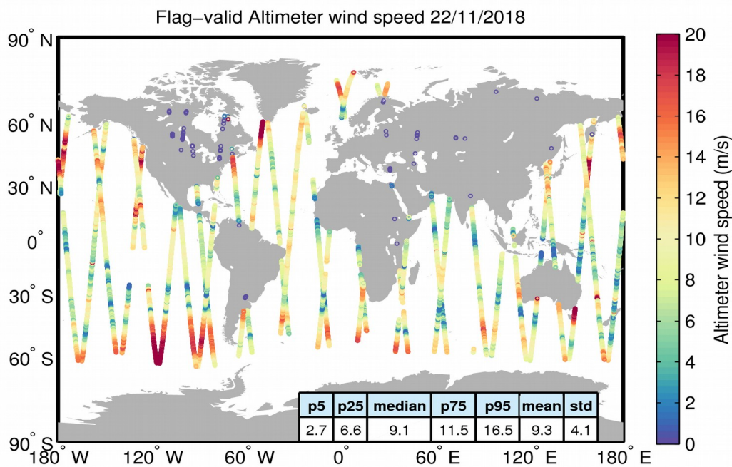
Figure 31. Geographical distribution of flag-valid wind data over oceans and lakes for 22/11/2018. The statistical values shown in the table refer to the wind in m/s and are calculated over all measurements shown in the figure.
