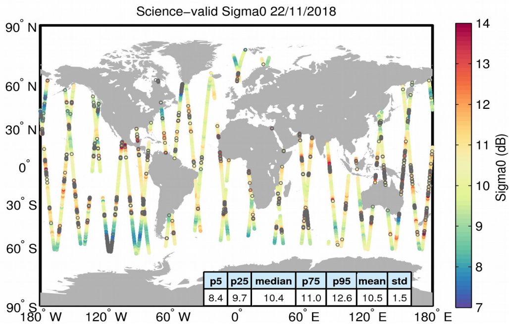
Figure 27. Geographical distribution of science-valid sigma0 data over oceans and lakes for 22/11/2018. The statistical values shown in the table refer to the sigma0 in dB and are calculated over all measurements shown in the figure. Gray circles denote records that have been rejected based on the editing criteria described in Table 4.
