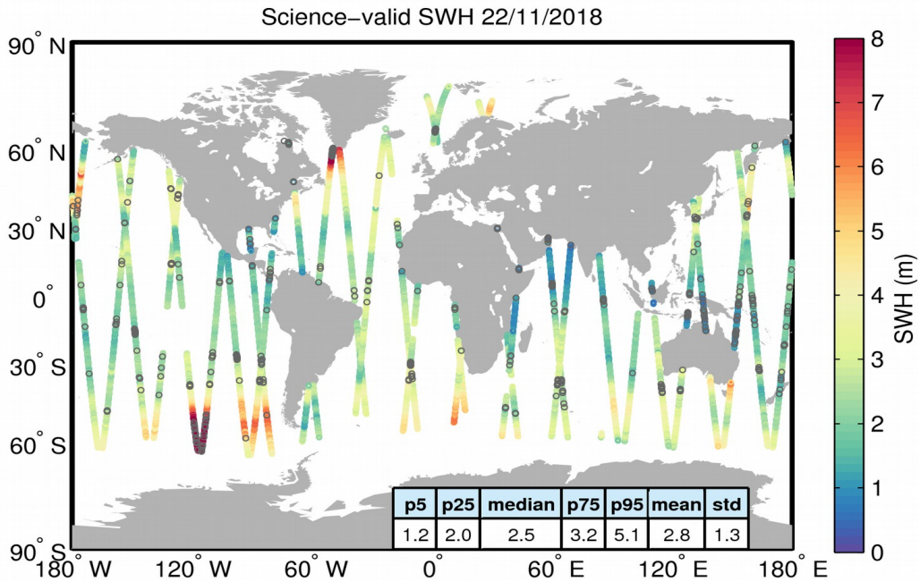
Figure 19. Geographical distribution of science-valid SWH data over oceans and lakes for 22/11/2018. The statistical values shown in the table refer to the SWH in m and are calculated over all measurements shown in the figure. Gray circles denote records that have been rejected based on the editing criteria described in Table 3.
