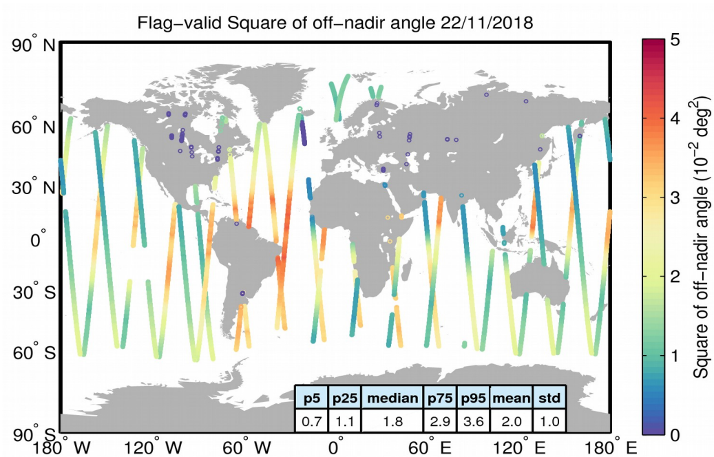
Figure 37. Geographical distribution of flag-valid mispointing data over oceans and lakes for 22/11/2018. The statistical values shown in the table refer to the mispointing in 10^{-2} deg 2 and are calculated over all measurements shown in the figure.
