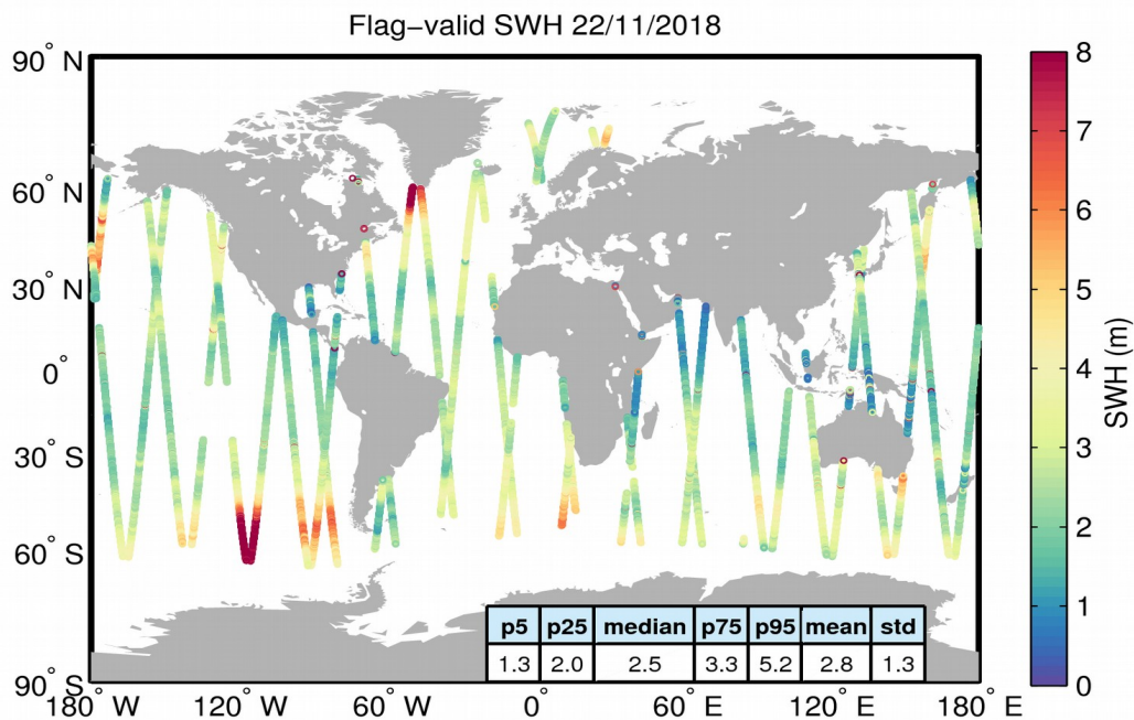
Figure 15. Geographical distribution of flag-valid SWH data over oceans and lakes for 22/11/2018. The statistical values shown in the table refer to the SWH in m and are calculated over all measurements shown in the figure.
