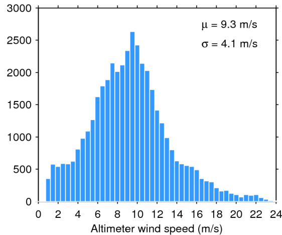
Figure 33. Histogram of flag-valid wind over oceans and lakes for 22/11/2018. The mean ( \mu ) and standard deviation ( \sigma ) are also shown. Note that values larger than 24 m/s are excluded from the histogram for the sake of readability but not from the computation of \mu and \sigma .
