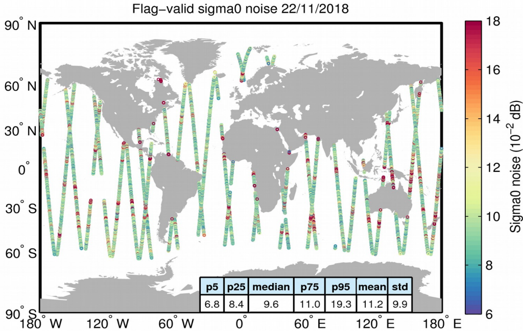
Figure 26. Geographical distribution of flag-valid 20-Hz sigma0 measurement noise over oceans and lakes for 22/11/2018. The statistical values shown in the table refer to the sigma0 noise and are calculated over all measurements shown in the figure.
