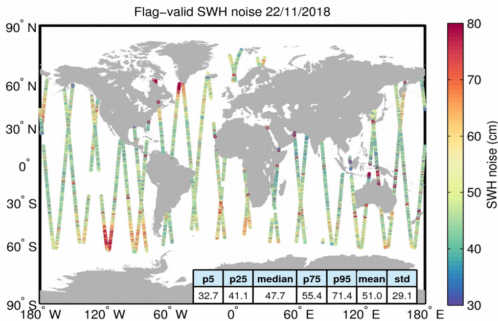
Figure 18. Geographical distribution of flag-valid 20-Hz SWH measurement noise over oceans and lakes for 22/11/2018. The statistical values shown in the figure refer to the SWH noise and are calculated over all measurements shown in the figure.
