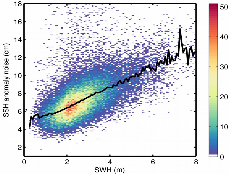
Figure 9. 2D histogram showing flag-valid SSH anomaly noise as a function of SWH for 22/11/2018. The black line denotes the median SSH anomaly noise as a function of SWH.
