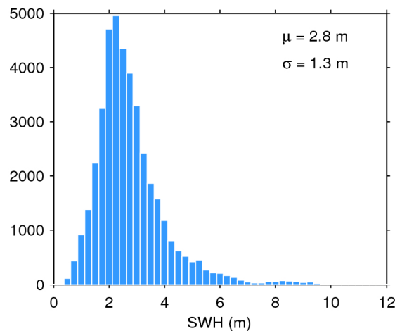
Figure 20. Histogram of science-valid SWH over oceans and lakes for 22/11/2018. The mean ( \mu ) and standard deviation ( \sigma ) are also shown. Note that values larger than 12 m are excluded from the histogram for the sake of readability but not from the computation of \mu and \sigma .
