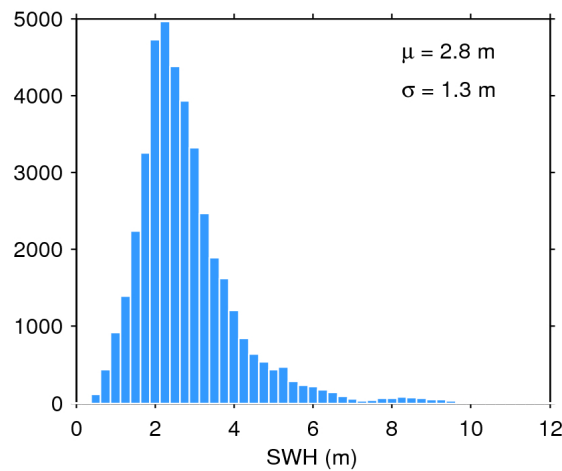
Figure 17. Histogram of flag-valid SWH over oceans and lakes for 22/11/2018. The mean ( \mu ) and standard deviation ( \sigma ) are also shown. Note that values larger than 12 m are excluded from the histogram for the sake of readability but not from the computation of \mu and \sigma .
