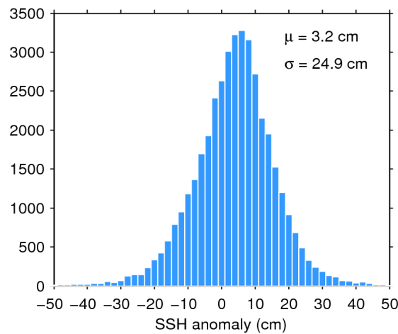
Figure 7. Histogram of flag-valid SSH anomaly over oceans and lakes for 22/11/2018. The mean ( \mu ) and standard deviation ( \sigma ) are also shown. Note that values outside [-50 50] cm are excluded from the histogram for the sake of readability but not from the computation of \mu and \sigma .
