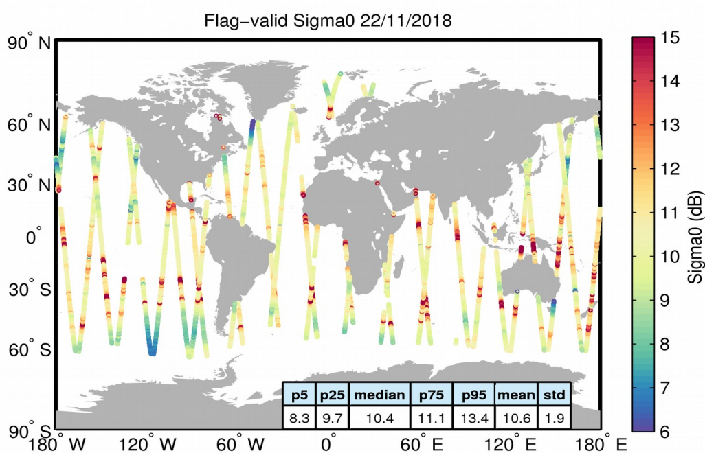
Figure 23. Geographical distribution of flag-valid sigma0 data over oceans and lakes for 22/11/2018. The statistical values shown in the table refer to the sigma0 in dB and are calculated over all measurements shown in the figure.
