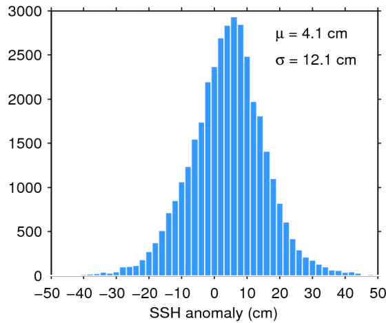
Figure 11. Histogram of science-valid SSH anomaly over oceans and lakes for 22/11/2018. The mean ( \mu ) and standard deviation ( \sigma ) are also shown. Note that values outside [-50 50] cm are excluded from the histogram for the sake of readability but not from the computation of \mu and \sigma .
