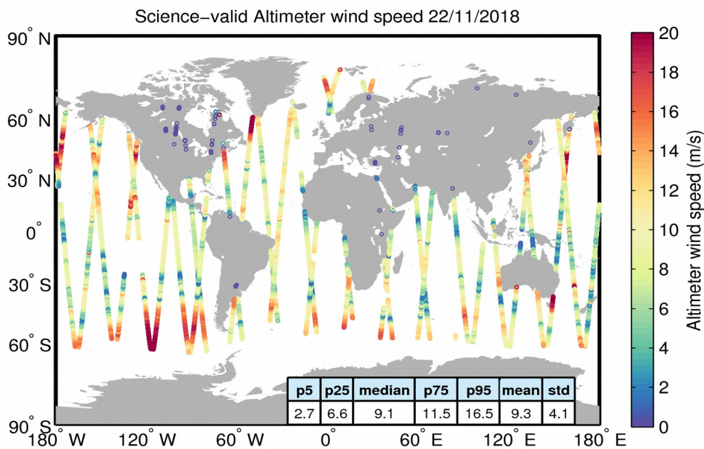
Figure 34. Geographical distribution of science-valid wind data over oceans and lakes for 22/11/2018. The statistical values shown in the table refer to the wind in m/s and are calculated over all measurements shown in the figure. Gray circles denote records that have been rejected based on the editing criteria described in Table 5.
