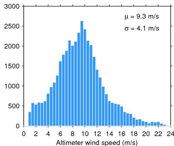
Figure 35. Histogram of science-valid wind over oceans and lakes for 22/11/2018. The mean ( \mu ) and standard deviation ( \sigma ) are also shown. Note that values larger than 24 m/s are excluded from the histogram for the sake of readability but not from the computation of \mu and \sigma .
