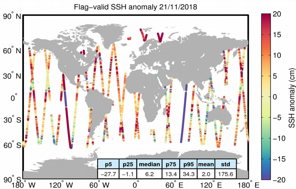
Figure 5. Geographical distribution of flag-valid 1-Hz SSH anomaly data over oceans and lakes for 21/11/2018. The statistical values shown in the table refer to the SSH anomaly in cm and are calculated over all measurements shown in the figure.
