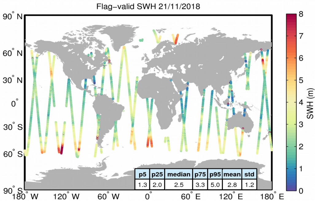
Figure 15. Geographical distribution of flag-valid SWH data over oceans and lakes for 21/11/2018. The statistical values shown in the table refer to the SWH in m and are calculated over all measurements shown in the figure.
