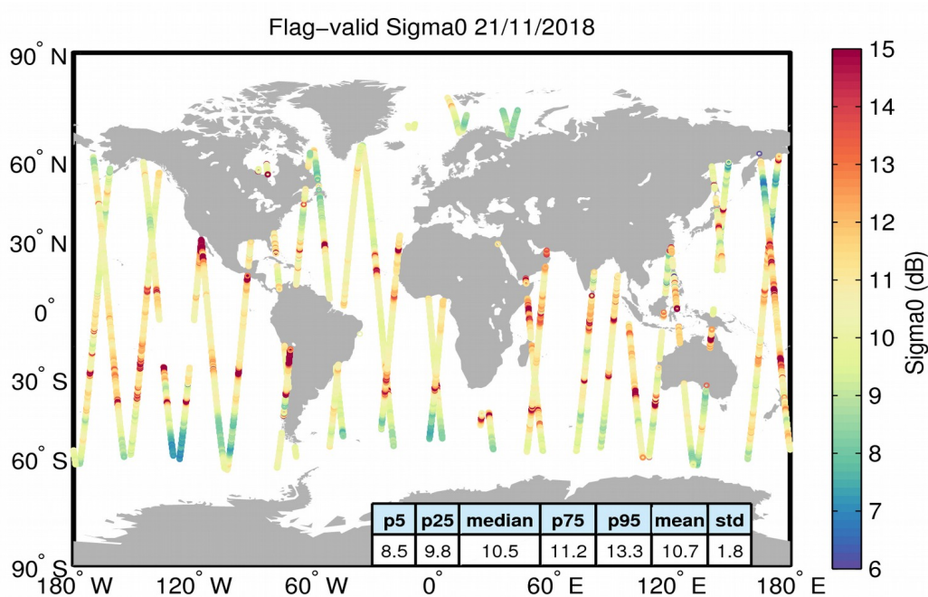
Figure 23. Geographical distribution of flag-valid sigma0 data over oceans and lakes for 21/11/2018. The statistical values shown in the table refer to the sigma0 in dB and are calculated over all measurements shown in the figure.
