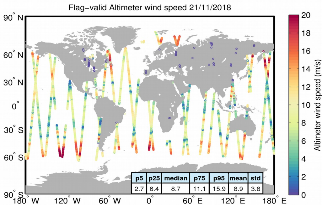
Figure 31. Geographical distribution of flag-valid wind data over oceans and lakes for 21/11/2018. The statistical values shown in the table refer to the wind in m/s and are calculated over all measurements shown in the figure.
