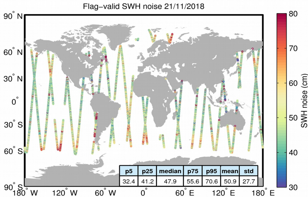
Figure 18. Geographical distribution of flag-valid 20-Hz SWH measurement noise over oceans and lakes for 21/11/2018. The statistical values shown in the figure refer to the SWH noise and are calculated over all measurements shown in the figure.
