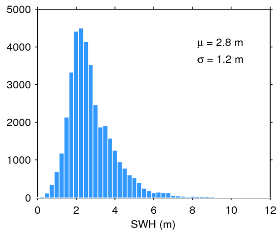
Figure 17. Histogram of flag-valid SWH over oceans and lakes for 21/11/2018. The mean ( \mu ) and standard deviation ( \sigma ) are also shown. Note that values larger than 12 m are excluded from the histogram for the sake of readability but not from the computation of \mu and \sigma .
