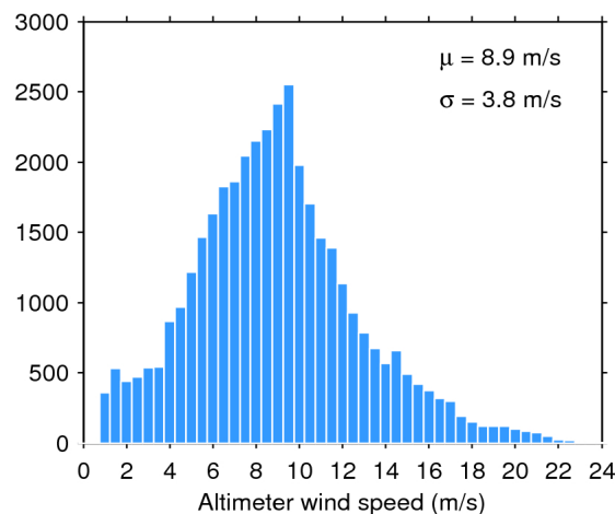
Figure 35. Histogram of science-valid wind over oceans and lakes for 21/11/2018. The mean ( \mu ) and standard deviation ( \sigma ) are also shown. Note that values larger than 24 m/s are excluded from the histogram for the sake of readability but not from the computation of \mu and \sigma .
