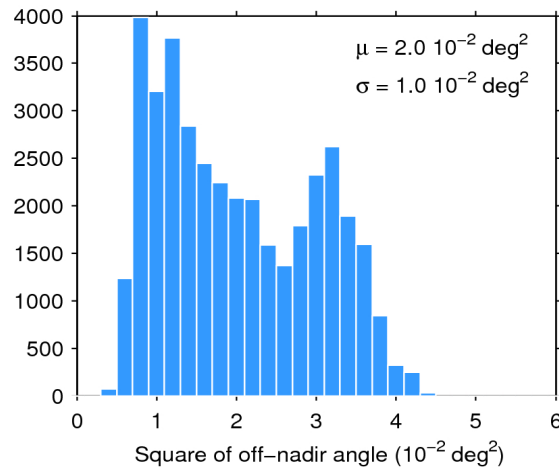
Figure 39. Histogram of flag-valid mispointing over oceans and lakes for 21/11/2018. The mean ( \mu ) and standard deviation ( \sigma ) are also shown. Note that values larger than 6 \cdot 10^{-2} \text{ deg}^2 are excluded from the histogram for the sake of readability but not from the computation of \mu and \sigma .
