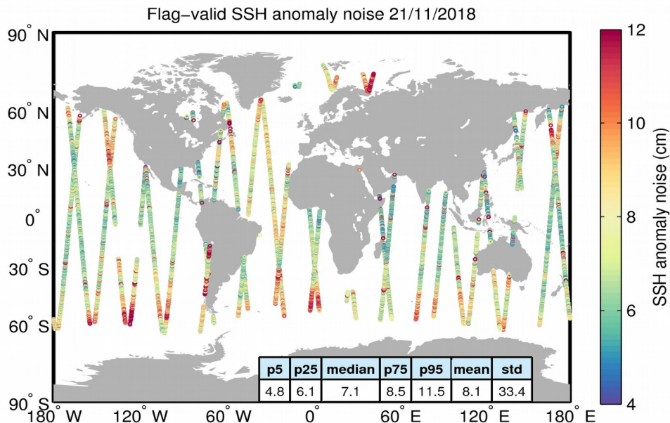
Figure 8. Geographical distribution of flag-valid 20-Hz SSH anomaly measurement noise over oceans and lakes for 21/11/2018. The statistical values shown in the table refer to the SSH anomaly noise and are calculated over all measurements shown in the figure.
