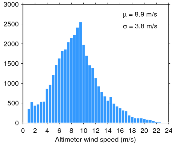
Figure 33. Histogram of flag-valid wind over oceans and lakes for 21/11/2018. The mean ( \mu ) and standard deviation ( \sigma ) are also shown. Note that values larger than 24 m/s are excluded from the histogram for the sake of readability but not from the computation of \mu and \sigma .
