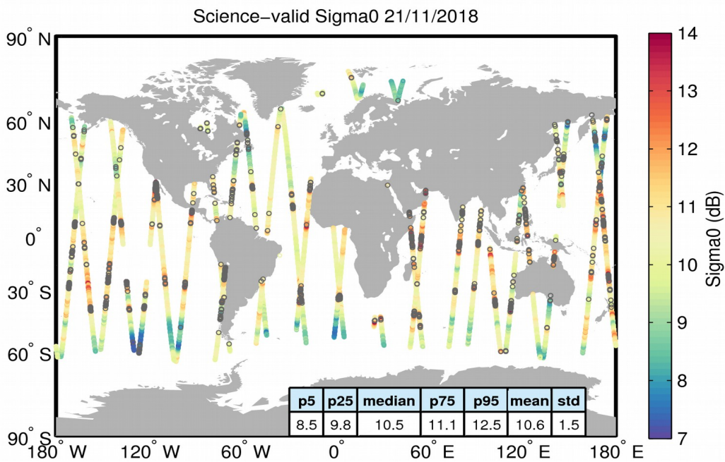
Figure 27. Geographical distribution of science-valid sigma0 data over oceans and lakes for 21/11/2018. The statistical values shown in the table refer to the sigma0 in dB and are calculated over all measurements shown in the figure. Gray circles denote records that have been rejected based on the editing criteria described in Table 4.
