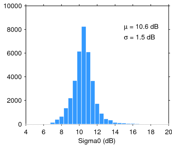
Figure 28. Histogram of science-valid sigma0 over oceans and lakes for 21/11/2018. The mean ( \mu ) and standard deviation ( \sigma ) are also shown. Note that values outside [4 20] dB are excluded from the histogram for the sake of readability but not from the computation of \mu and \sigma .
