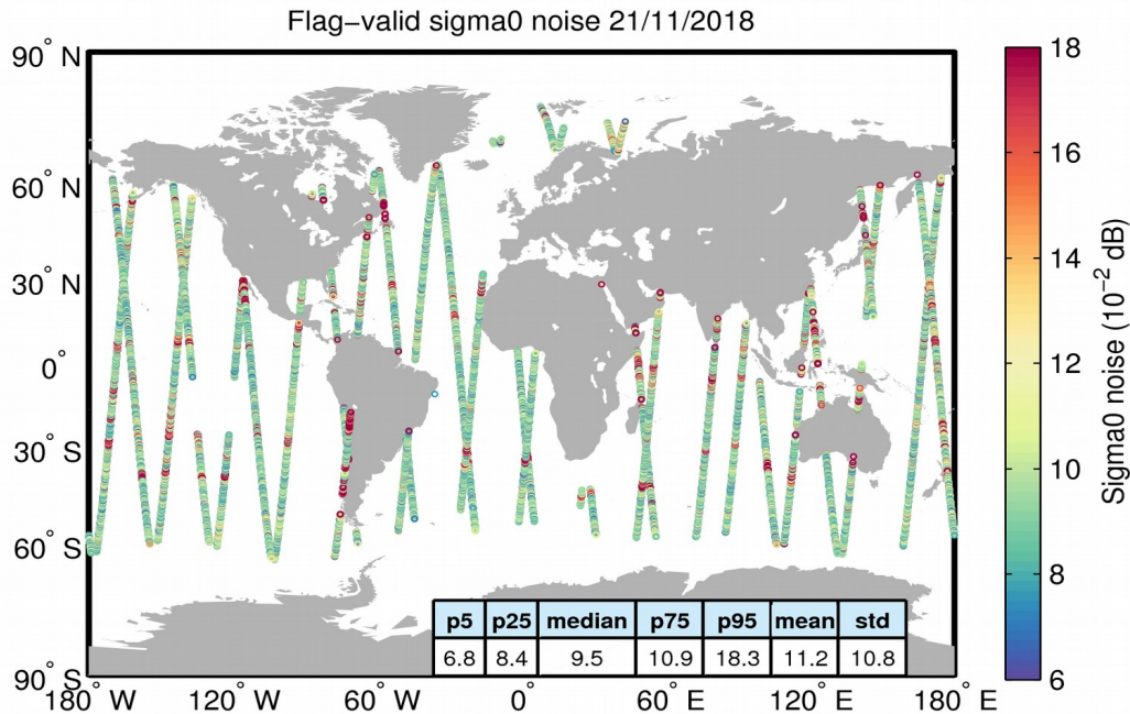
Figure 26. Geographical distribution of flag-valid 20-Hz sigma0 measurement noise over oceans and lakes for 21/11/2018. The statistical values shown in the table refer to the sigma0 noise and are calculated over all measurements shown in the figure.
