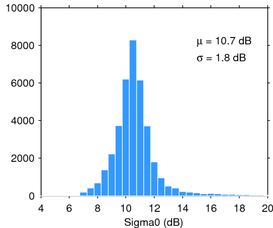
Figure 25. Histogram of flag-valid sigma0 over oceans and lakes for 21/11/2018. The mean ( \mu ) and standard deviation ( \sigma ) are also shown. Note that values outside [4 20] dB are excluded from the histogram for the sake of readability but not from the computation of \mu and \sigma .
