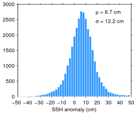
Figure 11. Histogram of science-valid SSH anomaly over oceans and lakes for 21/11/2018. The mean ( \mu ) and standard deviation ( \sigma ) are also shown. Note that values outside [-50 50] cm are excluded from the histogram for the sake of readability but not from the computation of \mu and \sigma .
