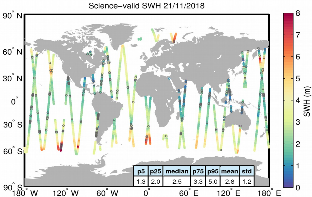
Figure 19. Geographical distribution of science-valid SWH data over oceans and lakes for 21/11/2018. The statistical values shown in the table refer to the SWH in m and are calculated over all measurements shown in the figure. Gray circles denote records that have been rejected based on the editing criteria described in Table 3.
