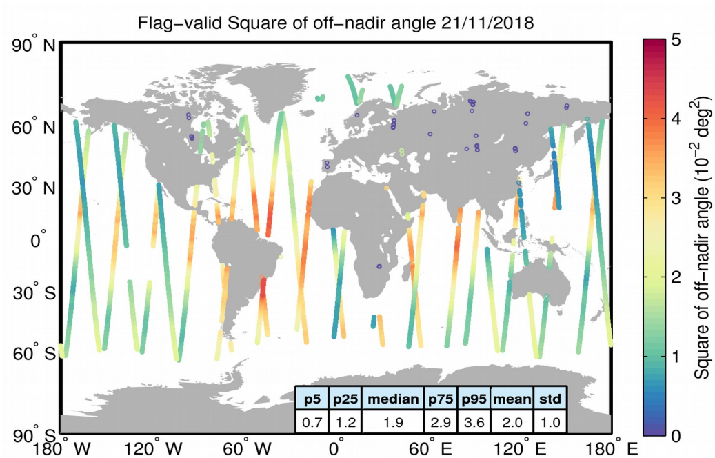
Figure 37. Geographical distribution of flag-valid mispointing data over oceans and lakes for 21/11/2018. The statistical values shown in the table refer to the mispointing in 10^{-2} \text{ deg}^2 and are calculated over all measurements shown in the figure.
