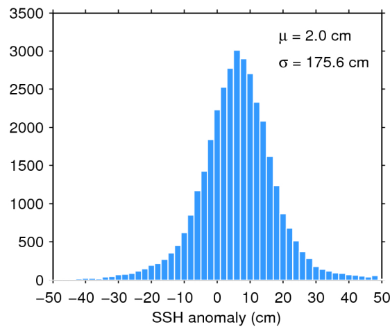
Figure 7. Histogram of flag-valid SSH anomaly over oceans and lakes for 21/11/2018. The mean ( \mu ) and standard deviation ( \sigma ) are also shown. Note that values outside [-50\ 50] cm are excluded from the histogram for the sake of readability but not from the computation of \mu and \sigma .
