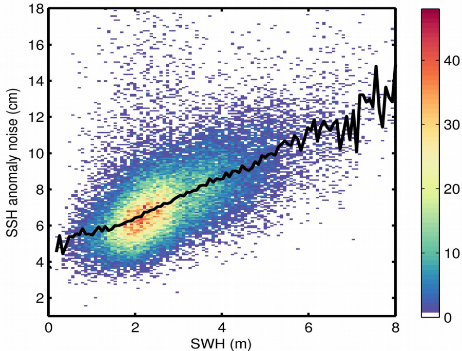
Figure 9. 2D histogram showing flag-valid SSH anomaly noise as a function of SWH for 21/11/2018. The black line denotes the median SSH anomaly noise as a function of SWH.
