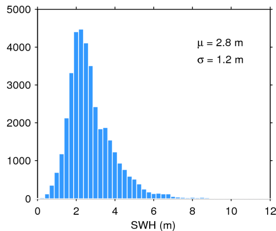
Figure 20. Histogram of science-valid SWH over oceans and lakes for 21/11/2018. The mean ( \mu ) and standard deviation ( \sigma ) are also shown. Note that values larger than 12 m are excluded from the histogram for the sake of readability but not from the computation of \mu and \sigma .
