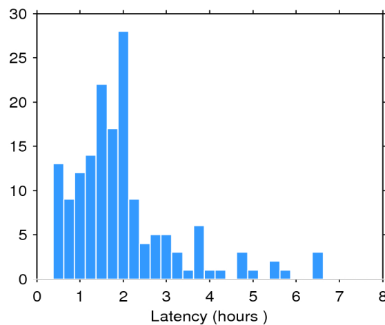
Figure 2. Histogram of the data latency for 21/11/2018. The y-axis denotes the number of files that are made available with a delay of x-hours with respect to the mean time of the records stored in the file.
