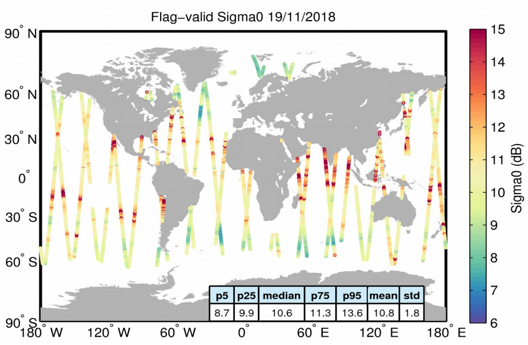
Figure 23. Geographical distribution of flag-valid sigma0 data over oceans and lakes for 19/11/2018. The statistical values shown in the table refer to the sigma0 in dB and are calculated over all measurements shown in the figure.
