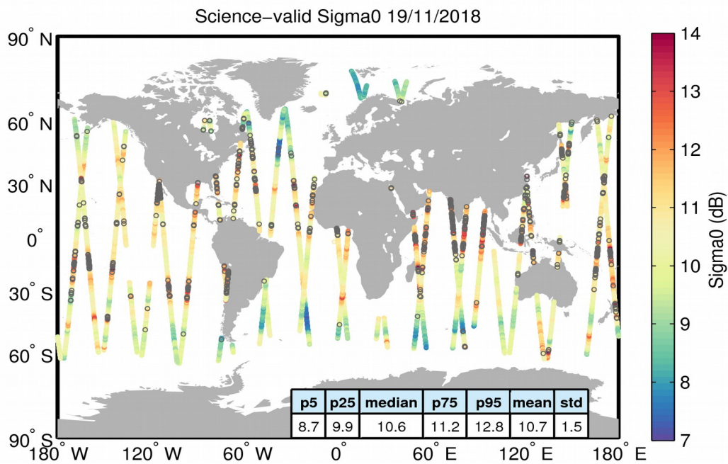
Figure 27. Geographical distribution of science-valid sigma0 data over oceans and lakes for 19/11/2018. The statistical values shown in the table refer to the sigma0 in dB and are calculated over all measurements shown in the figure. Gray circles denote records that have been rejected based on the editing criteria described in Table 4.
