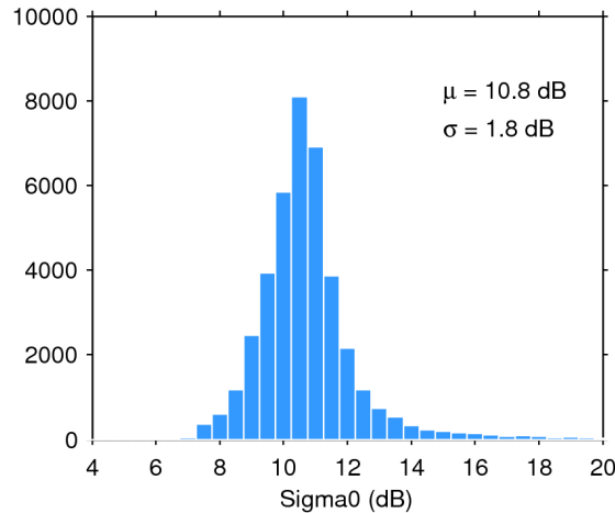
Figure 25. Histogram of flag-valid sigma0 over oceans and lakes for 19/11/2018. The mean ( \mu ) and standard deviation ( \sigma ) are also shown. Note that values outside [4 20] dB are excluded from the histogram for the sake of readability but not from the computation of \mu and \sigma .
