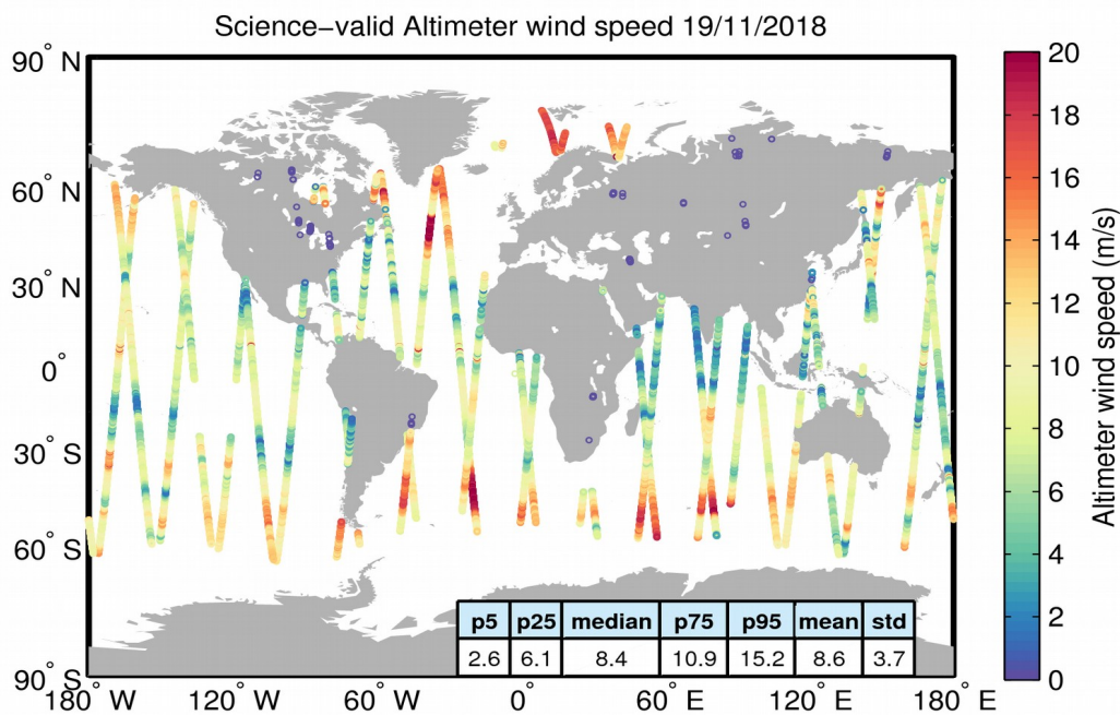
Figure 34. Geographical distribution of science-valid wind data over oceans and lakes for 19/11/2018. The statistical values shown in the table refer to the wind in m/s and are calculated over all measurements shown in the figure. Gray circles denote records that have been rejected based on the editing criteria described in Table 5.
