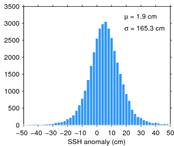
Figure 7. Histogram of flag-valid SSH anomaly over oceans and lakes for 19/11/2018. The mean ( \mu ) and standard deviation ( \sigma ) are also shown. Note that values outside [-50 50] cm are excluded from the histogram for the sake of readability but not from the computation of \mu and \sigma .
