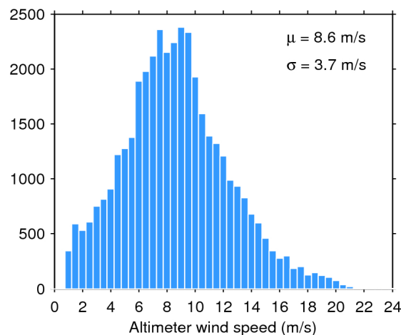
Figure 35. Histogram of science-valid wind over oceans and lakes for 19/11/2018. The mean ( \mu ) and standard deviation ( \sigma ) are also shown. Note that values larger than 24 m/s are excluded from the histogram for the sake of readability but not from the computation of \mu and \sigma .
