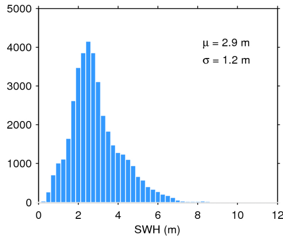
Figure 20. Histogram of science-valid SWH over oceans and lakes for 19/11/2018. The mean ( \mu ) and standard deviation ( \sigma ) are also shown. Note that values larger than 12 m are excluded from the histogram for the sake of readability but not from the computation of \mu and \sigma .
