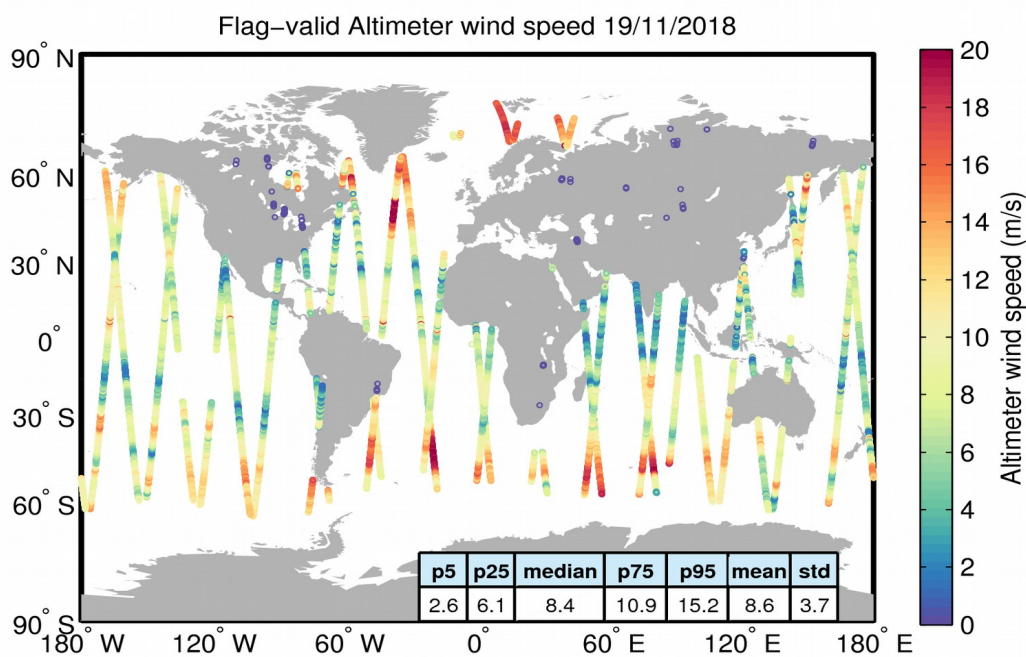
Figure 31. Geographical distribution of flag-valid wind data over oceans and lakes for 19/11/2018. The statistical values shown in the table refer to the wind in m/s and are calculated over all measurements shown in the figure.
