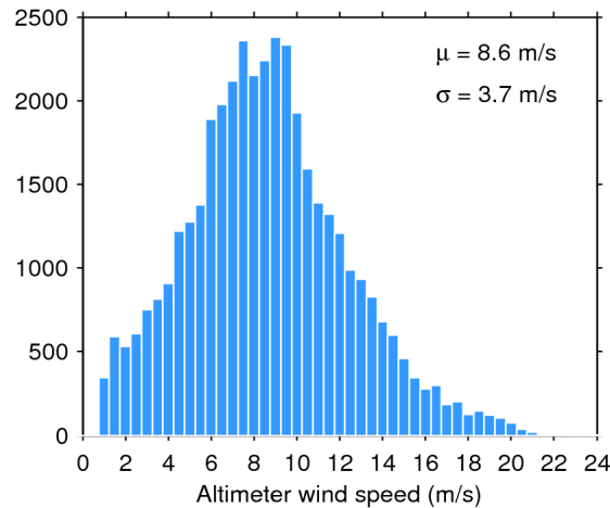
Figure 33. Histogram of flag-valid wind over oceans and lakes for 19/11/2018. The mean ( \mu ) and standard deviation ( \sigma ) are also shown. Note that values larger than 24 m/s are excluded from the histogram for the sake of readability but not from the computation of \mu and \sigma .
