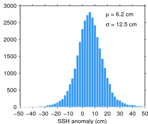
Figure 11. Histogram of science-valid SSH anomaly over oceans and lakes for 19/11/2018. The mean ( \mu ) and standard deviation ( \sigma ) are also shown. Note that values outside [-50 50] cm are excluded from the histogram for the sake of readability but not from the computation of \mu and \sigma .
