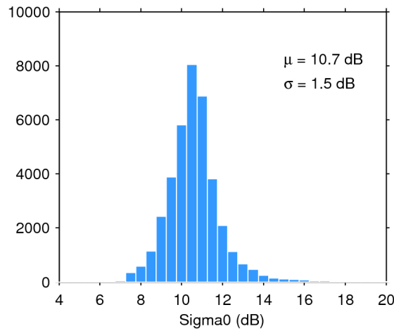
Figure 28. Histogram of science-valid sigma0 over oceans and lakes for 19/11/2018. The mean ( \mu ) and standard deviation ( \sigma ) are also shown. Note that values outside [4 20] dB are excluded from the histogram for the sake of readability but not from the computation of \mu and \sigma .
