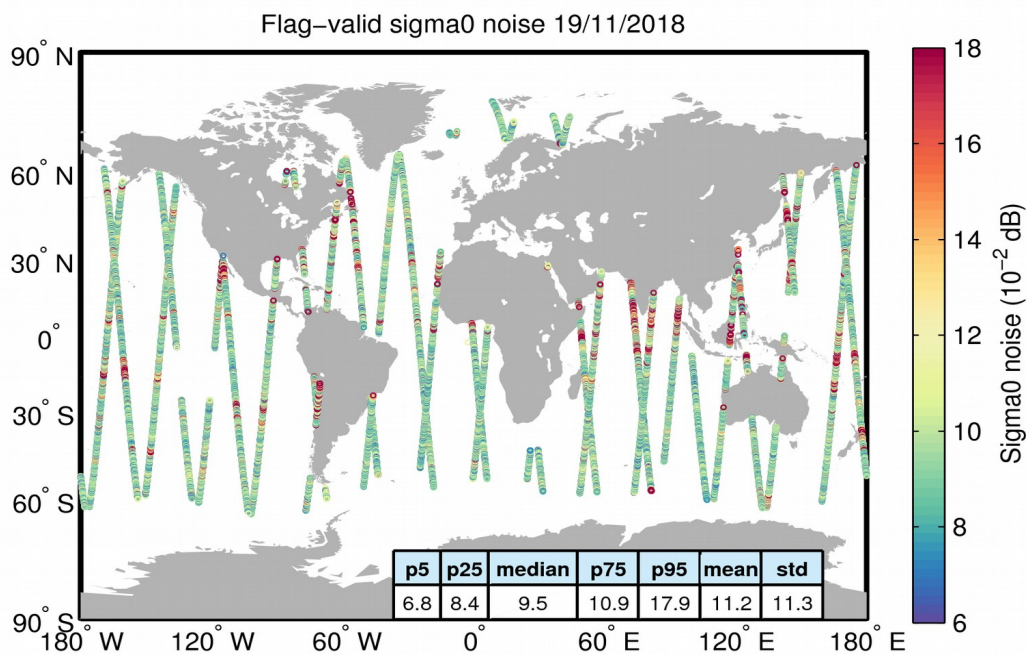
Figure 26. Geographical distribution of flag-valid 20-Hz sigma0 measurement noise over oceans and lakes for 19/11/2018. The statistical values shown in the table refer to the sigma0 noise and are calculated over all measurements shown in the figure.
