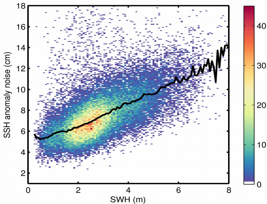
Figure 9. 2D histogram showing flag-valid SSH anomaly noise as a function of SWH for 19/11/2018. The black line denotes the median SSH anomaly noise as a function of SWH.
