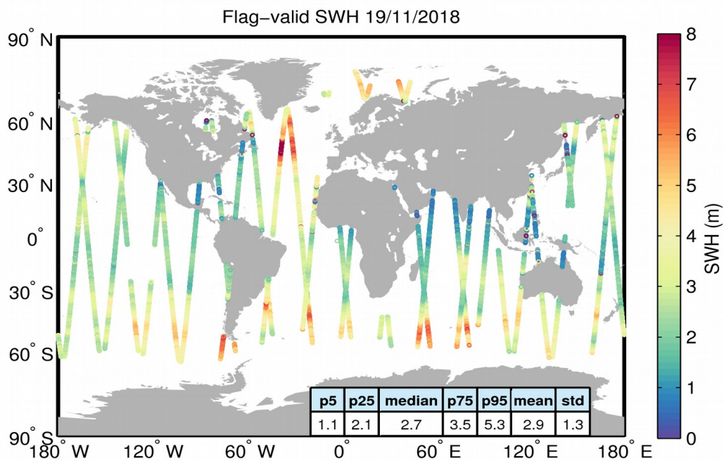
Figure 15. Geographical distribution of flag-valid SWH data over oceans and lakes for 19/11/2018. The statistical values shown in the table refer to the SWH in m and are calculated over all measurements shown in the figure.
