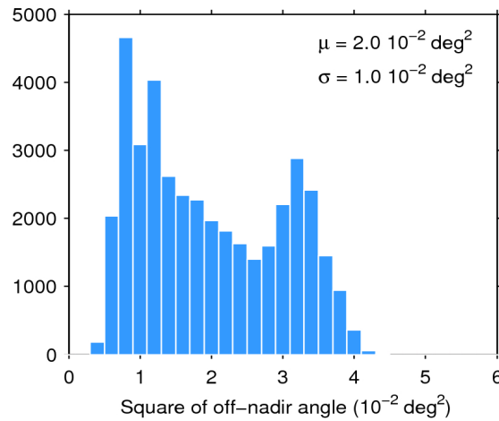
Figure 39. Histogram of flag-valid mispointing over oceans and lakes for 19/11/2018. The mean ( \mu ) and standard deviation ( \sigma ) are also shown. Note that values larger than 6 \cdot 10^{-2} \text{ deg}^2 are excluded from the histogram for the sake of readability but not from the computation of \mu and \sigma .
