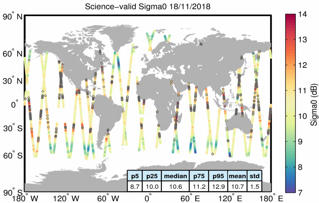
Figure 27. Geographical distribution of science-valid sigma0 data over oceans and lakes for 18/11/2018. The statistical values shown in the table refer to the sigma0 in dB and are calculated over all measurements shown in the figure. Gray circles denote records that have been rejected based on the editing criteria described in Table 4.
