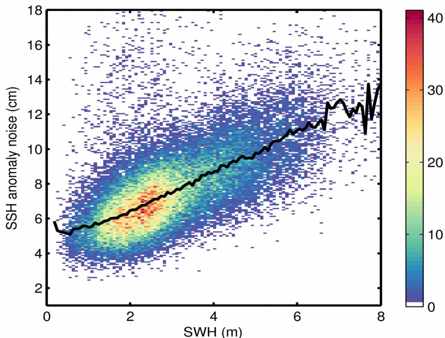
Figure 9. 2D histogram showing flag-valid SSH anomaly noise as a function of SWH for 18/11/2018. The black line denotes the median SSH anomaly noise as a function of SWH.
