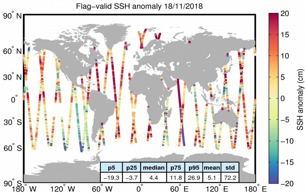
Figure 5. Geographical distribution of flag-valid 1-Hz SSH anomaly data over oceans and lakes for 18/11/2018. The statistical values shown in the table refer to the SSH anomaly in cm and are calculated over all measurements shown in the figure.
