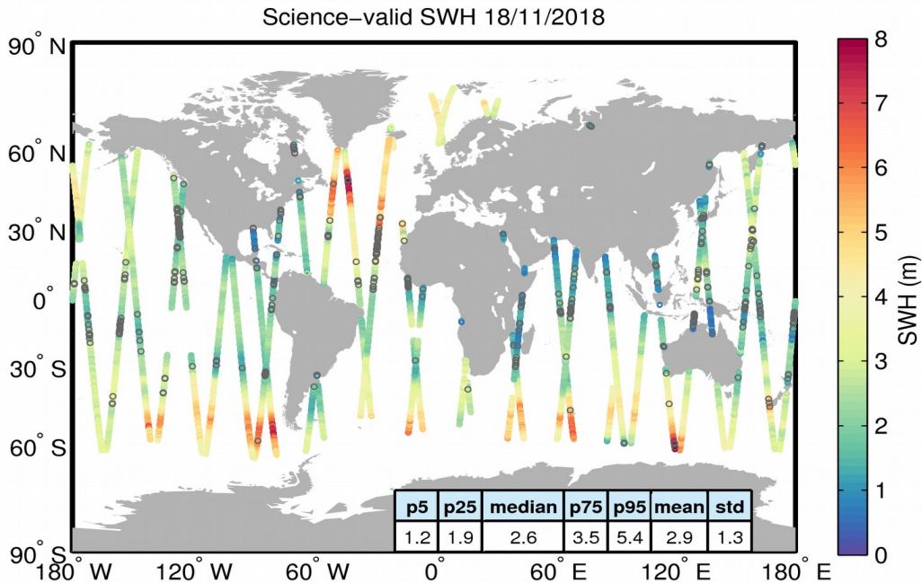
Figure 19. Geographical distribution of science-valid SWH data over oceans and lakes for 18/11/2018. The statistical values shown in the table refer to the SWH in m and are calculated over all measurements shown in the figure. Gray circles denote records that have been rejected based on the editing criteria described in Table 3.
