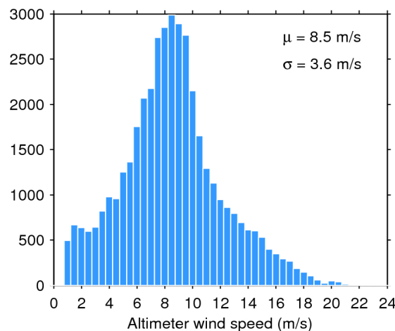
Figure 35. Histogram of science-valid wind over oceans and lakes for 18/11/2018. The mean ( \mu ) and standard deviation ( \sigma ) are also shown. Note that values larger than 24 m/s are excluded from the histogram for the sake of readability but not from the computation of \mu and \sigma .
