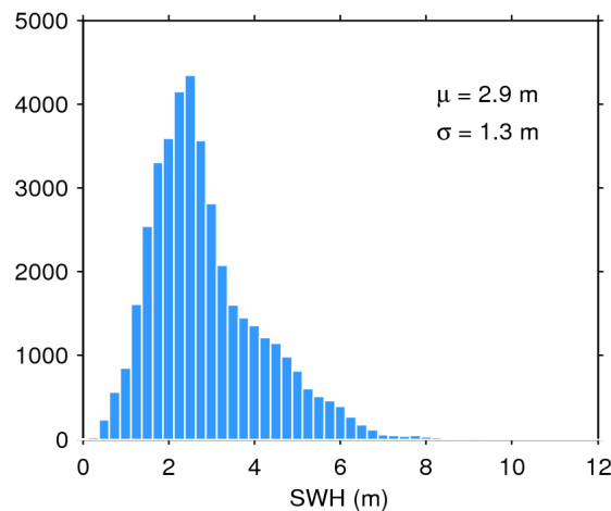
Figure 20. Histogram of science-valid SWH over oceans and lakes for 18/11/2018. The mean ( \mu ) and standard deviation ( \sigma ) are also shown. Note that values larger than 12 m are excluded from the histogram for the sake of readability but not from the computation of \mu and \sigma .
