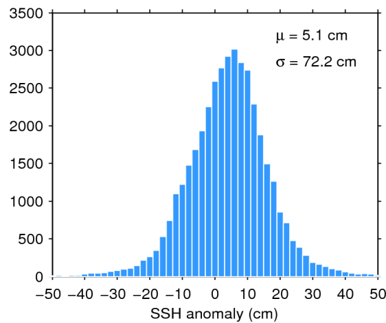
Figure 7. Histogram of flag-valid SSH anomaly over oceans and lakes for 18/11/2018. The mean ( \mu ) and standard deviation ( \sigma ) are also shown. Note that values outside [-50\ 50] cm are excluded from the histogram for the sake of readability but not from the computation of \mu and \sigma .
