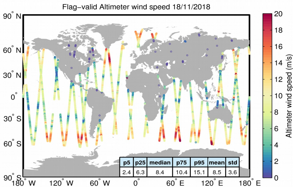
Figure 31. Geographical distribution of flag-valid wind data over oceans and lakes for 18/11/2018. The statistical values shown in the table refer to the wind in m/s and are calculated over all measurements shown in the figure.
