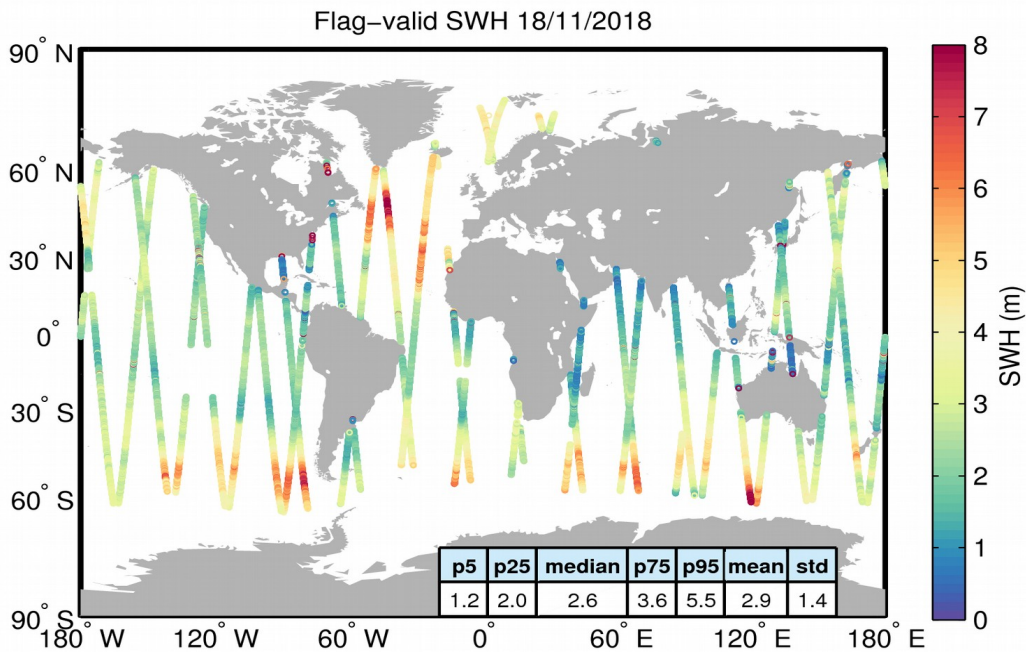
Figure 15. Geographical distribution of flag-valid SWH data over oceans and lakes for 18/11/2018. The statistical values shown in the table refer to the SWH in m and are calculated over all measurements shown in the figure.
