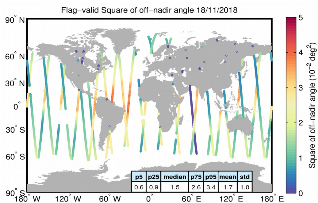
Figure 37. Geographical distribution of flag-valid mispointing data over oceans and lakes for 18/11/2018. The statistical values shown in the table refer to the mispointing in 10^{-2} deg 2 and are calculated over all measurements shown in the figure.
