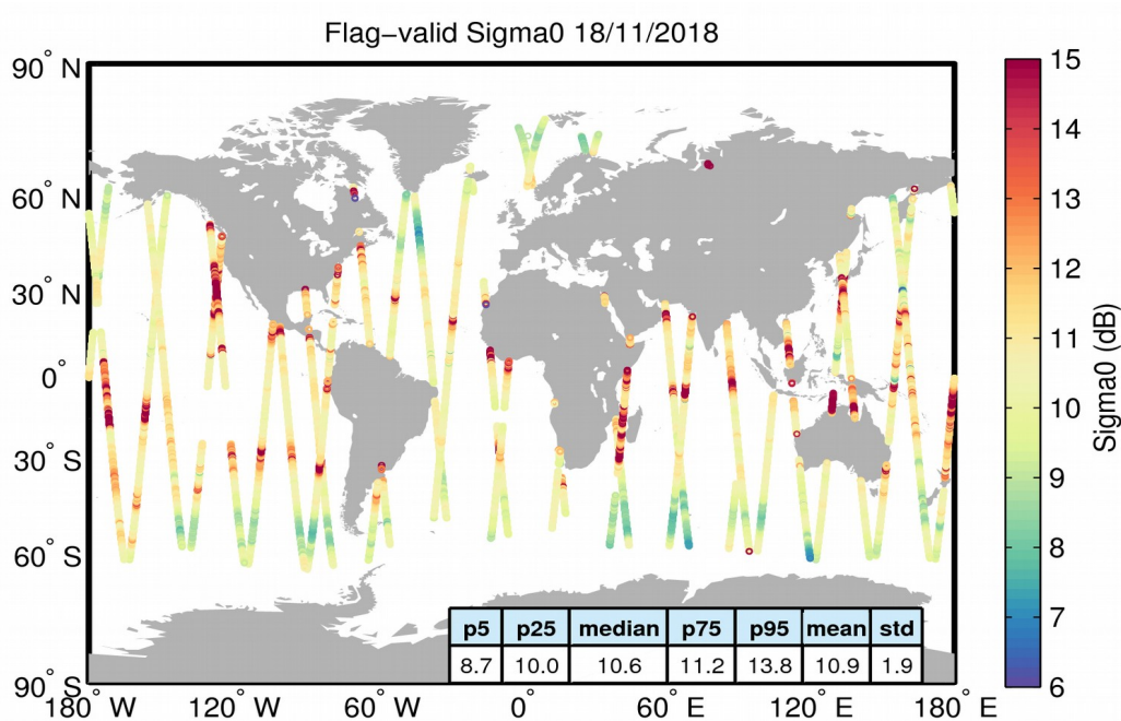
Figure 23. Geographical distribution of flag-valid sigma0 data over oceans and lakes for 18/11/2018. The statistical values shown in the table refer to the sigma0 in dB and are calculated over all measurements shown in the figure.
