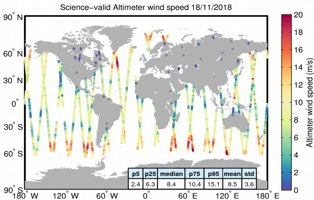
Figure 34. Geographical distribution of science-valid wind data over oceans and lakes for 18/11/2018. The statistical values shown in the table refer to the wind in m/s and are calculated over all measurements shown in the figure. Gray circles denote records that have been rejected based on the editing criteria described in Table 5.
