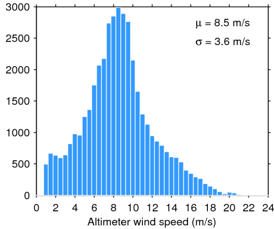
Figure 33. Histogram of flag-valid wind over oceans and lakes for 18/11/2018. The mean ( \mu ) and standard deviation ( \sigma ) are also shown. Note that values larger than 24 m/s are excluded from the histogram for the sake of readability but not from the computation of \mu and \sigma .
