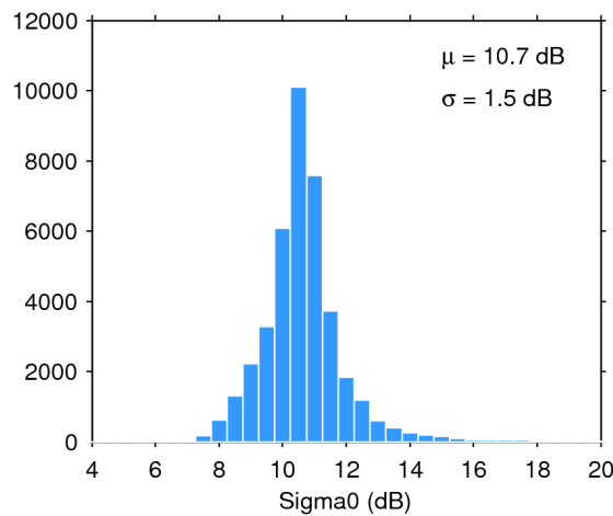
Figure 28. Histogram of science-valid sigma0 over oceans and lakes for 18/11/2018. The mean ( \mu ) and standard deviation ( \sigma ) are also shown. Note that values outside [4 20] dB are excluded from the histogram for the sake of readability but not from the computation of \mu and \sigma .
