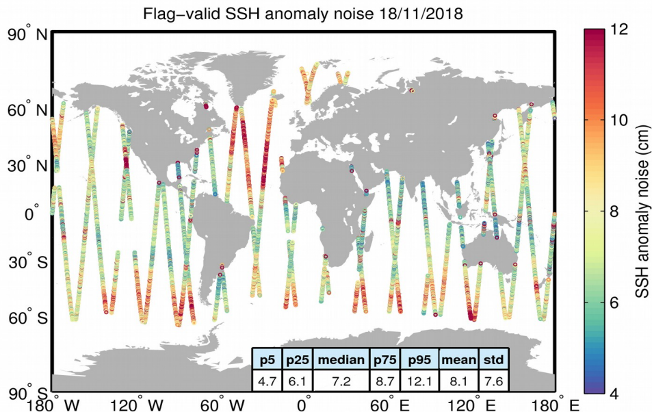
Figure 8. Geographical distribution of flag-valid 20-Hz SSH anomaly measurement noise over oceans and lakes for 18/11/2018. The statistical values shown in the table refer to the SSH anomaly noise and are calculated over all measurements shown in the figure.
