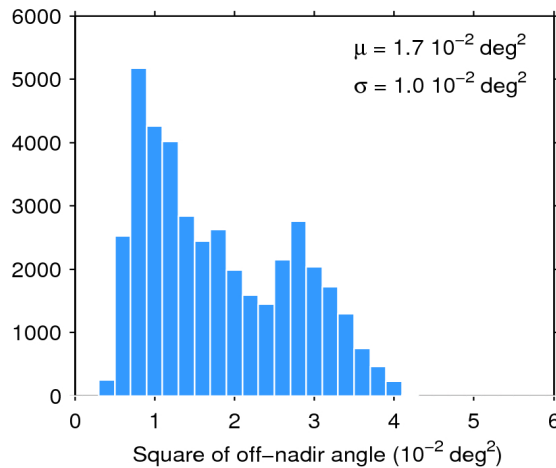
Figure 39. Histogram of flag-valid mispointing over oceans and lakes for 18/11/2018. The mean ( \mu ) and standard deviation ( \sigma ) are also shown. Note that values larger than 6 \cdot 10^{-2} \text{ deg}^2 are excluded from the histogram for the sake of readability but not from the computation of \mu and \sigma .
