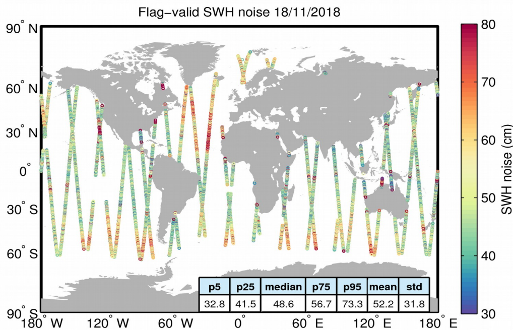
Figure 18. Geographical distribution of flag-valid 20-Hz SWH measurement noise over oceans and lakes for 18/11/2018. The statistical values shown in the figure refer to the SWH noise and are calculated over all measurements shown in the figure.
