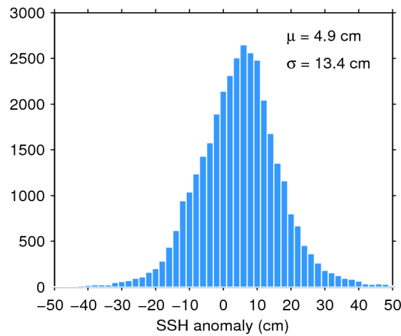
Figure 11. Histogram of science-valid SSH anomaly over oceans and lakes for 18/11/2018. The mean ( \mu ) and standard deviation ( \sigma ) are also shown. Note that values outside [-50 50] cm are excluded from the histogram for the sake of readability but not from the computation of \mu and \sigma .
