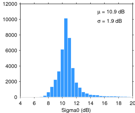
Figure 25. Histogram of flag-valid sigma0 over oceans and lakes for 18/11/2018. The mean ( \mu ) and standard deviation ( \sigma ) are also shown. Note that values outside [4 20] dB are excluded from the histogram for the sake of readability but not from the computation of \mu and \sigma .
