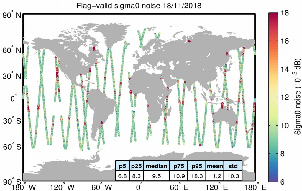
Figure 26. Geographical distribution of flag-valid 20-Hz sigma0 measurement noise over oceans and lakes for 18/11/2018. The statistical values shown in the table refer to the sigma0 noise and are calculated over all measurements shown in the figure.
