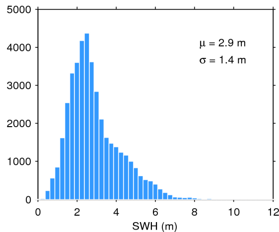
Figure 17. Histogram of flag-valid SWH over oceans and lakes for 18/11/2018. The mean ( \mu ) and standard deviation ( \sigma ) are also shown. Note that values larger than 12 m are excluded from the histogram for the sake of readability but not from the computation of \mu and \sigma .
