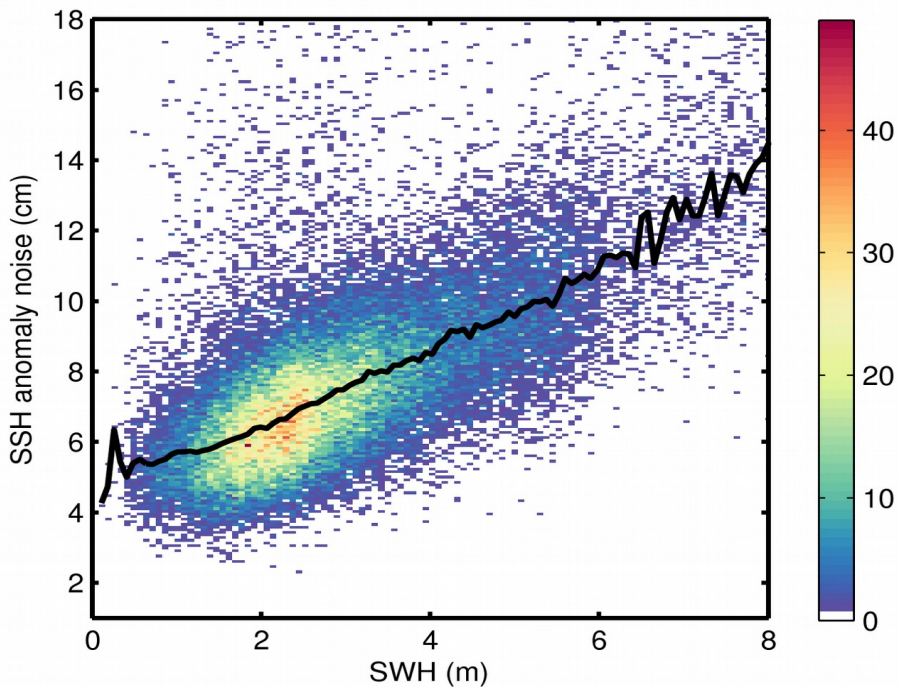
Figure 9. 2D histogram showing flag-valid SSH anomaly noise as a function of SWH for 17/11/2018. The black line denotes the median SSH anomaly noise as a function of SWH.
