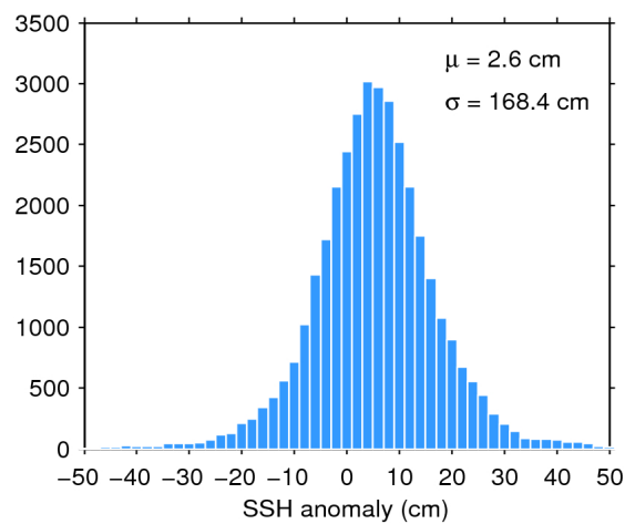
Figure 7. Histogram of flag-valid SSH anomaly over oceans and lakes for 17/11/2018. The mean ( \mu ) and standard deviation ( \sigma ) are also shown. Note that values outside [-50\ 50] cm are excluded from the histogram for the sake of readability but not from the computation of \mu and \sigma .
