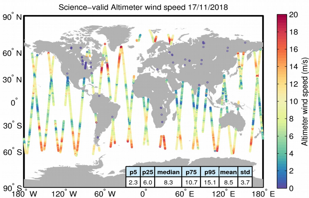
Figure 34. Geographical distribution of science-valid wind data over oceans and lakes for 17/11/2018. The statistical values shown in the table refer to the wind in m/s and are calculated over all measurements shown in the figure. Gray circles denote records that have been rejected based on the editing criteria described in Table 5.
