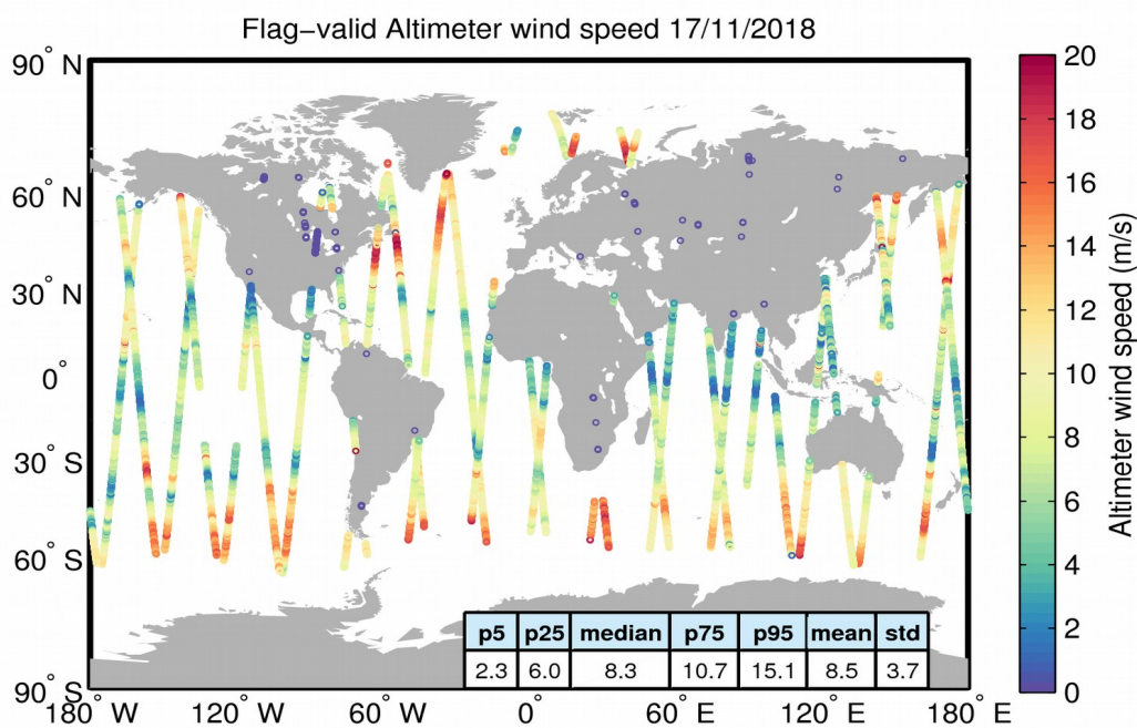
Figure 31. Geographical distribution of flag-valid wind data over oceans and lakes for 17/11/2018. The statistical values shown in the table refer to the wind in m/s and are calculated over all measurements shown in the figure.
