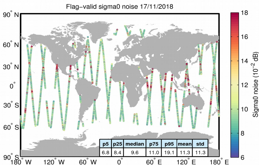
Figure 26. Geographical distribution of flag-valid 20-Hz sigma0 measurement noise over oceans and lakes for 17/11/2018. The statistical values shown in the table refer to the sigma0 noise and are calculated over all measurements shown in the figure.
