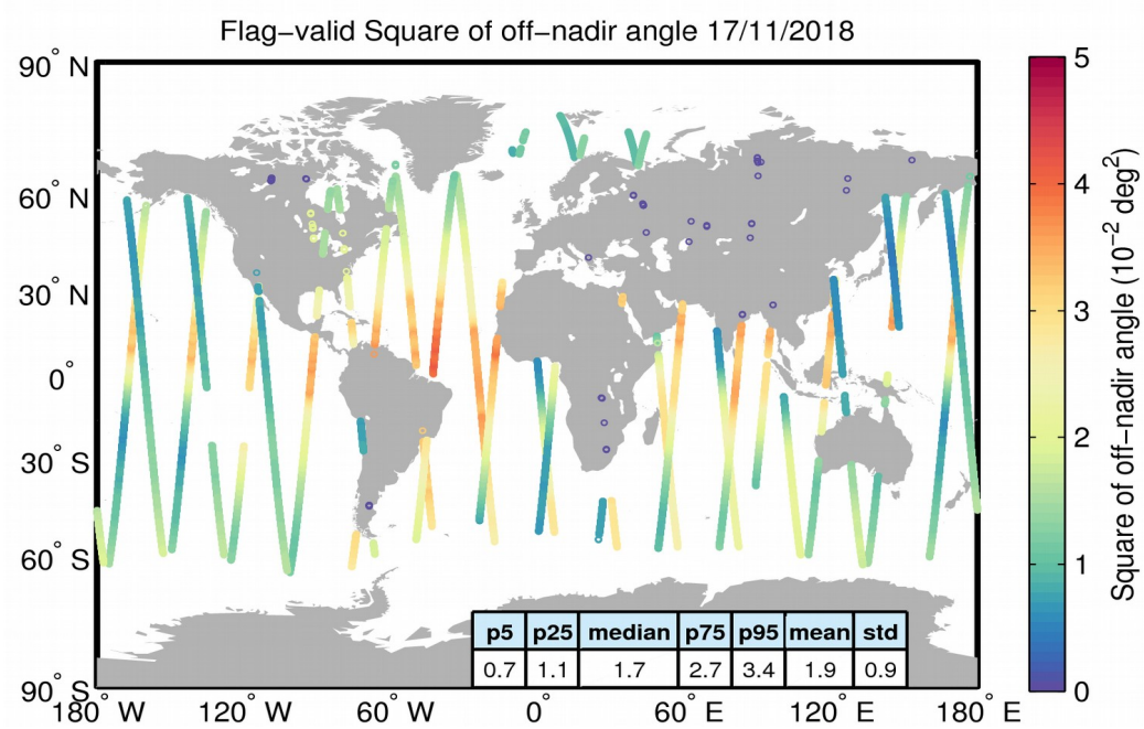
Figure 37. Geographical distribution of flag-valid mispointing data over oceans and lakes for 17/11/2018. The statistical values shown in the table refer to the mispointing in 10^{-2} deg 2 and are calculated over all measurements shown in the figure.
