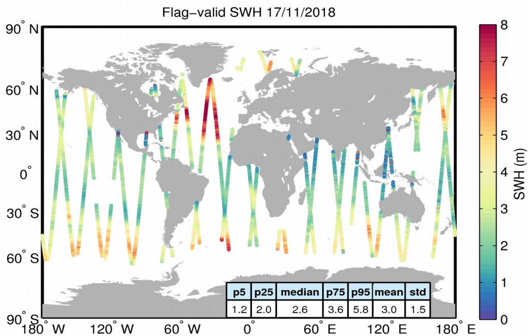
Figure 15. Geographical distribution of flag-valid SWH data over oceans and lakes for 17/11/2018. The statistical values shown in the table refer to the SWH in m and are calculated over all measurements shown in the figure.
