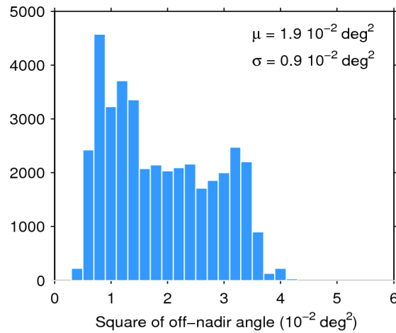
Figure 39. Histogram of flag-valid mispointing over oceans and lakes for 17/11/2018. The mean ( \mu ) and standard deviation ( \sigma ) are also shown. Note that values larger than 6 \cdot 10^{-2} \text{ deg}^2 are excluded from the histogram for the sake of readability but not from the computation of \mu and \sigma .
