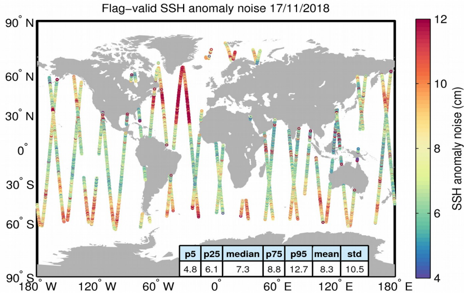
Figure 8. Geographical distribution of flag-valid 20-Hz SSH anomaly measurement noise over oceans and lakes for 17/11/2018. The statistical values shown in the table refer to the SSH anomaly noise and are calculated over all measurements shown in the figure.
