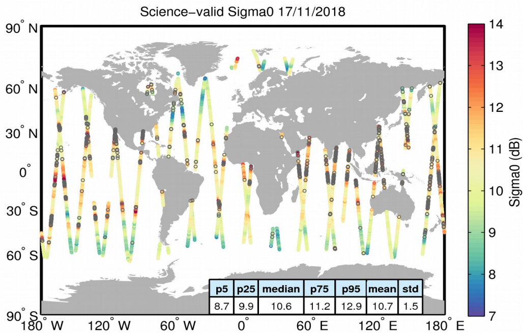
Figure 27. Geographical distribution of science-valid sigma0 data over oceans and lakes for 17/11/2018. The statistical values shown in the table refer to the sigma0 in dB and are calculated over all measurements shown in the figure. Gray circles denote records that have been rejected based on the editing criteria described in Table 4.
