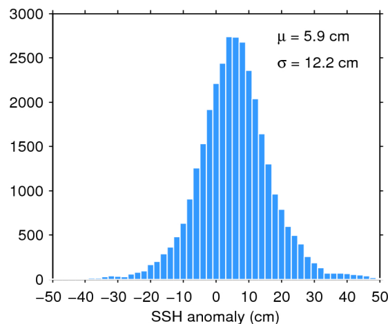
Figure 11. Histogram of science-valid SSH anomaly over oceans and lakes for 17/11/2018. The mean ( \mu ) and standard deviation ( \sigma ) are also shown. Note that values outside [-50 50] cm are excluded from the histogram for the sake of readability but not from the computation of \mu and \sigma .
