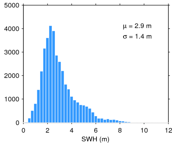
Figure 20. Histogram of science-valid SWH over oceans and lakes for 17/11/2018. The mean ( \mu ) and standard deviation ( \sigma ) are also shown. Note that values larger than 12 m are excluded from the histogram for the sake of readability but not from the computation of \mu and \sigma .
