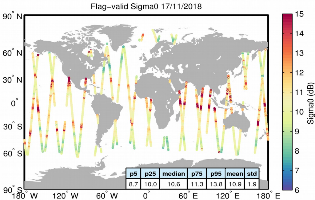
Figure 23. Geographical distribution of flag-valid sigma0 data over oceans and lakes for 17/11/2018. The statistical values shown in the table refer to the sigma0 in dB and are calculated over all measurements shown in the figure.
