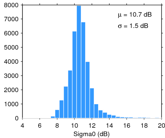
Figure 28. Histogram of science-valid sigma0 over oceans and lakes for 17/11/2018. The mean ( \mu ) and standard deviation ( \sigma ) are also shown. Note that values outside [4 20] dB are excluded from the histogram for the sake of readability but not from the computation of \mu and \sigma .
