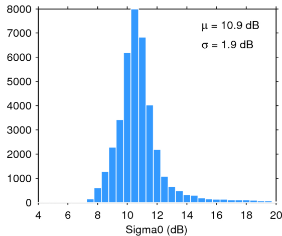
Figure 25. Histogram of flag-valid sigma0 over oceans and lakes for 17/11/2018. The mean ( \mu ) and standard deviation ( \sigma ) are also shown. Note that values outside [4 20] dB are excluded from the histogram for the sake of readability but not from the computation of \mu and \sigma .
