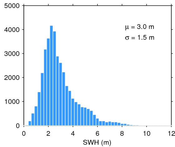
Figure 17. Histogram of flag-valid SWH over oceans and lakes for 17/11/2018. The mean ( \mu ) and standard deviation ( \sigma ) are also shown. Note that values larger than 12 m are excluded from the histogram for the sake of readability but not from the computation of \mu and \sigma .
