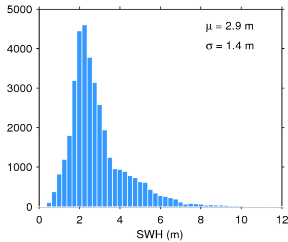
Figure 17. Histogram of flag-valid SWH over oceans and lakes for 15/11/2018. The mean ( \mu ) and standard deviation ( \sigma ) are also shown. Note that values larger than 12 m are excluded from the histogram for the sake of readability but not from the computation of \mu and \sigma .
