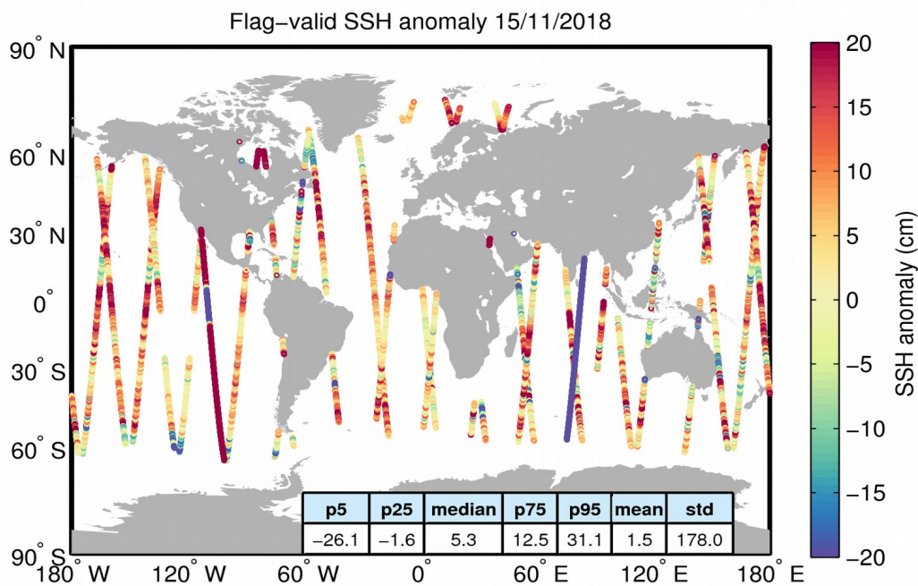
Figure 5. Geographical distribution of flag-valid 1-Hz SSH anomaly data over oceans and lakes for 15/11/2018. The statistical values shown in the table refer to the SSH anomaly in cm and are calculated over all measurements shown in the figure.
