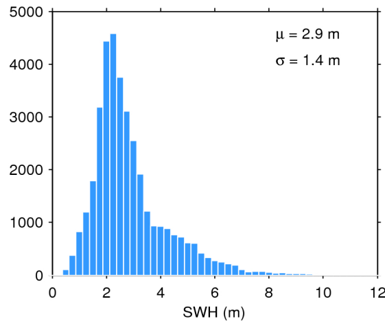
Figure 20. Histogram of science-valid SWH over oceans and lakes for 15/11/2018. The mean ( \mu ) and standard deviation ( \sigma ) are also shown. Note that values larger than 12 m are excluded from the histogram for the sake of readability but not from the computation of \mu and \sigma .
