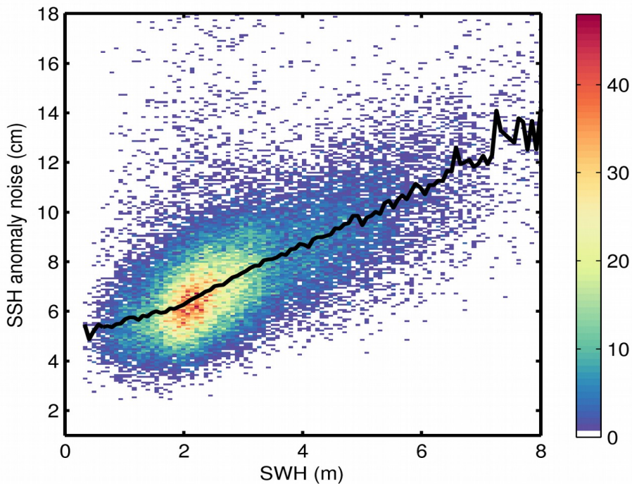
Figure 9. 2D histogram showing flag-valid SSH anomaly noise as a function of SWH for 15/11/2018. The black line denotes the median SSH anomaly noise as a function of SWH.
