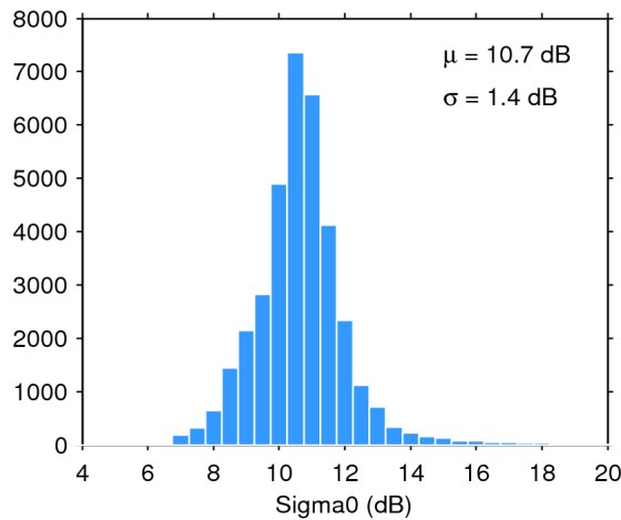
Figure 28. Histogram of science-valid sigma0 over oceans and lakes for 15/11/2018. The mean ( \mu ) and standard deviation ( \sigma ) are also shown. Note that values outside [4 20] dB are excluded from the histogram for the sake of readability but not from the computation of \mu and \sigma .
