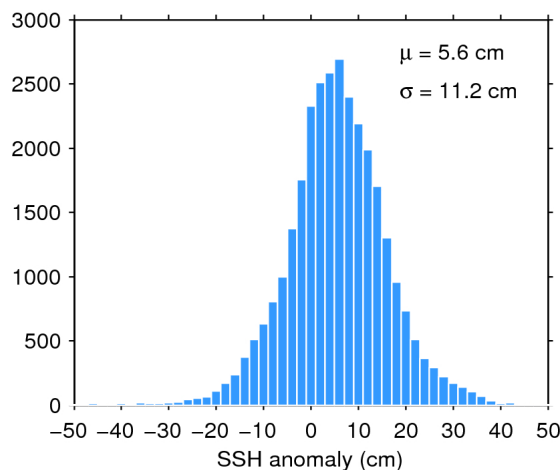
Figure 11. Histogram of science-valid SSH anomaly over oceans and lakes for 15/11/2018. The mean ( \mu ) and standard deviation ( \sigma ) are also shown. Note that values outside [-50 50] cm are excluded from the histogram for the sake of readability but not from the computation of \mu and \sigma .
