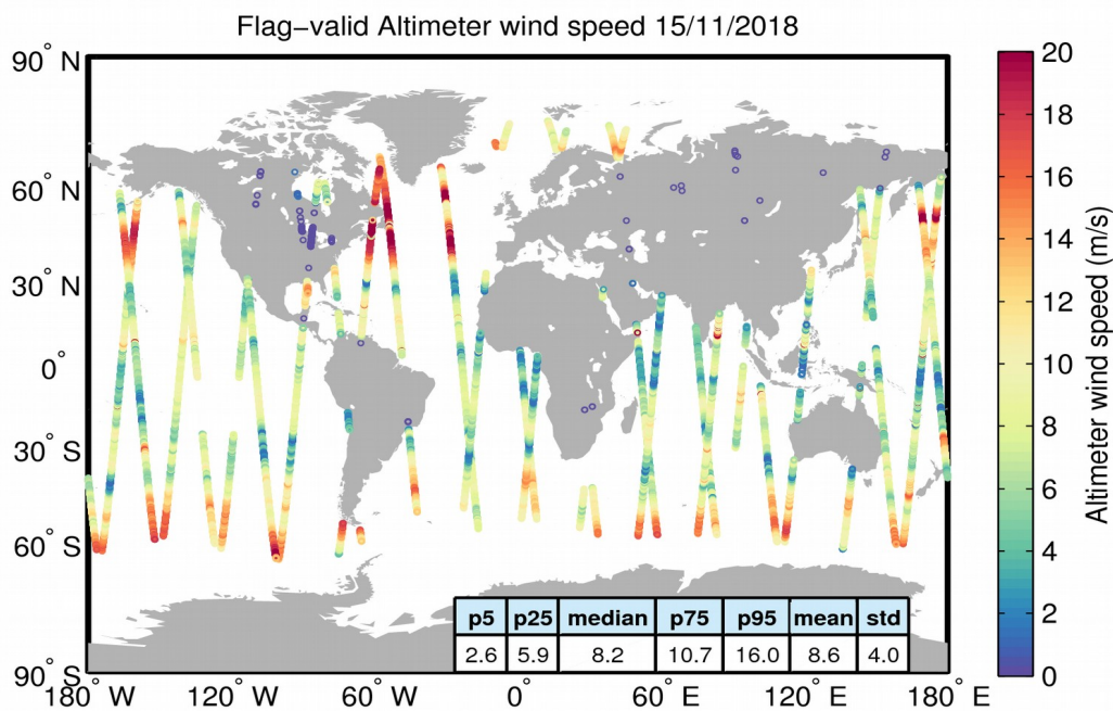
Figure 31. Geographical distribution of flag-valid wind data over oceans and lakes for 15/11/2018. The statistical values shown in the table refer to the wind in m/s and are calculated over all measurements shown in the figure.
