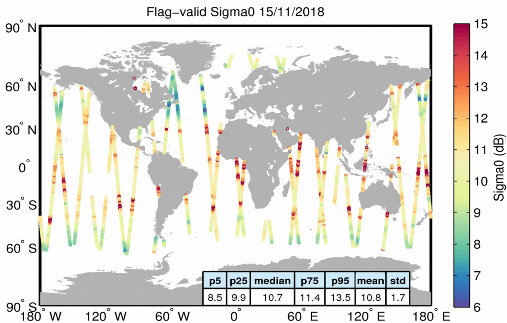
Figure 23. Geographical distribution of flag-valid sigma0 data over oceans and lakes for 15/11/2018. The statistical values shown in the table refer to the sigma0 in dB and are calculated over all measurements shown in the figure.
