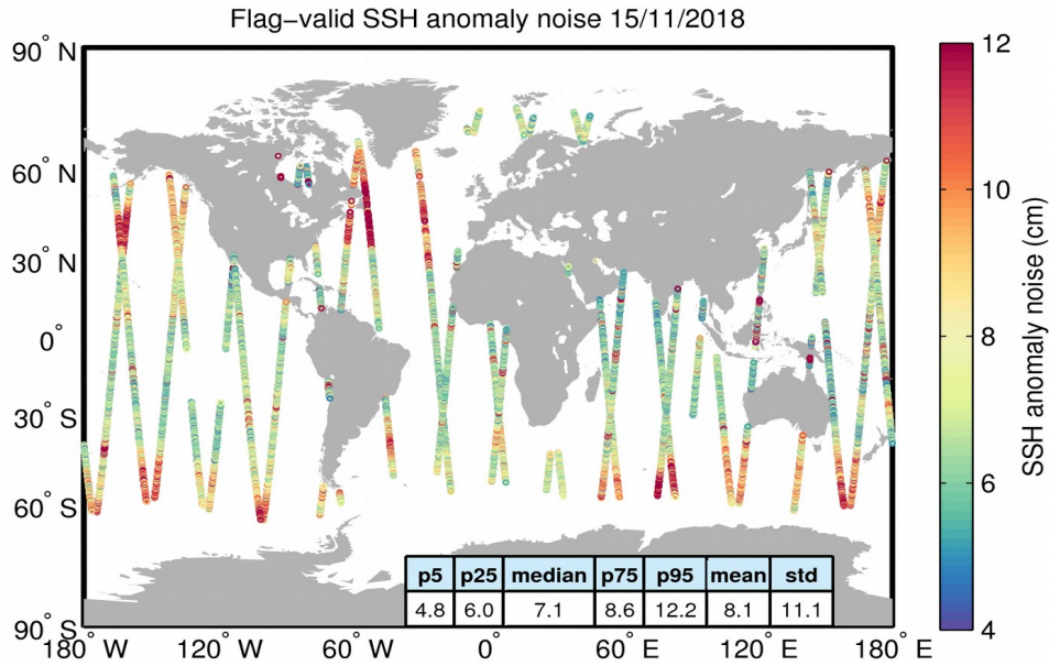
Figure 8. Geographical distribution of flag-valid 20-Hz SSH anomaly measurement noise over oceans and lakes for 15/11/2018. The statistical values shown in the table refer to the SSH anomaly noise and are calculated over all measurements shown in the figure.
