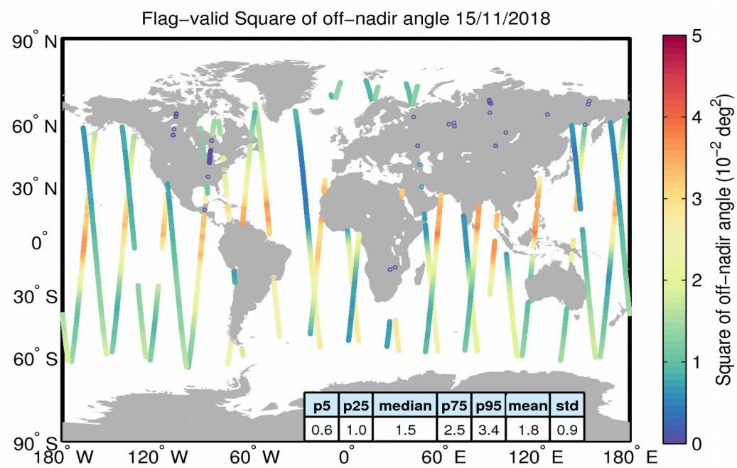
Figure 37. Geographical distribution of flag-valid mispointing data over oceans and lakes for 15/11/2018. The statistical values shown in the table refer to the mispointing in 10^{-2} deg 2 and are calculated over all measurements shown in the figure.
