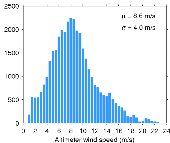
Figure 35. Histogram of science-valid wind over oceans and lakes for 15/11/2018. The mean ( \mu ) and standard deviation ( \sigma ) are also shown. Note that values larger than 24 m/s are excluded from the histogram for the sake of readability but not from the computation of \mu and \sigma .
