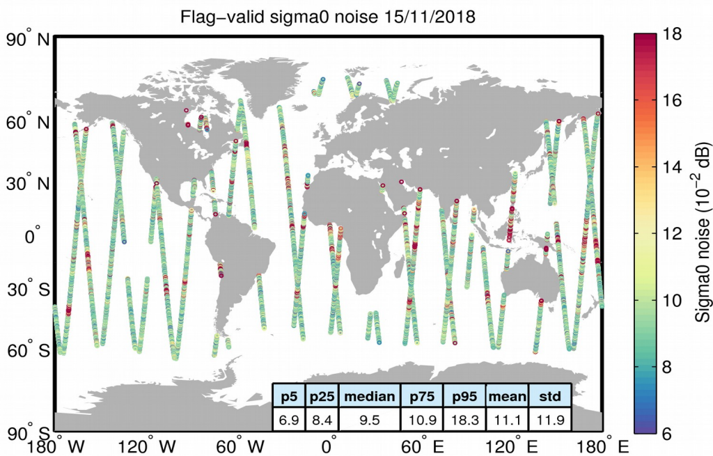
Figure 26. Geographical distribution of flag-valid 20-Hz sigma0 measurement noise over oceans and lakes for 15/11/2018. The statistical values shown in the table refer to the sigma0 noise and are calculated over all measurements shown in the figure.
