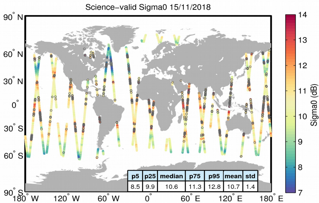
Figure 27. Geographical distribution of science-valid sigma0 data over oceans and lakes for 15/11/2018. The statistical values shown in the table refer to the sigma0 in dB and are calculated over all measurements shown in the figure. Gray circles denote records that have been rejected based on the editing criteria described in Table 4.
