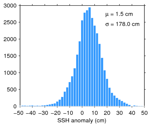
Figure 7. Histogram of flag-valid SSH anomaly over oceans and lakes for 15/11/2018. The mean ( \mu ) and standard deviation ( \sigma ) are also shown. Note that values outside [-50 50] cm are excluded from the histogram for the sake of readability but not from the computation of \mu and \sigma .
