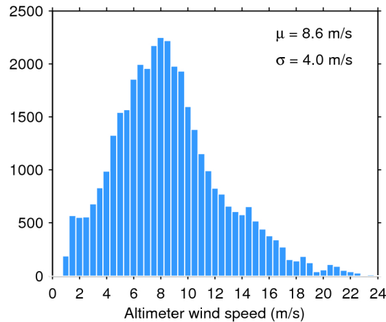
Figure 33. Histogram of flag-valid wind over oceans and lakes for 15/11/2018. The mean ( \mu ) and standard deviation ( \sigma ) are also shown. Note that values larger than 24 m/s are excluded from the histogram for the sake of readability but not from the computation of \mu and \sigma .
