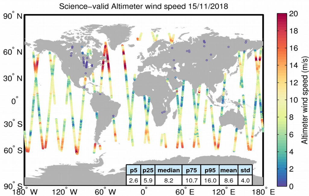
Figure 34. Geographical distribution of science-valid wind data over oceans and lakes for 15/11/2018. The statistical values shown in the table refer to the wind in m/s and are calculated over all measurements shown in the figure. Gray circles denote records that have been rejected based on the editing criteria described in Table 5.
