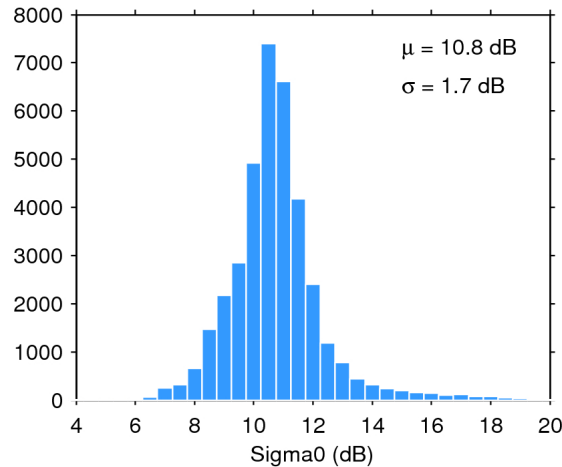
Figure 25. Histogram of flag-valid sigma0 over oceans and lakes for 15/11/2018. The mean ( \mu ) and standard deviation ( \sigma ) are also shown. Note that values outside [4 20] dB are excluded from the histogram for the sake of readability but not from the computation of \mu and \sigma .
