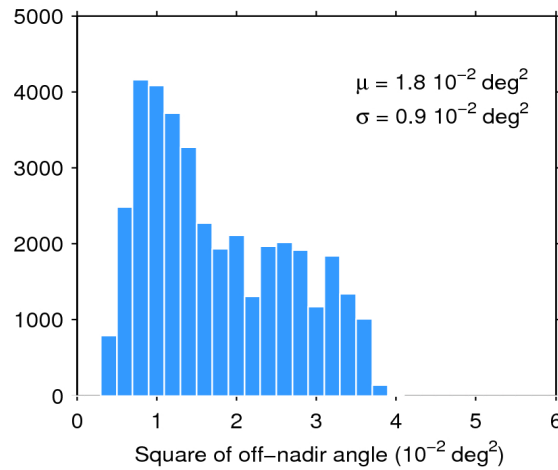
Figure 39. Histogram of flag-valid mispointing over oceans and lakes for 15/11/2018. The mean ( \mu ) and standard deviation ( \sigma ) are also shown. Note that values larger than 6 \cdot 10^{-2} \text{ deg}^2 are excluded from the histogram for the sake of readability but not from the computation of \mu and \sigma .
