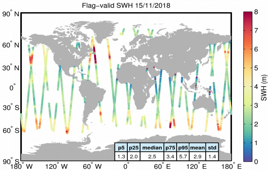
Figure 15. Geographical distribution of flag-valid SWH data over oceans and lakes for 15/11/2018. The statistical values shown in the table refer to the SWH in m and are calculated over all measurements shown in the figure.
