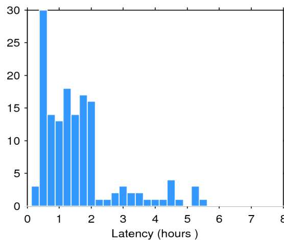
Figure 2. Histogram of the data latency for 15/11/2018. The y-axis denotes the number of files that are made available with a delay of x-hours with respect to the mean time of the records stored in the file.
