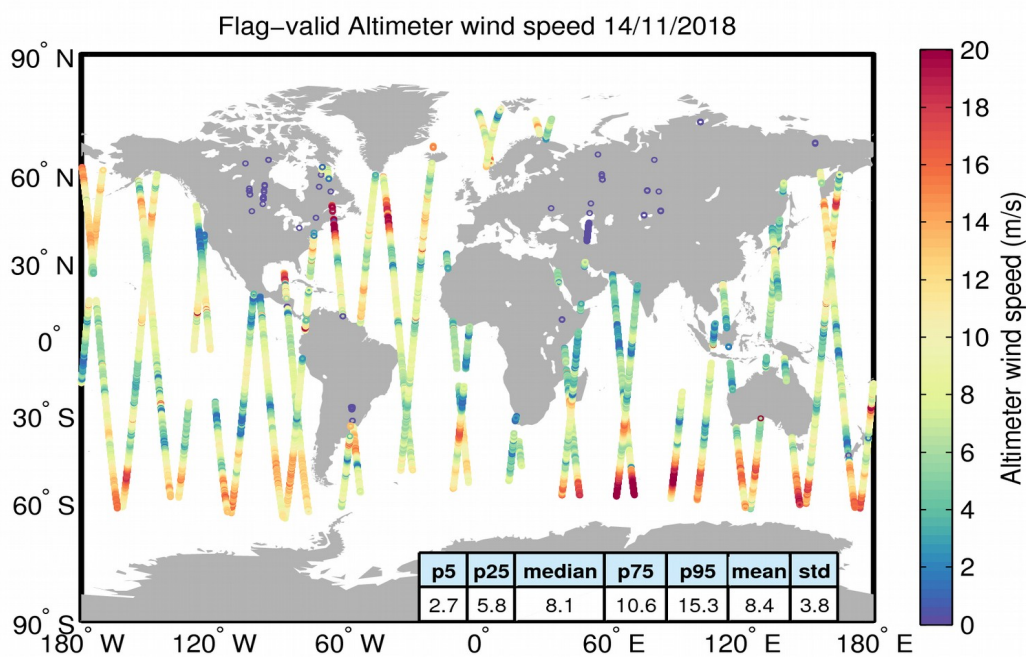
Figure 31. Geographical distribution of flag-valid wind data over oceans and lakes for 14/11/2018. The statistical values shown in the table refer to the wind in m/s and are calculated over all measurements shown in the figure.
