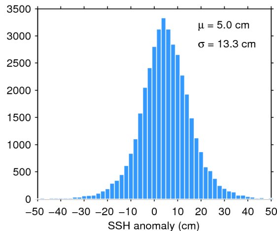
Figure 11. Histogram of science-valid SSH anomaly over oceans and lakes for 14/11/2018. The mean ( \mu ) and standard deviation ( \sigma ) are also shown. Note that values outside [-50 50] cm are excluded from the histogram for the sake of readability but not from the computation of \mu and \sigma .
