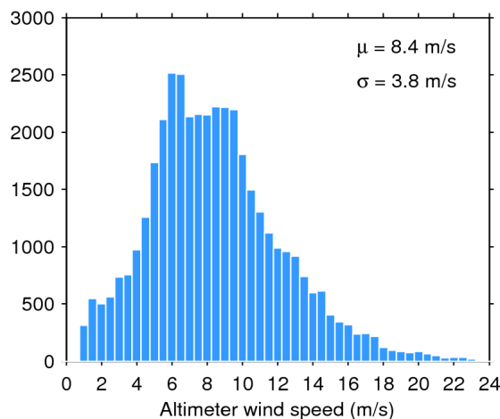
Figure 35. Histogram of science-valid wind over oceans and lakes for 14/11/2018. The mean ( \mu ) and standard deviation ( \sigma ) are also shown. Note that values larger than 24 m/s are excluded from the histogram for the sake of readability but not from the computation of \mu and \sigma .
