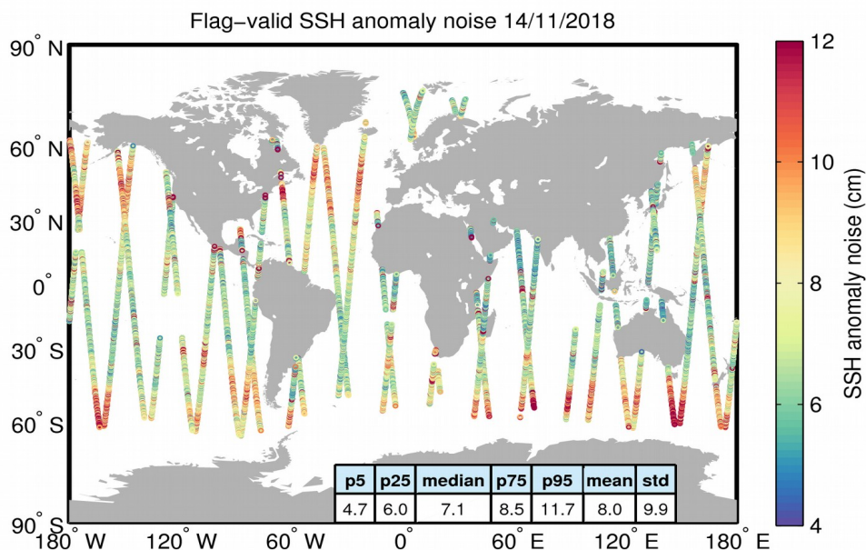
Figure 8. Geographical distribution of flag-valid 20-Hz SSH anomaly measurement noise over oceans and lakes for 14/11/2018. The statistical values shown in the table refer to the SSH anomaly noise and are calculated over all measurements shown in the figure.
