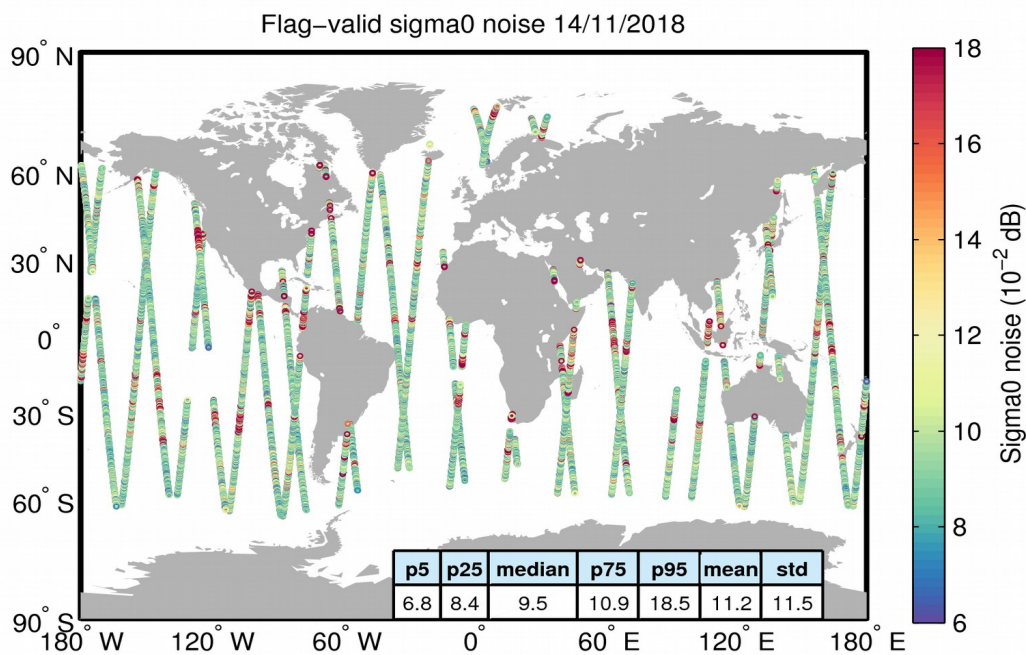
Figure 26. Geographical distribution of flag-valid 20-Hz sigma0 measurement noise over oceans and lakes for 14/11/2018. The statistical values shown in the table refer to the sigma0 noise and are calculated over all measurements shown in the figure.
