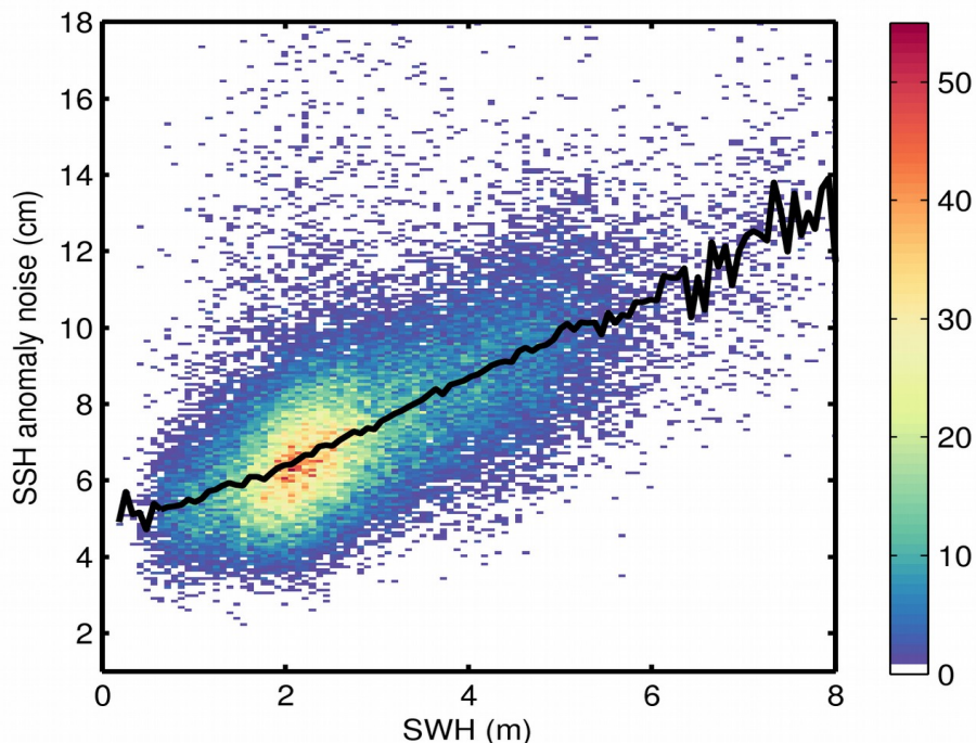
Figure 9. 2D histogram showing flag-valid SSH anomaly noise as a function of SWH for 14/11/2018. The black line denotes the median SSH anomaly noise as a function of SWH.
