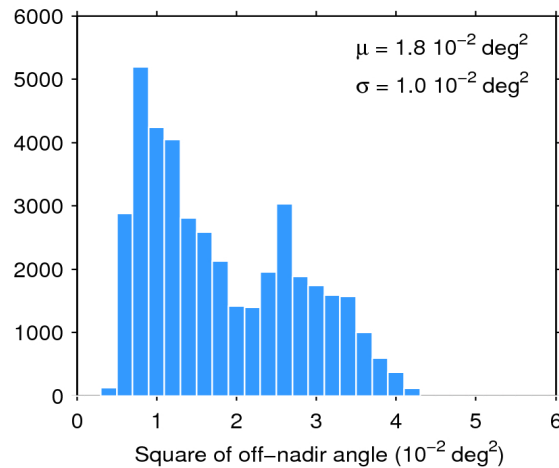
Figure 39. Histogram of flag-valid mispointing over oceans and lakes for 14/11/2018. The mean ( \mu ) and standard deviation ( \sigma ) are also shown. Note that values larger than 6 \cdot 10^{-2} \text{ deg}^2 are excluded from the histogram for the sake of readability but not from the computation of \mu and \sigma .
