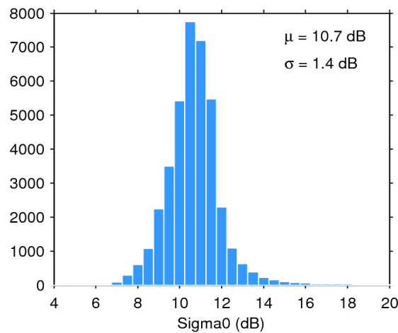
Figure 28. Histogram of science-valid sigma0 over oceans and lakes for 14/11/2018. The mean ( \mu ) and standard deviation ( \sigma ) are also shown. Note that values outside [4 20] dB are excluded from the histogram for the sake of readability but not from the computation of \mu and \sigma .
