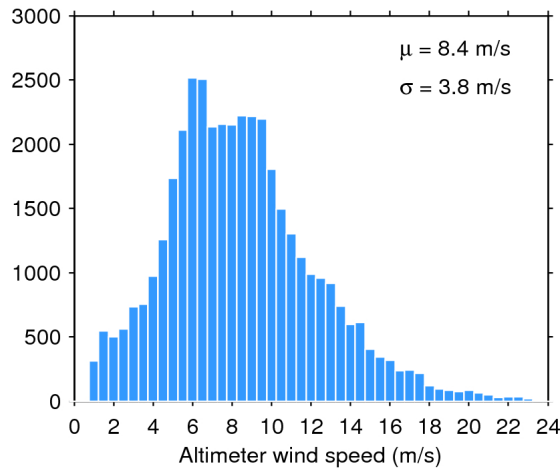
Figure 33. Histogram of flag-valid wind over oceans and lakes for 14/11/2018. The mean ( \mu ) and standard deviation ( \sigma ) are also shown. Note that values larger than 24 m/s are excluded from the histogram for the sake of readability but not from the computation of \mu and \sigma .
