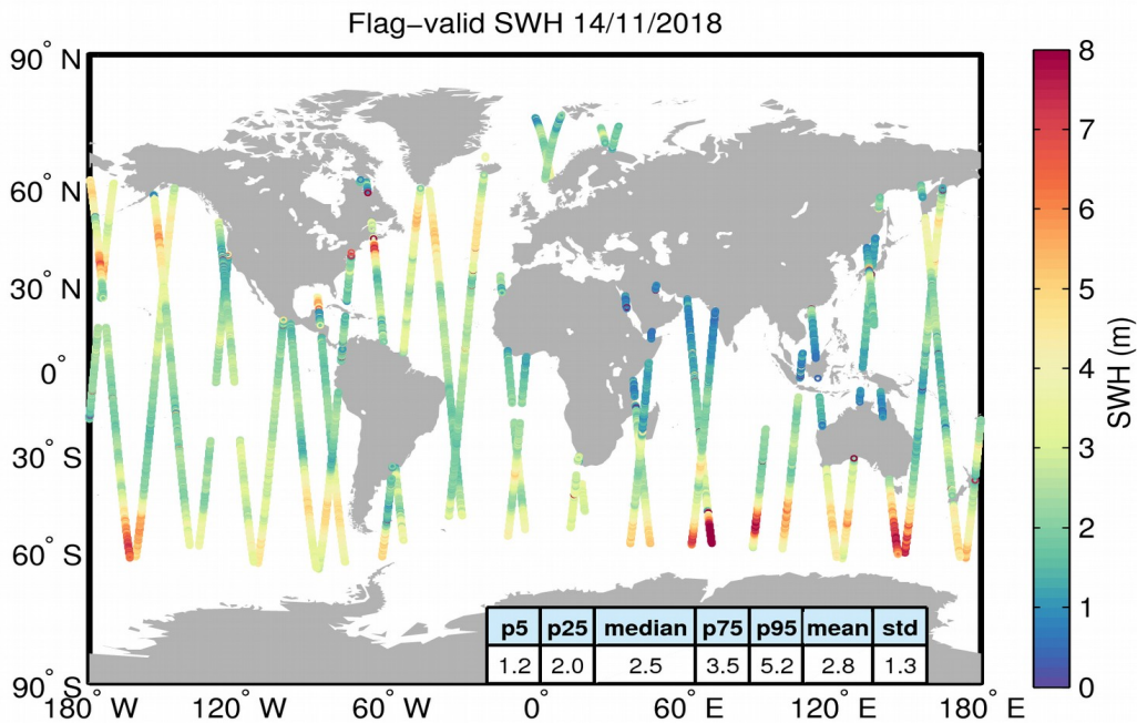
Figure 15. Geographical distribution of flag-valid SWH data over oceans and lakes for 14/11/2018. The statistical values shown in the table refer to the SWH in m and are calculated over all measurements shown in the figure.
