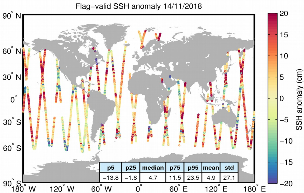
Figure 5. Geographical distribution of flag-valid 1-Hz SSH anomaly data over oceans and lakes for 14/11/2018. The statistical values shown in the table refer to the SSH anomaly in cm and are calculated over all measurements shown in the figure.
