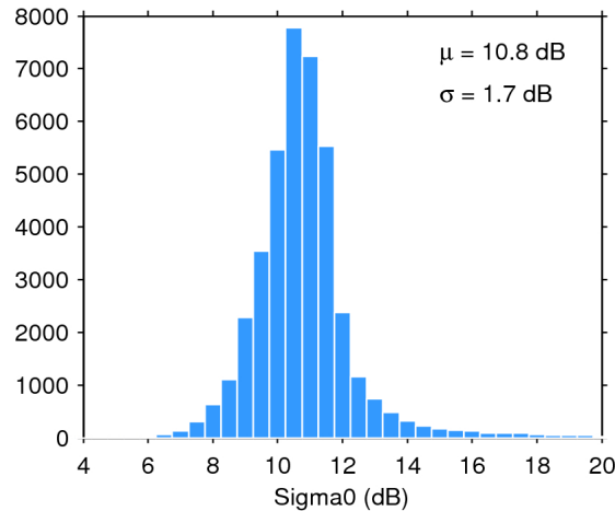
Figure 25. Histogram of flag-valid sigma0 over oceans and lakes for 14/11/2018. The mean ( \mu ) and standard deviation ( \sigma ) are also shown. Note that values outside [4 20] dB are excluded from the histogram for the sake of readability but not from the computation of \mu and \sigma .
