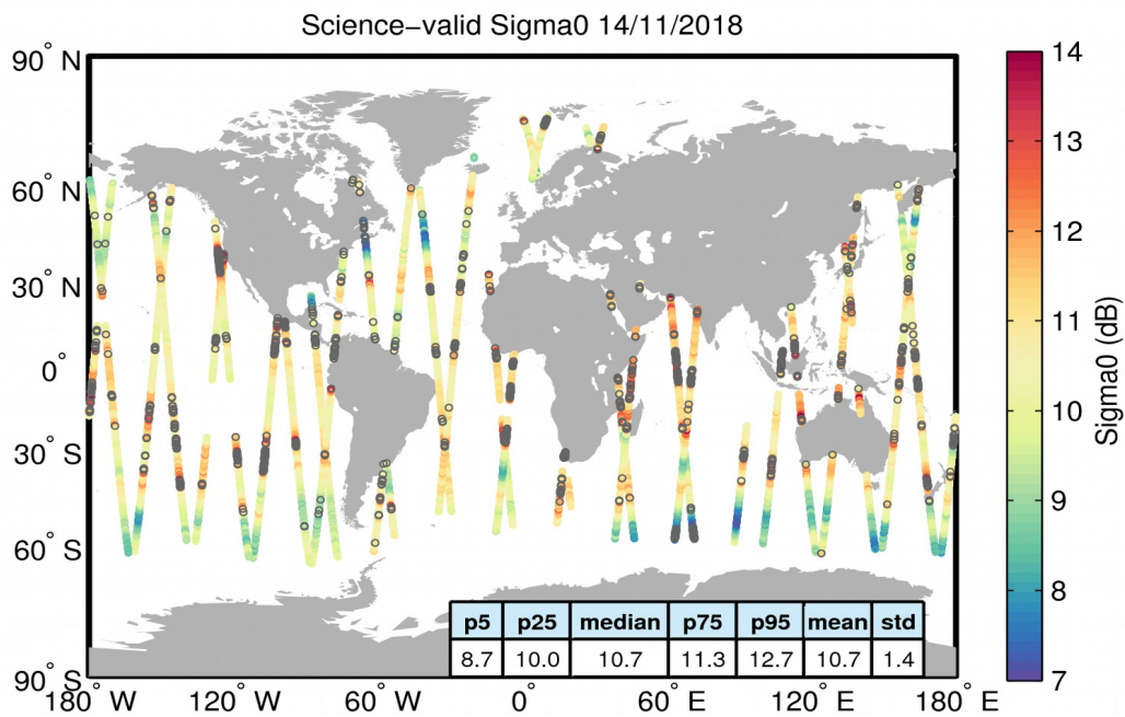
Figure 27. Geographical distribution of science-valid sigma0 data over oceans and lakes for 14/11/2018. The statistical values shown in the table refer to the sigma0 in dB and are calculated over all measurements shown in the figure. Gray circles denote records that have been rejected based on the editing criteria described in Table 4.
