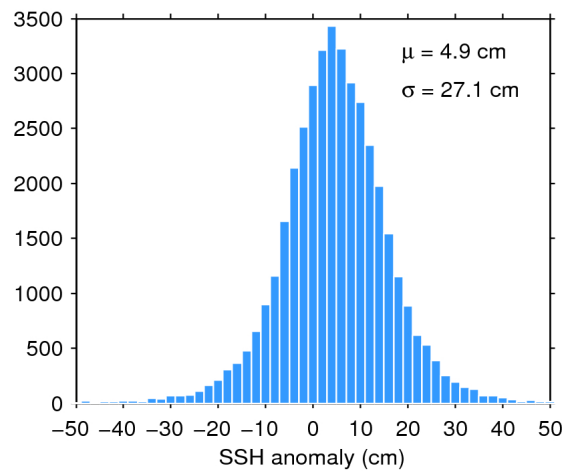
Figure 7. Histogram of flag-valid SSH anomaly over oceans and lakes for 14/11/2018. The mean ( \mu ) and standard deviation ( \sigma ) are also shown. Note that values outside [-50\ 50] cm are excluded from the histogram for the sake of readability but not from the computation of \mu and \sigma .
