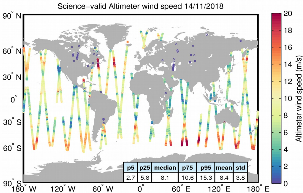
Figure 34. Geographical distribution of science-valid wind data over oceans and lakes for 14/11/2018. The statistical values shown in the table refer to the wind in m/s and are calculated over all measurements shown in the figure. Gray circles denote records that have been rejected based on the editing criteria described in Table 5.
