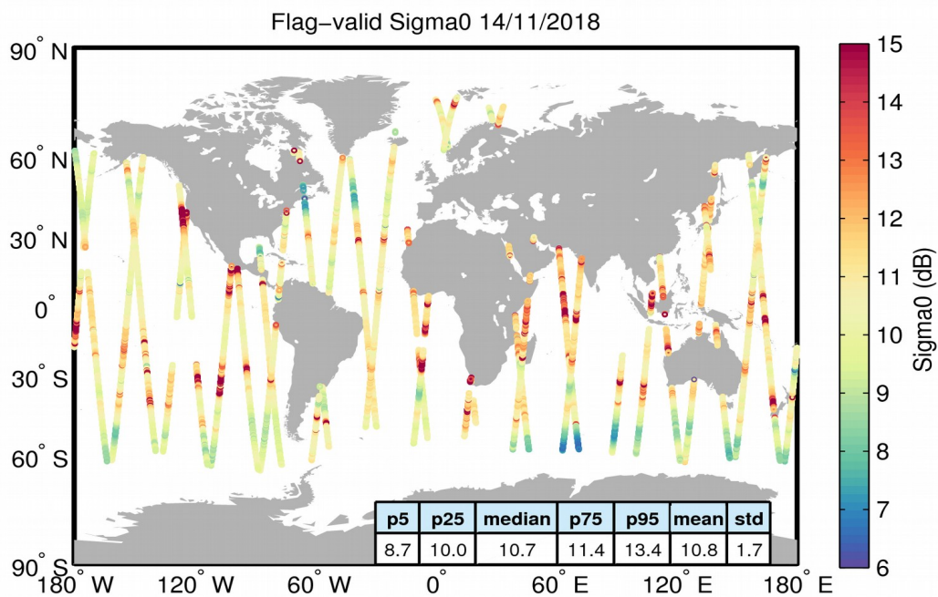
Figure 23. Geographical distribution of flag-valid sigma0 data over oceans and lakes for 14/11/2018. The statistical values shown in the table refer to the sigma0 in dB and are calculated over all measurements shown in the figure.
