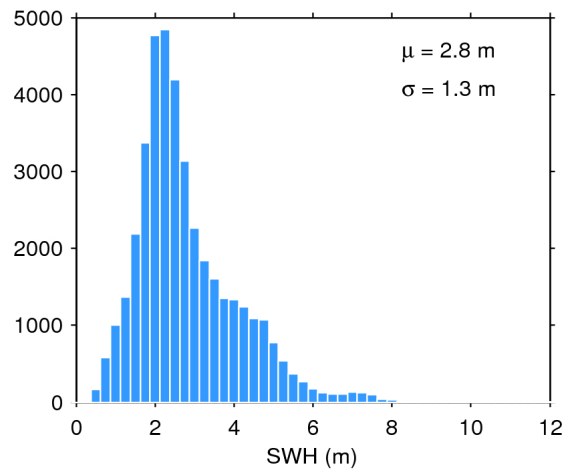
Figure 17. Histogram of flag-valid SWH over oceans and lakes for 14/11/2018. The mean ( \mu ) and standard deviation ( \sigma ) are also shown. Note that values larger than 12 m are excluded from the histogram for the sake of readability but not from the computation of \mu and \sigma .
