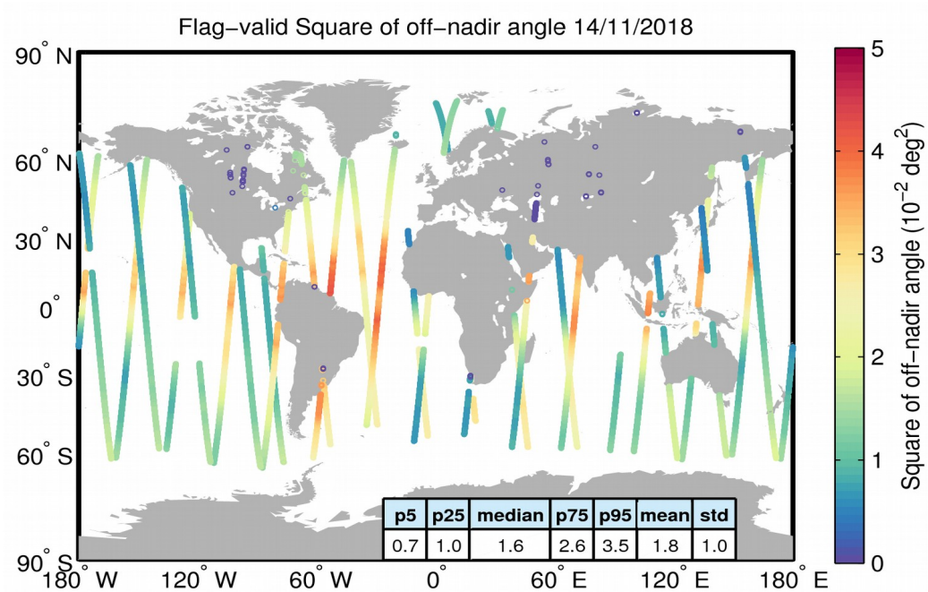
Figure 37. Geographical distribution of flag-valid mispointing data over oceans and lakes for 14/11/2018. The statistical values shown in the table refer to the mispointing in 10^{-2} deg 2 and are calculated over all measurements shown in the figure.
