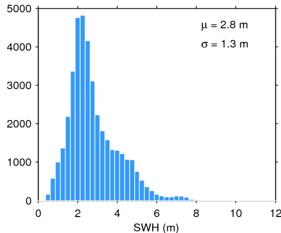
Figure 20. Histogram of science-valid SWH over oceans and lakes for 14/11/2018. The mean ( \mu ) and standard deviation ( \sigma ) are also shown. Note that values larger than 12 m are excluded from the histogram for the sake of readability but not from the computation of \mu and \sigma .
