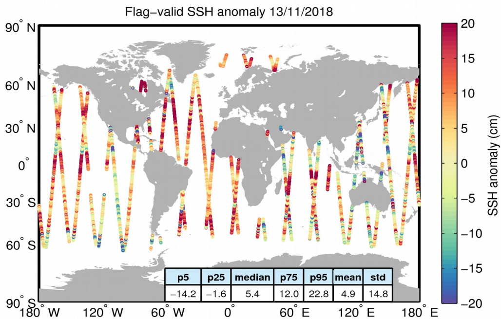
Figure 5. Geographical distribution of flag-valid 1-Hz SSH anomaly data over oceans and lakes for 13/11/2018. The statistical values shown in the table refer to the SSH anomaly in cm and are calculated over all measurements shown in the figure.
