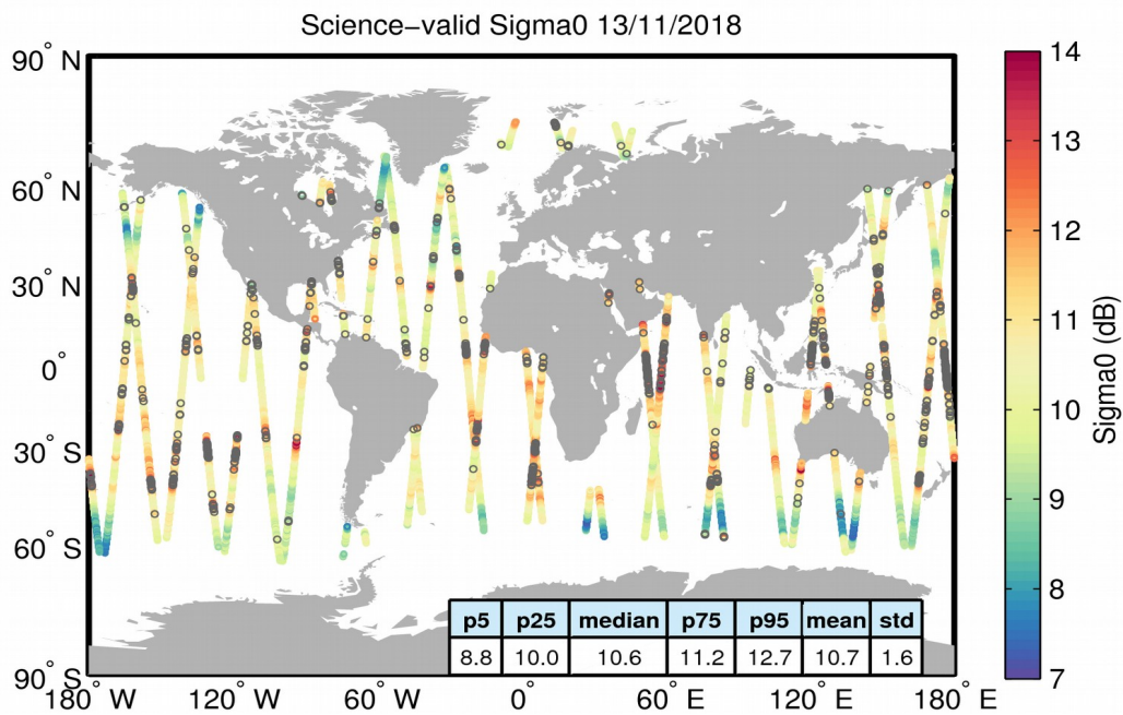
Figure 27. Geographical distribution of science-valid sigma0 data over oceans and lakes for 13/11/2018. The statistical values shown in the table refer to the sigma0 in dB and are calculated over all measurements shown in the figure. Gray circles denote records that have been rejected based on the editing criteria described in Table 4.
