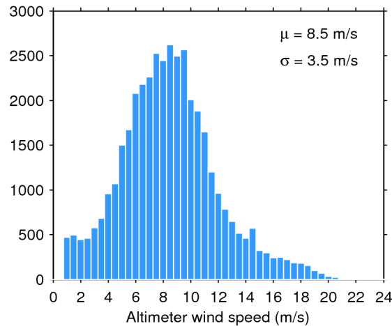
Figure 33. Histogram of flag-valid wind over oceans and lakes for 13/11/2018. The mean ( \mu ) and standard deviation ( \sigma ) are also shown. Note that values larger than 24 m/s are excluded from the histogram for the sake of readability but not from the computation of \mu and \sigma .
