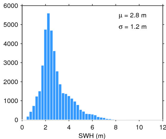
Figure 20. Histogram of science-valid SWH over oceans and lakes for 13/11/2018. The mean ( \mu ) and standard deviation ( \sigma ) are also shown. Note that values larger than 12 m are excluded from the histogram for the sake of readability but not from the computation of \mu and \sigma .
