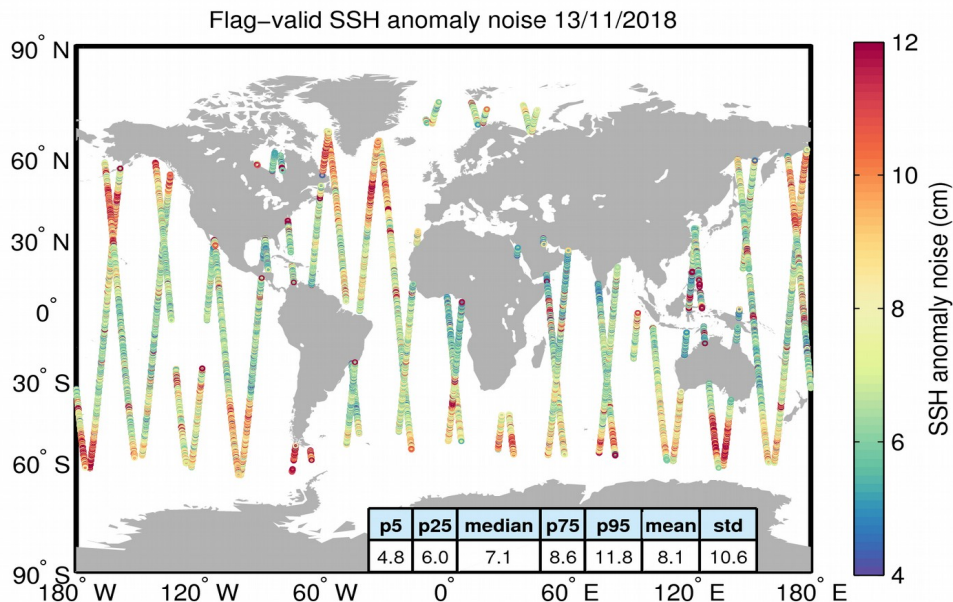
Figure 8. Geographical distribution of flag-valid 20-Hz SSH anomaly measurement noise over oceans and lakes for 13/11/2018. The statistical values shown in the table refer to the SSH anomaly noise and are calculated over all measurements shown in the figure.
