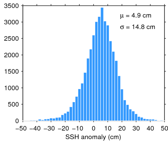
Figure 7. Histogram of flag-valid SSH anomaly over oceans and lakes for 13/11/2018. The mean ( \mu ) and standard deviation ( \sigma ) are also shown. Note that values outside [-50\ 50] cm are excluded from the histogram for the sake of readability but not from the computation of \mu and \sigma .
