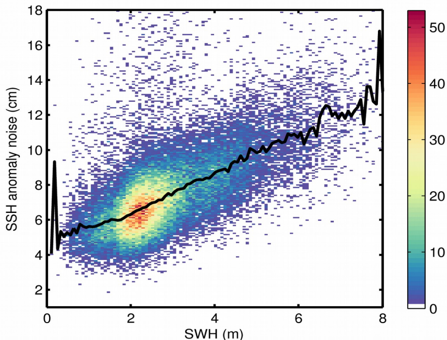
Figure 9. 2D histogram showing flag-valid SSH anomaly noise as a function of SWH for 13/11/2018. The black line denotes the median SSH anomaly noise as a function of SWH.
