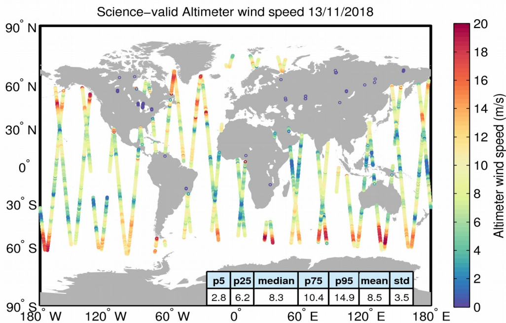
Figure 34. Geographical distribution of science-valid wind data over oceans and lakes for 13/11/2018. The statistical values shown in the table refer to the wind in m/s and are calculated over all measurements shown in the figure. Gray circles denote records that have been rejected based on the editing criteria described in Table 5.
