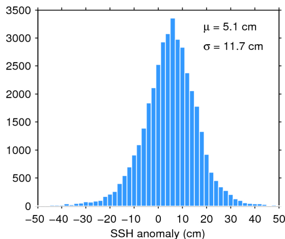
Figure 11. Histogram of science-valid SSH anomaly over oceans and lakes for 13/11/2018. The mean ( \mu ) and standard deviation ( \sigma ) are also shown. Note that values outside [-50 50] cm are excluded from the histogram for the sake of readability but not from the computation of \mu and \sigma .
