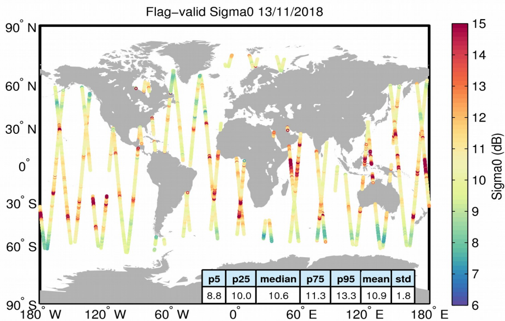
Figure 23. Geographical distribution of flag-valid sigma0 data over oceans and lakes for 13/11/2018. The statistical values shown in the table refer to the sigma0 in dB and are calculated over all measurements shown in the figure.
