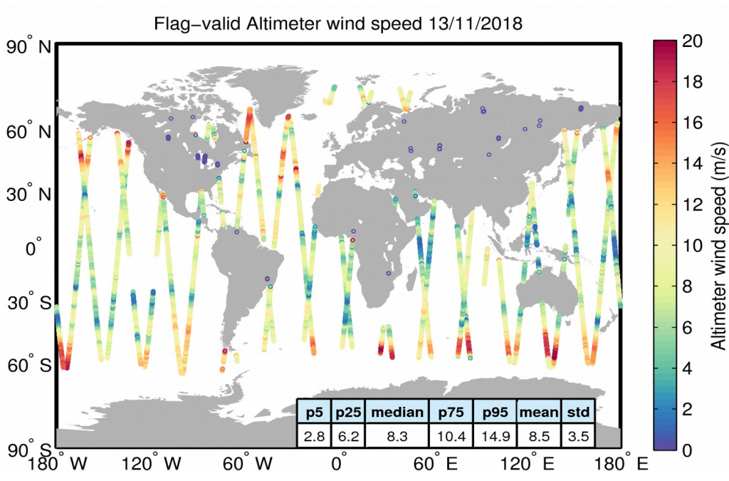
Figure 31. Geographical distribution of flag-valid wind data over oceans and lakes for 13/11/2018. The statistical values shown in the table refer to the wind in m/s and are calculated over all measurements shown in the figure.
