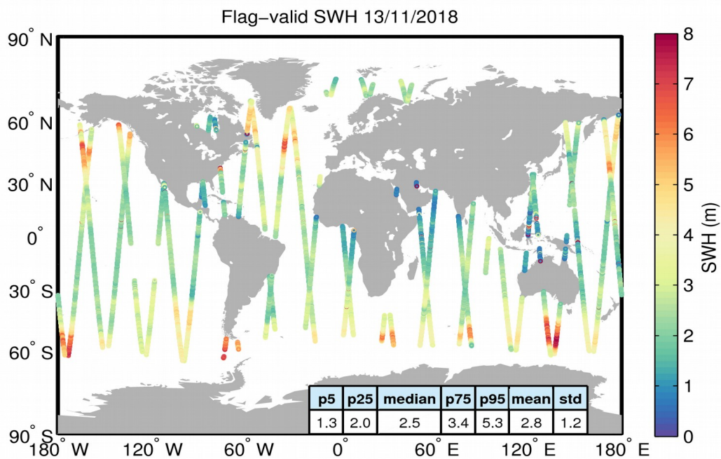
Figure 15. Geographical distribution of flag-valid SWH data over oceans and lakes for 13/11/2018. The statistical values shown in the table refer to the SWH in m and are calculated over all measurements shown in the figure.
