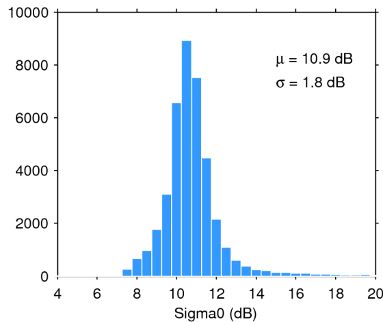
Figure 25. Histogram of flag-valid sigma0 over oceans and lakes for 13/11/2018. The mean ( \mu ) and standard deviation ( \sigma ) are also shown. Note that values outside [4 20] dB are excluded from the histogram for the sake of readability but not from the computation of \mu and \sigma .
