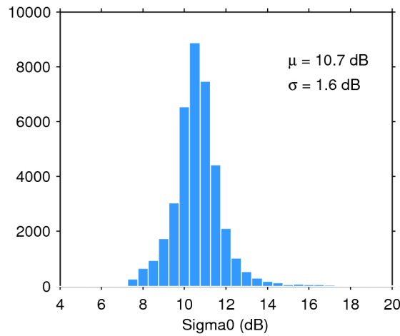
Figure 28. Histogram of science-valid sigma0 over oceans and lakes for 13/11/2018. The mean ( \mu ) and standard deviation ( \sigma ) are also shown. Note that values outside [4 20] dB are excluded from the histogram for the sake of readability but not from the computation of \mu and \sigma .
