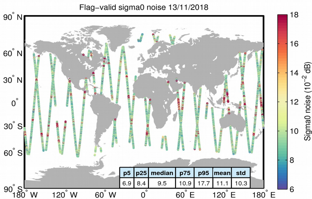
Figure 26. Geographical distribution of flag-valid 20-Hz sigma0 measurement noise over oceans and lakes for 13/11/2018. The statistical values shown in the table refer to the sigma0 noise and are calculated over all measurements shown in the figure.
