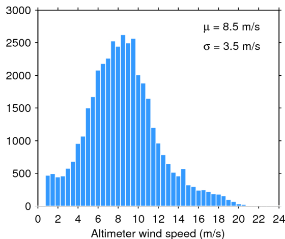
Figure 35. Histogram of science-valid wind over oceans and lakes for 13/11/2018. The mean ( \mu ) and standard deviation ( \sigma ) are also shown. Note that values larger than 24 m/s are excluded from the histogram for the sake of readability but not from the computation of \mu and \sigma .
