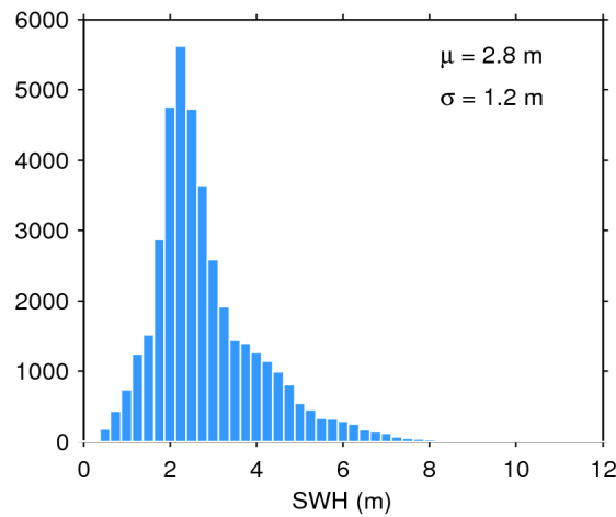
Figure 17. Histogram of flag-valid SWH over oceans and lakes for 13/11/2018. The mean ( \mu ) and standard deviation ( \sigma ) are also shown. Note that values larger than 12 m are excluded from the histogram for the sake of readability but not from the computation of \mu and \sigma .
