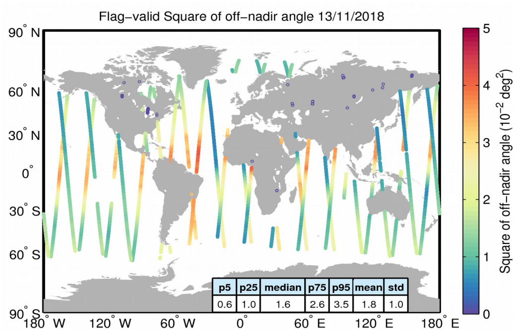
Figure 37. Geographical distribution of flag-valid mispointing data over oceans and lakes for 13/11/2018. The statistical values shown in the table refer to the mispointing in 10^{-2} deg 2 and are calculated over all measurements shown in the figure.
