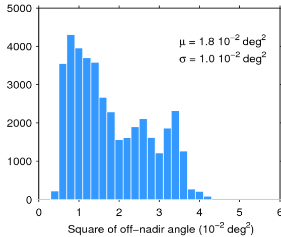
Figure 39. Histogram of flag-valid mispointing over oceans and lakes for 13/11/2018. The mean ( \mu ) and standard deviation ( \sigma ) are also shown. Note that values larger than 6 \cdot 10^{-2} \text{ deg}^2 are excluded from the histogram for the sake of readability but not from the computation of \mu and \sigma .
