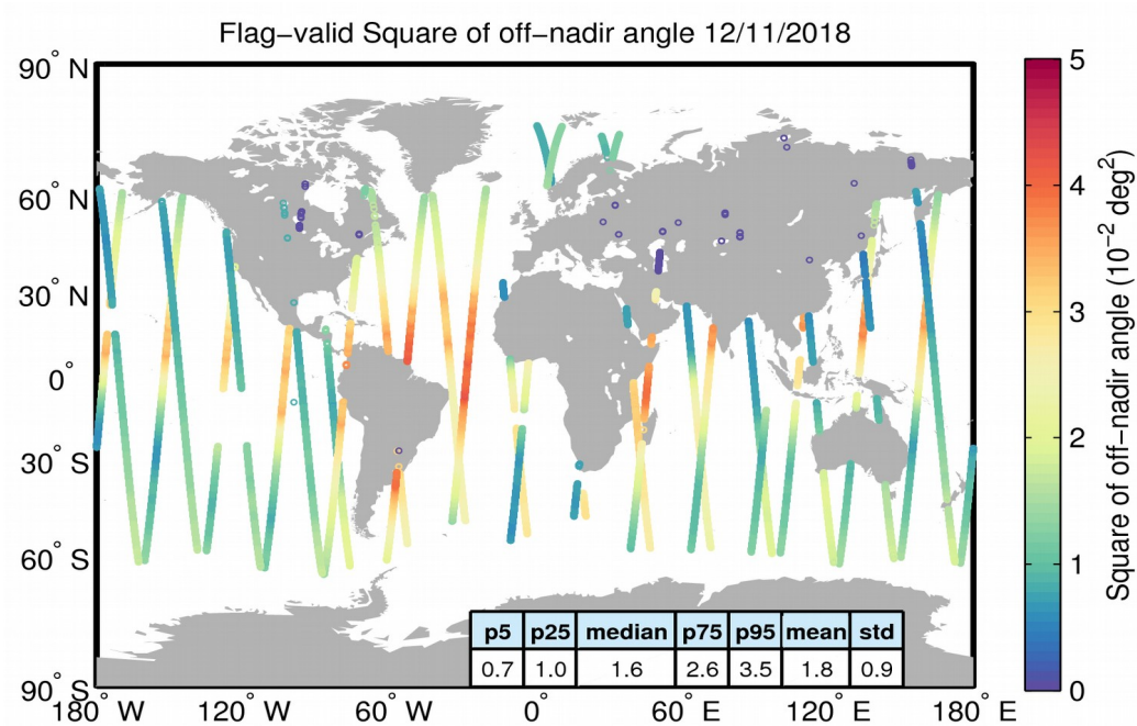
Figure 37. Geographical distribution of flag-valid mispointing data over oceans and lakes for 12/11/2018. The statistical values shown in the table refer to the mispointing in 10^{-2} \text{deg}^2 and are calculated over all measurements shown in the figure.
