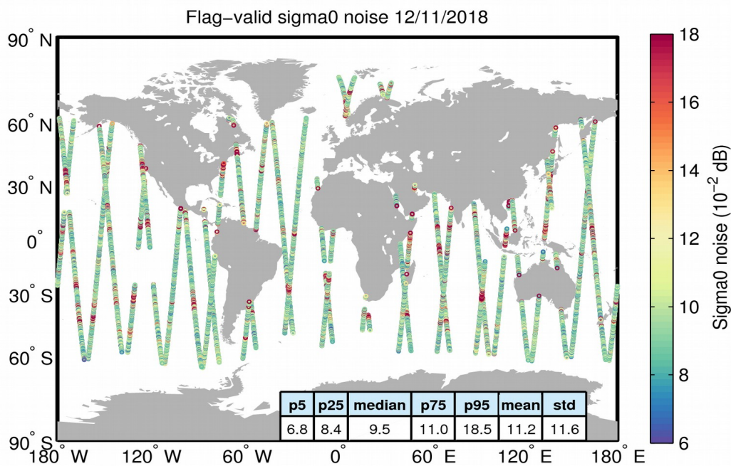
Figure 26. Geographical distribution of flag-valid 20-Hz sigma0 measurement noise over oceans and lakes for 12/11/2018. The statistical values shown in the table refer to the sigma0 noise and are calculated over all measurements shown in the figure.
