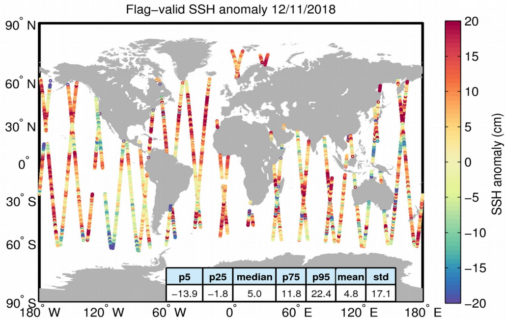
Figure 5. Geographical distribution of flag-valid 1-Hz SSH anomaly data over oceans and lakes for 12/11/2018. The statistical values shown in the table refer to the SSH anomaly in cm and are calculated over all measurements shown in the figure.
