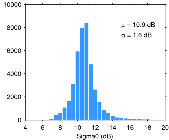
Figure 25. Histogram of flag-valid sigma0 over oceans and lakes for 12/11/2018. The mean ( \mu ) and standard deviation ( \sigma ) are also shown. Note that values outside [4 20] dB are excluded from the histogram for the sake of readability but not from the computation of \mu and \sigma .
