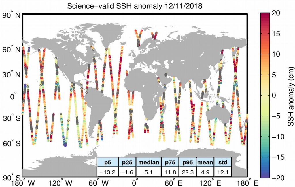
Figure 10. Geographical distribution of science-valid SSH anomaly data over oceans and lakes for 12/11/2018. The statistical values shown in the table refer to the SSH anomaly in cm and are calculated over all measurements shown in the figure. Gray circles denote records that have been rejected based on the editing criteria described in Table 2.
