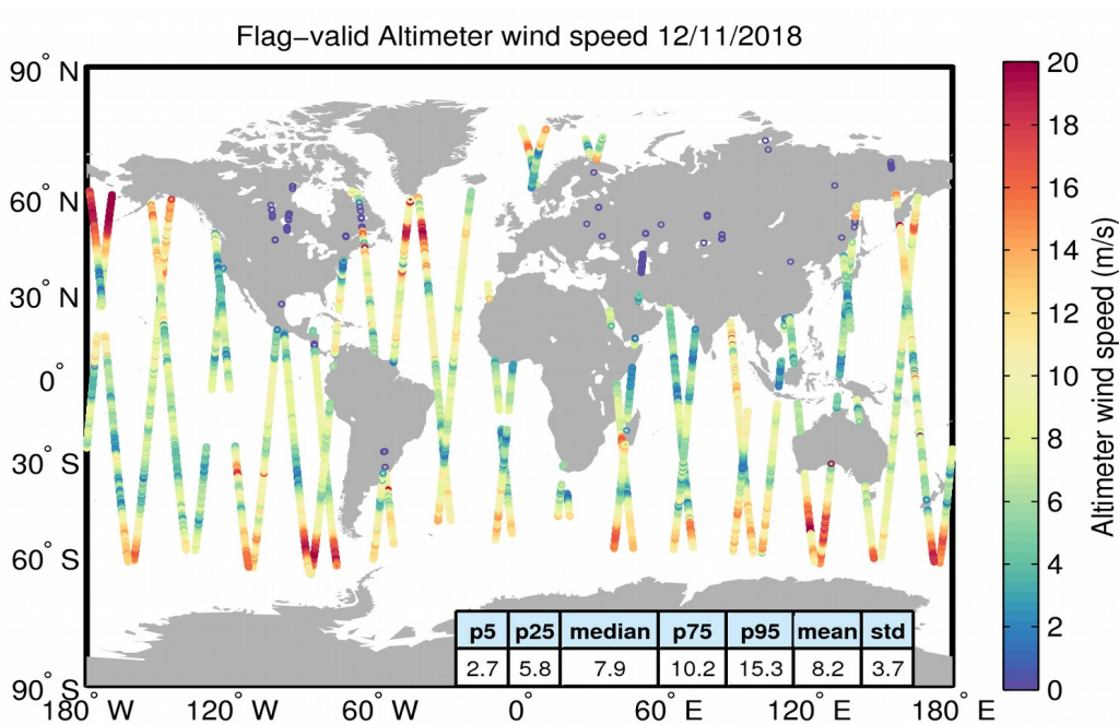
Figure 31. Geographical distribution of flag-valid wind data over oceans and lakes for 12/11/2018. The statistical values shown in the table refer to the wind in m/s and are calculated over all measurements shown in the figure.
