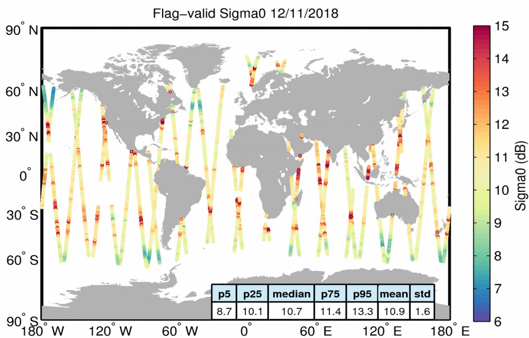
Figure 23. Geographical distribution of flag-valid sigma0 data over oceans and lakes for 12/11/2018. The statistical values shown in the table refer to the sigma0 in dB and are calculated over all measurements shown in the figure.
