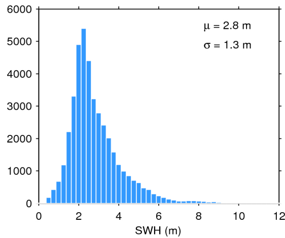
Figure 17. Histogram of flag-valid SWH over oceans and lakes for 12/11/2018. The mean ( \mu ) and standard deviation ( \sigma ) are also shown. Note that values larger than 12 m are excluded from the histogram for the sake of readability but not from the computation of \mu and \sigma .
