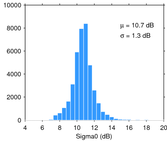
Figure 28. Histogram of science-valid sigma0 over oceans and lakes for 12/11/2018. The mean ( \mu ) and standard deviation ( \sigma ) are also shown. Note that values outside [4 20] dB are excluded from the histogram for the sake of readability but not from the computation of \mu and \sigma .
