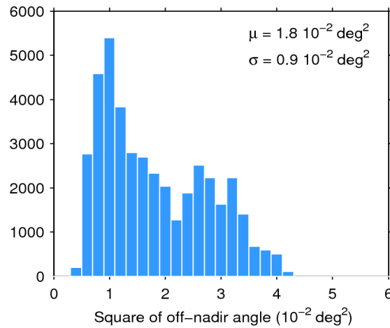
Figure 39. Histogram of flag-valid mispointing over oceans and lakes for 12/11/2018. The mean ( \mu ) and standard deviation ( \sigma ) are also shown. Note that values larger than 6 \cdot 10^{-2} \text{ deg}^2 are excluded from the histogram for the sake of readability but not from the computation of \mu and \sigma .
