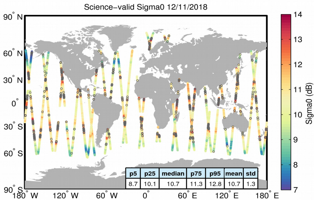
Figure 27. Geographical distribution of science-valid sigma0 data over oceans and lakes for 12/11/2018. The statistical values shown in the table refer to the sigma0 in dB and are calculated over all measurements shown in the figure. Gray circles denote records that have been rejected based on the editing criteria described in Table 4.
