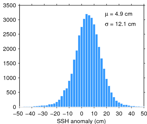
Figure 11. Histogram of science-valid SSH anomaly over oceans and lakes for 12/11/2018. The mean ( \mu ) and standard deviation ( \sigma ) are also shown. Note that values outside [-50 50] cm are excluded from the histogram for the sake of readability but not from the computation of \mu and \sigma .
