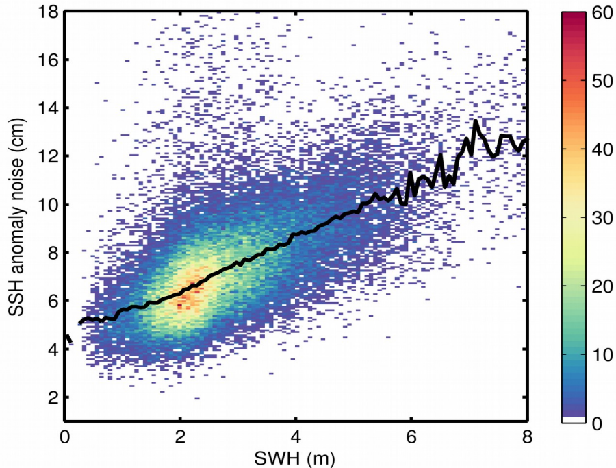
Figure 9. 2D histogram showing flag-valid SSH anomaly noise as a function of SWH for 12/11/2018. The black line denotes the median SSH anomaly noise as a function of SWH.
