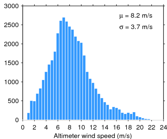
Figure 35. Histogram of science-valid wind over oceans and lakes for 12/11/2018. The mean ( \mu ) and standard deviation ( \sigma ) are also shown. Note that values larger than 24 m/s are excluded from the histogram for the sake of readability but not from the computation of \mu and \sigma .
