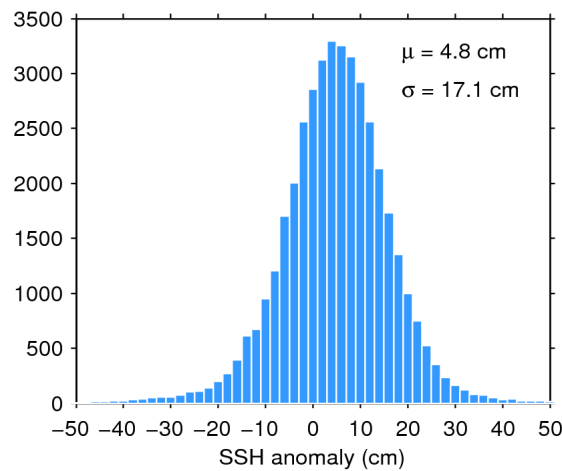
Figure 7. Histogram of flag-valid SSH anomaly over oceans and lakes for 12/11/2018. The mean ( \mu ) and standard deviation ( \sigma ) are also shown. Note that values outside [-50\ 50] cm are excluded from the histogram for the sake of readability but not from the computation of \mu and \sigma .
