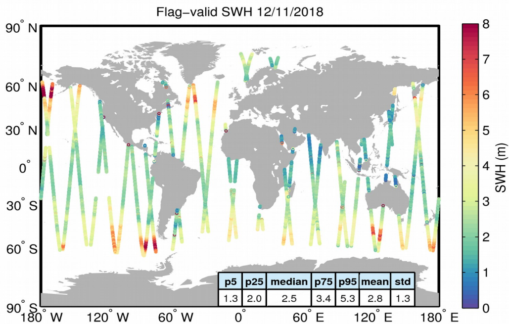
Figure 15. Geographical distribution of flag-valid SWH data over oceans and lakes for 12/11/2018. The statistical values shown in the table refer to the SWH in m and are calculated over all measurements shown in the figure.
