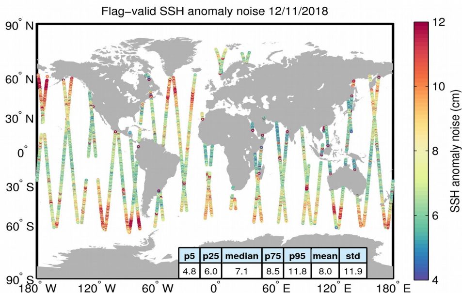
Figure 8. Geographical distribution of flag-valid 20-Hz SSH anomaly measurement noise over oceans and lakes for 12/11/2018. The statistical values shown in the table refer to the SSH anomaly noise and are calculated over all measurements shown in the figure.
