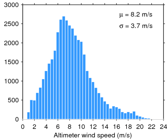
Figure 33. Histogram of flag-valid wind over oceans and lakes for 12/11/2018. The mean ( \mu ) and standard deviation ( \sigma ) are also shown. Note that values larger than 24 m/s are excluded from the histogram for the sake of readability but not from the computation of \mu and \sigma .
