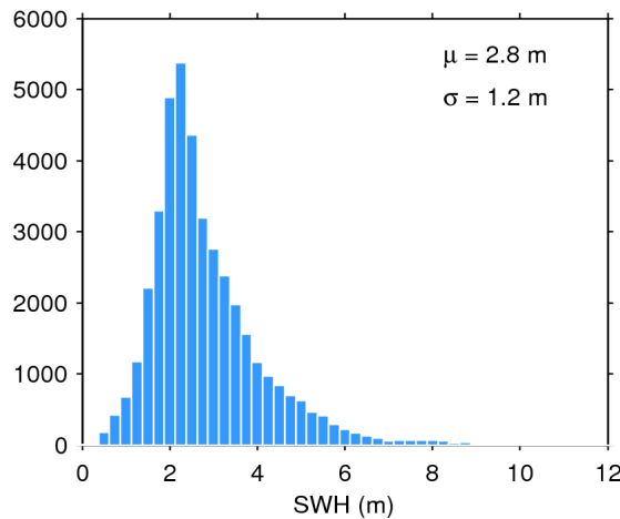
Figure 20. Histogram of science-valid SWH over oceans and lakes for 12/11/2018. The mean ( \mu ) and standard deviation ( \sigma ) are also shown. Note that values larger than 12 m are excluded from the histogram for the sake of readability but not from the computation of \mu and \sigma .
