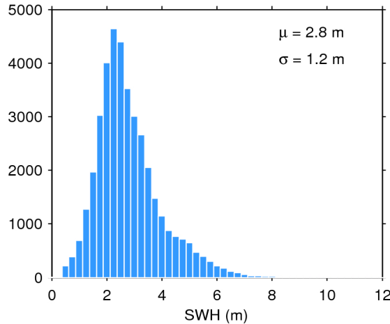
Figure 20. Histogram of science-valid SWH over oceans and lakes for 11/11/2018. The mean ( \mu ) and standard deviation ( \sigma ) are also shown. Note that values larger than 12 m are excluded from the histogram for the sake of readability but not from the computation of \mu and \sigma .
