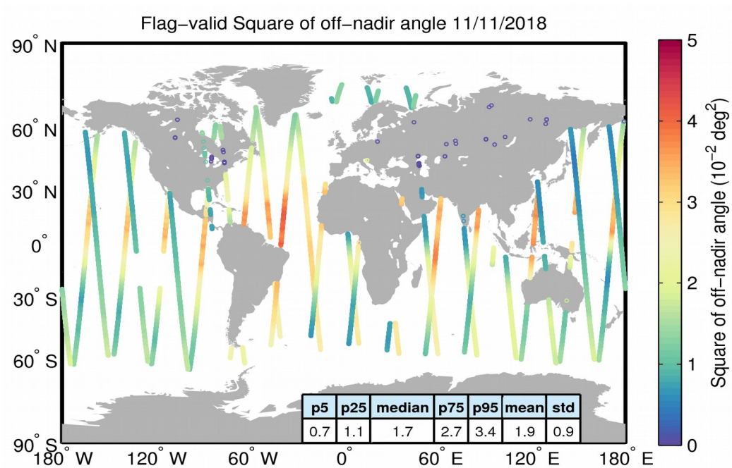
Figure 37. Geographical distribution of flag-valid mispointing data over oceans and lakes for 11/11/2018. The statistical values shown in the table refer to the mispointing in 10^{-2} \text{ deg}^2 and are calculated over all measurements shown in the figure.
