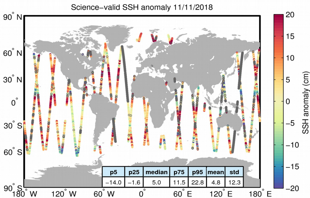
Figure 10. Geographical distribution of science-valid SSH anomaly data over oceans and lakes for 11/11/2018. The statistical values shown in the table refer to the SSH anomaly in cm and are calculated over all measurements shown in the figure. Gray circles denote records that have been rejected based on the editing criteria described in Table 2.
