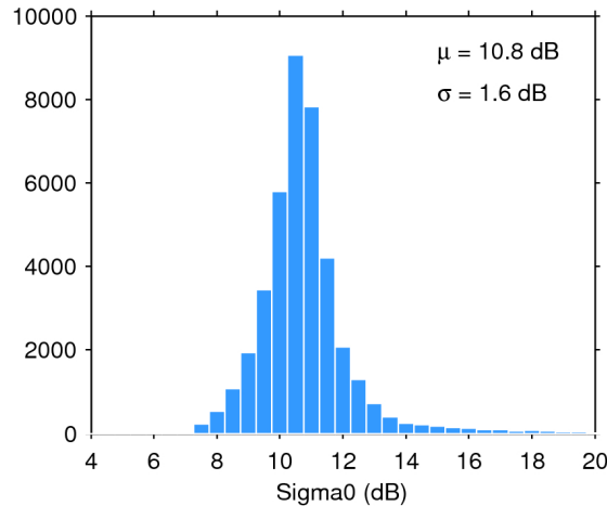
Figure 25. Histogram of flag-valid sigma0 over oceans and lakes for 11/11/2018. The mean ( \mu ) and standard deviation ( \sigma ) are also shown. Note that values outside [4 20] dB are excluded from the histogram for the sake of readability but not from the computation of \mu and \sigma .
