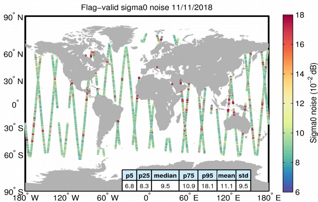
Figure 26. Geographical distribution of flag-valid 20-Hz sigma0 measurement noise over oceans and lakes for 11/11/2018. The statistical values shown in the table refer to the sigma0 noise and are calculated over all measurements shown in the figure.
