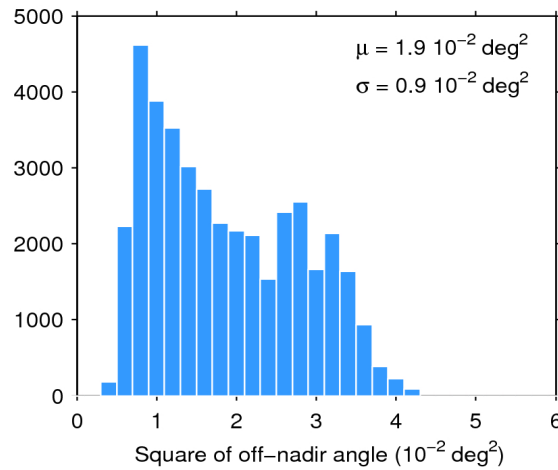
Figure 39. Histogram of flag-valid mispointing over oceans and lakes for 11/11/2018. The mean ( \mu ) and standard deviation ( \sigma ) are also shown. Note that values larger than 6 \cdot 10^{-2} \text{ deg}^2 are excluded from the histogram for the sake of readability but not from the computation of \mu and \sigma .
