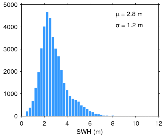
Figure 17. Histogram of flag-valid SWH over oceans and lakes for 11/11/2018. The mean ( \mu ) and standard deviation ( \sigma ) are also shown. Note that values larger than 12 m are excluded from the histogram for the sake of readability but not from the computation of \mu and \sigma .
