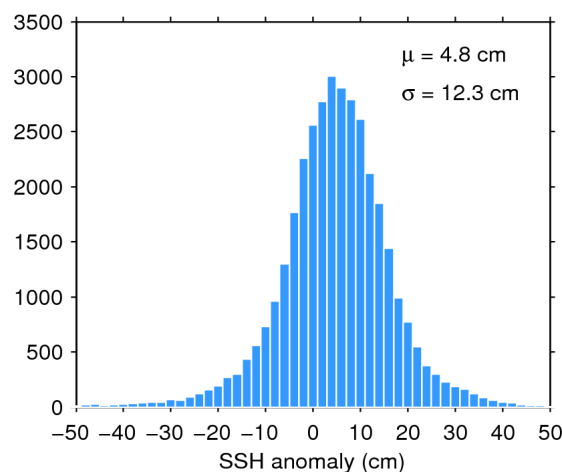
Figure 11. Histogram of science-valid SSH anomaly over oceans and lakes for 11/11/2018. The mean ( \mu ) and standard deviation ( \sigma ) are also shown. Note that values outside [-50 50] cm are excluded from the histogram for the sake of readability but not from the computation of \mu and \sigma .
