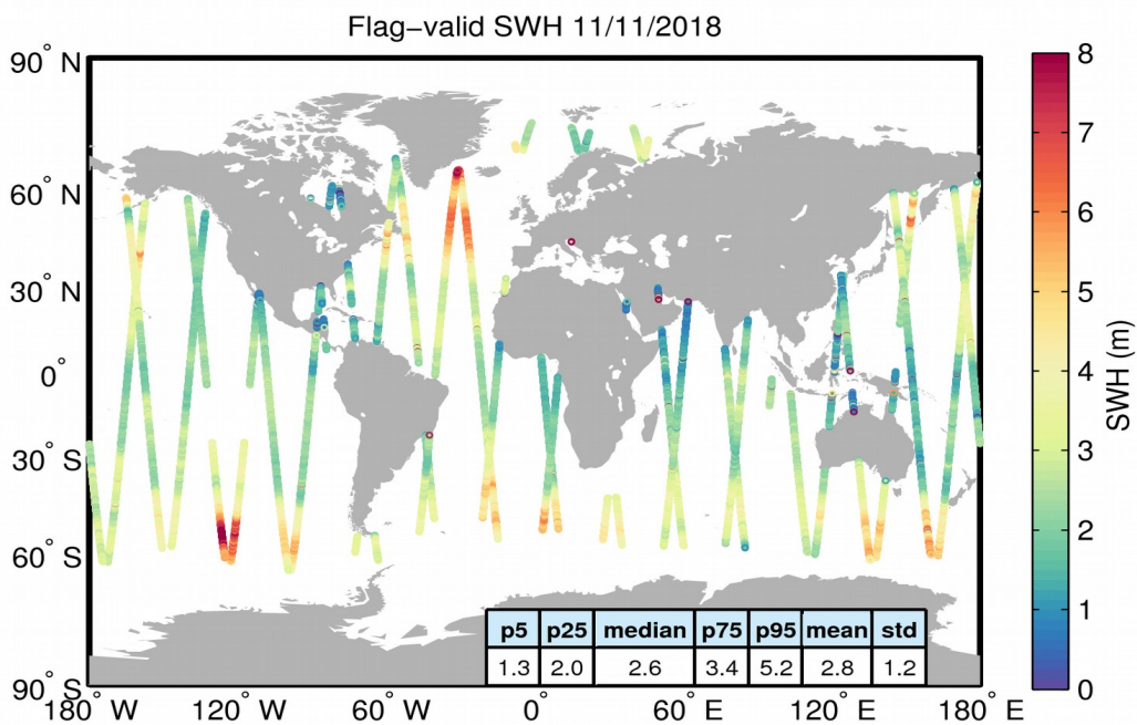
Figure 15. Geographical distribution of flag-valid SWH data over oceans and lakes for 11/11/2018. The statistical values shown in the table refer to the SWH in m and are calculated over all measurements shown in the figure.
