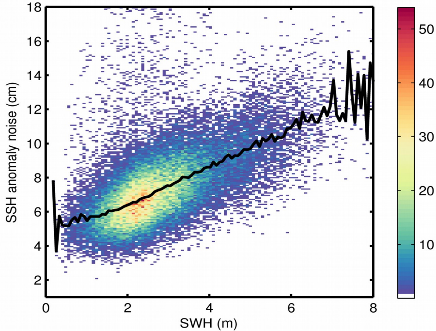
Figure 9. 2D histogram showing flag-valid SSH anomaly noise as a function of SWH for 11/11/2018. The black line denotes the median SSH anomaly noise as a function of SWH.
