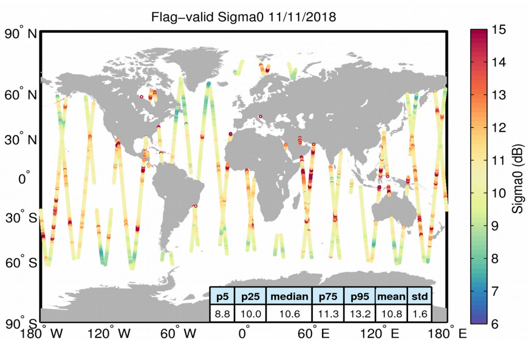
Figure 23. Geographical distribution of flag-valid sigma0 data over oceans and lakes for 11/11/2018. The statistical values shown in the table refer to the sigma0 in dB and are calculated over all measurements shown in the figure.
