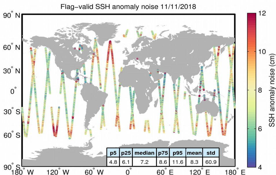
Figure 8. Geographical distribution of flag-valid 20-Hz SSH anomaly measurement noise over oceans and lakes for 11/11/2018. The statistical values shown in the table refer to the SSH anomaly noise and are calculated over all measurements shown in the figure.
