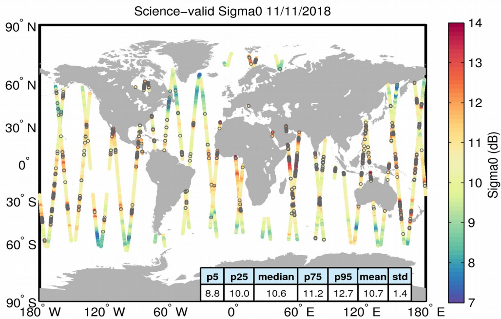
Figure 27. Geographical distribution of science-valid sigma0 data over oceans and lakes for 11/11/2018. The statistical values shown in the table refer to the sigma0 in dB and are calculated over all measurements shown in the figure. Gray circles denote records that have been rejected based on the editing criteria described in Table 4.
