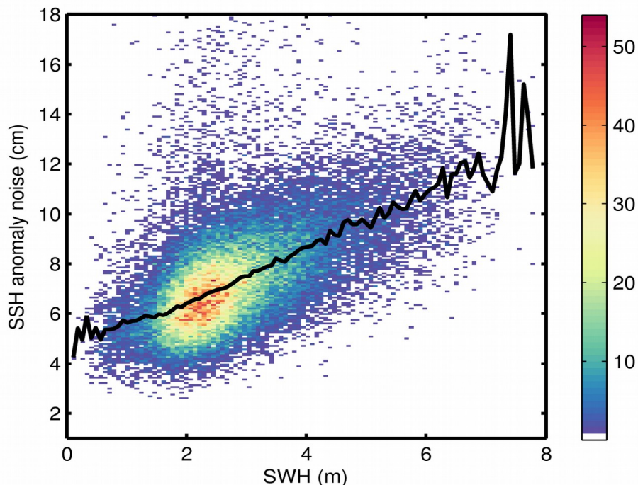
Figure 9. 2D histogram showing flag-valid SSH anomaly noise as a function of SWH for 10/11/2018. The black line denotes the median SSH anomaly noise as a function of SWH.
