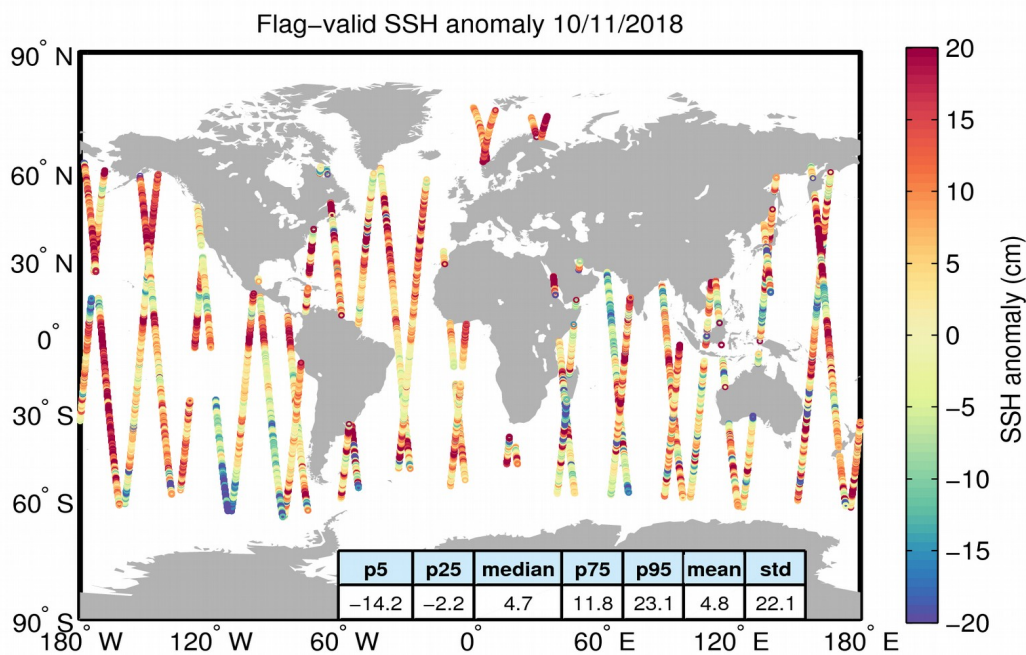
Figure 5. Geographical distribution of flag-valid 1-Hz SSH anomaly data over oceans and lakes for 10/11/2018. The statistical values shown in the table refer to the SSH anomaly in cm and are calculated over all measurements shown in the figure.
