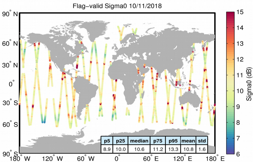
Figure 23. Geographical distribution of flag-valid sigma0 data over oceans and lakes for 10/11/2018. The statistical values shown in the table refer to the sigma0 in dB and are calculated over all measurements shown in the figure.
