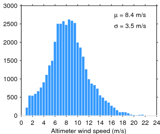
Figure 35. Histogram of science-valid wind over oceans and lakes for 10/11/2018. The mean ( \mu ) and standard deviation ( \sigma ) are also shown. Note that values larger than 24 m/s are excluded from the histogram for the sake of readability but not from the computation of \mu and \sigma .
