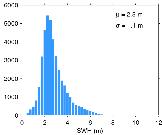
Figure 17. Histogram of flag-valid SWH over oceans and lakes for 10/11/2018. The mean ( \mu ) and standard deviation ( \sigma ) are also shown. Note that values larger than 12 m are excluded from the histogram for the sake of readability but not from the computation of \mu and \sigma .
