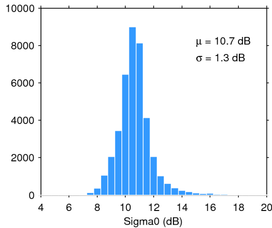
Figure 28. Histogram of science-valid sigma0 over oceans and lakes for 10/11/2018. The mean ( \mu ) and standard deviation ( \sigma ) are also shown. Note that values outside [4 20] dB are excluded from the histogram for the sake of readability but not from the computation of \mu and \sigma .
