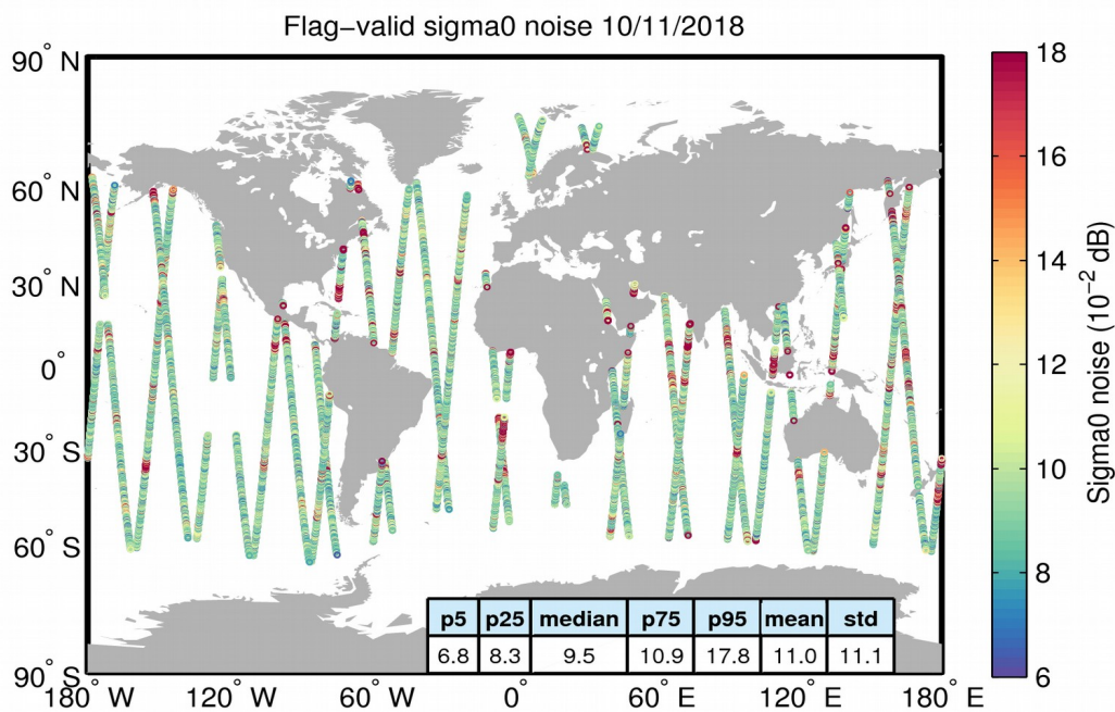
Figure 26. Geographical distribution of flag-valid 20-Hz sigma0 measurement noise over oceans and lakes for 10/11/2018. The statistical values shown in the table refer to the sigma0 noise and are calculated over all measurements shown in the figure.
