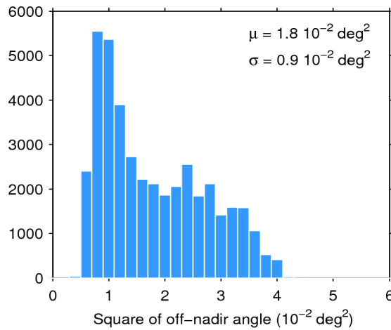
Figure 39. Histogram of flag-valid mispointing over oceans and lakes for 10/11/2018. The mean ( \mu ) and standard deviation ( \sigma ) are also shown. Note that values larger than 6 \cdot 10^{-2} \text{ deg}^2 are excluded from the histogram for the sake of readability but not from the computation of \mu and \sigma .
