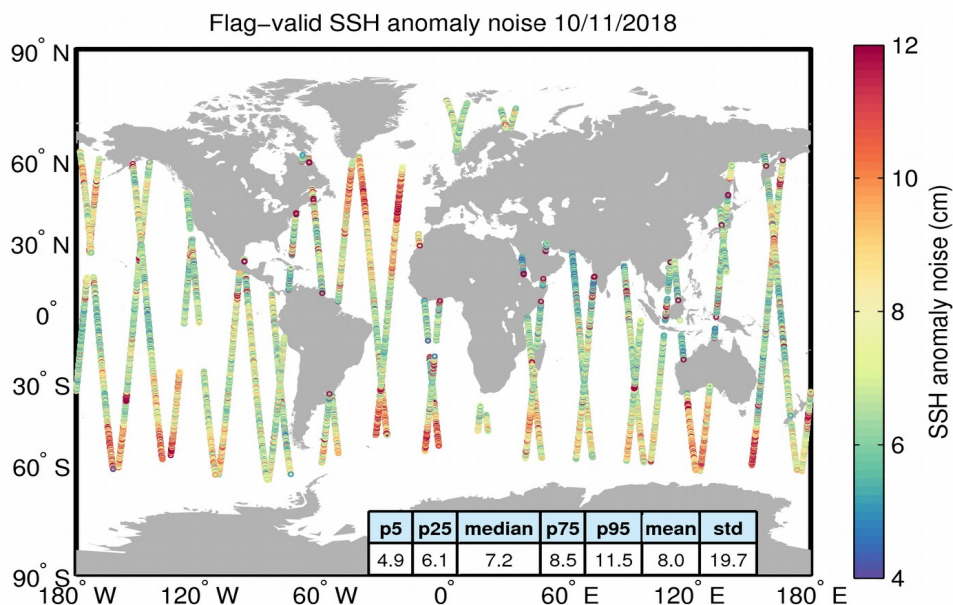
Figure 8. Geographical distribution of flag-valid 20-Hz SSH anomaly measurement noise over oceans and lakes for 10/11/2018. The statistical values shown in the table refer to the SSH anomaly noise and are calculated over all measurements shown in the figure.
