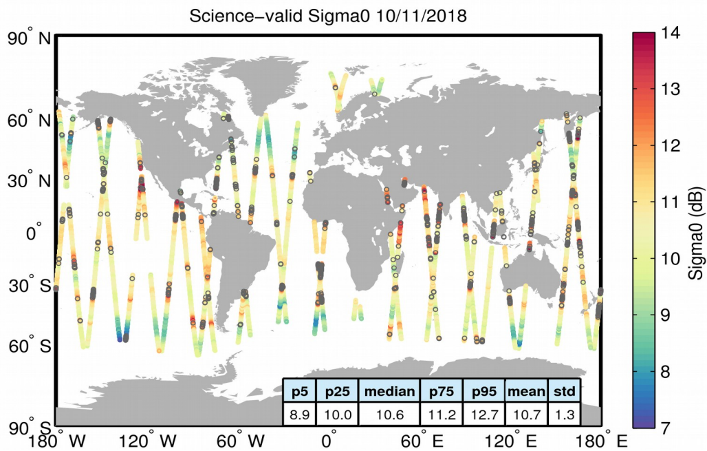
Figure 27. Geographical distribution of science-valid sigma0 data over oceans and lakes for 10/11/2018. The statistical values shown in the table refer to the sigma0 in dB and are calculated over all measurements shown in the figure. Gray circles denote records that have been rejected based on the editing criteria described in Table 4.
