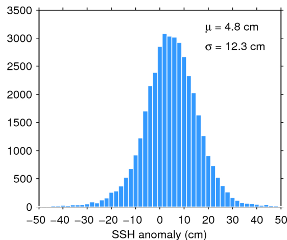
Figure 11. Histogram of science-valid SSH anomaly over oceans and lakes for 10/11/2018. The mean ( \mu ) and standard deviation ( \sigma ) are also shown. Note that values outside [-50 50] cm are excluded from the histogram for the sake of readability but not from the computation of \mu and \sigma .
