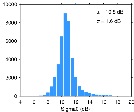
Figure 25. Histogram of flag-valid sigma0 over oceans and lakes for 10/11/2018. The mean ( \mu ) and standard deviation ( \sigma ) are also shown. Note that values outside [4 20] dB are excluded from the histogram for the sake of readability but not from the computation of \mu and \sigma .
