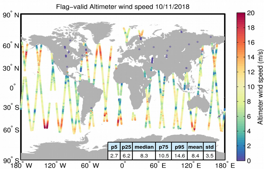
Figure 31. Geographical distribution of flag-valid wind data over oceans and lakes for 10/11/2018. The statistical values shown in the table refer to the wind in m/s and are calculated over all measurements shown in the figure.
