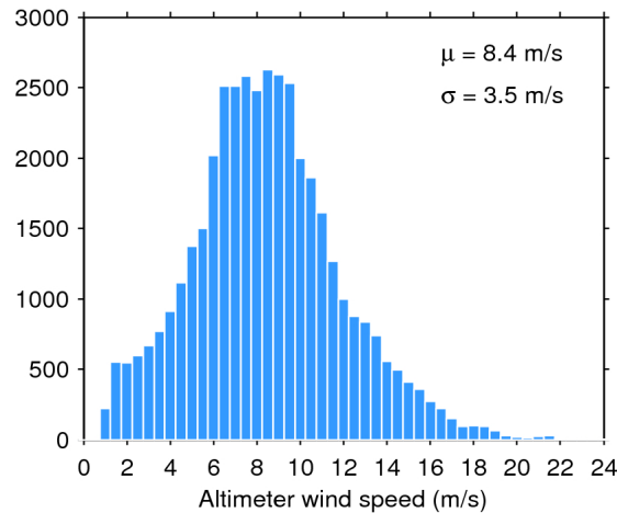
Figure 33. Histogram of flag-valid wind over oceans and lakes for 10/11/2018. The mean ( \mu ) and standard deviation ( \sigma ) are also shown. Note that values larger than 24 m/s are excluded from the histogram for the sake of readability but not from the computation of \mu and \sigma .
