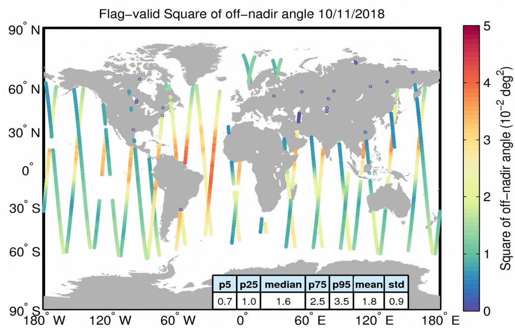
Figure 37. Geographical distribution of flag-valid mispointing data over oceans and lakes for 10/11/2018. The statistical values shown in the table refer to the mispointing in 10^{-2} \text{deg}^2 and are calculated over all measurements shown in the figure.
