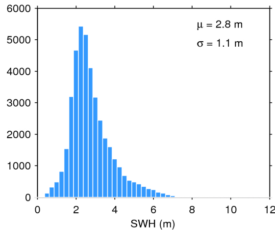
Figure 20. Histogram of science-valid SWH over oceans and lakes for 10/11/2018. The mean ( \mu ) and standard deviation ( \sigma ) are also shown. Note that values larger than 12 m are excluded from the histogram for the sake of readability but not from the computation of \mu and \sigma .
