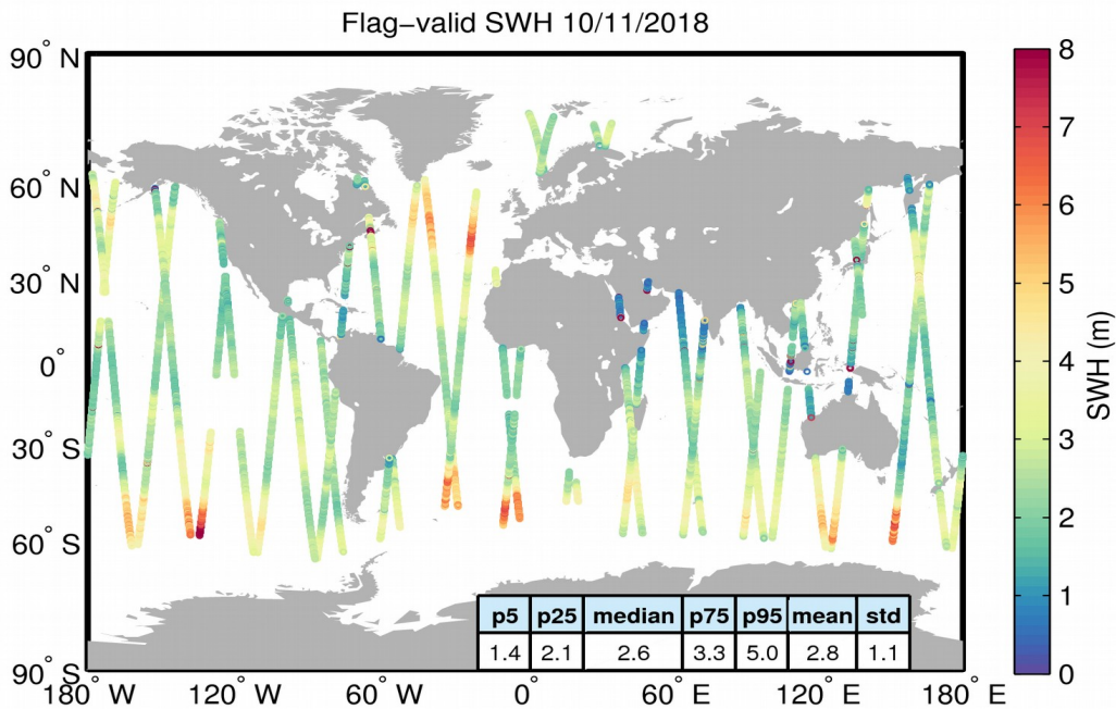
Figure 15. Geographical distribution of flag-valid SWH data over oceans and lakes for 10/11/2018. The statistical values shown in the table refer to the SWH in m and are calculated over all measurements shown in the figure.
