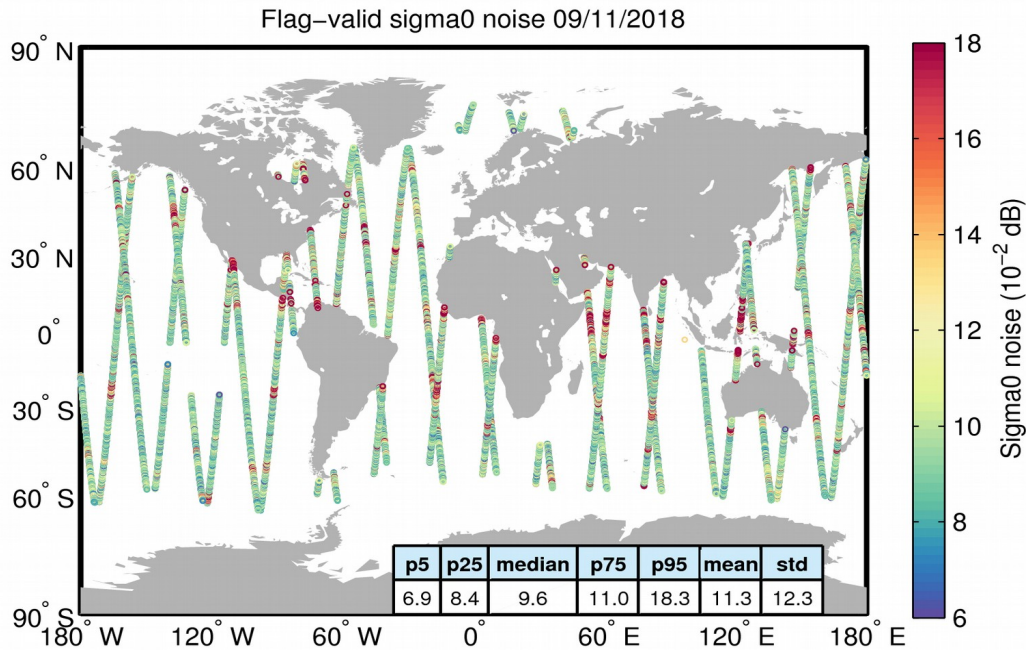
Figure 26. Geographical distribution of flag-valid 20-Hz sigma0 measurement noise over oceans and lakes for 09/11/2018. The statistical values shown in the table refer to the sigma0 noise and are calculated over all measurements shown in the figure.
