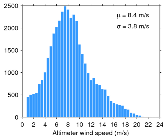
Figure 35. Histogram of science-valid wind over oceans and lakes for 09/11/2018. The mean ( \mu ) and standard deviation ( \sigma ) are also shown. Note that values larger than 24 m/s are excluded from the histogram for the sake of readability but not from the computation of \mu and \sigma .
