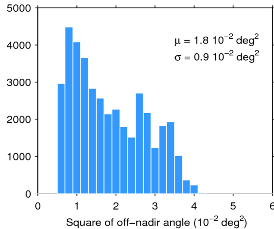
Figure 39. Histogram of flag-valid mispointing over oceans and lakes for 09/11/2018. The mean ( \mu ) and standard deviation ( \sigma ) are also shown. Note that values larger than 6 \cdot 10^{-2} \text{ deg}^2 are excluded from the histogram for the sake of readability but not from the computation of \mu and \sigma .
