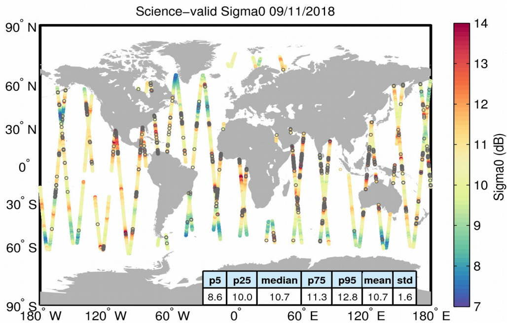
Figure 27. Geographical distribution of science-valid sigma0 data over oceans and lakes for 09/11/2018. The statistical values shown in the table refer to the sigma0 in dB and are calculated over all measurements shown in the figure. Gray circles denote records that have been rejected based on the editing criteria described in Table 4.
