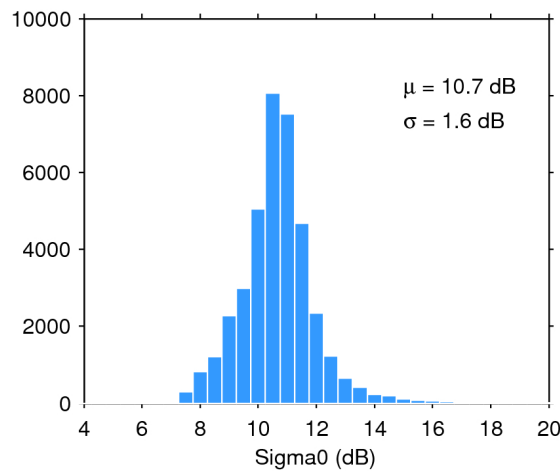
Figure 28. Histogram of science-valid sigma0 over oceans and lakes for 09/11/2018. The mean ( \mu ) and standard deviation ( \sigma ) are also shown. Note that values outside [4 20] dB are excluded from the histogram for the sake of readability but not from the computation of \mu and \sigma .
