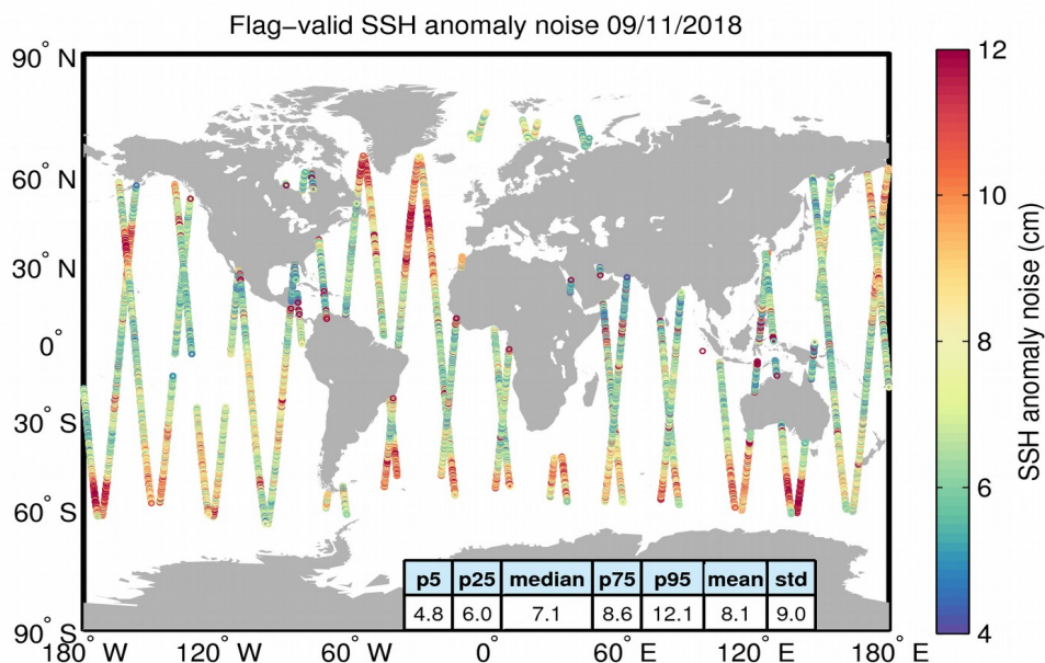
Figure 8. Geographical distribution of flag-valid 20-Hz SSH anomaly measurement noise over oceans and lakes for 09/11/2018. The statistical values shown in the table refer to the SSH anomaly noise and are calculated over all measurements shown in the figure.
