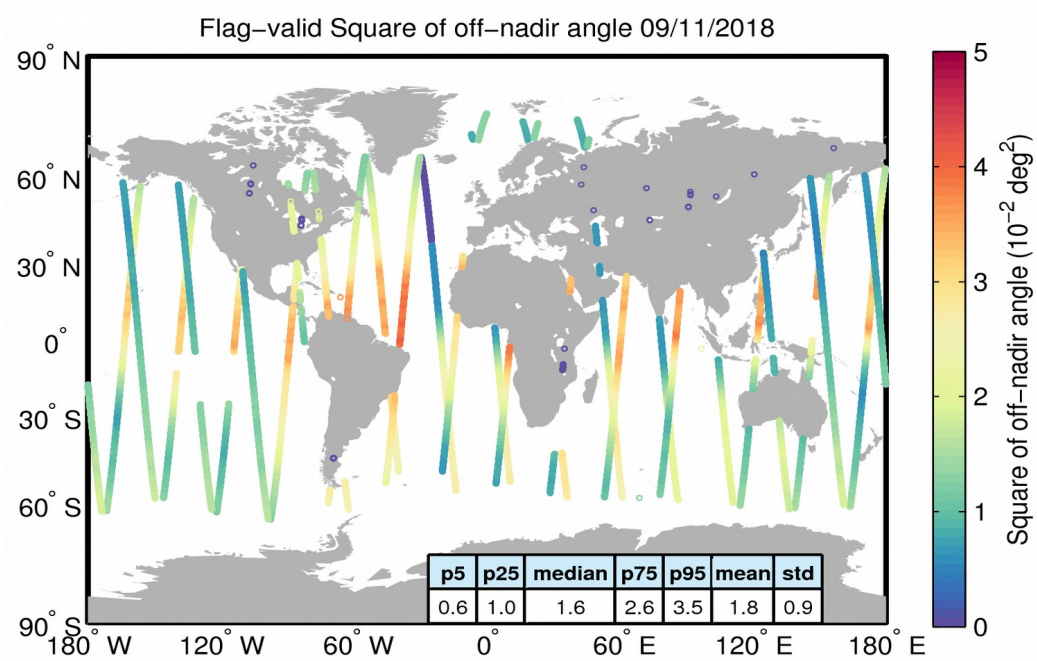
Figure 37. Geographical distribution of flag-valid mispointing data over oceans and lakes for 09/11/2018. The statistical values shown in the table refer to the mispointing in 10^{-2} deg 2 and are calculated over all measurements shown in the figure.
