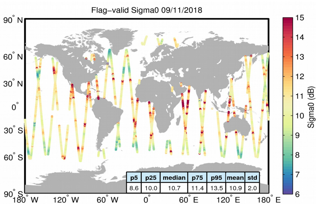
Figure 23. Geographical distribution of flag-valid sigma0 data over oceans and lakes for 09/11/2018. The statistical values shown in the table refer to the sigma0 in dB and are calculated over all measurements shown in the figure.
