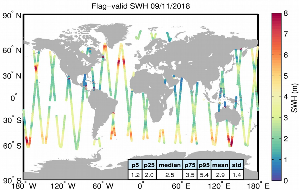
Figure 15. Geographical distribution of flag-valid SWH data over oceans and lakes for 09/11/2018. The statistical values shown in the table refer to the SWH in m and are calculated over all measurements shown in the figure.
