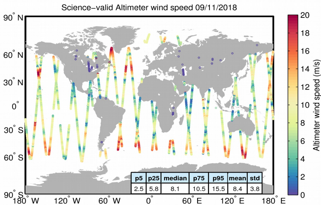
Figure 34. Geographical distribution of science-valid wind data over oceans and lakes for 09/11/2018. The statistical values shown in the table refer to the wind in m/s and are calculated over all measurements shown in the figure. Gray circles denote records that have been rejected based on the editing criteria described in Table 5.
