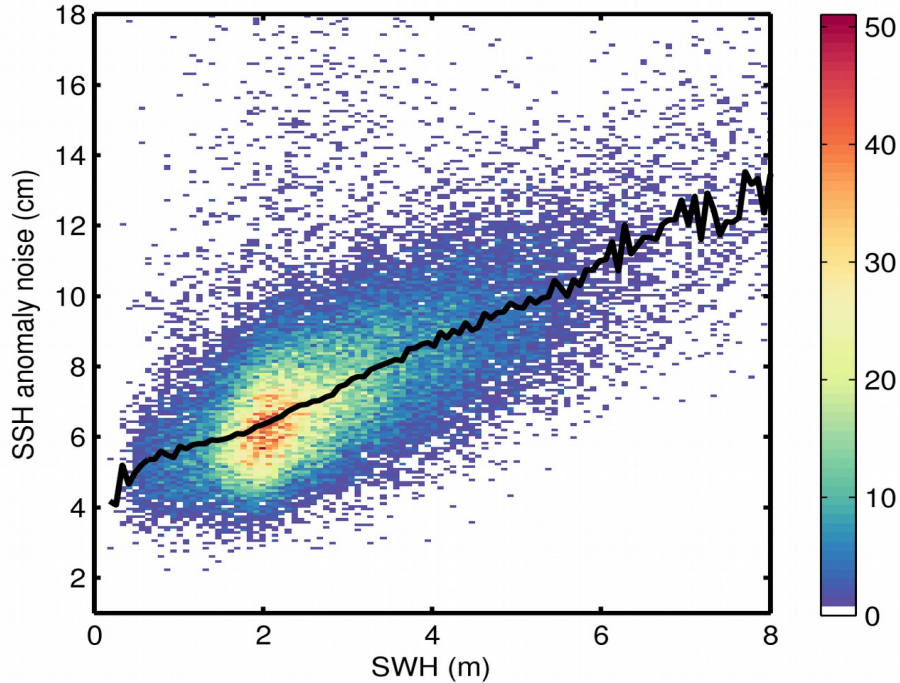
Figure 9. 2D histogram showing flag-valid SSH anomaly noise as a function of SWH for 09/11/2018. The black line denotes the median SSH anomaly noise as a function of SWH.
