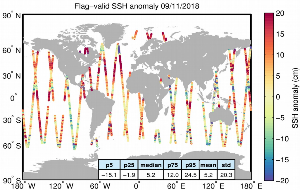
Figure 5. Geographical distribution of flag-valid 1-Hz SSH anomaly data over oceans and lakes for 09/11/2018. The statistical values shown in the table refer to the SSH anomaly in cm and are calculated over all measurements shown in the figure.
