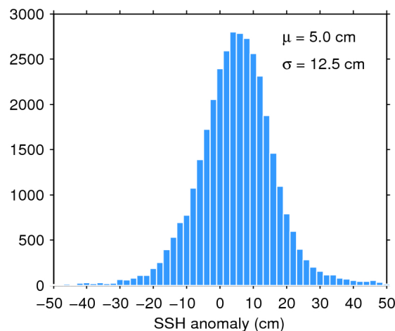
Figure 11. Histogram of science-valid SSH anomaly over oceans and lakes for 09/11/2018. The mean ( \mu ) and standard deviation ( \sigma ) are also shown. Note that values outside [-50 50] cm are excluded from the histogram for the sake of readability but not from the computation of \mu and \sigma .
