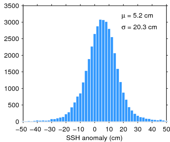
Figure 7. Histogram of flag-valid SSH anomaly over oceans and lakes for 09/11/2018. The mean ( \mu ) and standard deviation ( \sigma ) are also shown. Note that values outside [-50 50] cm are excluded from the histogram for the sake of readability but not from the computation of \mu and \sigma .
