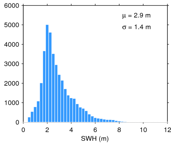
Figure 17. Histogram of flag-valid SWH over oceans and lakes for 09/11/2018. The mean ( \mu ) and standard deviation ( \sigma ) are also shown. Note that values larger than 12 m are excluded from the histogram for the sake of readability but not from the computation of \mu and \sigma .
