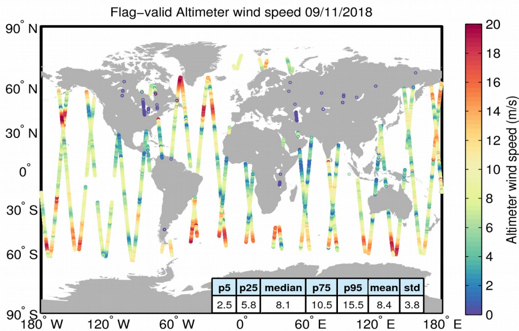
Figure 31. Geographical distribution of flag-valid wind data over oceans and lakes for 09/11/2018. The statistical values shown in the table refer to the wind in m/s and are calculated over all measurements shown in the figure.
