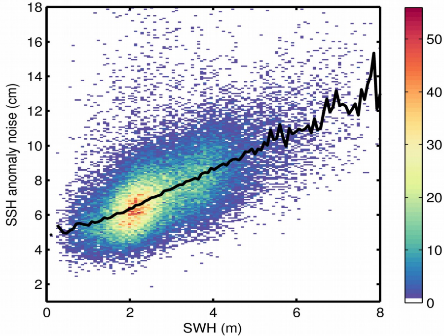
Figure 9. 2D histogram showing flag-valid SSH anomaly noise as a function of SWH for 08/11/2018. The black line denotes the median SSH anomaly noise as a function of SWH.
