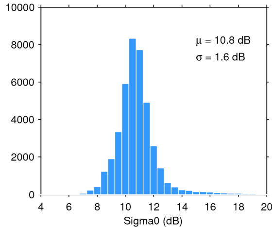
Figure 25. Histogram of flag-valid sigma0 over oceans and lakes for 08/11/2018. The mean ( \mu ) and standard deviation ( \sigma ) are also shown. Note that values outside [4 20] dB are excluded from the histogram for the sake of readability but not from the computation of \mu and \sigma .
