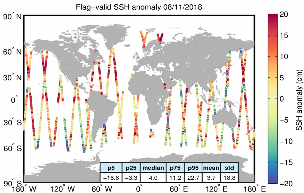
Figure 5. Geographical distribution of flag-valid 1-Hz SSH anomaly data over oceans and lakes for 08/11/2018. The statistical values shown in the table refer to the SSH anomaly in cm and are calculated over all measurements shown in the figure.
