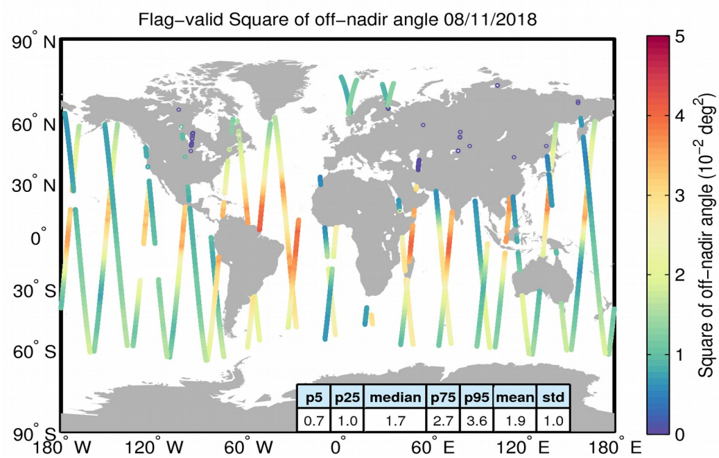
Figure 37. Geographical distribution of flag-valid mispointing data over oceans and lakes for 08/11/2018. The statistical values shown in the table refer to the mispointing in 10^{-2} \text{deg}^2 and are calculated over all measurements shown in the figure.
