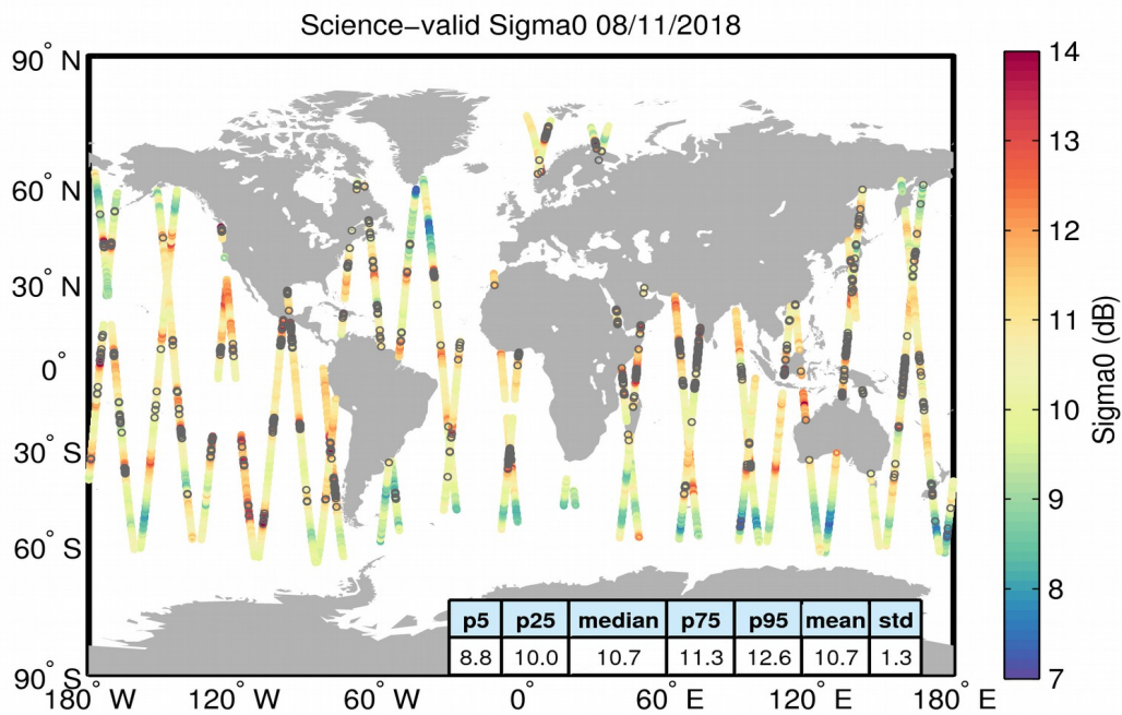
Figure 27. Geographical distribution of science-valid sigma0 data over oceans and lakes for 08/11/2018. The statistical values shown in the table refer to the sigma0 in dB and are calculated over all measurements shown in the figure. Gray circles denote records that have been rejected based on the editing criteria described in Table 4.
