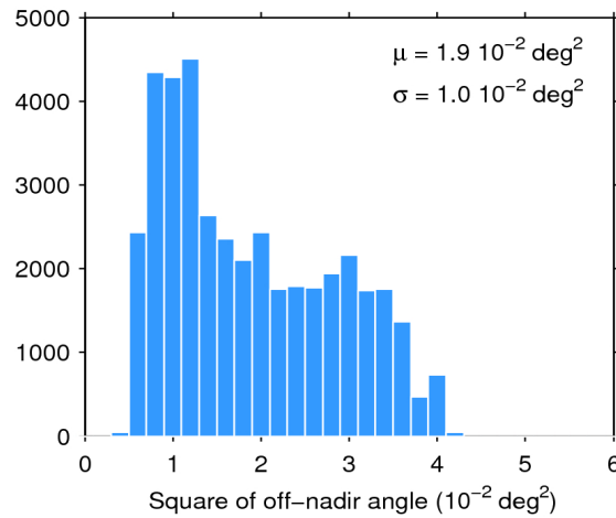
Figure 39. Histogram of flag-valid mispointing over oceans and lakes for 08/11/2018. The mean ( \mu ) and standard deviation ( \sigma ) are also shown. Note that values larger than 6 \cdot 10^{-2} \text{ deg}^2 are excluded from the histogram for the sake of readability but not from the computation of \mu and \sigma .
