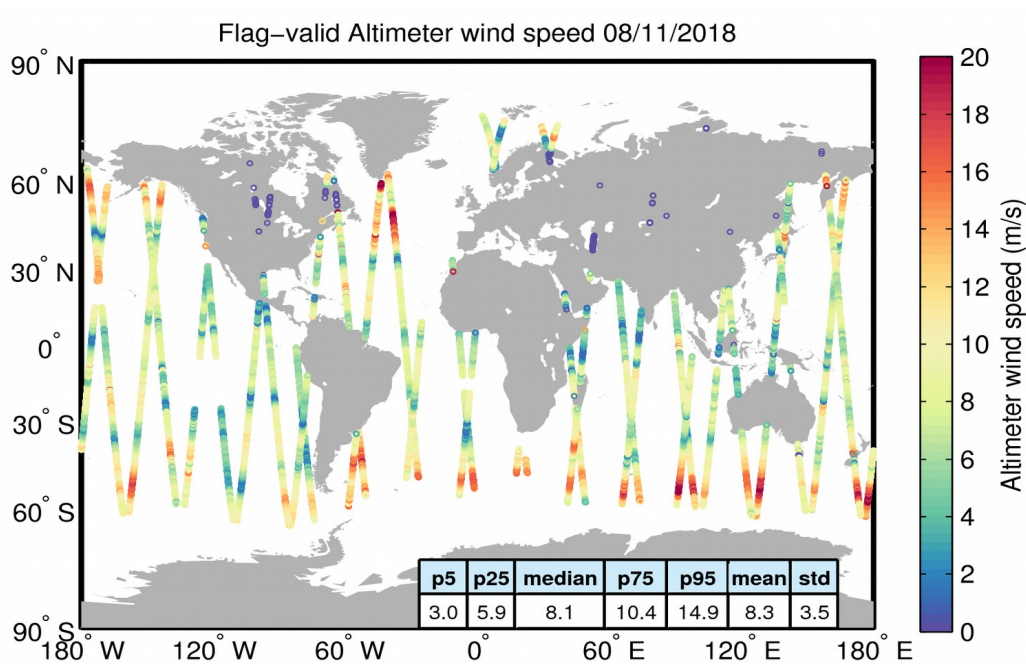
Figure 31. Geographical distribution of flag-valid wind data over oceans and lakes for 08/11/2018. The statistical values shown in the table refer to the wind in m/s and are calculated over all measurements shown in the figure.
