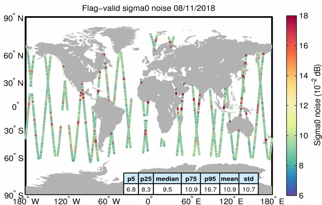
Figure 26. Geographical distribution of flag-valid 20-Hz sigma0 measurement noise over oceans and lakes for 08/11/2018. The statistical values shown in the table refer to the sigma0 noise and are calculated over all measurements shown in the figure.
