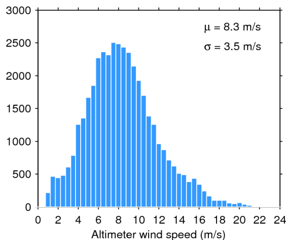
Figure 35. Histogram of science-valid wind over oceans and lakes for 08/11/2018. The mean ( \mu ) and standard deviation ( \sigma ) are also shown. Note that values larger than 24 m/s are excluded from the histogram for the sake of readability but not from the computation of \mu and \sigma .
