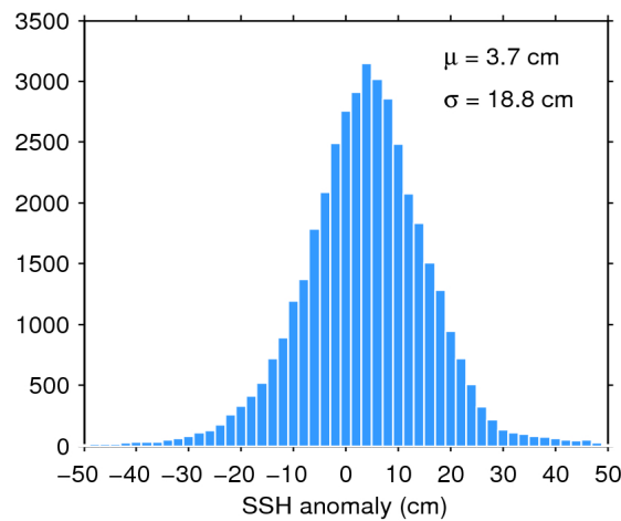
Figure 7. Histogram of flag-valid SSH anomaly over oceans and lakes for 08/11/2018. The mean ( \mu ) and standard deviation ( \sigma ) are also shown. Note that values outside [-50 50] cm are excluded from the histogram for the sake of readability but not from the computation of \mu and \sigma .
