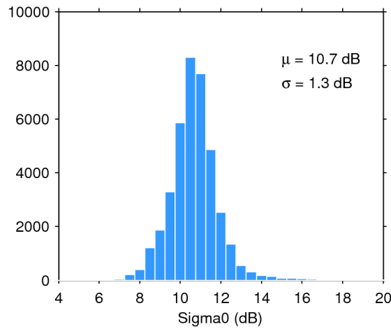
Figure 28. Histogram of science-valid sigma0 over oceans and lakes for 08/11/2018. The mean ( \mu ) and standard deviation ( \sigma ) are also shown. Note that values outside [4 20] dB are excluded from the histogram for the sake of readability but not from the computation of \mu and \sigma .
