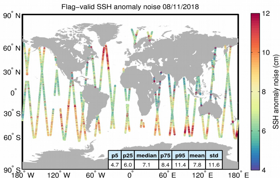
Figure 8. Geographical distribution of flag-valid 20-Hz SSH anomaly measurement noise over oceans and lakes for 08/11/2018. The statistical values shown in the table refer to the SSH anomaly noise and are calculated over all measurements shown in the figure.
