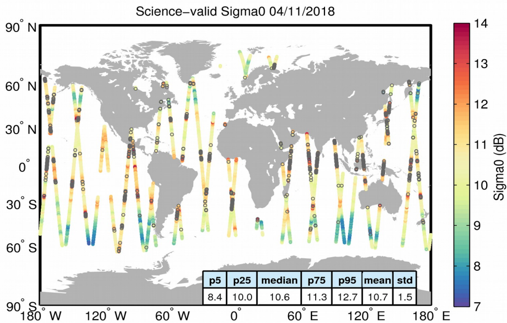
Figure 27. Geographical distribution of science-valid sigma0 data over oceans and lakes for 04/11/2018. The statistical values shown in the table refer to the sigma0 in dB and are calculated over all measurements shown in the figure. Gray circles denote records that have been rejected based on the editing criteria described in Table 4.
