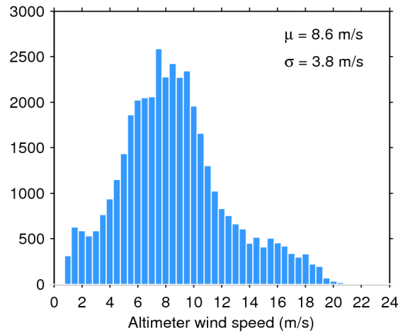
Figure 33. Histogram of flag-valid wind over oceans and lakes for 04/11/2018. The mean ( \mu ) and standard deviation ( \sigma ) are also shown. Note that values larger than 24 m/s are excluded from the histogram for the sake of readability but not from the computation of \mu and \sigma .
