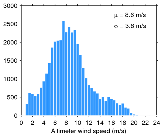
Figure 35. Histogram of science-valid wind over oceans and lakes for 04/11/2018. The mean ( \mu ) and standard deviation ( \sigma ) are also shown. Note that values larger than 24 m/s are excluded from the histogram for the sake of readability but not from the computation of \mu and \sigma .
