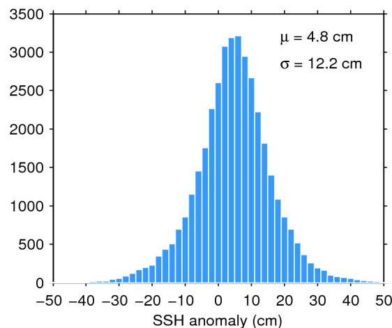
Figure 11. Histogram of science-valid SSH anomaly over oceans and lakes for 04/11/2018. The mean ( \mu ) and standard deviation ( \sigma ) are also shown. Note that values outside [-50 50] cm are excluded from the histogram for the sake of readability but not from the computation of \mu and \sigma .
