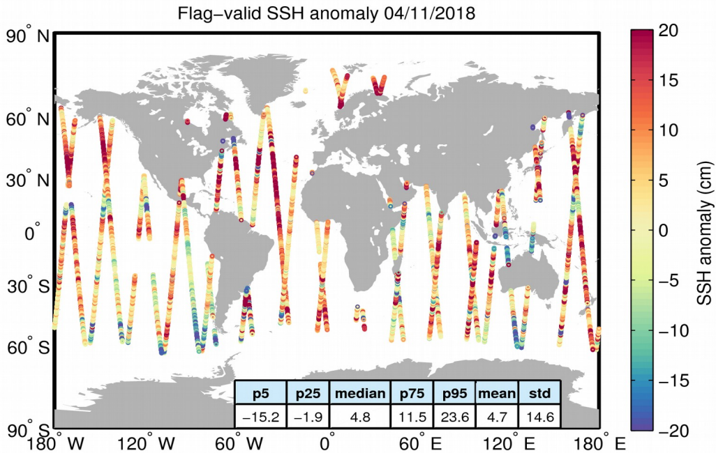
Figure 5. Geographical distribution of flag-valid 1-Hz SSH anomaly data over oceans and lakes for 04/11/2018. The statistical values shown in the table refer to the SSH anomaly in cm and are calculated over all measurements shown in the figure.
