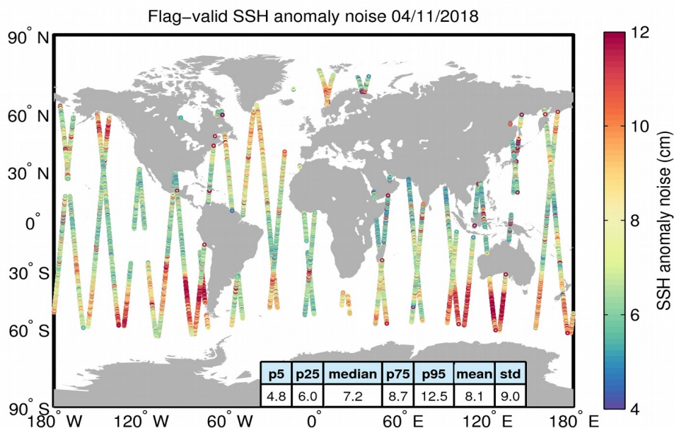
Figure 8. Geographical distribution of flag-valid 20-Hz SSH anomaly measurement noise over oceans and lakes for 04/11/2018. The statistical values shown in the table refer to the SSH anomaly noise and are calculated over all measurements shown in the figure.
