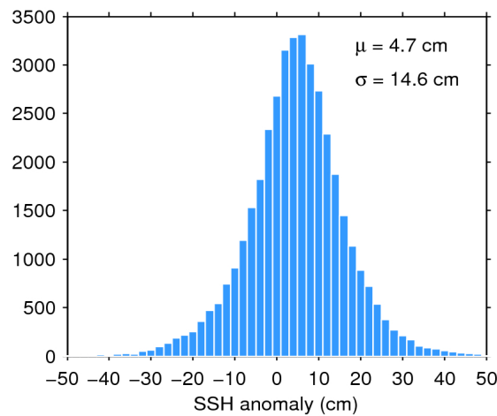
Figure 7. Histogram of flag-valid SSH anomaly over oceans and lakes for 04/11/2018. The mean ( \mu ) and standard deviation ( \sigma ) are also shown. Note that values outside [-50\ 50] cm are excluded from the histogram for the sake of readability but not from the computation of \mu and \sigma .
