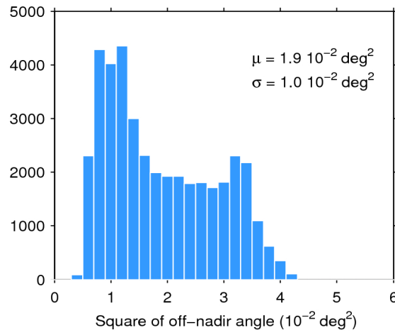
Figure 39. Histogram of flag-valid mispointing over oceans and lakes for 04/11/2018. The mean ( \mu ) and standard deviation ( \sigma ) are also shown. Note that values larger than 6 \cdot 10^{-2} \text{ deg}^2 are excluded from the histogram for the sake of readability but not from the computation of \mu and \sigma .
