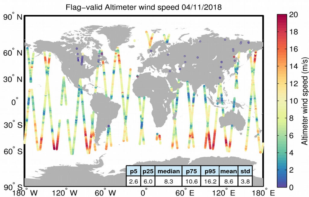
Figure 31. Geographical distribution of flag-valid wind data over oceans and lakes for 04/11/2018. The statistical values shown in the table refer to the wind in m/s and are calculated over all measurements shown in the figure.
