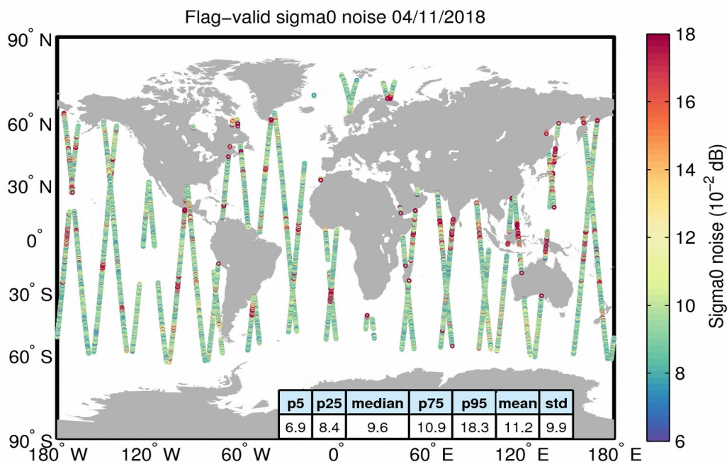
Figure 26. Geographical distribution of flag-valid 20-Hz sigma0 measurement noise over oceans and lakes for 04/11/2018. The statistical values shown in the table refer to the sigma0 noise and are calculated over all measurements shown in the figure.
