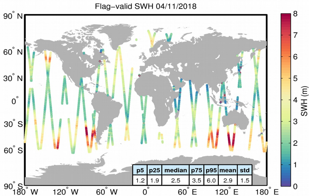
Figure 15. Geographical distribution of flag-valid SWH data over oceans and lakes for 04/11/2018. The statistical values shown in the table refer to the SWH in m and are calculated over all measurements shown in the figure.
