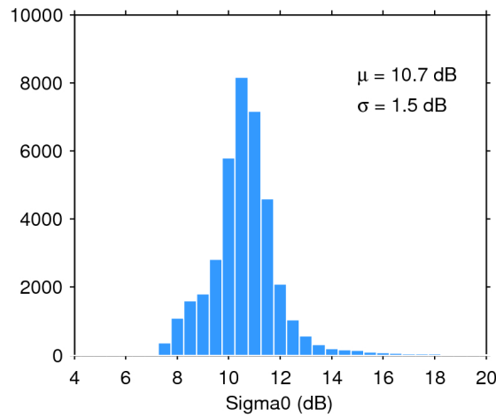
Figure 28. Histogram of science-valid sigma0 over oceans and lakes for 04/11/2018. The mean ( \mu ) and standard deviation ( \sigma ) are also shown. Note that values outside [4 20] dB are excluded from the histogram for the sake of readability but not from the computation of \mu and \sigma .
