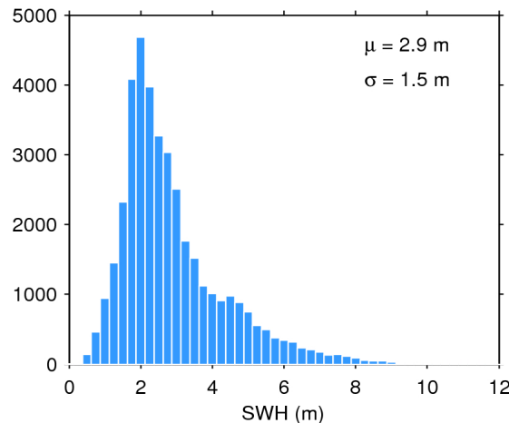
Figure 20. Histogram of science-valid SWH over oceans and lakes for 04/11/2018. The mean ( \mu ) and standard deviation ( \sigma ) are also shown. Note that values larger than 12 m are excluded from the histogram for the sake of readability but not from the computation of \mu and \sigma .
