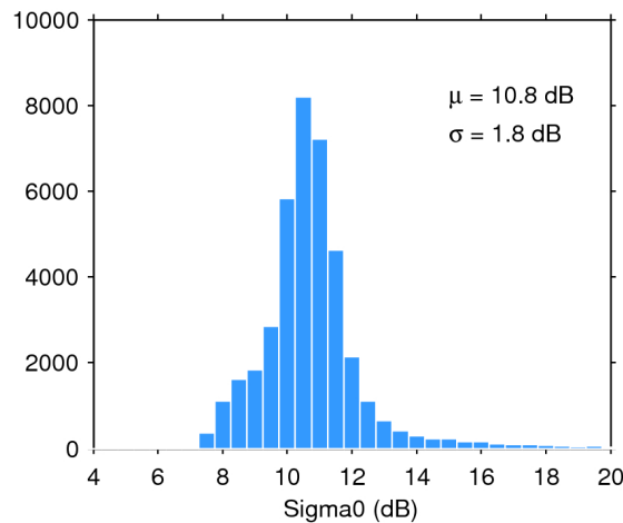
Figure 25. Histogram of flag-valid sigma0 over oceans and lakes for 04/11/2018. The mean ( \mu ) and standard deviation ( \sigma ) are also shown. Note that values outside [4 20] dB are excluded from the histogram for the sake of readability but not from the computation of \mu and \sigma .
