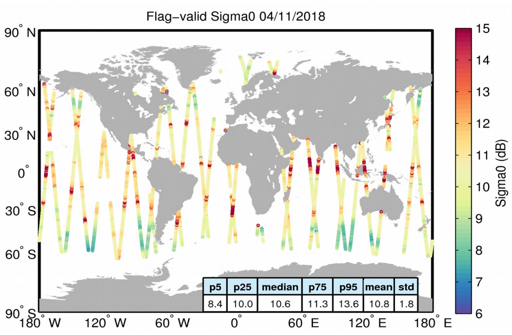
Figure 23. Geographical distribution of flag-valid sigma0 data over oceans and lakes for 04/11/2018. The statistical values shown in the table refer to the sigma0 in dB and are calculated over all measurements shown in the figure.
