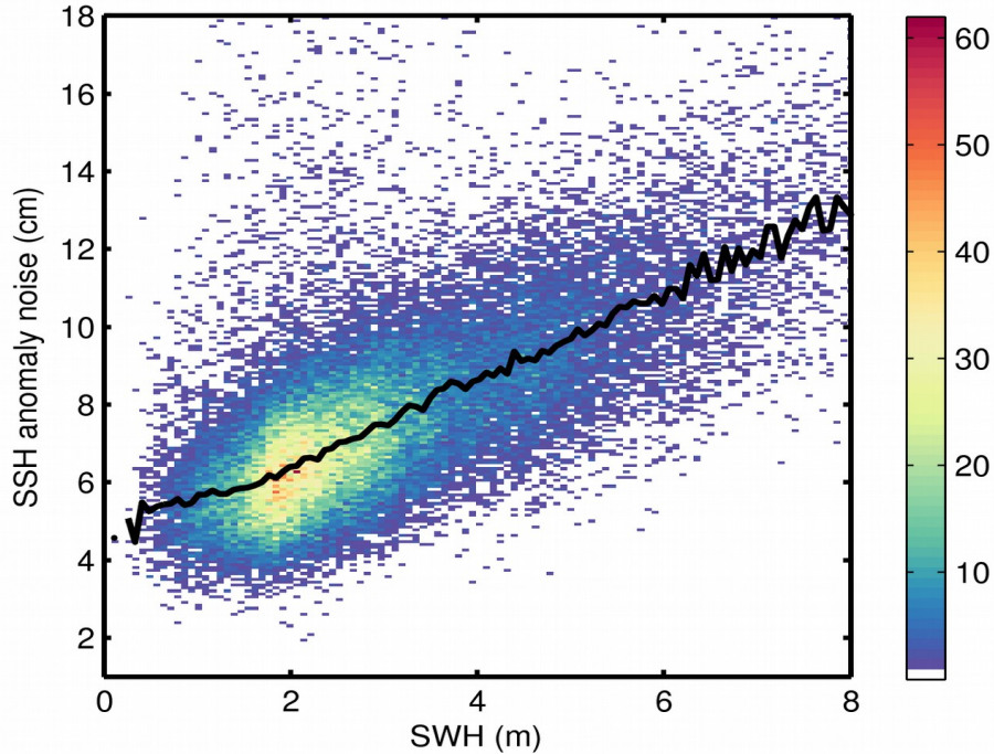
Figure 9. 2D histogram showing flag-valid SSH anomaly noise as a function of SWH for 04/11/2018. The black line denotes the median SSH anomaly noise as a function of SWH.
