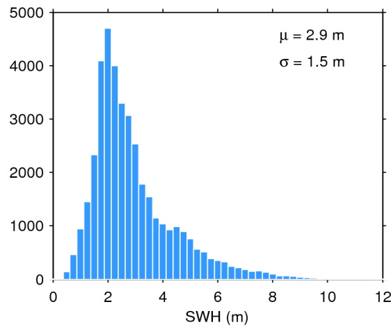
Figure 17. Histogram of flag-valid SWH over oceans and lakes for 04/11/2018. The mean ( \mu ) and standard deviation ( \sigma ) are also shown. Note that values larger than 12 m are excluded from the histogram for the sake of readability but not from the computation of \mu and \sigma .
