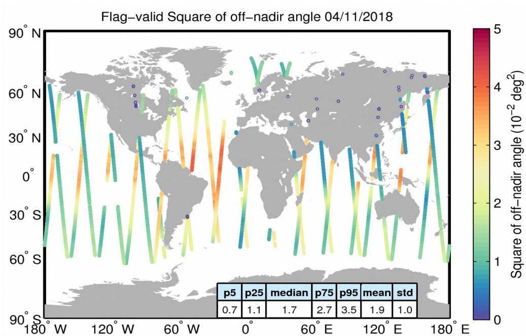
Figure 37. Geographical distribution of flag-valid mispointing data over oceans and lakes for 04/11/2018. The statistical values shown in the table refer to the mispointing in 10^{-2} \text{ deg}^2 and are calculated over all measurements shown in the figure.
