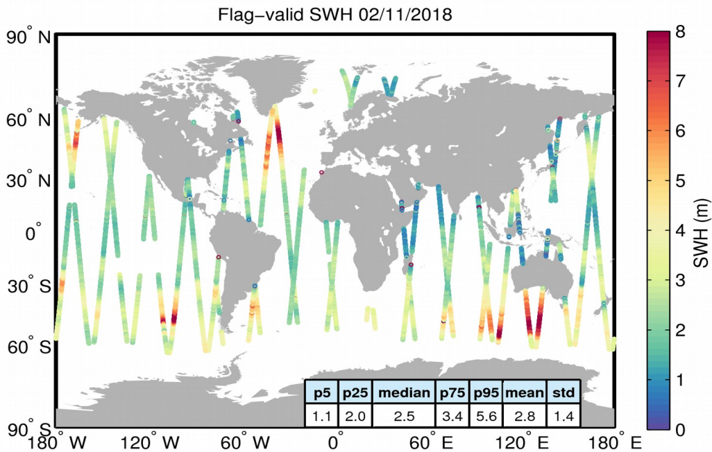
Figure 15. Geographical distribution of flag-valid SWH data over oceans and lakes for 02/11/2018. The statistical values shown in the table refer to the SWH in m and are calculated over all measurements shown in the figure.
