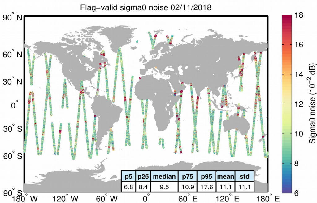
Figure 26. Geographical distribution of flag-valid 20-Hz sigma0 measurement noise over oceans and lakes for 02/11/2018. The statistical values shown in the table refer to the sigma0 noise and are calculated over all measurements shown in the figure.
