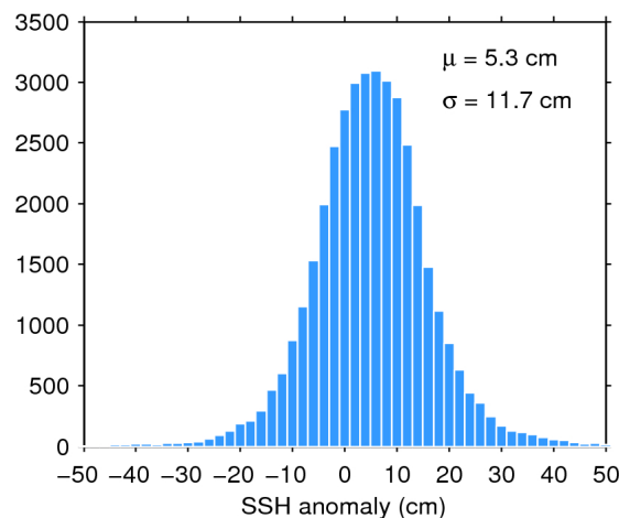
Figure 11. Histogram of science-valid SSH anomaly over oceans and lakes for 02/11/2018. The mean ( \mu ) and standard deviation ( \sigma ) are also shown. Note that values outside [-50 50] cm are excluded from the histogram for the sake of readability but not from the computation of \mu and \sigma .
