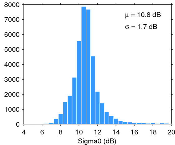
Figure 25. Histogram of flag-valid sigma0 over oceans and lakes for 02/11/2018. The mean ( \mu ) and standard deviation ( \sigma ) are also shown. Note that values outside [4 20] dB are excluded from the histogram for the sake of readability but not from the computation of \mu and \sigma .
