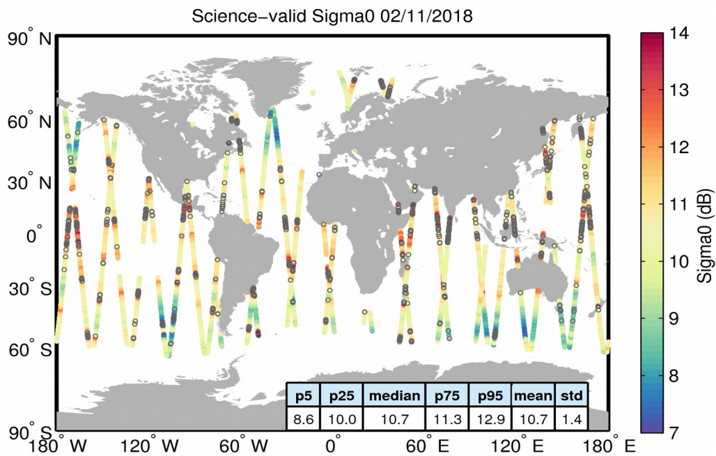
Figure 27. Geographical distribution of science-valid sigma0 data over oceans and lakes for 02/11/2018. The statistical values shown in the table refer to the sigma0 in dB and are calculated over all measurements shown in the figure. Gray circles denote records that have been rejected based on the editing criteria described in Table 4.
