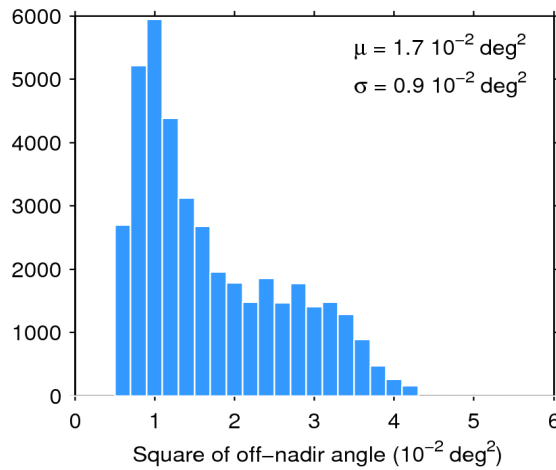
Figure 39. Histogram of flag-valid mispointing over oceans and lakes for 02/11/2018. The mean ( \mu ) and standard deviation ( \sigma ) are also shown. Note that values larger than 6 \cdot 10^{-2} \text{ deg}^2 are excluded from the histogram for the sake of readability but not from the computation of \mu and \sigma .
