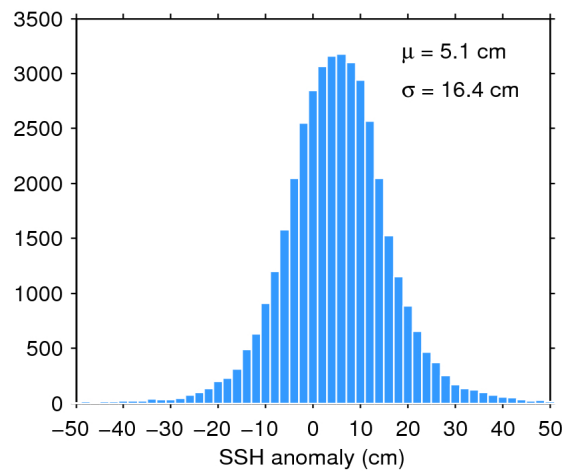
Figure 7. Histogram of flag-valid SSH anomaly over oceans and lakes for 02/11/2018. The mean ( \mu ) and standard deviation ( \sigma ) are also shown. Note that values outside [-50\ 50] cm are excluded from the histogram for the sake of readability but not from the computation of \mu and \sigma .
