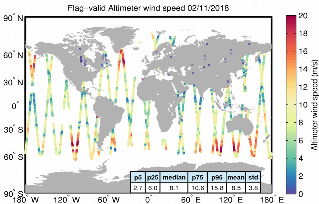
Figure 31. Geographical distribution of flag-valid wind data over oceans and lakes for 02/11/2018. The statistical values shown in the table refer to the wind in m/s and are calculated over all measurements shown in the figure.
