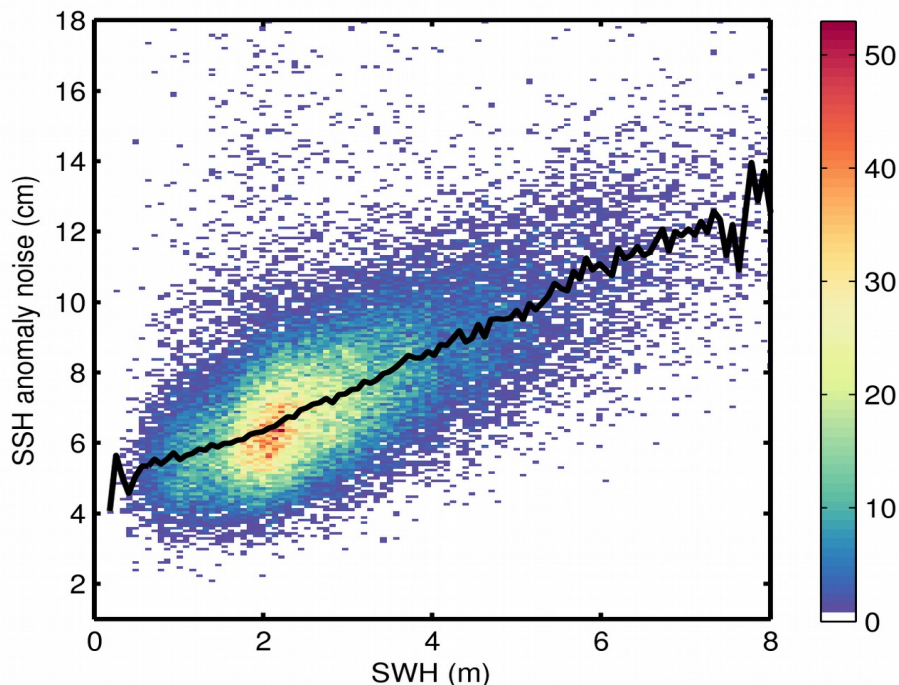
Figure 9. 2D histogram showing flag-valid SSH anomaly noise as a function of SWH for 02/11/2018. The black line denotes the median SSH anomaly noise as a function of SWH.
