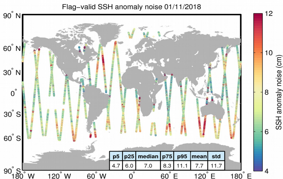
Figure 8. Geographical distribution of flag-valid 20-Hz SSH anomaly measurement noise over oceans and lakes for 01/11/2018. The statistical values shown in the table refer to the SSH anomaly noise and are calculated over all measurements shown in the figure.
