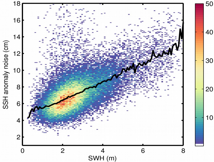
Figure 9. 2D histogram showing flag-valid SSH anomaly noise as a function of SWH for 01/11/2018. The black line denotes the median SSH anomaly noise as a function of SWH.
