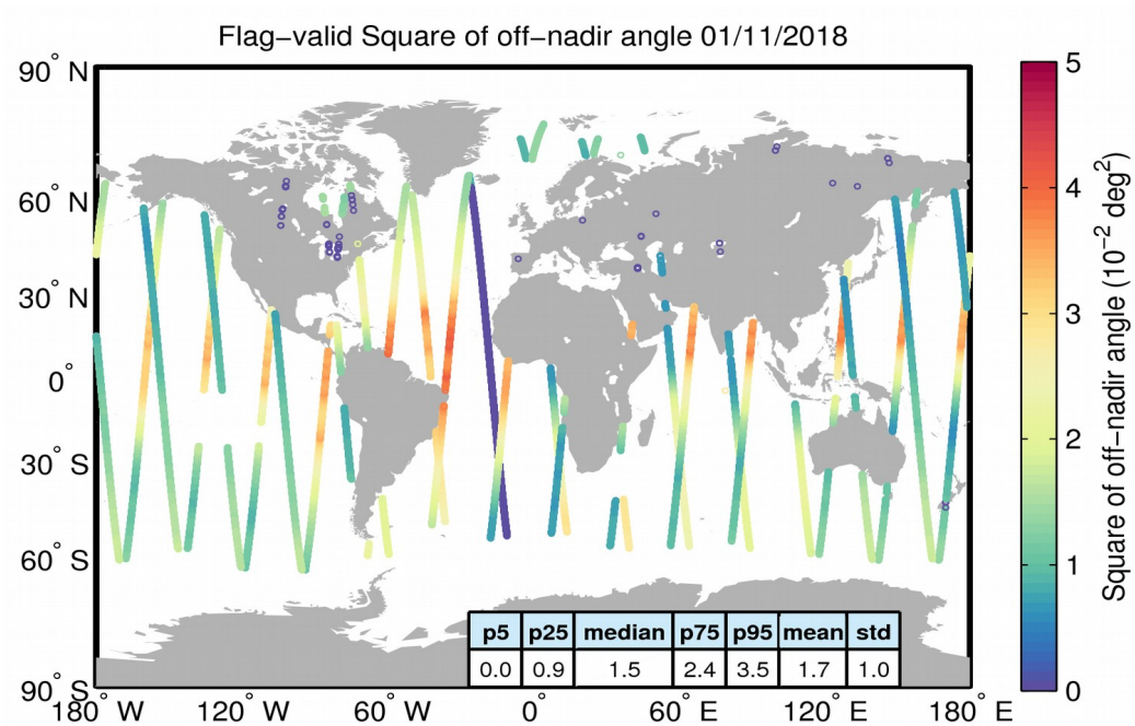
Figure 37. Geographical distribution of flag-valid mispointing data over oceans and lakes for 01/11/2018. The statistical values shown in the table refer to the mispointing in 10^{-2} \text{deg}^2 and are calculated over all measurements shown in the figure.
