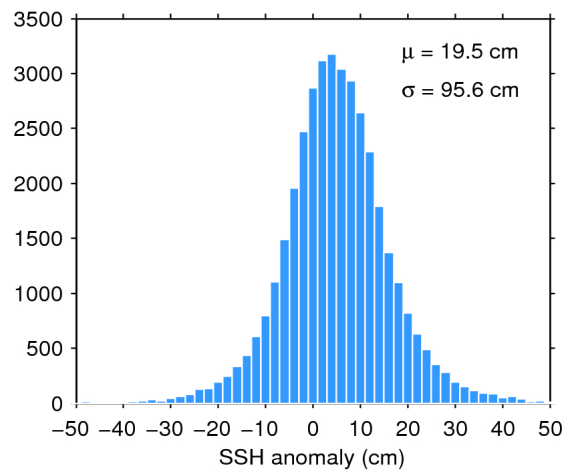
Figure 7. Histogram of flag-valid SSH anomaly over oceans and lakes for 01/11/2018. The mean ( \mu ) and standard deviation ( \sigma ) are also shown. Note that values outside [-50\ 50] cm are excluded from the histogram for the sake of readability but not from the computation of \mu and \sigma .
