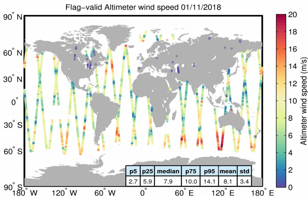
Figure 31. Geographical distribution of flag-valid wind data over oceans and lakes for 01/11/2018. The statistical values shown in the table refer to the wind in m/s and are calculated over all measurements shown in the figure.
