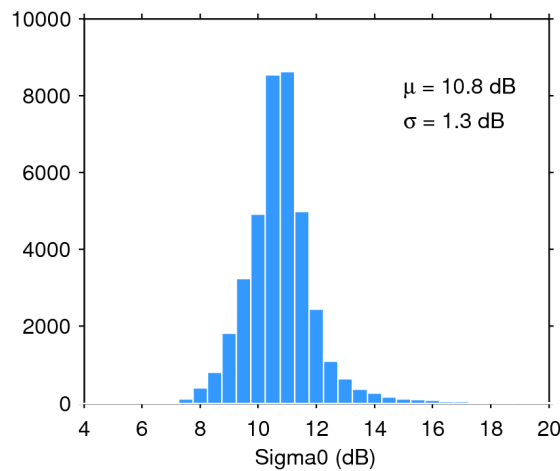
Figure 28. Histogram of science-valid sigma0 over oceans and lakes for 01/11/2018. The mean ( \mu ) and standard deviation ( \sigma ) are also shown. Note that values outside [4 20] dB are excluded from the histogram for the sake of readability but not from the computation of \mu and \sigma .
