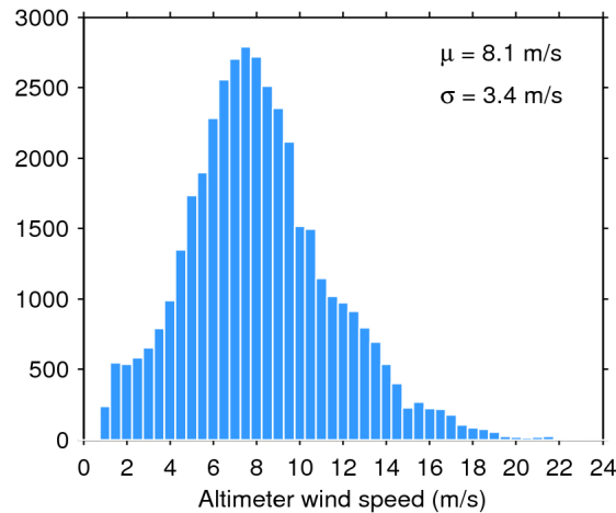
Figure 33. Histogram of flag-valid wind over oceans and lakes for 01/11/2018. The mean ( \mu ) and standard deviation ( \sigma ) are also shown. Note that values larger than 24 m/s are excluded from the histogram for the sake of readability but not from the computation of \mu and \sigma .
