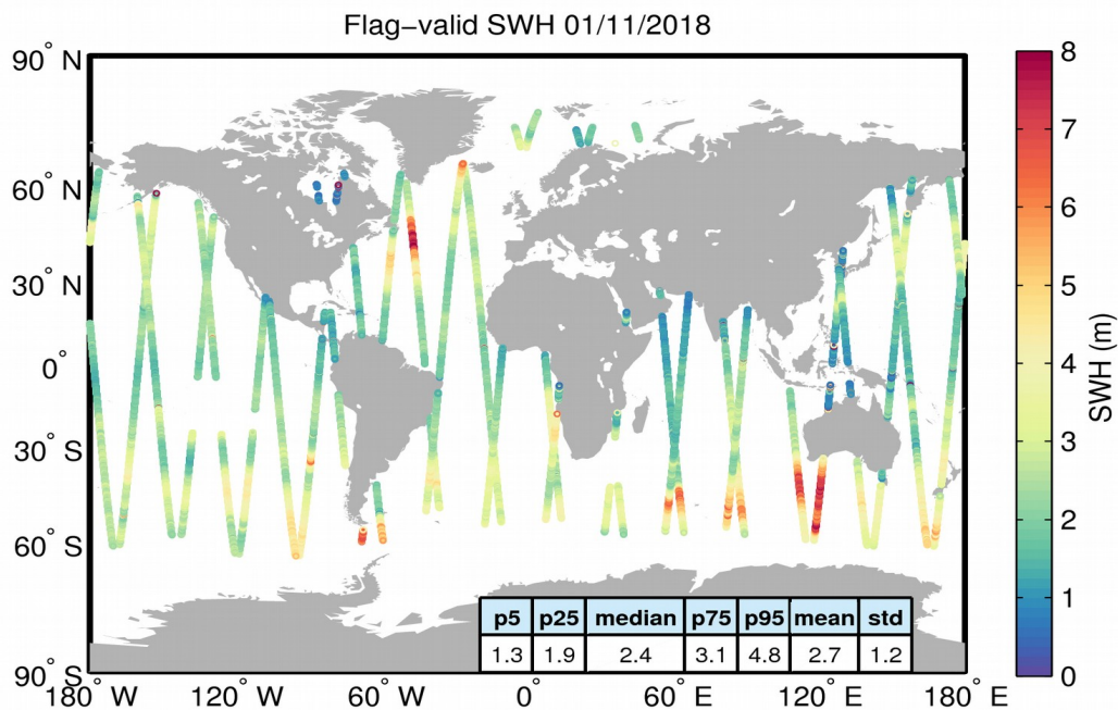
Figure 15. Geographical distribution of flag-valid SWH data over oceans and lakes for 01/11/2018. The statistical values shown in the table refer to the SWH in m and are calculated over all measurements shown in the figure.
