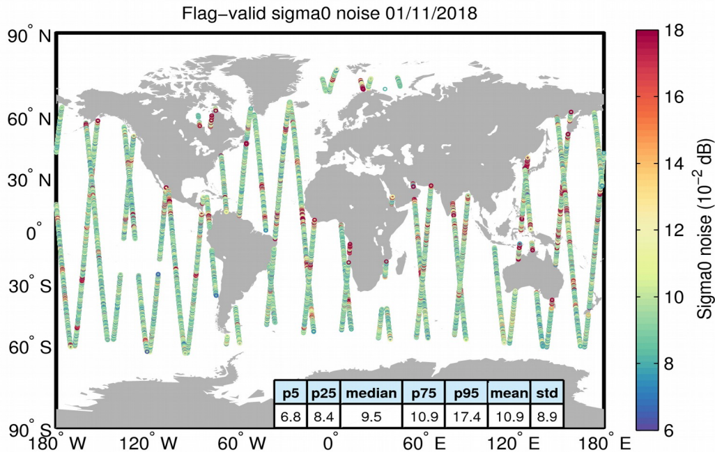
Figure 26. Geographical distribution of flag-valid 20-Hz sigma0 measurement noise over oceans and lakes for 01/11/2018. The statistical values shown in the table refer to the sigma0 noise and are calculated over all measurements shown in the figure.
