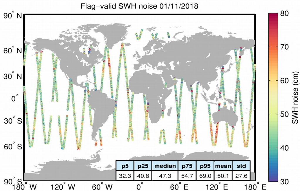
Figure 18. Geographical distribution of flag-valid 20-Hz SWH measurement noise over oceans and lakes for 01/11/2018. The statistical values shown in the figure refer to the SWH noise and are calculated over all measurements shown in the figure.
