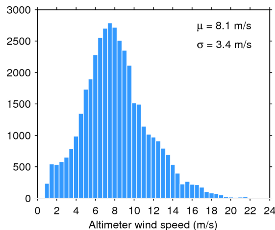
Figure 35. Histogram of science-valid wind over oceans and lakes for 01/11/2018. The mean ( \mu ) and standard deviation ( \sigma ) are also shown. Note that values larger than 24 m/s are excluded from the histogram for the sake of readability but not from the computation of \mu and \sigma .
