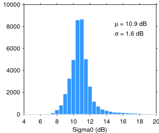
Figure 25. Histogram of flag-valid sigma0 over oceans and lakes for 01/11/2018. The mean ( \mu ) and standard deviation ( \sigma ) are also shown. Note that values outside [4 20] dB are excluded from the histogram for the sake of readability but not from the computation of \mu and \sigma .
