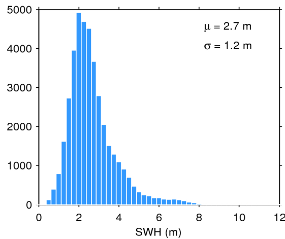
Figure 17. Histogram of flag-valid SWH over oceans and lakes for 01/11/2018. The mean ( \mu ) and standard deviation ( \sigma ) are also shown. Note that values larger than 12 m are excluded from the histogram for the sake of readability but not from the computation of \mu and \sigma .
