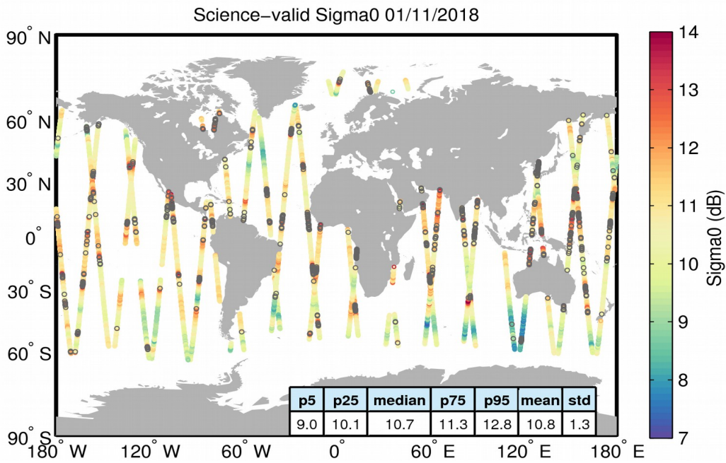
Figure 27. Geographical distribution of science-valid sigma0 data over oceans and lakes for 01/11/2018. The statistical values shown in the table refer to the sigma0 in dB and are calculated over all measurements shown in the figure. Gray circles denote records that have been rejected based on the editing criteria described in Table 4.
