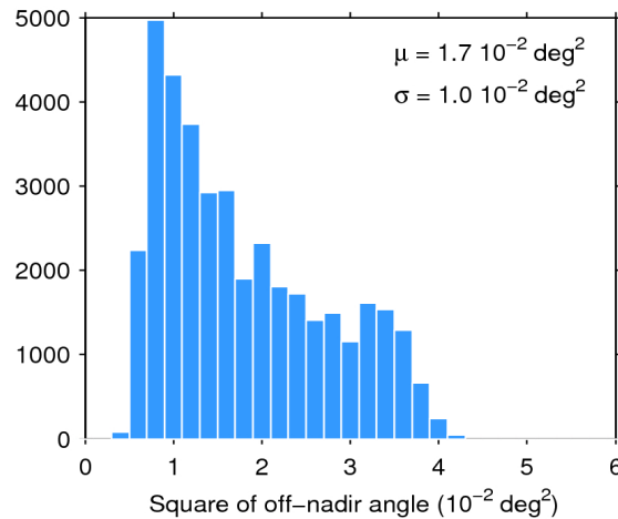
Figure 39. Histogram of flag-valid mispointing over oceans and lakes for 01/11/2018. The mean ( \mu ) and standard deviation ( \sigma ) are also shown. Note that values larger than 6 \cdot 10^{-2} \text{ deg}^2 are excluded from the histogram for the sake of readability but not from the computation of \mu and \sigma .
