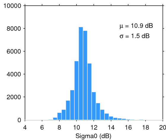
Figure 28. Histogram of science-valid sigma0 over oceans and lakes for 31/10/2018. The mean ( \mu ) and standard deviation ( \sigma ) are also shown. Note that values outside [4 20] dB are excluded from the histogram for the sake of readability but not from the computation of \mu and \sigma .
