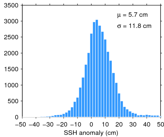
Figure 11. Histogram of science-valid SSH anomaly over oceans and lakes for 31/10/2018. The mean ( \mu ) and standard deviation ( \sigma ) are also shown. Note that values outside [-50 50] cm are excluded from the histogram for the sake of readability but not from the computation of \mu and \sigma .
