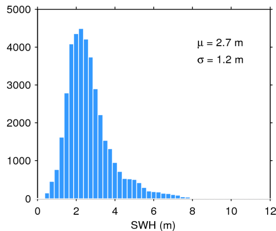
Figure 20. Histogram of science-valid SWH over oceans and lakes for 31/10/2018. The mean ( \mu ) and standard deviation ( \sigma ) are also shown. Note that values larger than 12 m are excluded from the histogram for the sake of readability but not from the computation of \mu and \sigma .
