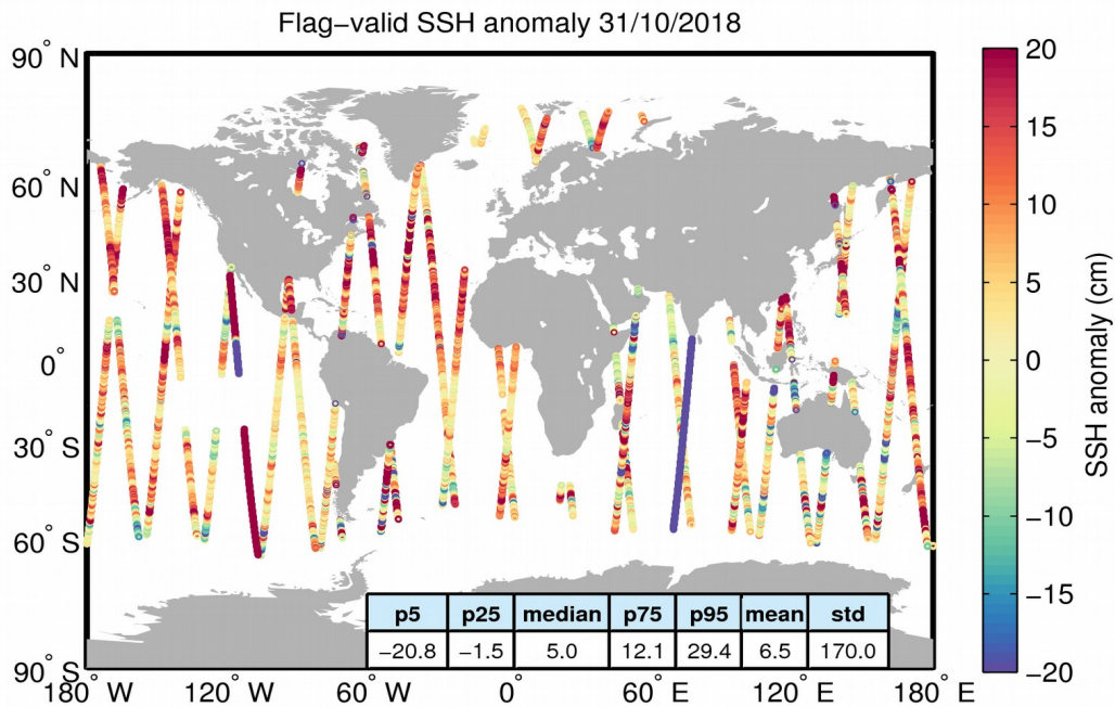
Figure 5. Geographical distribution of flag-valid 1-Hz SSH anomaly data over oceans and lakes for 31/10/2018. The statistical values shown in the table refer to the SSH anomaly in cm and are calculated over all measurements shown in the figure.
