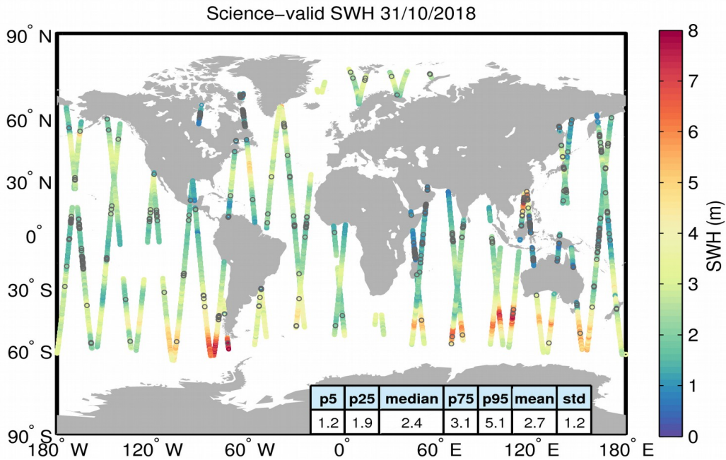
Figure 19. Geographical distribution of science-valid SWH data over oceans and lakes for 31/10/2018. The statistical values shown in the table refer to the SWH in m and are calculated over all measurements shown in the figure. Gray circles denote records that have been rejected based on the editing criteria described in Table 3.
