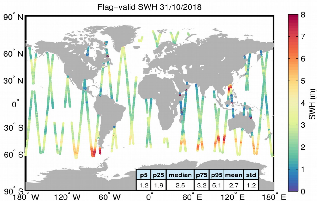
Figure 15. Geographical distribution of flag-valid SWH data over oceans and lakes for 31/10/2018. The statistical values shown in the table refer to the SWH in m and are calculated over all measurements shown in the figure.
