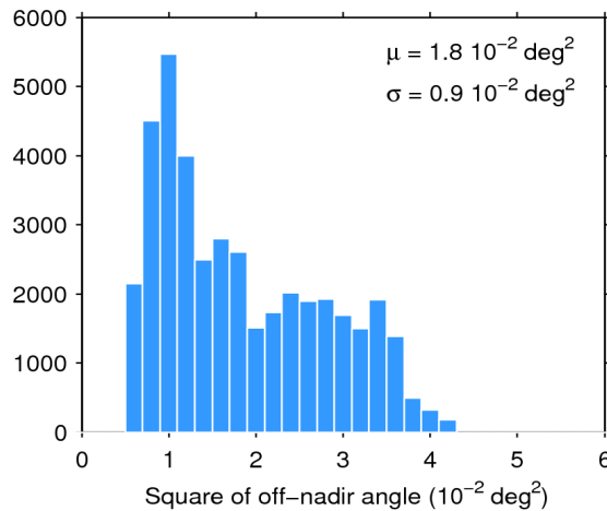
Figure 39. Histogram of flag-valid mispointing over oceans and lakes for 31/10/2018. The mean ( \mu ) and standard deviation ( \sigma ) are also shown. Note that values larger than 6 \cdot 10^{-2} \text{ deg}^2 are excluded from the histogram for the sake of readability but not from the computation of \mu and \sigma .
