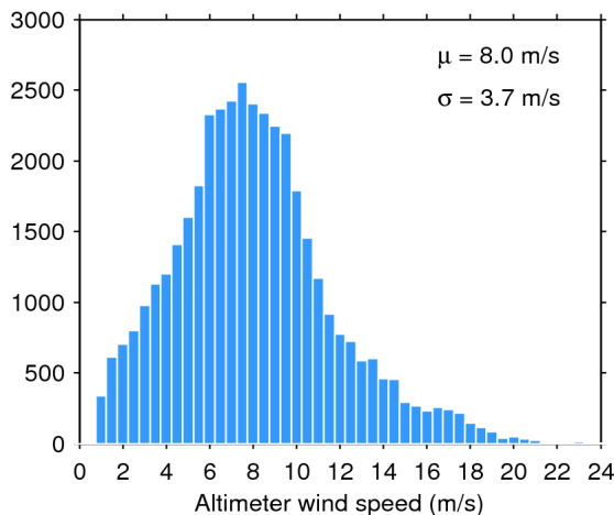
Figure 33. Histogram of flag-valid wind over oceans and lakes for 31/10/2018. The mean ( \mu ) and standard deviation ( \sigma ) are also shown. Note that values larger than 24 m/s are excluded from the histogram for the sake of readability but not from the computation of \mu and \sigma .
