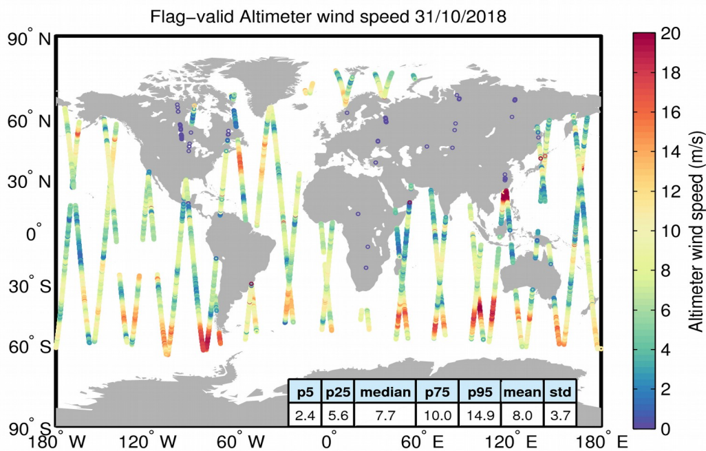
Figure 31. Geographical distribution of flag-valid wind data over oceans and lakes for 31/10/2018. The statistical values shown in the table refer to the wind in m/s and are calculated over all measurements shown in the figure.
