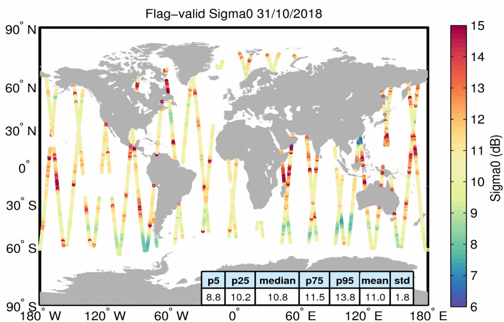
Figure 23. Geographical distribution of flag-valid sigma0 data over oceans and lakes for 31/10/2018. The statistical values shown in the table refer to the sigma0 in dB and are calculated over all measurements shown in the figure.
