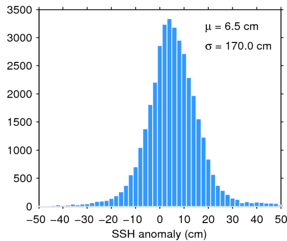
Figure 7. Histogram of flag-valid SSH anomaly over oceans and lakes for 31/10/2018. The mean ( \mu ) and standard deviation ( \sigma ) are also shown. Note that values outside [-50 50] cm are excluded from the histogram for the sake of readability but not from the computation of \mu and \sigma .
