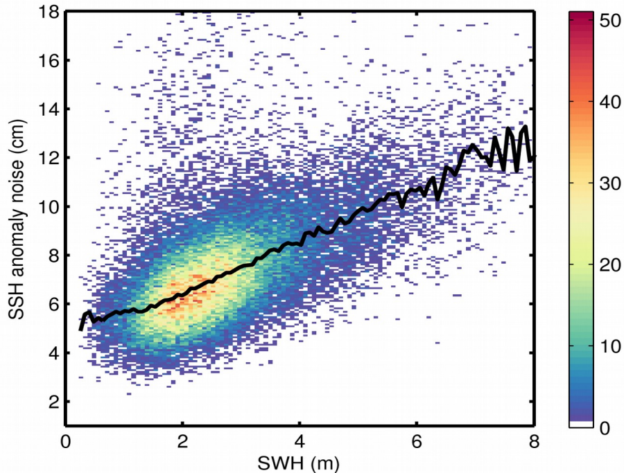
Figure 9. 2D histogram showing flag-valid SSH anomaly noise as a function of SWH for 31/10/2018. The black line denotes the median SSH anomaly noise as a function of SWH.
