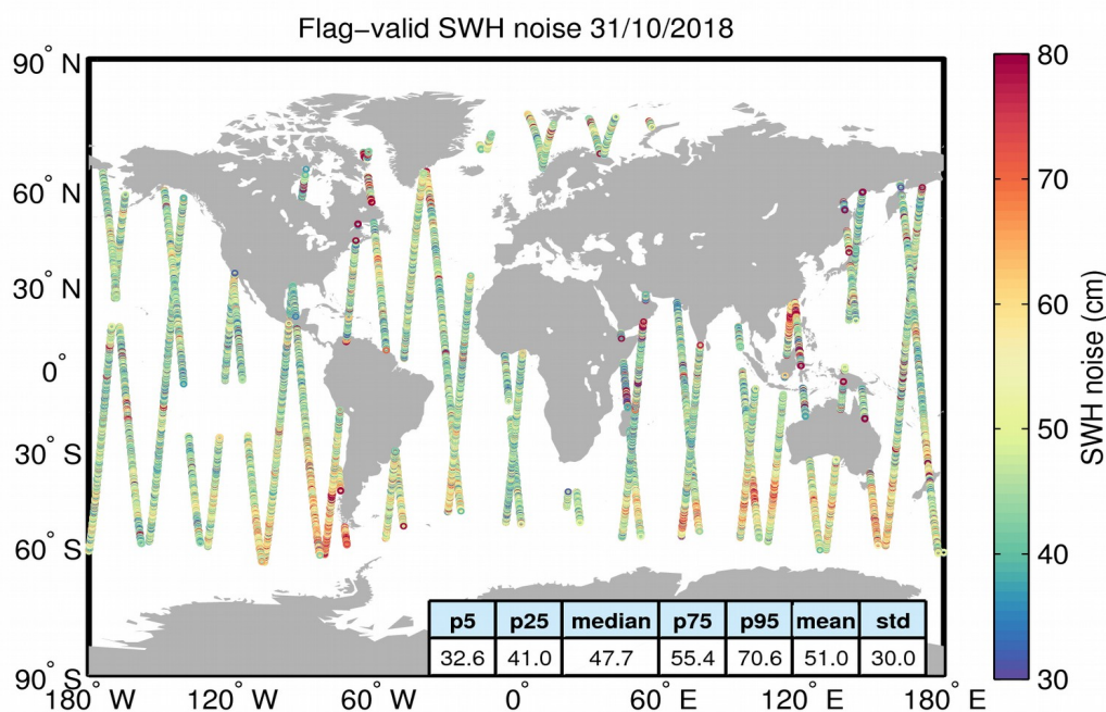
Figure 18. Geographical distribution of flag-valid 20-Hz SWH measurement noise over oceans and lakes for 31/10/2018. The statistical values shown in the table refer to the SWH noise and are calculated over all measurements shown in the figure.
