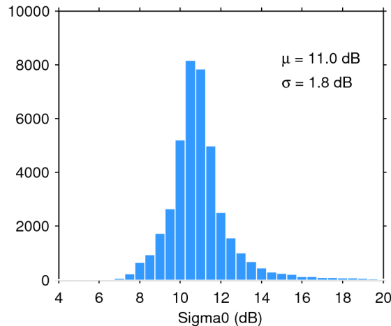
Figure 25. Histogram of flag-valid sigma0 over oceans and lakes for 31/10/2018. The mean ( \mu ) and standard deviation ( \sigma ) are also shown. Note that values outside [4 20] dB are excluded from the histogram for the sake of readability but not from the computation of \mu and \sigma .
