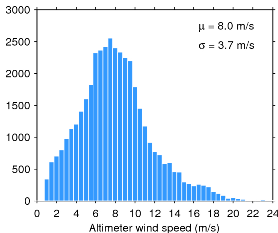
Figure 35. Histogram of science-valid wind over oceans and lakes for 31/10/2018. The mean ( \mu ) and standard deviation ( \sigma ) are also shown. Note that values larger than 24 m/s are excluded from the histogram for the sake of readability but not from the computation of \mu and \sigma .
