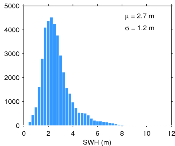
Figure 17. Histogram of flag-valid SWH over oceans and lakes for 31/10/2018. The mean ( \mu ) and standard deviation ( \sigma ) are also shown. Note that values larger than 12 m are excluded from the histogram for the sake of readability but not from the computation of \mu and \sigma .
