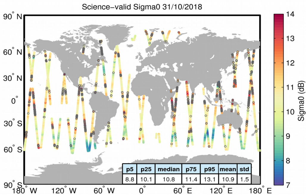
Figure 27. Geographical distribution of science-valid sigma0 data over oceans and lakes for 31/10/2018. The statistical values shown in the table refer to the sigma0 in dB and are calculated over all measurements shown in the figure. Gray circles denote records that have been rejected based on the editing criteria described in Table 4.
