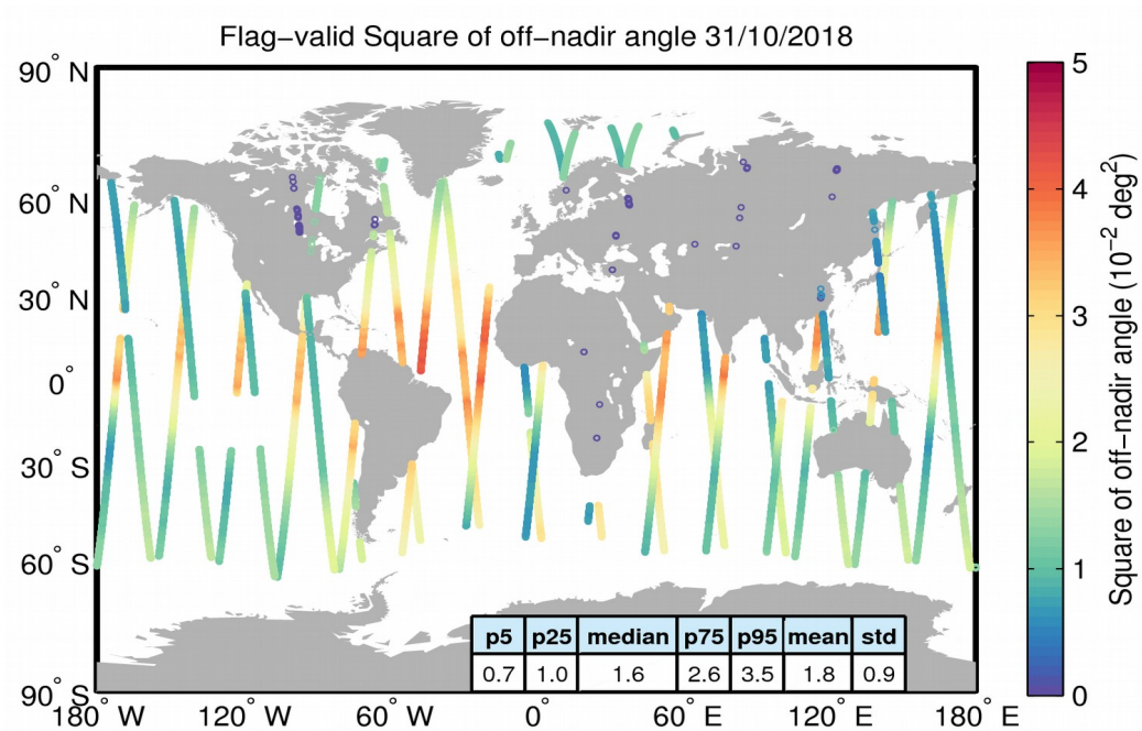
Figure 37. Geographical distribution of flag-valid mispointing data over oceans and lakes for 31/10/2018. The statistical values shown in the table refer to the mispointing in 10^{-2} deg 2 and are calculated over all measurements shown in the figure.
