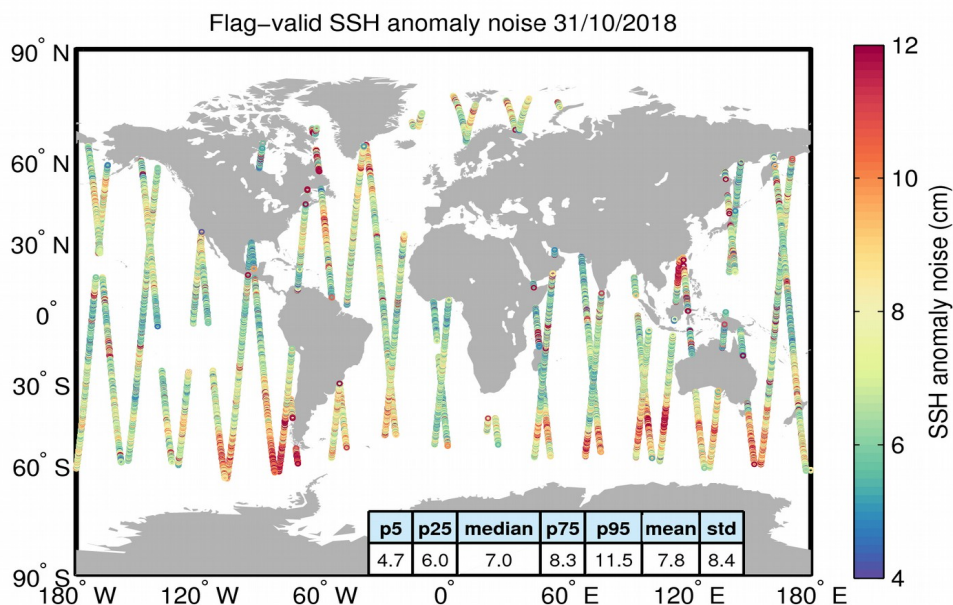
Figure 8. Geographical distribution of flag-valid 20-Hz SSH anomaly measurement noise over oceans and lakes for 31/10/2018. The statistical values shown in the table refer to the SSH anomaly noise and are calculated over all measurements shown in the figure.
