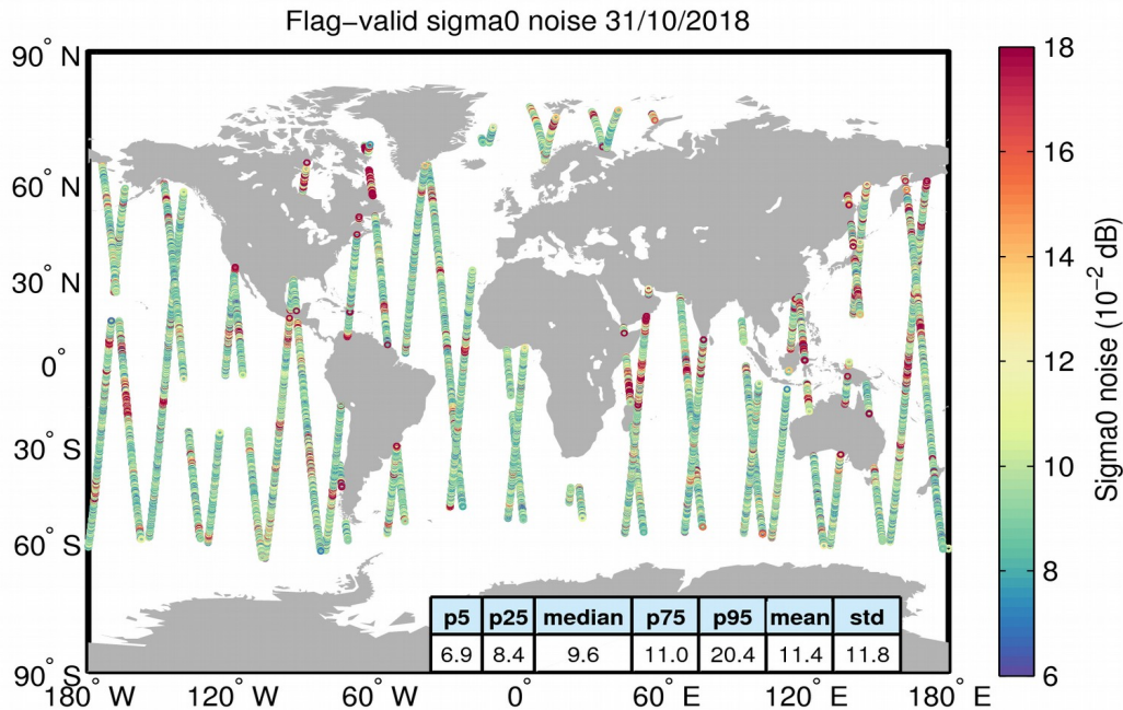
Figure 26. Geographical distribution of flag-valid 20-Hz sigma0 measurement noise over oceans and lakes for 31/10/2018. The statistical values shown in the table refer to the sigma0 noise and are calculated over all measurements shown in the figure.
