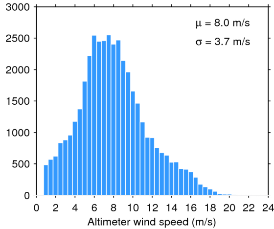
Figure 33. Histogram of flag-valid wind over oceans and lakes for 30/10/2018. The mean ( \mu ) and standard deviation ( \sigma ) are also shown. Note that values larger than 24 m/s are excluded from the histogram for the sake of readability but not from the computation of \mu and \sigma .
