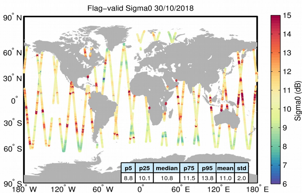
Figure 23. Geographical distribution of flag-valid sigma0 data over oceans and lakes for 30/10/2018. The statistical values shown in the table refer to the sigma0 in dB and are calculated over all measurements shown in the figure.
