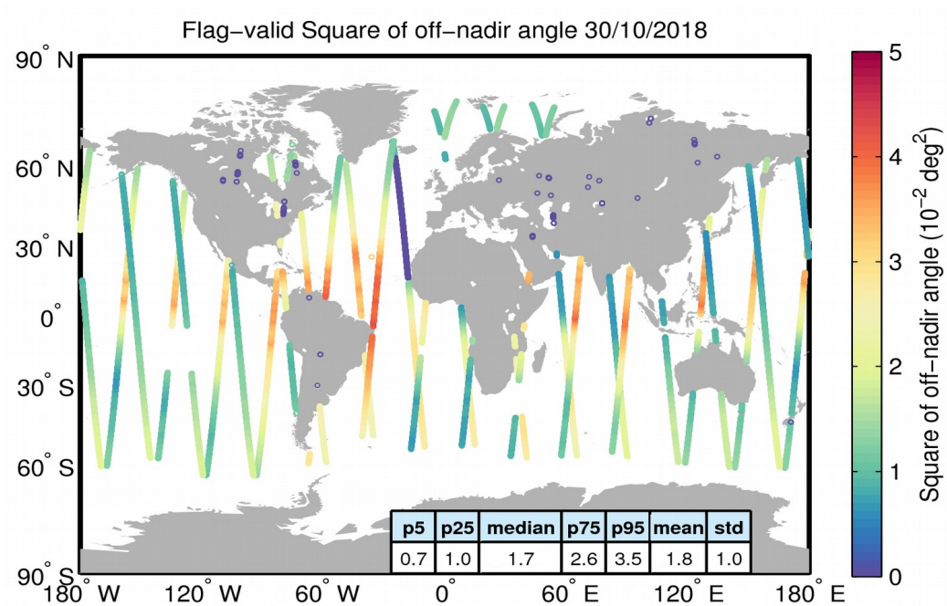
Figure 37. Geographical distribution of flag-valid mispointing data over oceans and lakes for 30/10/2018. The statistical values shown in the table refer to the mispointing in 10^{-2} deg 2 and are calculated over all measurements shown in the figure.
