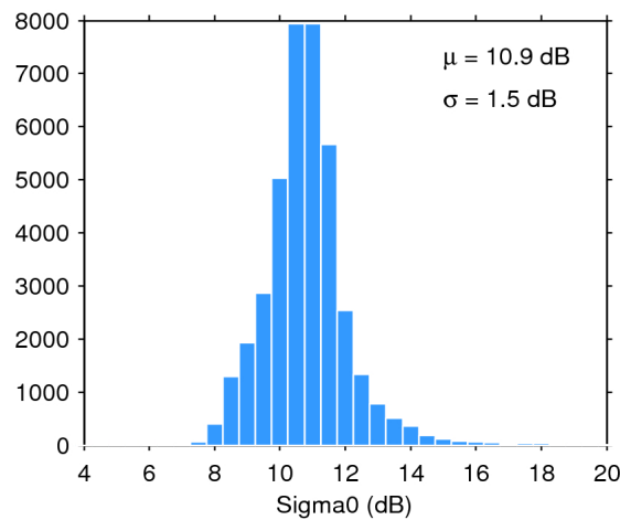
Figure 28. Histogram of science-valid sigma0 over oceans and lakes for 30/10/2018. The mean ( \mu ) and standard deviation ( \sigma ) are also shown. Note that values outside [4 20] dB are excluded from the histogram for the sake of readability but not from the computation of \mu and \sigma .
