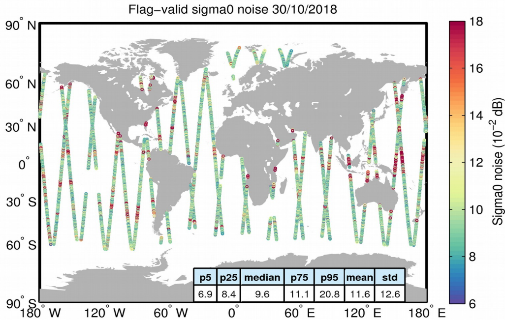
Figure 26. Geographical distribution of flag-valid 20-Hz sigma0 measurement noise over oceans and lakes for 30/10/2018. The statistical values shown in the table refer to the sigma0 noise and are calculated over all measurements shown in the figure.
