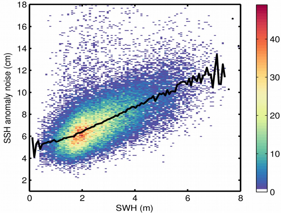
Figure 9. 2D histogram showing flag-valid SSH anomaly noise as a function of SWH for 30/10/2018. The black line denotes the median SSH anomaly noise as a function of SWH.
