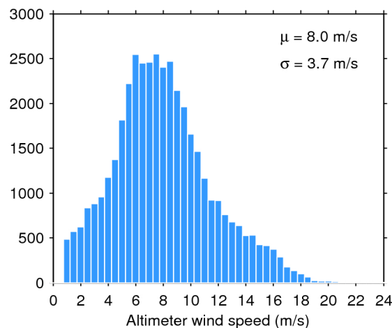
Figure 35. Histogram of science-valid wind over oceans and lakes for 30/10/2018. The mean ( \mu ) and standard deviation ( \sigma ) are also shown. Note that values larger than 24 m/s are excluded from the histogram for the sake of readability but not from the computation of \mu and \sigma .
