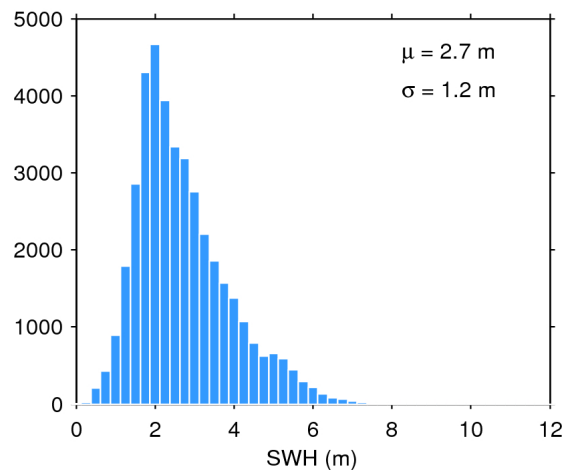
Figure 20. Histogram of science-valid SWH over oceans and lakes for 30/10/2018. The mean ( \mu ) and standard deviation ( \sigma ) are also shown. Note that values larger than 12 m are excluded from the histogram for the sake of readability but not from the computation of \mu and \sigma .
