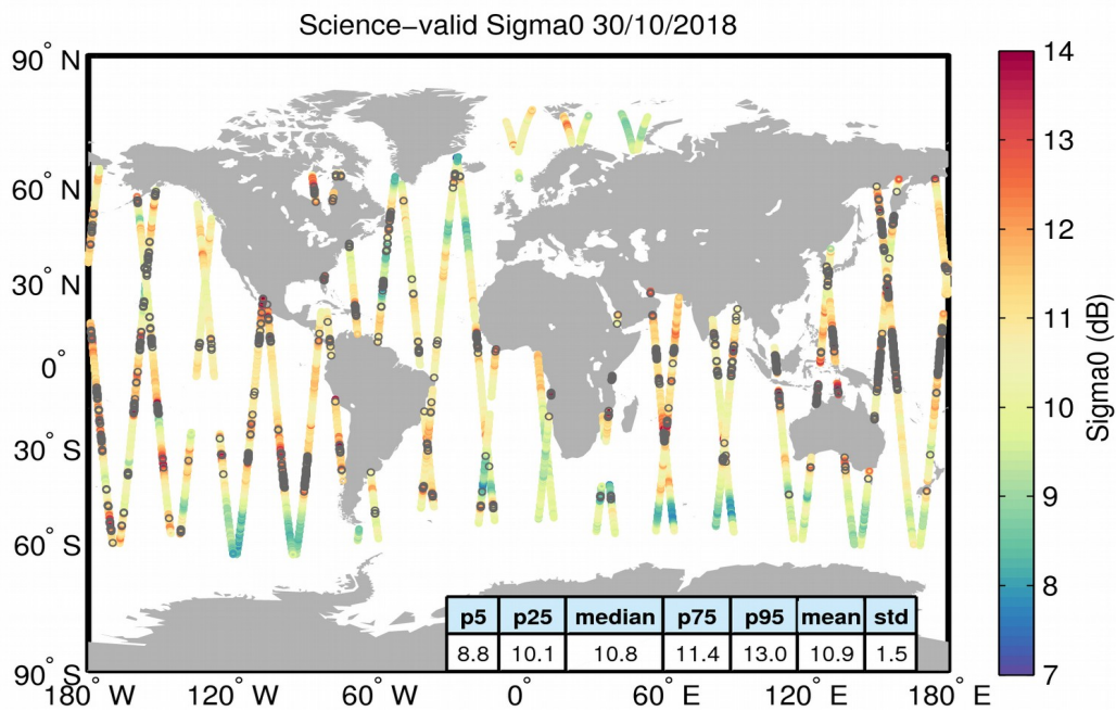
Figure 27. Geographical distribution of science-valid sigma0 data over oceans and lakes for 30/10/2018. The statistical values shown in the table refer to the sigma0 in dB and are calculated over all measurements shown in the figure. Gray circles denote records that have been rejected based on the editing criteria described in Table 4.
