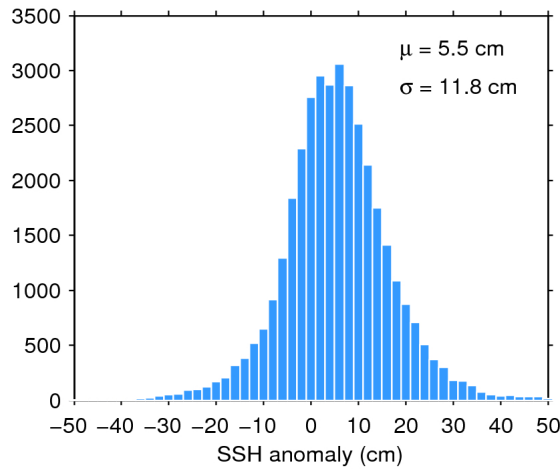
Figure 11. Histogram of science-valid SSH anomaly over oceans and lakes for 30/10/2018. The mean ( \mu ) and standard deviation ( \sigma ) are also shown. Note that values outside [-50 50] cm are excluded from the histogram for the sake of readability but not from the computation of \mu and \sigma .
