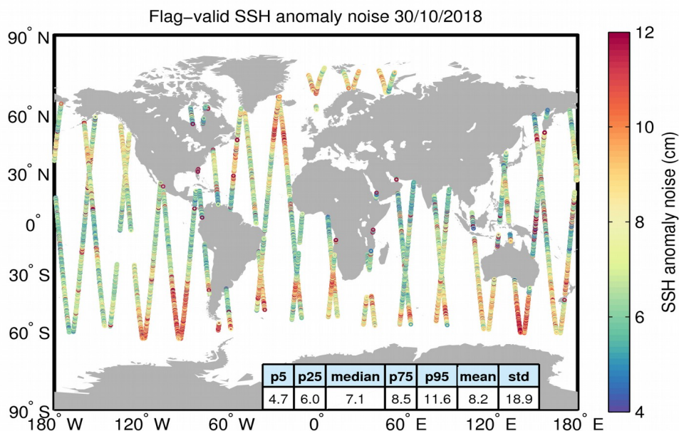
Figure 8. Geographical distribution of flag-valid 20-Hz SSH anomaly measurement noise over oceans and lakes for 30/10/2018. The statistical values shown in the table refer to the SSH anomaly noise and are calculated over all measurements shown in the figure.
