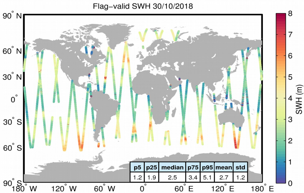
Figure 15. Geographical distribution of flag-valid SWH data over oceans and lakes for 30/10/2018. The statistical values shown in the table refer to the SWH in m and are calculated over all measurements shown in the figure.
