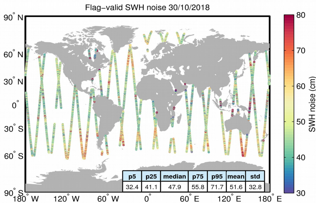
Figure 18. Geographical distribution of flag-valid 20-Hz SWH measurement noise over oceans and lakes for 30/10/2018. The statistical values shown in the table refer to the SWH noise and are calculated over all measurements shown in the figure.
