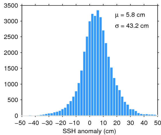
Figure 7. Histogram of flag-valid SSH anomaly over oceans and lakes for 30/10/2018. The mean ( \mu ) and standard deviation ( \sigma ) are also shown. Note that values outside [-50\ 50] cm are excluded from the histogram for the sake of readability but not from the computation of \mu and \sigma .
