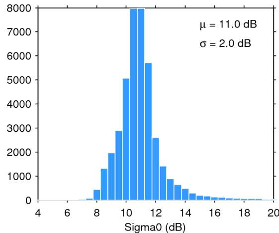
Figure 25. Histogram of flag-valid sigma0 over oceans and lakes for 30/10/2018. The mean ( \mu ) and standard deviation ( \sigma ) are also shown. Note that values outside [4 20] dB are excluded from the histogram for the sake of readability but not from the computation of \mu and \sigma .
