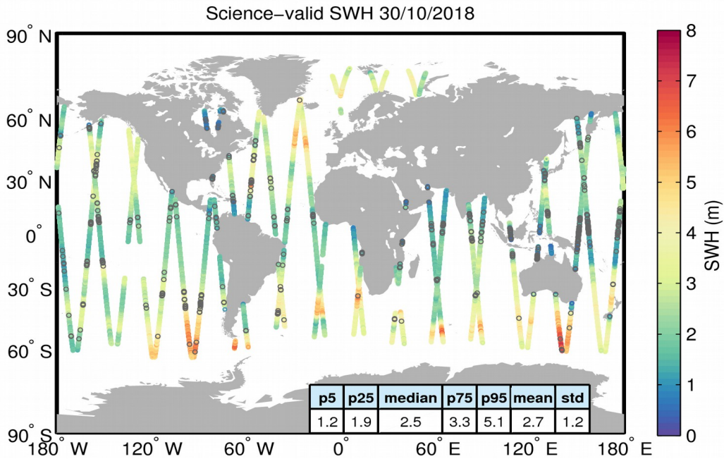
Figure 19. Geographical distribution of science-valid SWH data over oceans and lakes for 30/10/2018. The statistical values shown in the table refer to the SWH in m and are calculated over all measurements shown in the figure. Gray circles denote records that have been rejected based on the editing criteria described in Table 3.
