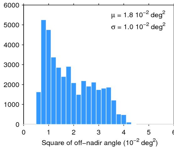
Figure 39. Histogram of flag-valid mispointing over oceans and lakes for 30/10/2018. The mean ( \mu ) and standard deviation ( \sigma ) are also shown. Note that values larger than 6 \cdot 10^{-2} \text{ deg}^2 are excluded from the histogram for the sake of readability but not from the computation of \mu and \sigma .
