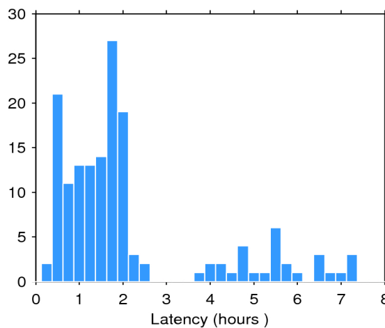
Figure 2. Histogram of the data latency for 30/10/2018. The y-axis denotes the number of files that are made available with a delay of x-hours with respect to the mean time of the records stored in the file.
