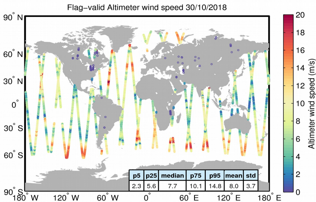
Figure 31. Geographical distribution of flag-valid wind data over oceans and lakes for 30/10/2018. The statistical values shown in the table refer to the wind in m/s and are calculated over all measurements shown in the figure.
