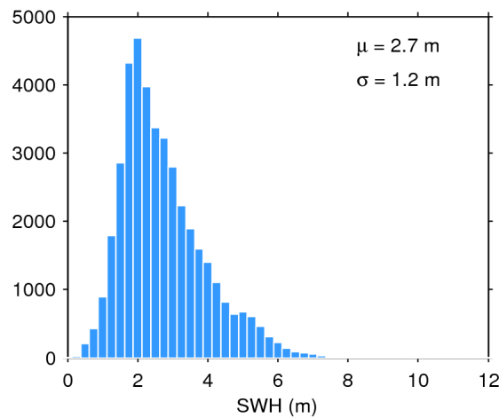
Figure 17. Histogram of flag-valid SWH over oceans and lakes for 30/10/2018. The mean ( \mu ) and standard deviation ( \sigma ) are also shown. Note that values larger than 12 m are excluded from the histogram for the sake of readability but not from the computation of \mu and \sigma .
