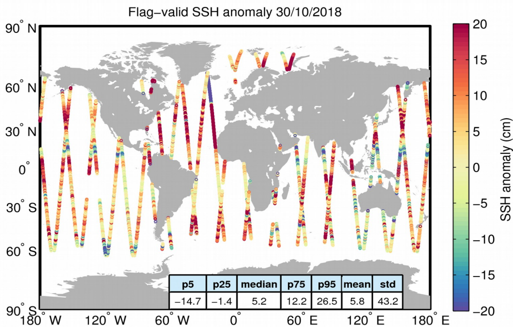
Figure 5. Geographical distribution of flag-valid 1-Hz SSH anomaly data over oceans and lakes for 30/10/2018. The statistical values shown in the table refer to the SSH anomaly in cm and are calculated over all measurements shown in the figure.
