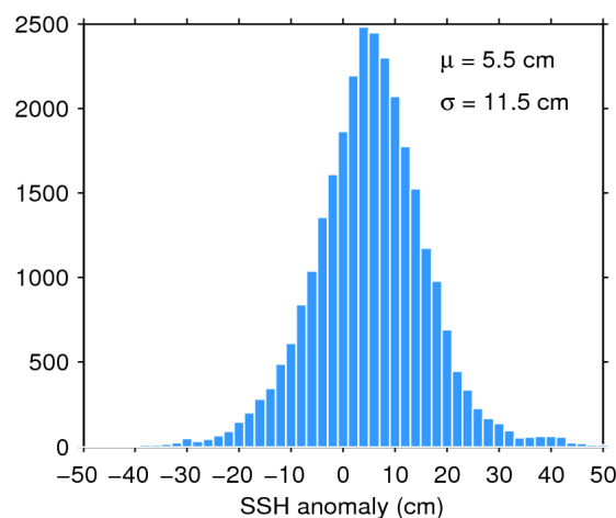
Figure 11. Histogram of science-valid SSH anomaly over oceans and lakes for 29/10/2018. The mean ( \mu ) and standard deviation ( \sigma ) are also shown. Note that values outside [-50 50] cm are excluded from the histogram for the sake of readability but not from the computation of \mu and \sigma .
