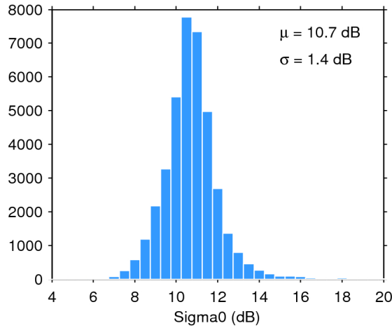
Figure 28. Histogram of science-valid sigma0 over oceans and lakes for 29/10/2018. The mean ( \mu ) and standard deviation ( \sigma ) are also shown. Note that values outside [4 20] dB are excluded from the histogram for the sake of readability but not from the computation of \mu and \sigma .
