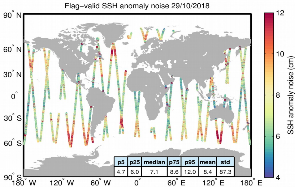
Figure 8. Geographical distribution of flag-valid 20-Hz SSH anomaly measurement noise over oceans and lakes for 29/10/2018. The statistical values shown in the table refer to the SSH anomaly noise and are calculated over all measurements shown in the figure.
