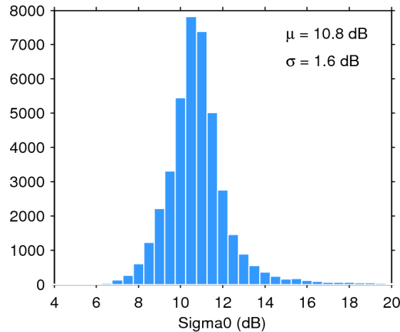
Figure 25. Histogram of flag-valid sigma0 over oceans and lakes for 29/10/2018. The mean ( \mu ) and standard deviation ( \sigma ) are also shown. Note that values outside [4 20] dB are excluded from the histogram for the sake of readability but not from the computation of \mu and \sigma .
