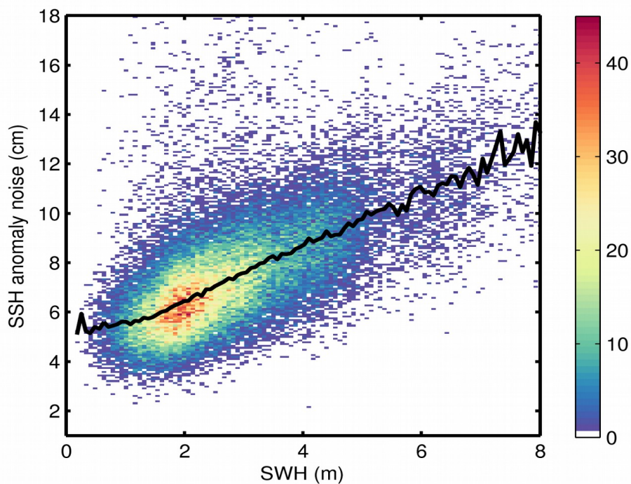
Figure 9. 2D histogram showing flag-valid SSH anomaly noise as a function of SWH for 29/10/2018. The black line denotes the median SSH anomaly noise as a function of SWH.
