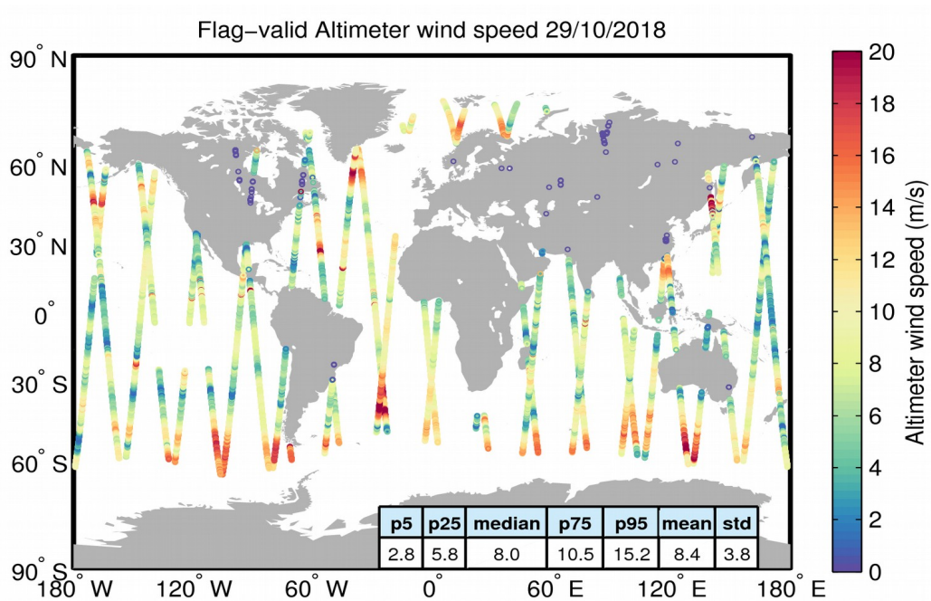
Figure 31. Geographical distribution of flag-valid wind data over oceans and lakes for 29/10/2018. The statistical values shown in the table refer to the wind in m/s and are calculated over all measurements shown in the figure.
