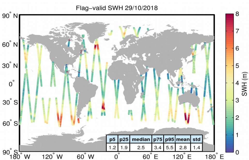
Figure 15. Geographical distribution of flag-valid SWH data over oceans and lakes for 29/10/2018. The statistical values shown in the table refer to the SWH in m and are calculated over all measurements shown in the figure.
