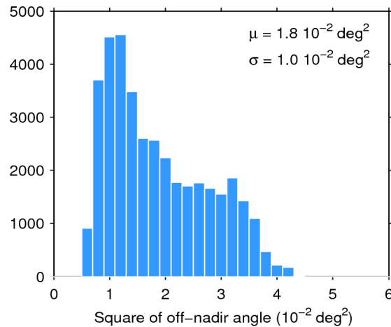
Figure 39. Histogram of flag-valid mispointing over oceans and lakes for 29/10/2018. The mean ( \mu ) and standard deviation ( \sigma ) are also shown. Note that values larger than 6 \cdot 10^{-2} \text{ deg}^2 are excluded from the histogram for the sake of readability but not from the computation of \mu and \sigma .
