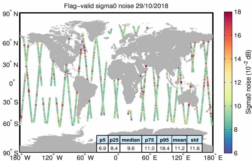
Figure 26. Geographical distribution of flag-valid 20-Hz sigma0 measurement noise over oceans and lakes for 29/10/2018. The statistical values shown in the table refer to the sigma0 noise and are calculated over all measurements shown in the figure.
