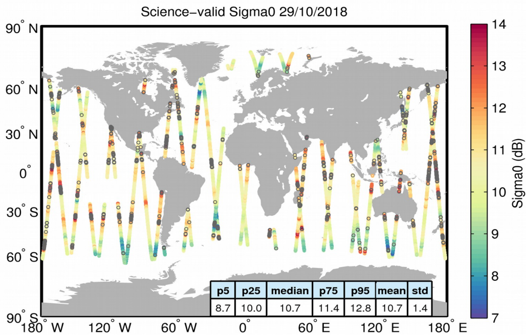
Figure 27. Geographical distribution of science-valid sigma0 data over oceans and lakes for 29/10/2018. The statistical values shown in the table refer to the sigma0 in dB and are calculated over all measurements shown in the figure. Gray circles denote records that have been rejected based on the editing criteria described in Table 4.
