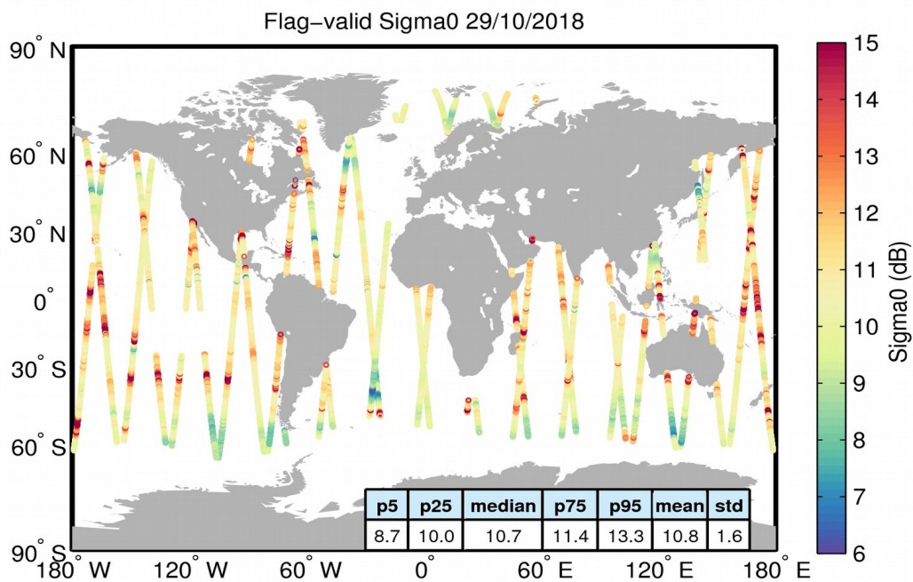
Figure 23. Geographical distribution of flag-valid sigma0 data over oceans and lakes for 29/10/2018. The statistical values shown in the table refer to the sigma0 in dB and are calculated over all measurements shown in the figure.
