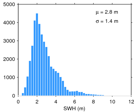
Figure 17. Histogram of flag-valid SWH over oceans and lakes for 29/10/2018. The mean ( \mu ) and standard deviation ( \sigma ) are also shown. Note that values larger than 12 m are excluded from the histogram for the sake of readability but not from the computation of \mu and \sigma .
