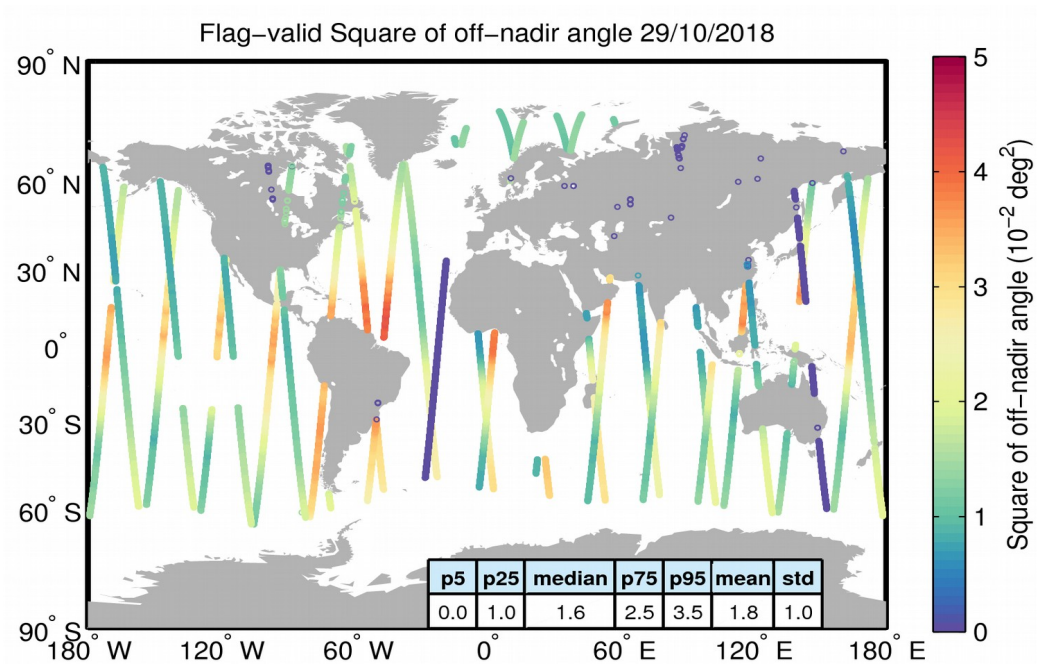
Figure 37. Geographical distribution of flag-valid mispointing data over oceans and lakes for 29/10/2018. The statistical values shown in the table refer to the mispointing in 10^{-2} deg 2 and are calculated over all measurements shown in the figure.
