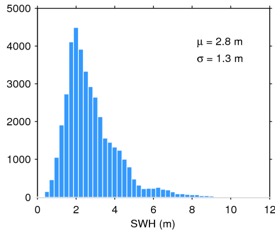
Figure 20. Histogram of science-valid SWH over oceans and lakes for 29/10/2018. The mean ( \mu ) and standard deviation ( \sigma ) are also shown. Note that values larger than 12 m are excluded from the histogram for the sake of readability but not from the computation of \mu and \sigma .
