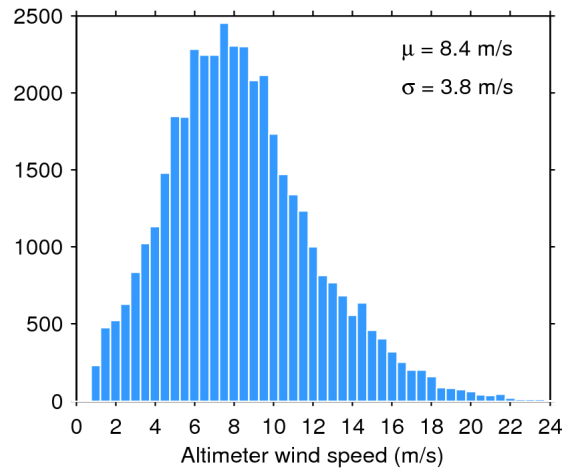
Figure 33. Histogram of flag-valid wind over oceans and lakes for 29/10/2018. The mean ( \mu ) and standard deviation ( \sigma ) are also shown. Note that values larger than 24 m/s are excluded from the histogram for the sake of readability but not from the computation of \mu and \sigma .
