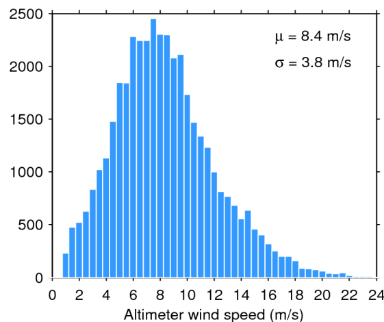
Figure 35. Histogram of science-valid wind over oceans and lakes for 29/10/2018. The mean ( \mu ) and standard deviation ( \sigma ) are also shown. Note that values larger than 24 m/s are excluded from the histogram for the sake of readability but not from the computation of \mu and \sigma .
