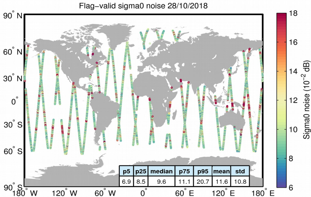
Figure 26. Geographical distribution of flag-valid 20-Hz sigma0 measurement noise over oceans and lakes for 28/10/2018. The statistical values shown in the table refer to the sigma0 noise and are calculated over all measurements shown in the figure.
