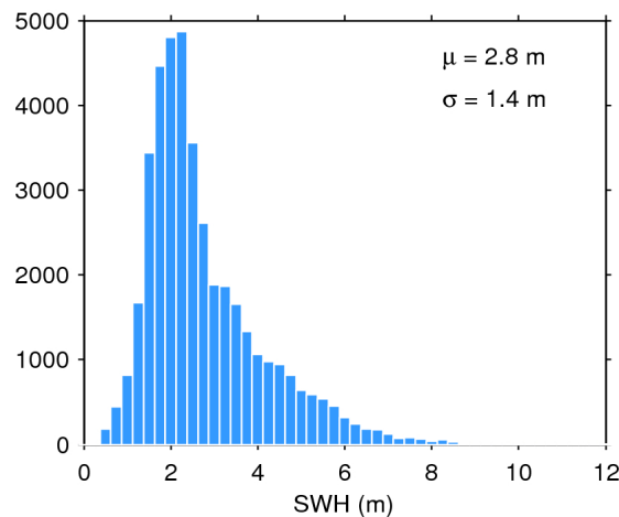
Figure 17. Histogram of flag-valid SWH over oceans and lakes for 28/10/2018. The mean ( \mu ) and standard deviation ( \sigma ) are also shown. Note that values larger than 12 m are excluded from the histogram for the sake of readability but not from the computation of \mu and \sigma .
