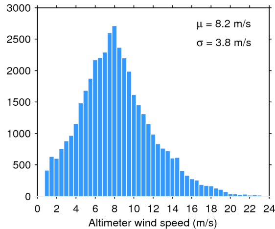
Figure 33. Histogram of flag-valid wind over oceans and lakes for 28/10/2018. The mean ( \mu ) and standard deviation ( \sigma ) are also shown. Note that values larger than 24 m/s are excluded from the histogram for the sake of readability but not from the computation of \mu and \sigma .
