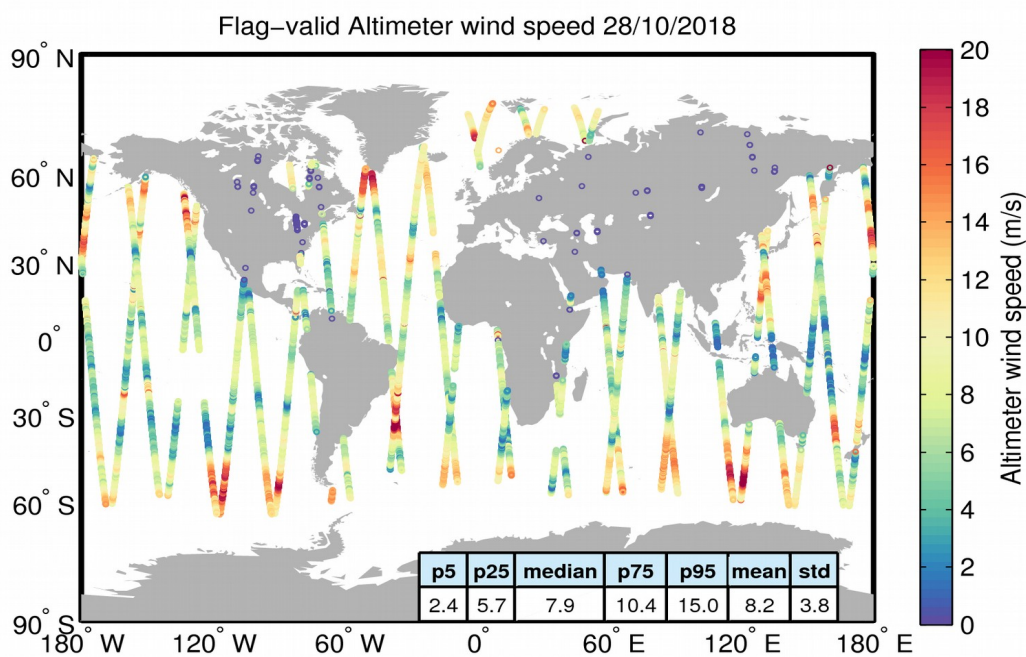
Figure 31. Geographical distribution of flag-valid wind data over oceans and lakes for 28/10/2018. The statistical values shown in the table refer to the wind in m/s and are calculated over all measurements shown in the figure.
