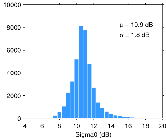
Figure 25. Histogram of flag-valid sigma0 over oceans and lakes for 28/10/2018. The mean ( \mu ) and standard deviation ( \sigma ) are also shown. Note that values outside [4 20] dB are excluded from the histogram for the sake of readability but not from the computation of \mu and \sigma .
