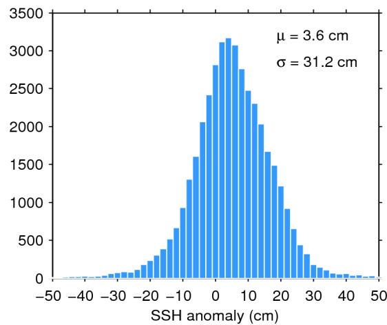
Figure 7. Histogram of flag-valid SSH anomaly over oceans and lakes for 28/10/2018. The mean ( \mu ) and standard deviation ( \sigma ) are also shown. Note that values outside [-50\ 50] cm are excluded from the histogram for the sake of readability but not from the computation of \mu and \sigma .
