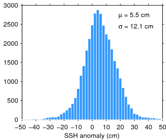
Figure 11. Histogram of science-valid SSH anomaly over oceans and lakes for 28/10/2018. The mean ( \mu ) and standard deviation ( \sigma ) are also shown. Note that values outside [-50 50] cm are excluded from the histogram for the sake of readability but not from the computation of \mu and \sigma .
