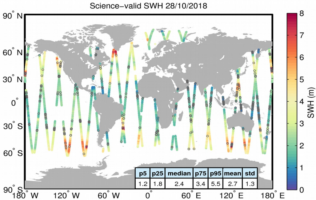
Figure 19. Geographical distribution of science-valid SWH data over oceans and lakes for 28/10/2018. The statistical values shown in the table refer to the SWH in m and are calculated over all measurements shown in the figure. Gray circles denote records that have been rejected based on the editing criteria described in Table 3.
