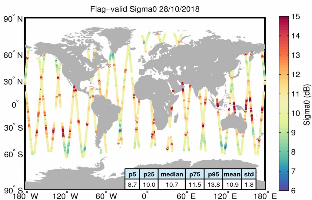
Figure 23. Geographical distribution of flag-valid sigma0 data over oceans and lakes for 28/10/2018. The statistical values shown in the table refer to the sigma0 in dB and are calculated over all measurements shown in the figure.
