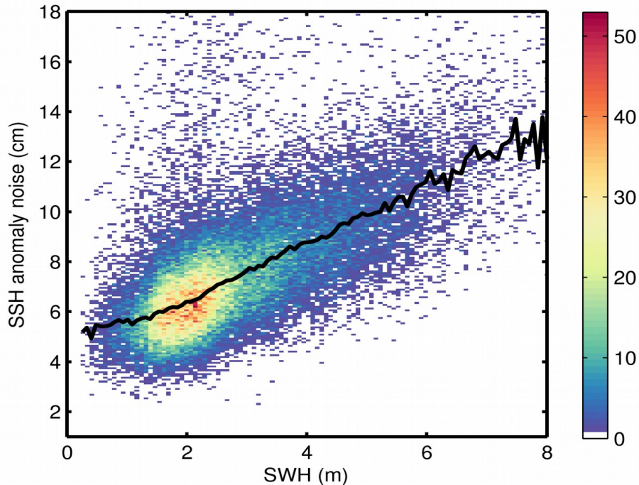
Figure 9. 2D histogram showing flag-valid SSH anomaly noise as a function of SWH for 28/10/2018. The black line denotes the median SSH anomaly noise as a function of SWH.
