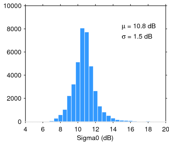
Figure 28. Histogram of science-valid sigma0 over oceans and lakes for 28/10/2018. The mean ( \mu ) and standard deviation ( \sigma ) are also shown. Note that values outside [4 20] dB are excluded from the histogram for the sake of readability but not from the computation of \mu and \sigma .
