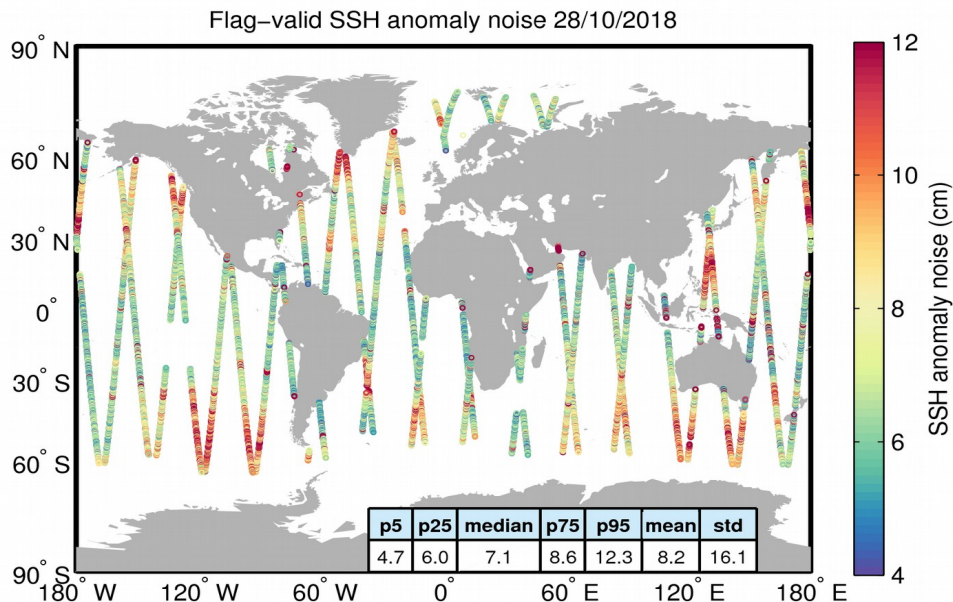
Figure 8. Geographical distribution of flag-valid 20-Hz SSH anomaly measurement noise over oceans and lakes for 28/10/2018. The statistical values shown in the table refer to the SSH anomaly noise and are calculated over all measurements shown in the figure.
