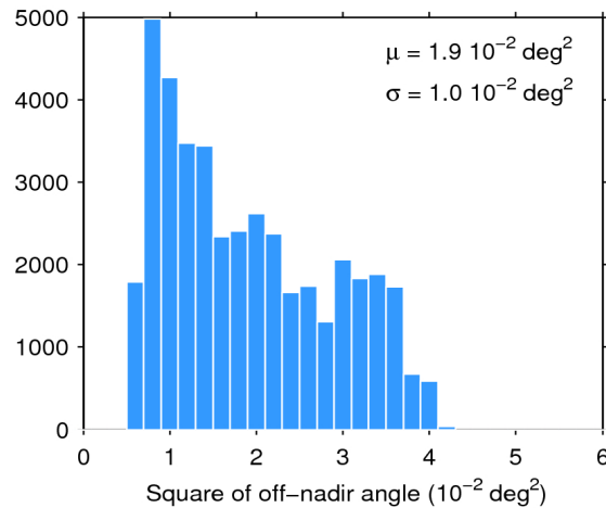
Figure 39. Histogram of flag-valid mispointing over oceans and lakes for 28/10/2018. The mean ( \mu ) and standard deviation ( \sigma ) are also shown. Note that values larger than 6 \cdot 10^{-2} \text{ deg}^2 are excluded from the histogram for the sake of readability but not from the computation of \mu and \sigma .
