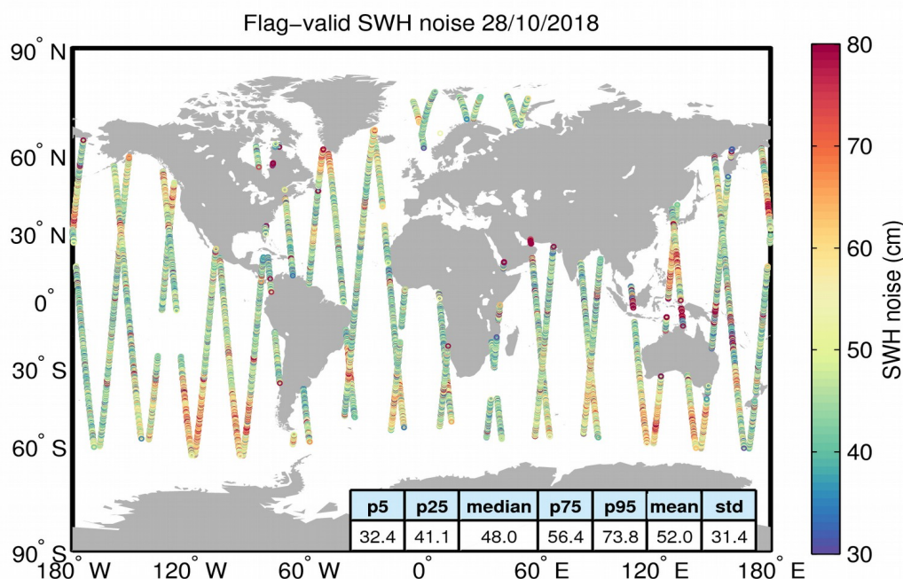
Figure 18. Geographical distribution of flag-valid 20-Hz SWH measurement noise over oceans and lakes for 28/10/2018. The statistical values shown in the figure refer to the SWH noise and are calculated over all measurements shown in the figure.
