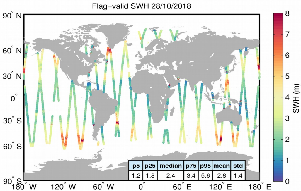
Figure 15. Geographical distribution of flag-valid SWH data over oceans and lakes for 28/10/2018. The statistical values shown in the table refer to the SWH in m and are calculated over all measurements shown in the figure.
