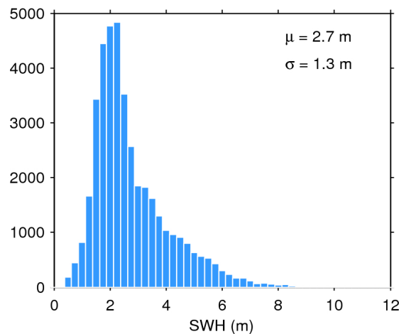
Figure 20. Histogram of science-valid SWH over oceans and lakes for 28/10/2018. The mean ( \mu ) and standard deviation ( \sigma ) are also shown. Note that values larger than 12 m are excluded from the histogram for the sake of readability but not from the computation of \mu and \sigma .
