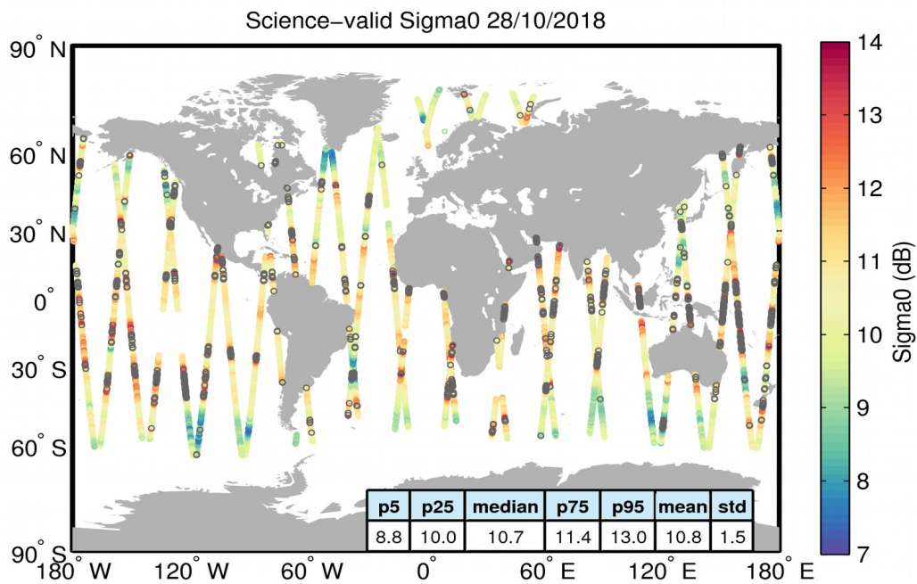
Figure 27. Geographical distribution of science-valid sigma0 data over oceans and lakes for 28/10/2018. The statistical values shown in the table refer to the sigma0 in dB and are calculated over all measurements shown in the figure. Gray circles denote records that have been rejected based on the editing criteria described in Table 4.
