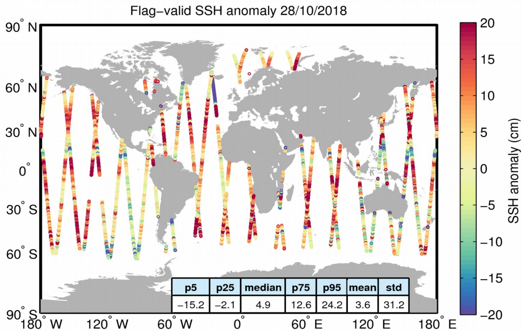
Figure 5. Geographical distribution of flag-valid 1-Hz SSH anomaly data over oceans and lakes for 28/10/2018. The statistical values shown in the table refer to the SSH anomaly in cm and are calculated over all measurements shown in the figure.
