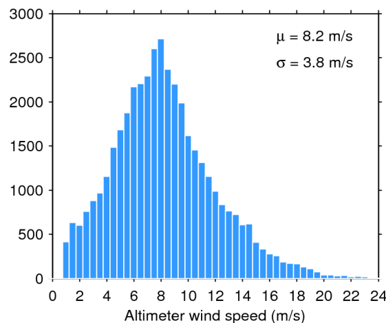
Figure 35. Histogram of science-valid wind over oceans and lakes for 28/10/2018. The mean ( \mu ) and standard deviation ( \sigma ) are also shown. Note that values larger than 24 m/s are excluded from the histogram for the sake of readability but not from the computation of \mu and \sigma .
