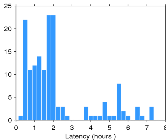
Figure 2. Histogram of the data latency for 28/10/2018. The y-axis denotes the number of files that are made available with a delay of x-hours with respect to the mean time of the records stored in the file.
