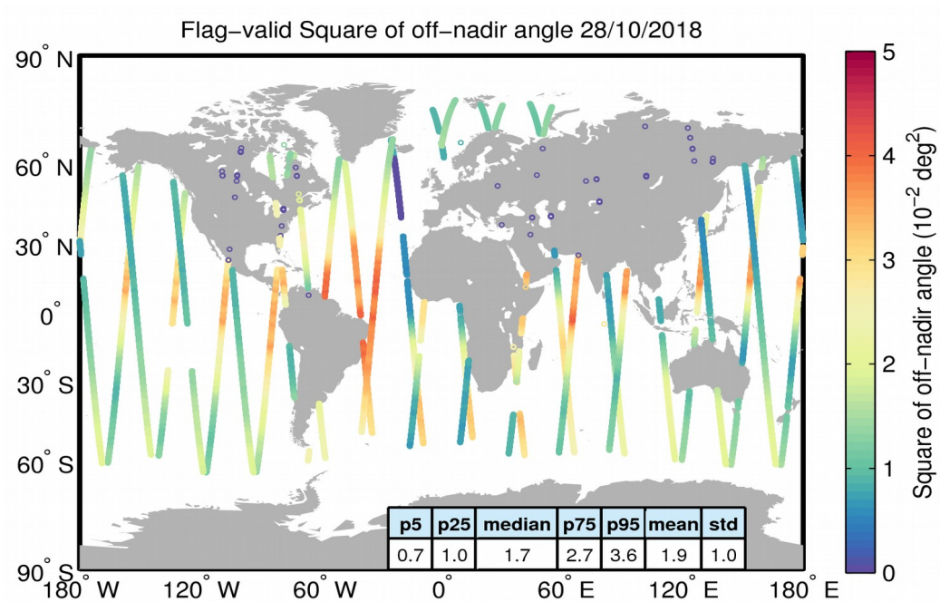
Figure 37. Geographical distribution of flag-valid mispointing data over oceans and lakes for 28/10/2018. The statistical values shown in the table refer to the mispointing in 10^{-2} deg 2 and are calculated over all measurements shown in the figure.
