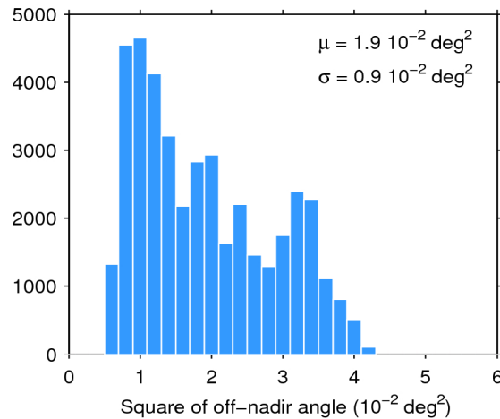
Figure 39. Histogram of flag-valid mispointing over oceans and lakes for 27/10/2018. The mean ( \mu ) and standard deviation ( \sigma ) are also shown. Note that values larger than 6 \cdot 10^{-2} \text{ deg}^2 are excluded from the histogram for the sake of readability but not from the computation of \mu and \sigma .
