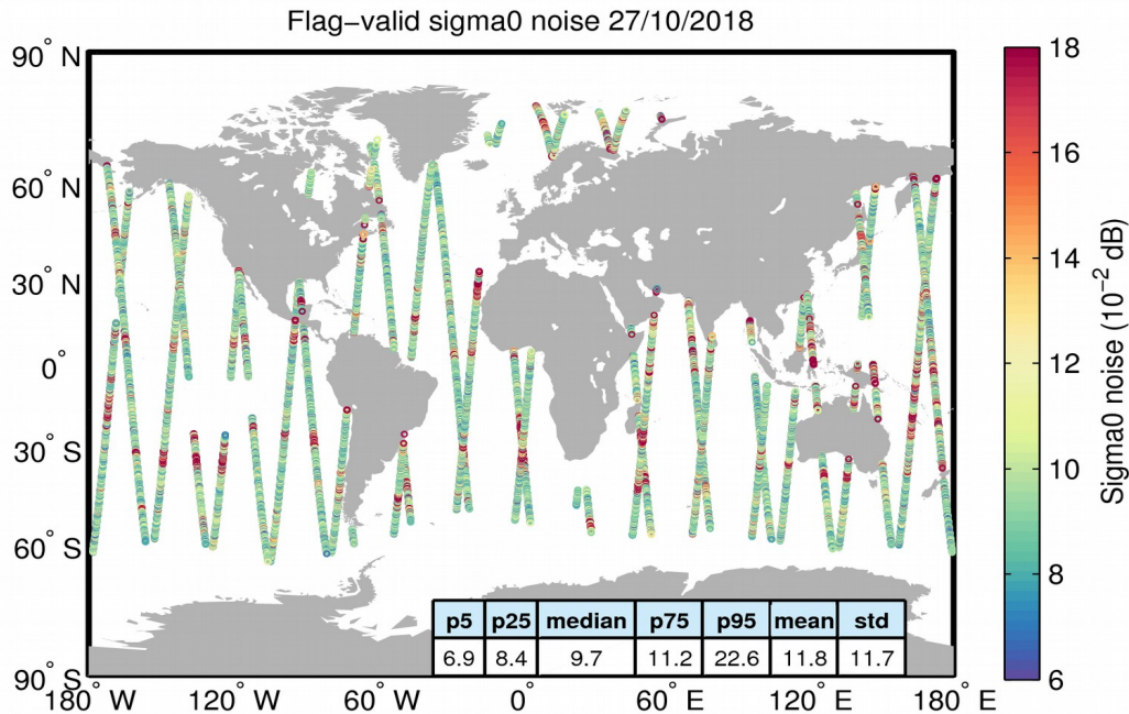
Figure 26. Geographical distribution of flag-valid 20-Hz sigma0 measurement noise over oceans and lakes for 27/10/2018. The statistical values shown in the table refer to the sigma0 noise and are calculated over all measurements shown in the figure.
