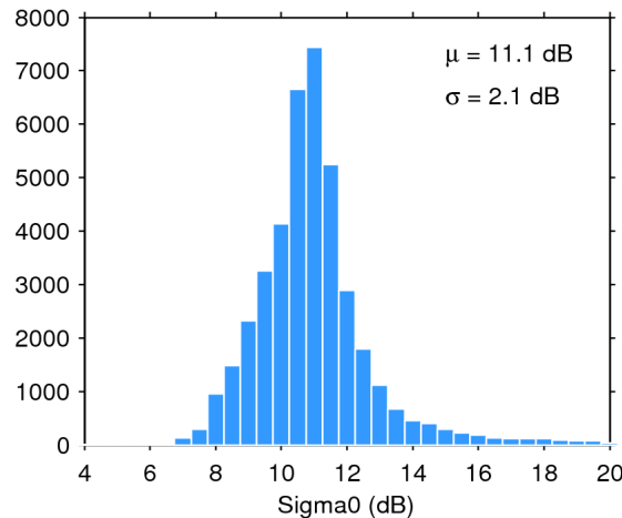
Figure 25. Histogram of flag-valid sigma0 over oceans and lakes for 27/10/2018. The mean ( \mu ) and standard deviation ( \sigma ) are also shown. Note that values outside [4 20] dB are excluded from the histogram for the sake of readability but not from the computation of \mu and \sigma .
