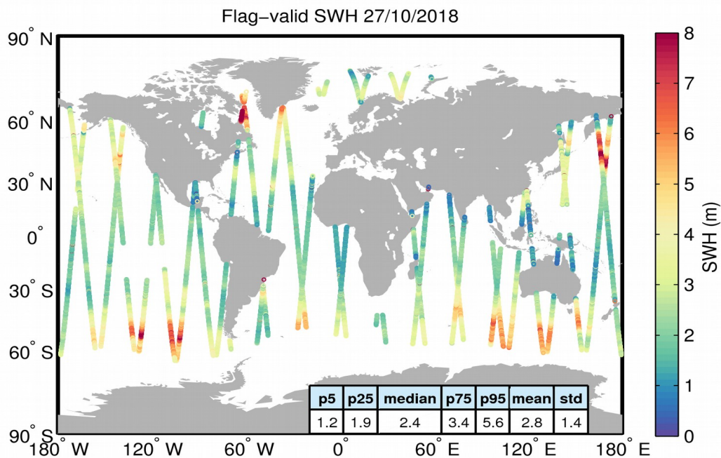
Figure 15. Geographical distribution of flag-valid SWH data over oceans and lakes for 27/10/2018. The statistical values shown in the table refer to the SWH in m and are calculated over all measurements shown in the figure.
