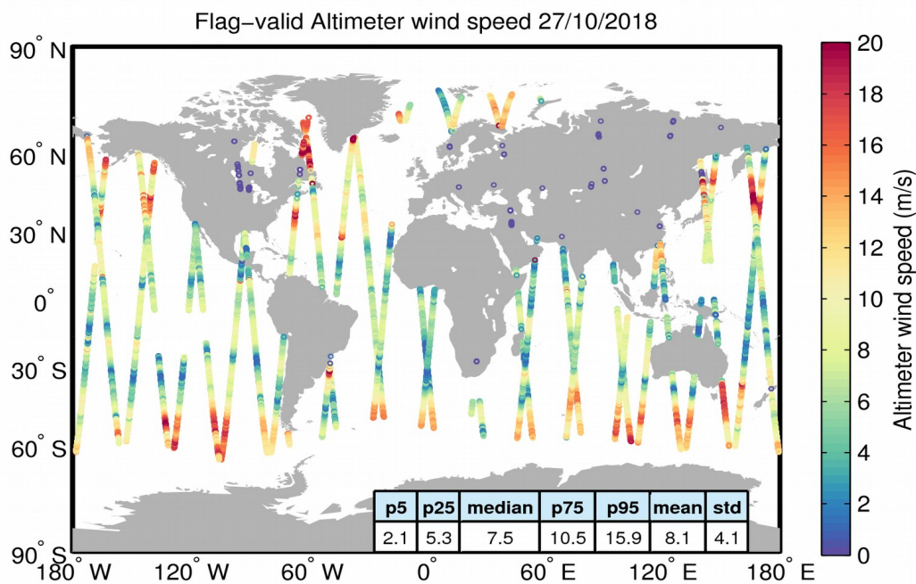
Figure 31. Geographical distribution of flag-valid wind data over oceans and lakes for 27/10/2018. The statistical values shown in the table refer to the wind in m/s and are calculated over all measurements shown in the figure.
