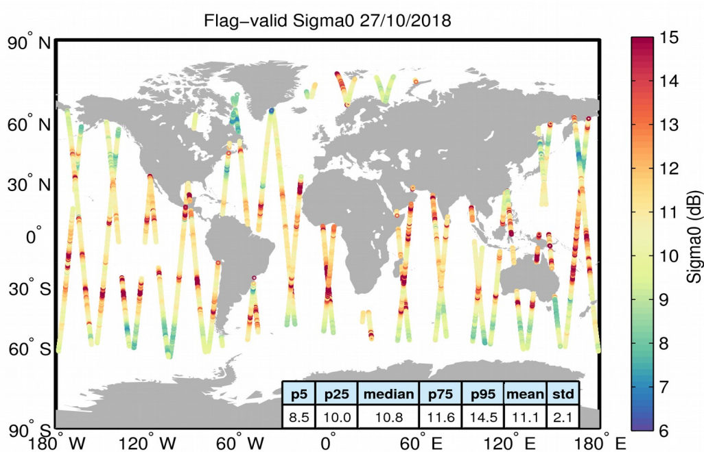
Figure 23. Geographical distribution of flag-valid sigma0 data over oceans and lakes for 27/10/2018. The statistical values shown in the table refer to the sigma0 in dB and are calculated over all measurements shown in the figure.
