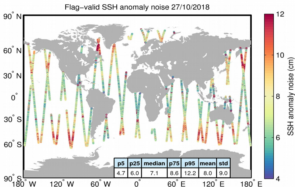
Figure 8. Geographical distribution of flag-valid 20-Hz SSH anomaly measurement noise over oceans and lakes for 27/10/2018. The statistical values shown in the table refer to the SSH anomaly noise and are calculated over all measurements shown in the figure.
