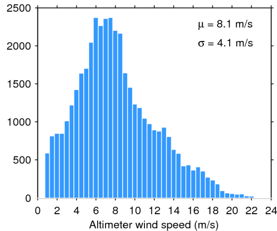
Figure 33. Histogram of flag-valid wind over oceans and lakes for 27/10/2018. The mean ( \mu ) and standard deviation ( \sigma ) are also shown. Note that values larger than 24 m/s are excluded from the histogram for the sake of readability but not from the computation of \mu and \sigma .
