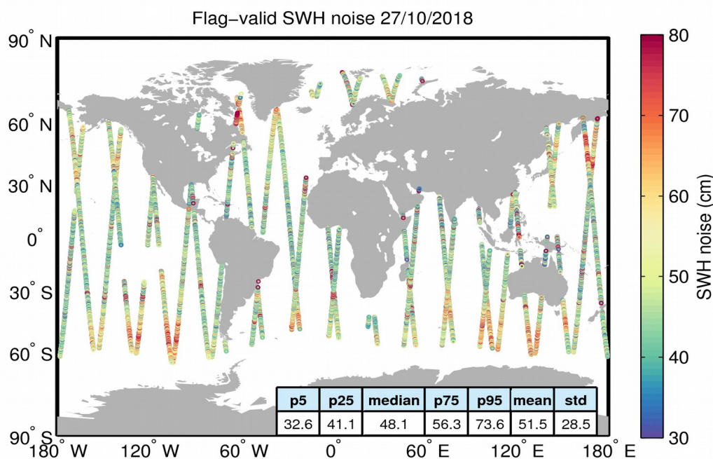
Figure 18. Geographical distribution of flag-valid 20-Hz SWH measurement noise over oceans and lakes for 27/10/2018. The statistical values shown in the figure refer to the SWH noise and are calculated over all measurements shown in the figure.
