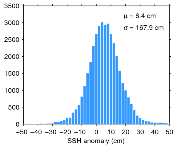
Figure 7. Histogram of flag-valid SSH anomaly over oceans and lakes for 27/10/2018. The mean ( \mu ) and standard deviation ( \sigma ) are also shown. Note that values outside [-50\ 50] cm are excluded from the histogram for the sake of readability but not from the computation of \mu and \sigma .
