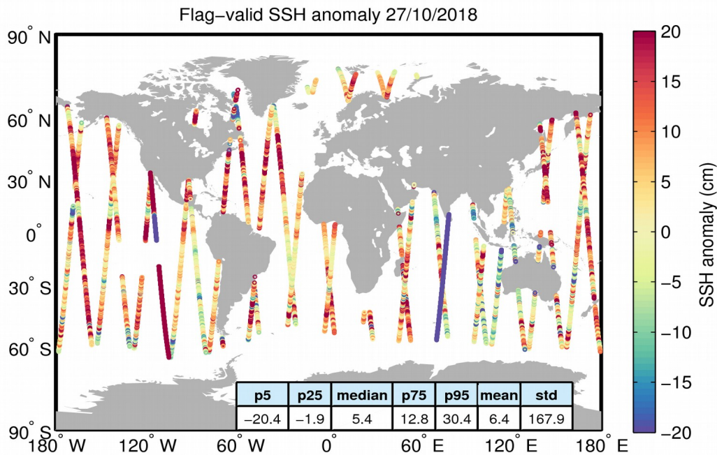
Figure 5. Geographical distribution of flag-valid 1-Hz SSH anomaly data over oceans and lakes for 27/10/2018. The statistical values shown in the table refer to the SSH anomaly in cm and are calculated over all measurements shown in the figure.
