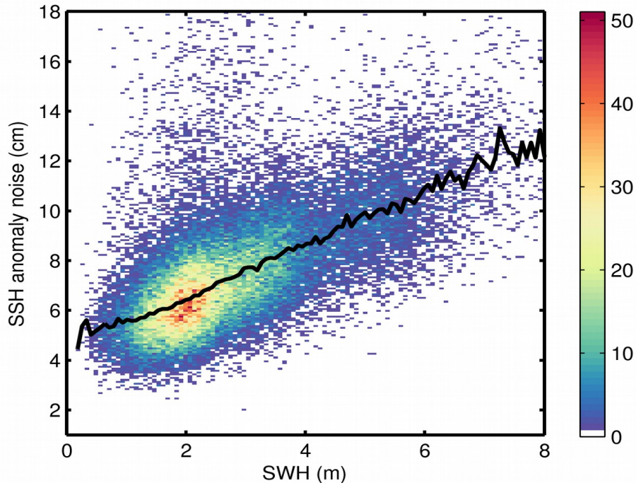
Figure 9. 2D histogram showing flag-valid SSH anomaly noise as a function of SWH for 27/10/2018. The black line denotes the median SSH anomaly noise as a function of SWH.
