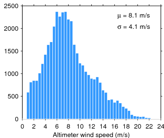
Figure 35. Histogram of science-valid wind over oceans and lakes for 27/10/2018. The mean ( \mu ) and standard deviation ( \sigma ) are also shown. Note that values larger than 24 m/s are excluded from the histogram for the sake of readability but not from the computation of \mu and \sigma .
