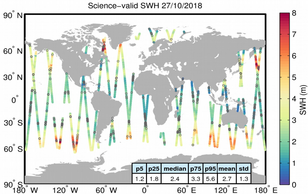
Figure 19. Geographical distribution of science-valid SWH data over oceans and lakes for 27/10/2018. The statistical values shown in the table refer to the SWH in m and are calculated over all measurements shown in the figure. Gray circles denote records that have been rejected based on the editing criteria described in Table 3.
