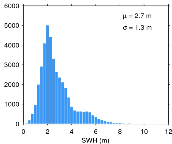
Figure 20. Histogram of science-valid SWH over oceans and lakes for 27/10/2018. The mean ( \mu ) and standard deviation ( \sigma ) are also shown. Note that values larger than 12 m are excluded from the histogram for the sake of readability but not from the computation of \mu and \sigma .
