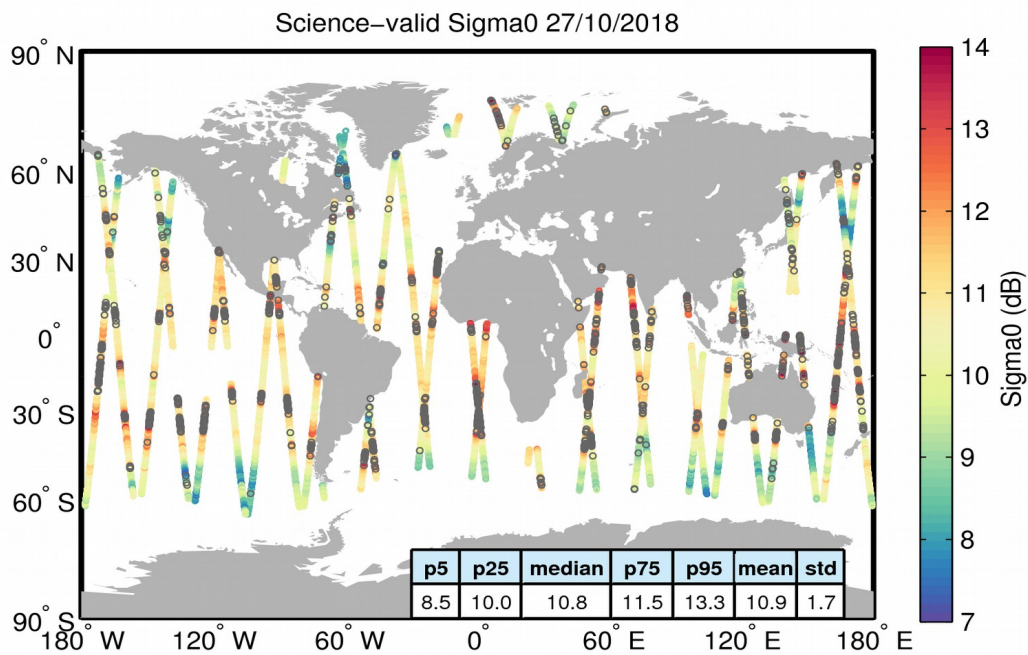
Figure 27. Geographical distribution of science-valid sigma0 data over oceans and lakes for 27/10/2018. The statistical values shown in the table refer to the sigma0 in dB and are calculated over all measurements shown in the figure. Gray circles denote records that have been rejected based on the editing criteria described in Table 4.
