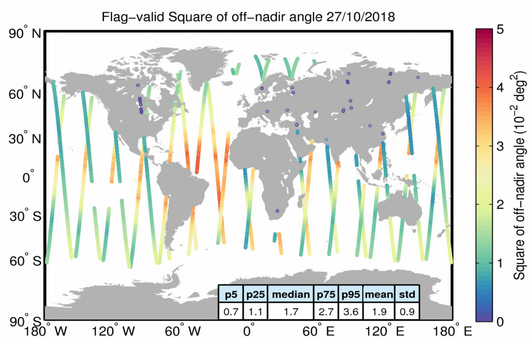
Figure 37. Geographical distribution of flag-valid mispointing data over oceans and lakes for 27/10/2018. The statistical values shown in the table refer to the mispointing in 10^{-2} \text{ deg}^2 and are calculated over all measurements shown in the figure.
