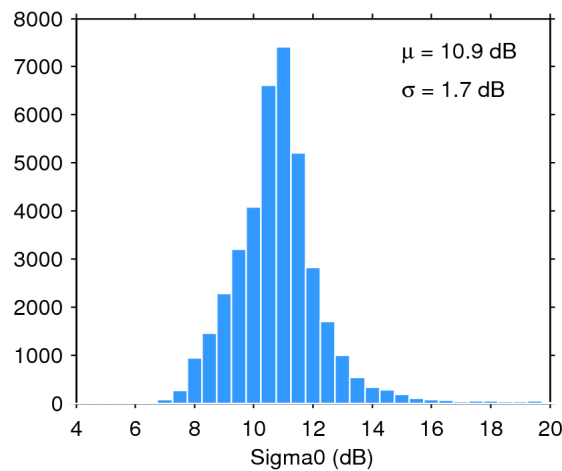
Figure 28. Histogram of science-valid sigma0 over oceans and lakes for 27/10/2018. The mean ( \mu ) and standard deviation ( \sigma ) are also shown. Note that values outside [4 20] dB are excluded from the histogram for the sake of readability but not from the computation of \mu and \sigma .
