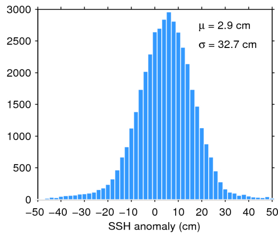
Figure 7. Histogram of flag-valid SSH anomaly over oceans and lakes for 26/10/2018. The mean ( \mu ) and standard deviation ( \sigma ) are also shown. Note that values outside [-50\ 50] cm are excluded from the histogram for the sake of readability but not from the computation of \mu and \sigma .
