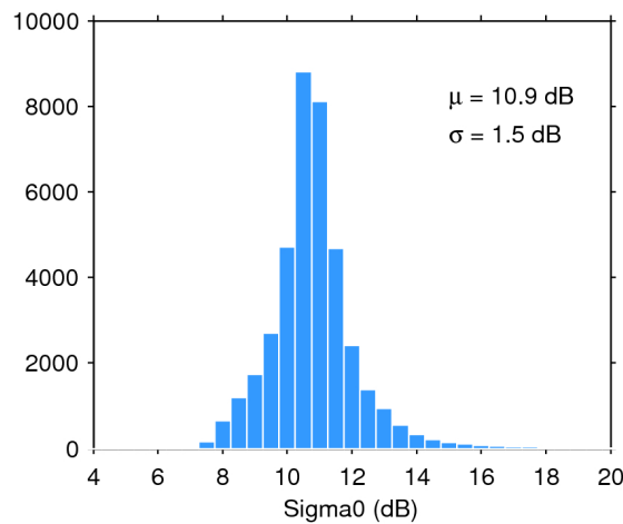
Figure 28. Histogram of science-valid sigma0 over oceans and lakes for 26/10/2018. The mean ( \mu ) and standard deviation ( \sigma ) are also shown. Note that values outside [4 20] dB are excluded from the histogram for the sake of readability but not from the computation of \mu and \sigma .
