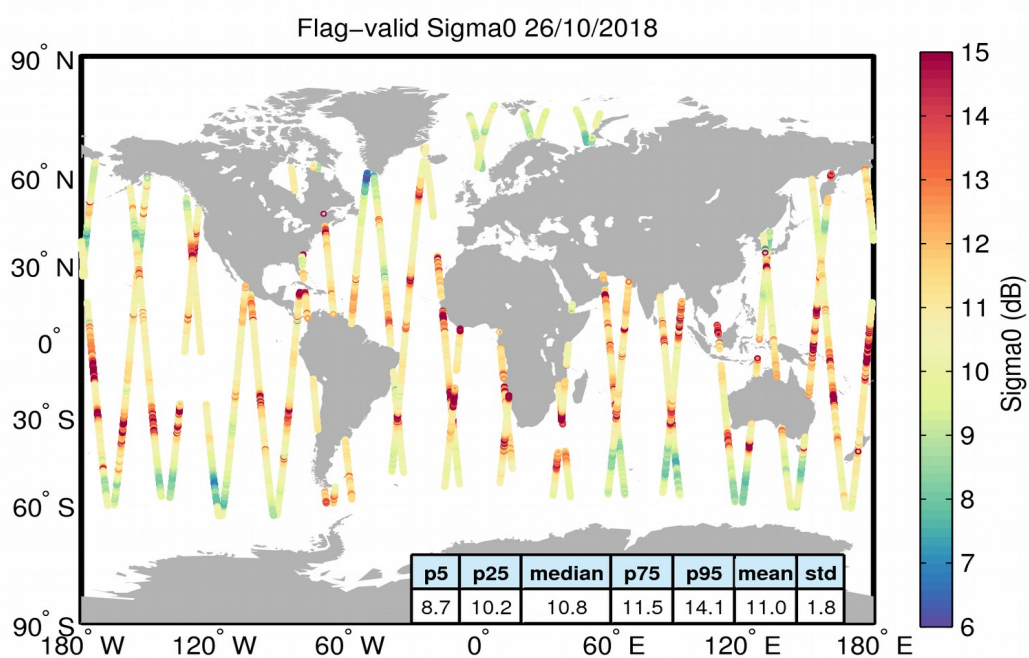
Figure 23. Geographical distribution of flag-valid sigma0 data over oceans and lakes for 26/10/2018. The statistical values shown in the table refer to the sigma0 in dB and are calculated over all measurements shown in the figure.
