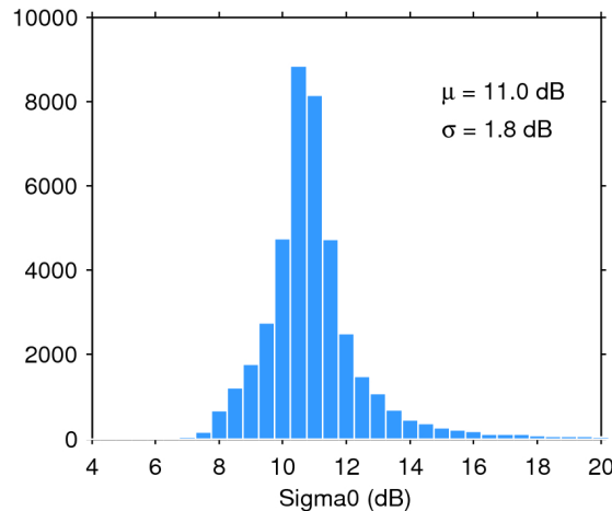
Figure 25. Histogram of flag-valid sigma0 over oceans and lakes for 26/10/2018. The mean ( \mu ) and standard deviation ( \sigma ) are also shown. Note that values outside [4 20] dB are excluded from the histogram for the sake of readability but not from the computation of \mu and \sigma .
