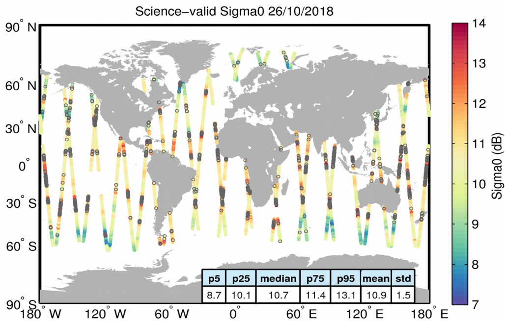
Figure 27. Geographical distribution of science-valid sigma0 data over oceans and lakes for 26/10/2018. The statistical values shown in the table refer to the sigma0 in dB and are calculated over all measurements shown in the figure. Gray circles denote records that have been rejected based on the editing criteria described in Table 4.
