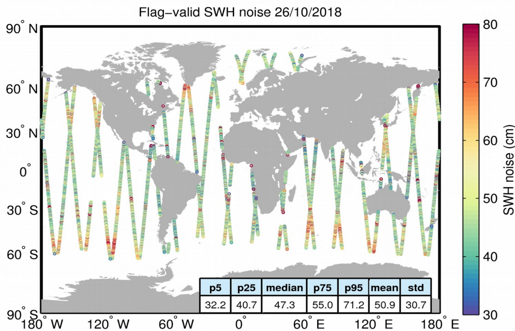
Figure 18. Geographical distribution of flag-valid 20-Hz SWH measurement noise over oceans and lakes for 26/10/2018. The statistical values shown in the figure refer to the SWH noise and are calculated over all measurements shown in the figure.
