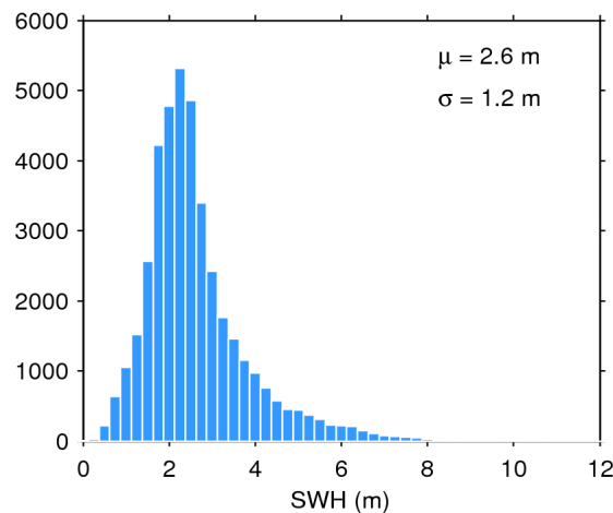
Figure 20. Histogram of science-valid SWH over oceans and lakes for 26/10/2018. The mean ( \mu ) and standard deviation ( \sigma ) are also shown. Note that values larger than 12 m are excluded from the histogram for the sake of readability but not from the computation of \mu and \sigma .
