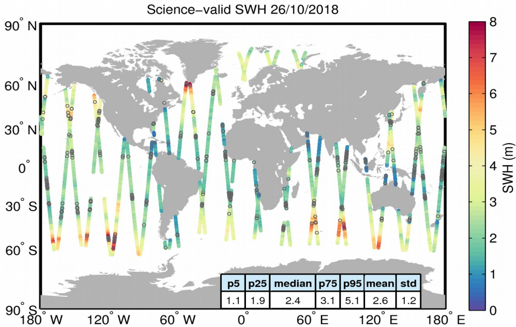
Figure 19. Geographical distribution of science-valid SWH data over oceans and lakes for 26/10/2018. The statistical values shown in the table refer to the SWH in m and are calculated over all measurements shown in the figure. Gray circles denote records that have been rejected based on the editing criteria described in Table 3.
