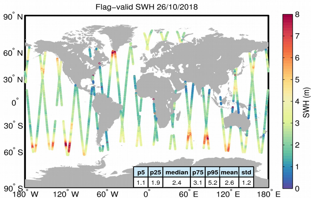
Figure 15. Geographical distribution of flag-valid SWH data over oceans and lakes for 26/10/2018. The statistical values shown in the table refer to the SWH in m and are calculated over all measurements shown in the figure.
