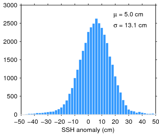
Figure 11. Histogram of science-valid SSH anomaly over oceans and lakes for 26/10/2018. The mean ( \mu ) and standard deviation ( \sigma ) are also shown. Note that values outside [-50 50] cm are excluded from the histogram for the sake of readability but not from the computation of \mu and \sigma .
