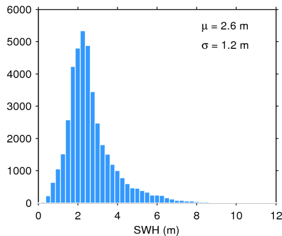
Figure 17. Histogram of flag-valid SWH over oceans and lakes for 26/10/2018. The mean ( \mu ) and standard deviation ( \sigma ) are also shown. Note that values larger than 12 m are excluded from the histogram for the sake of readability but not from the computation of \mu and \sigma .
