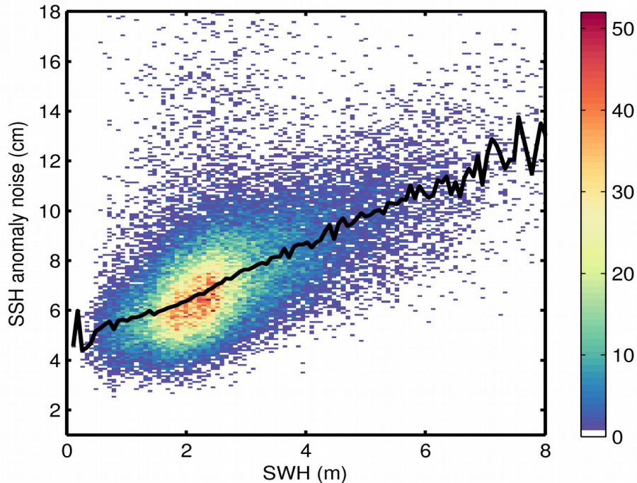
Figure 9. 2D histogram showing flag-valid SSH anomaly noise as a function of SWH for 26/10/2018. The black line denotes the median SSH anomaly noise as a function of SWH.
