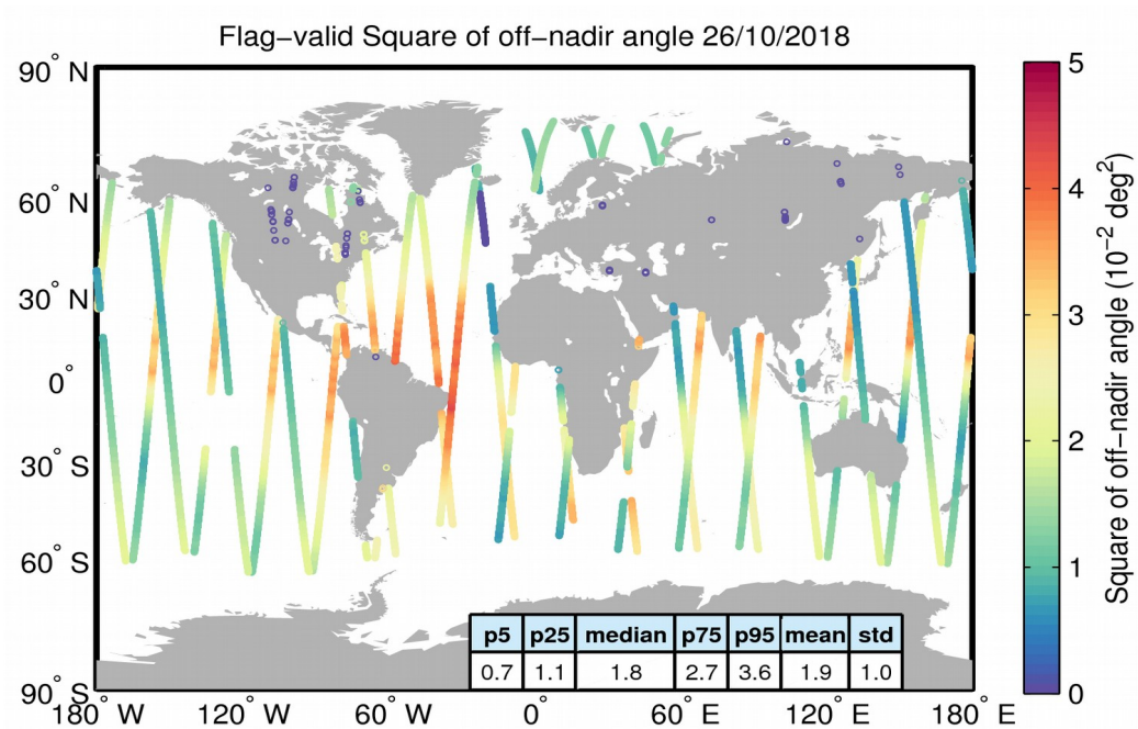
Figure 37. Geographical distribution of flag-valid mispointing data over oceans and lakes for 26/10/2018. The statistical values shown in the table refer to the mispointing in 10^{-2} deg 2 and are calculated over all measurements shown in the figure.
