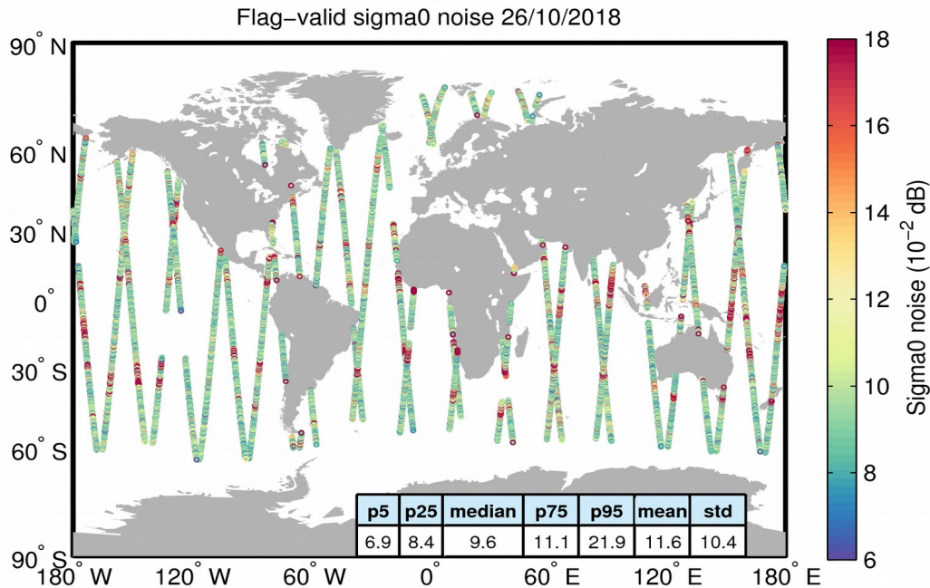
Figure 26. Geographical distribution of flag-valid 20-Hz sigma0 measurement noise over oceans and lakes for 26/10/2018. The statistical values shown in the table refer to the sigma0 noise and are calculated over all measurements shown in the figure.
