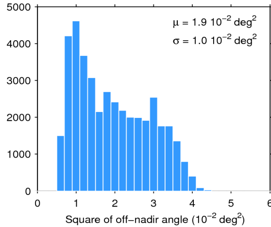
Figure 39. Histogram of flag-valid mispointing over oceans and lakes for 26/10/2018. The mean ( \mu ) and standard deviation ( \sigma ) are also shown. Note that values larger than 6 \cdot 10^{-2} \text{ deg}^2 are excluded from the histogram for the sake of readability but not from the computation of \mu and \sigma .
