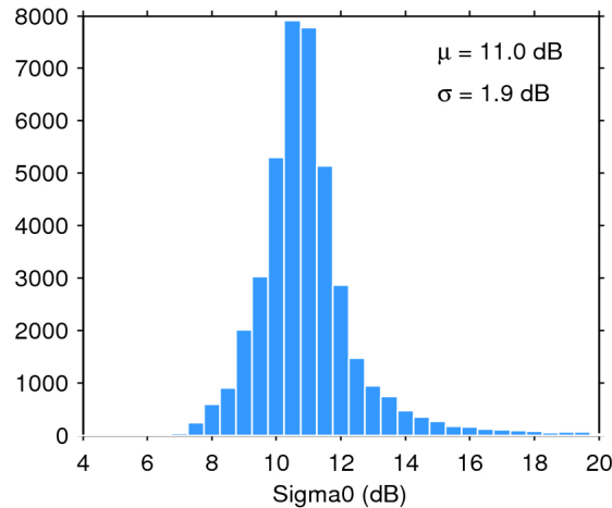
Figure 25. Histogram of flag-valid sigma0 over oceans and lakes for 25/10/2018. The mean ( \mu ) and standard deviation ( \sigma ) are also shown. Note that values outside [4 20] dB are excluded from the histogram for the sake of readability but not from the computation of \mu and \sigma .
