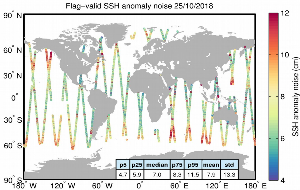
Figure 8. Geographical distribution of flag-valid 20-Hz SSH anomaly measurement noise over oceans and lakes for 25/10/2018. The statistical values shown in the table refer to the SSH anomaly noise and are calculated over all measurements shown in the figure.
