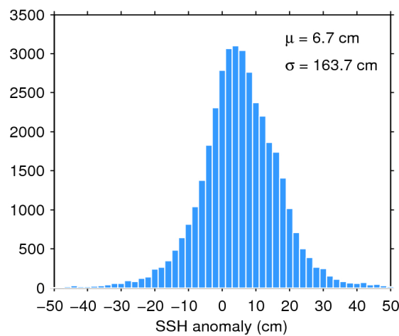
Figure 7. Histogram of flag-valid SSH anomaly over oceans and lakes for 25/10/2018. The mean ( \mu ) and standard deviation ( \sigma ) are also shown. Note that values outside [-50 50] cm are excluded from the histogram for the sake of readability but not from the computation of \mu and \sigma .
