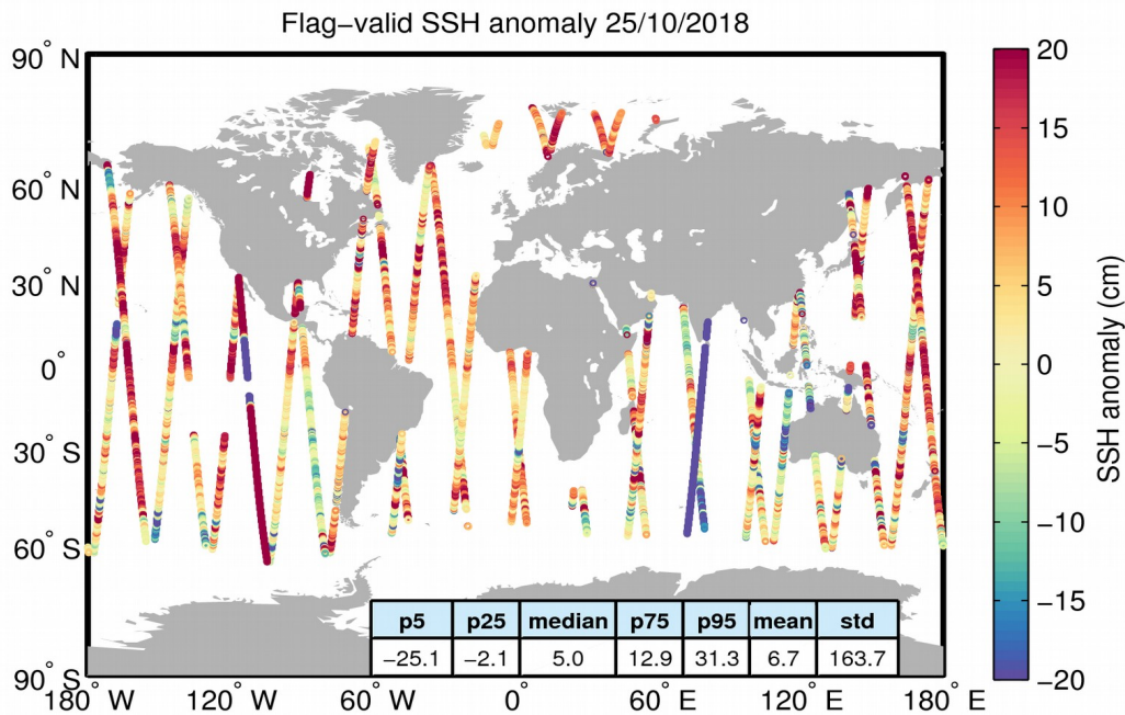
Figure 5. Geographical distribution of flag-valid 1-Hz SSH anomaly data over oceans and lakes for 25/10/2018. The statistical values shown in the table refer to the SSH anomaly in cm and are calculated over all measurements shown in the figure.
