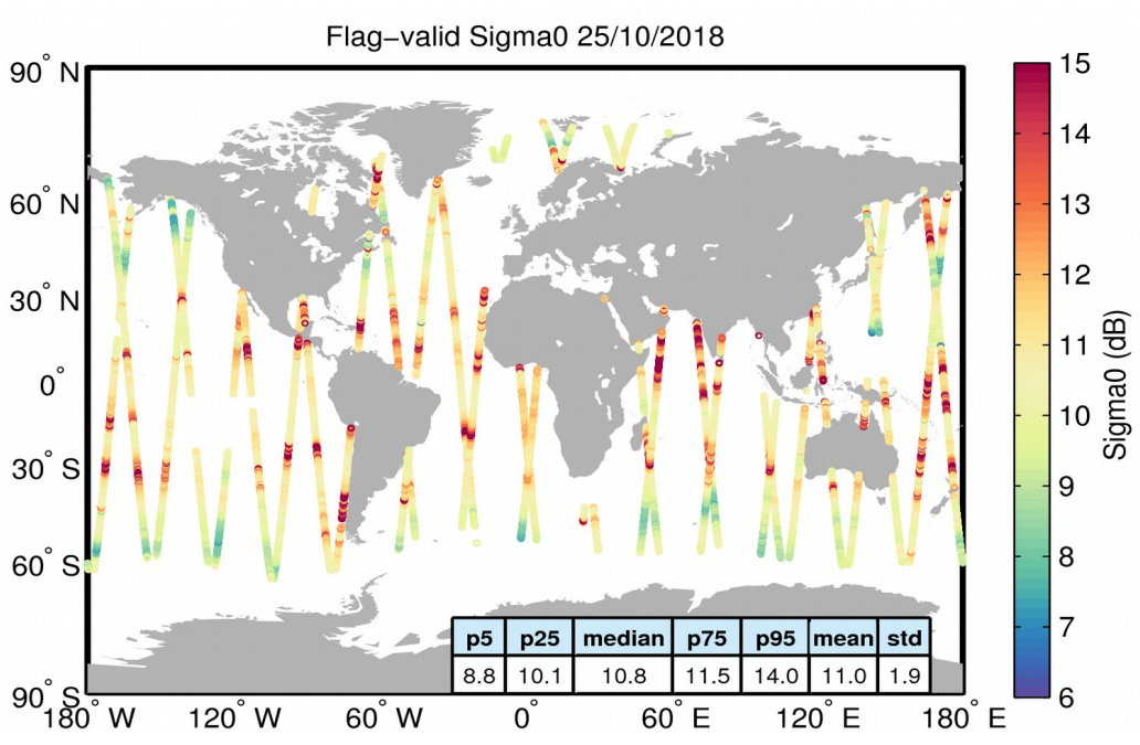
Figure 23. Geographical distribution of flag-valid sigma0 data over oceans and lakes for 25/10/2018. The statistical values shown in the table refer to the sigma0 in dB and are calculated over all measurements shown in the figure.
