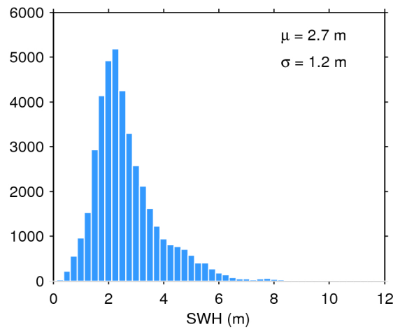
Figure 17. Histogram of flag-valid SWH over oceans and lakes for 25/10/2018. The mean ( \mu ) and standard deviation ( \sigma ) are also shown. Note that values larger than 12 m are excluded from the histogram for the sake of readability but not from the computation of \mu and \sigma .
