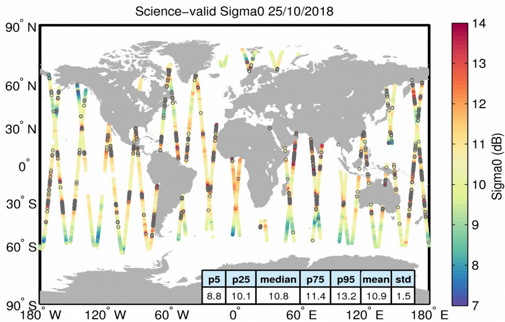
Figure 27. Geographical distribution of science-valid sigma0 data over oceans and lakes for 25/10/2018. The statistical values shown in the table refer to the sigma0 in dB and are calculated over all measurements shown in the figure. Gray circles denote records that have been rejected based on the editing criteria described in Table 4.
