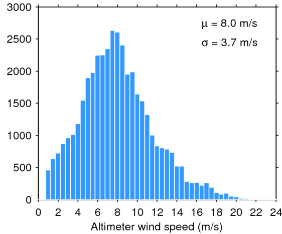
Figure 33. Histogram of flag-valid wind over oceans and lakes for 25/10/2018. The mean ( \mu ) and standard deviation ( \sigma ) are also shown. Note that values larger than 24 m/s are excluded from the histogram for the sake of readability but not from the computation of \mu and \sigma .
