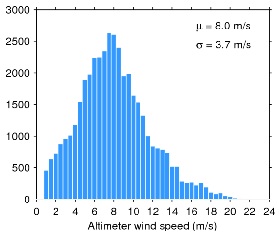
Figure 35. Histogram of science-valid wind over oceans and lakes for 25/10/2018. The mean ( \mu ) and standard deviation ( \sigma ) are also shown. Note that values larger than 24 m/s are excluded from the histogram for the sake of readability but not from the computation of \mu and \sigma .
