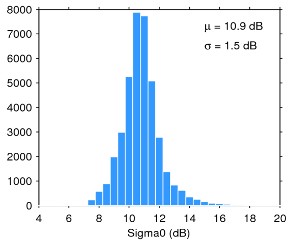
Figure 28. Histogram of science-valid sigma0 over oceans and lakes for 25/10/2018. The mean ( \mu ) and standard deviation ( \sigma ) are also shown. Note that values outside [4 20] dB are excluded from the histogram for the sake of readability but not from the computation of \mu and \sigma .
