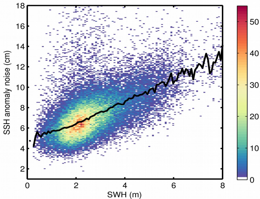
Figure 9. 2D histogram showing flag-valid SSH anomaly noise as a function of SWH for 25/10/2018. The black line denotes the median SSH anomaly noise as a function of SWH.
