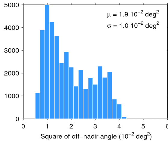
Figure 39. Histogram of flag-valid mispointing over oceans and lakes for 25/10/2018. The mean ( \mu ) and standard deviation ( \sigma ) are also shown. Note that values larger than 6 \cdot 10^{-2} \text{ deg}^2 are excluded from the histogram for the sake of readability but not from the computation of \mu and \sigma .
