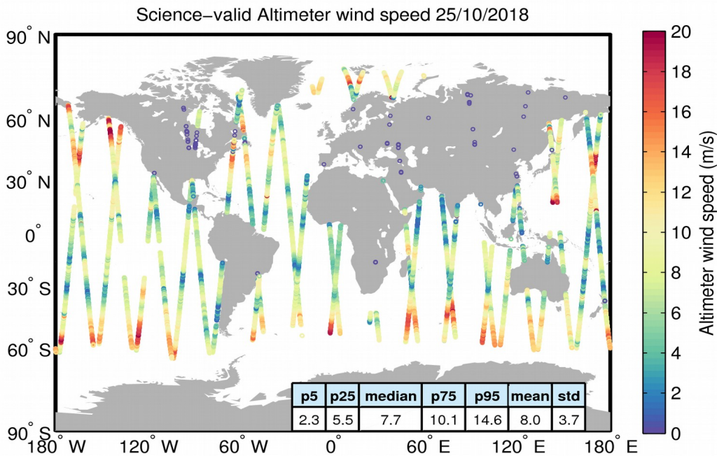
Figure 34. Geographical distribution of science-valid wind data over oceans and lakes for 25/10/2018. The statistical values shown in the table refer to the wind in m/s and are calculated over all measurements shown in the figure. Gray circles denote records that have been rejected based on the editing criteria described in Table 5.
