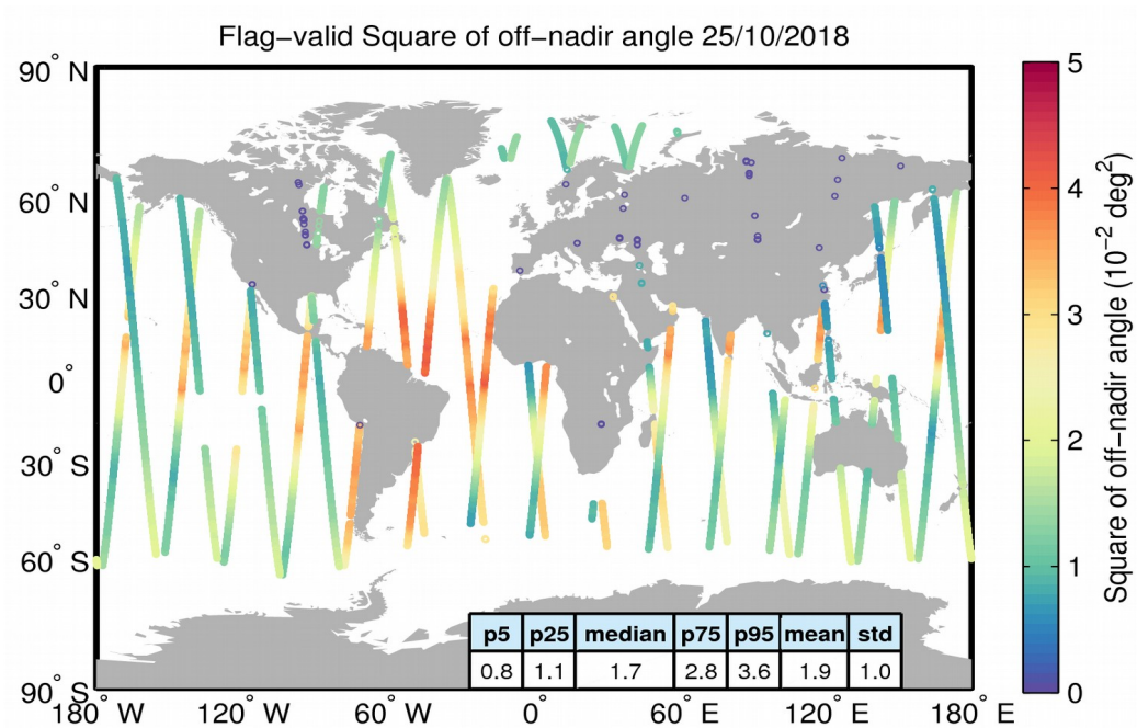
Figure 37. Geographical distribution of flag-valid mispointing data over oceans and lakes for 25/10/2018. The statistical values shown in the table refer to the mispointing in 10^{-2} deg 2 and are calculated over all measurements shown in the figure.
