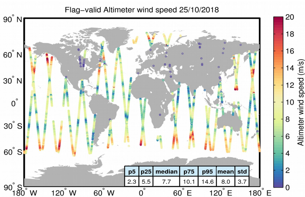
Figure 31. Geographical distribution of flag-valid wind data over oceans and lakes for 25/10/2018. The statistical values shown in the table refer to the wind in m/s and are calculated over all measurements shown in the figure.
