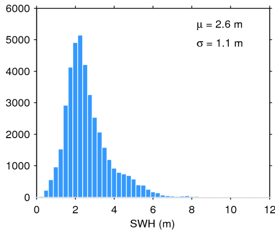
Figure 20. Histogram of science-valid SWH over oceans and lakes for 25/10/2018. The mean ( \mu ) and standard deviation ( \sigma ) are also shown. Note that values larger than 12 m are excluded from the histogram for the sake of readability but not from the computation of \mu and \sigma .
