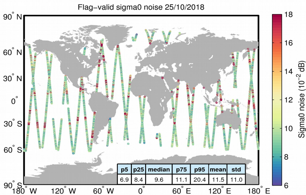
Figure 26. Geographical distribution of flag-valid 20-Hz sigma0 measurement noise over oceans and lakes for 25/10/2018. The statistical values shown in the table refer to the sigma0 noise and are calculated over all measurements shown in the figure.
