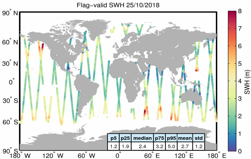
Figure 15. Geographical distribution of flag-valid SWH data over oceans and lakes for 25/10/2018. The statistical values shown in the table refer to the SWH in m and are calculated over all measurements shown in the figure.
