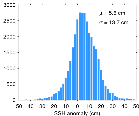
Figure 11. Histogram of science-valid SSH anomaly over oceans and lakes for 25/10/2018. The mean ( \mu ) and standard deviation ( \sigma ) are also shown. Note that values outside [-50 50] cm are excluded from the histogram for the sake of readability but not from the computation of \mu and \sigma .
