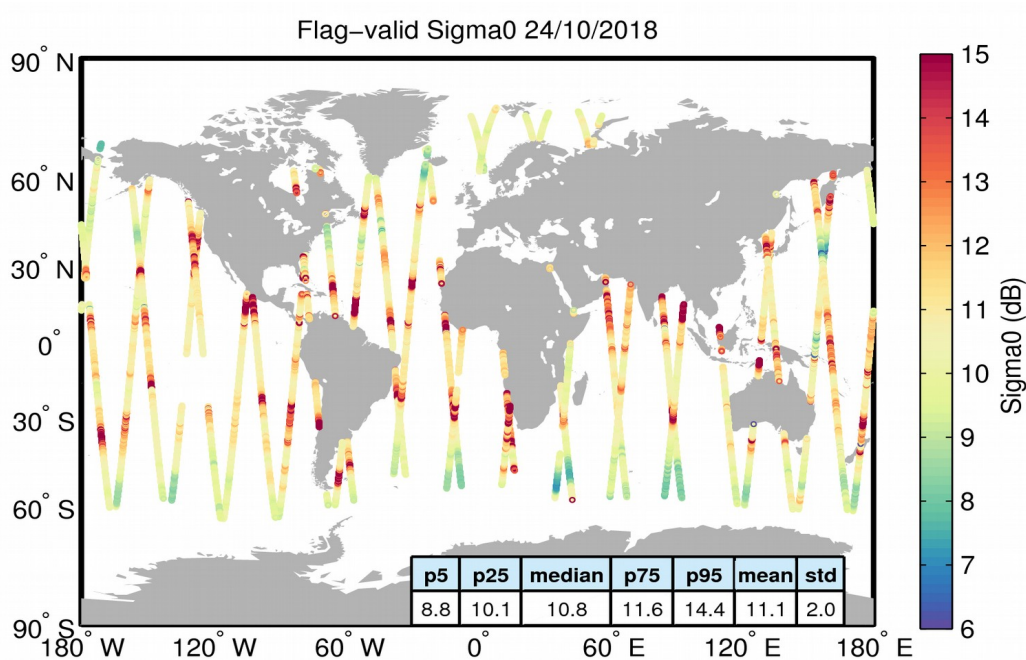
Figure 23. Geographical distribution of flag-valid sigma0 data over oceans and lakes for 24/10/2018. The statistical values shown in the table refer to the sigma0 in dB and are calculated over all measurements shown in the figure.
