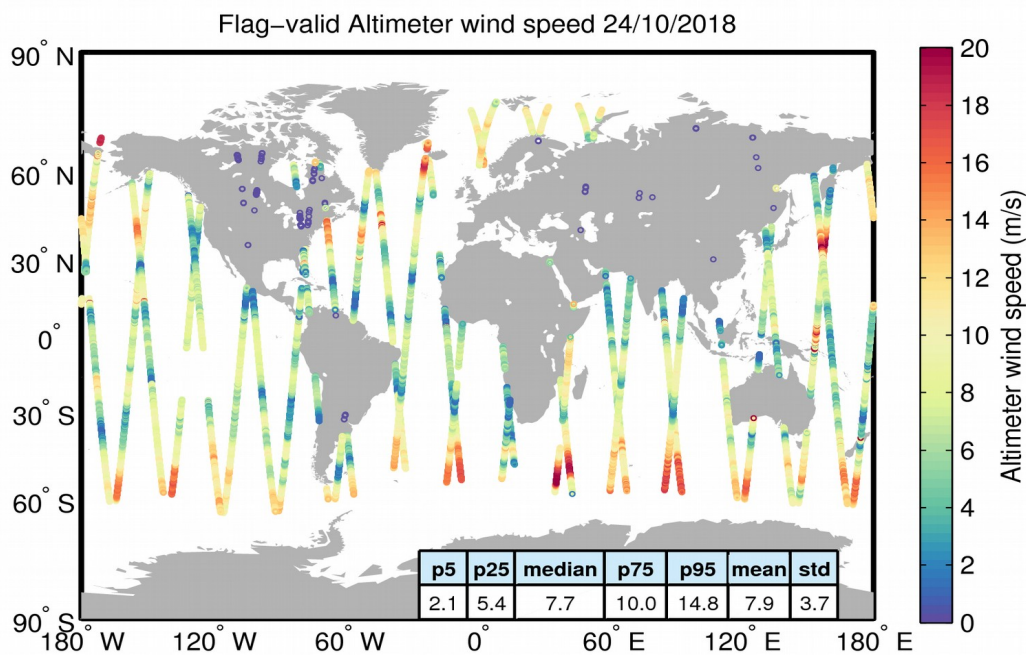
Figure 31. Geographical distribution of flag-valid wind data over oceans and lakes for 24/10/2018. The statistical values shown in the table refer to the wind in m/s and are calculated over all measurements shown in the figure.
