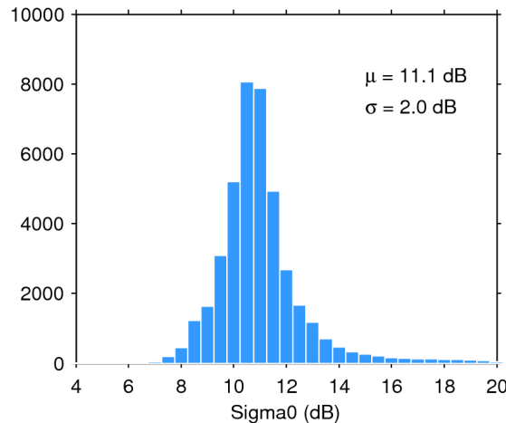
Figure 25. Histogram of flag-valid sigma0 over oceans and lakes for 24/10/2018. The mean ( \mu ) and standard deviation ( \sigma ) are also shown. Note that values outside [4 20] dB are excluded from the histogram for the sake of readability but not from the computation of \mu and \sigma .
