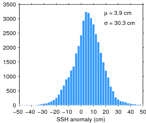
Figure 7. Histogram of flag-valid SSH anomaly over oceans and lakes for 24/10/2018. The mean ( \mu ) and standard deviation ( \sigma ) are also shown. Note that values outside [-50 50] cm are excluded from the histogram for the sake of readability but not from the computation of \mu and \sigma .
