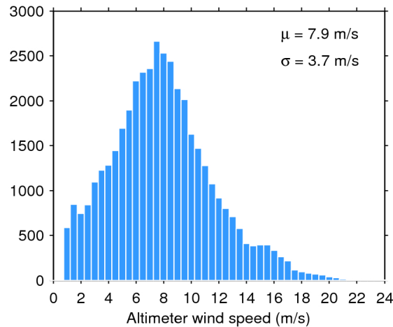
Figure 33. Histogram of flag-valid wind over oceans and lakes for 24/10/2018. The mean ( \mu ) and standard deviation ( \sigma ) are also shown. Note that values larger than 24 m/s are excluded from the histogram for the sake of readability but not from the computation of \mu and \sigma .
