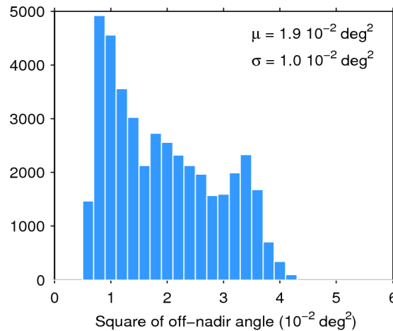
Figure 39. Histogram of flag-valid mispointing over oceans and lakes for 24/10/2018. The mean ( \mu ) and standard deviation ( \sigma ) are also shown. Note that values larger than 6 \cdot 10^{-2} \text{ deg}^2 are excluded from the histogram for the sake of readability but not from the computation of \mu and \sigma .
