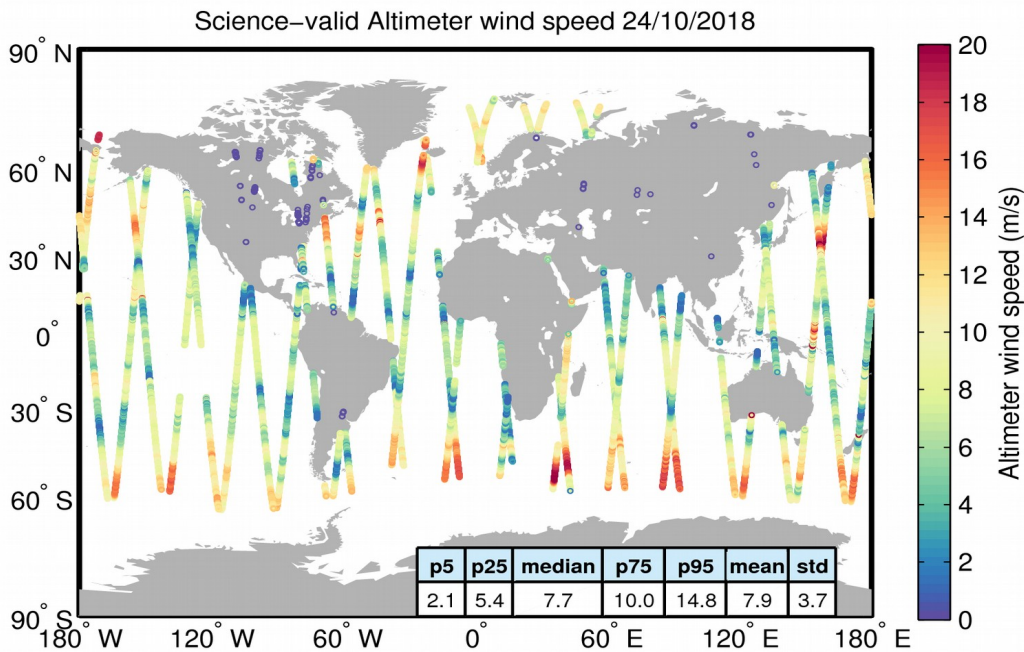
Figure 34. Geographical distribution of science-valid wind data over oceans and lakes for 24/10/2018. The statistical values shown in the table refer to the wind in m/s and are calculated over all measurements shown in the figure. Gray circles denote records that have been rejected based on the editing criteria described in Table 5.
