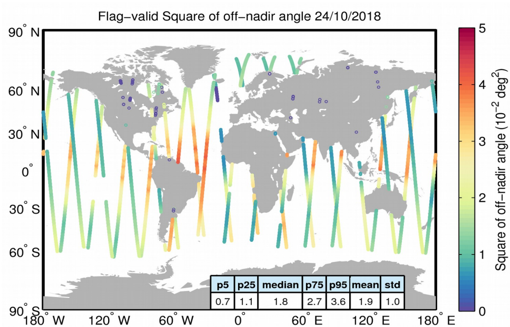
Figure 37. Geographical distribution of flag-valid mispointing data over oceans and lakes for 24/10/2018. The statistical values shown in the table refer to the mispointing in 10^{-2} deg 2 and are calculated over all measurements shown in the figure.
