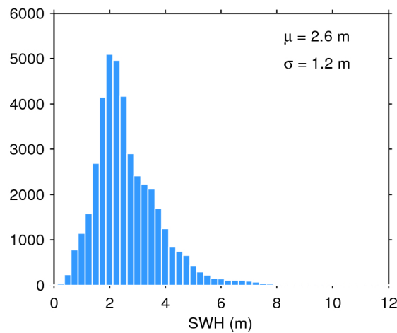
Figure 17. Histogram of flag-valid SWH over oceans and lakes for 24/10/2018. The mean ( \mu ) and standard deviation ( \sigma ) are also shown. Note that values larger than 12 m are excluded from the histogram for the sake of readability but not from the computation of \mu and \sigma .
