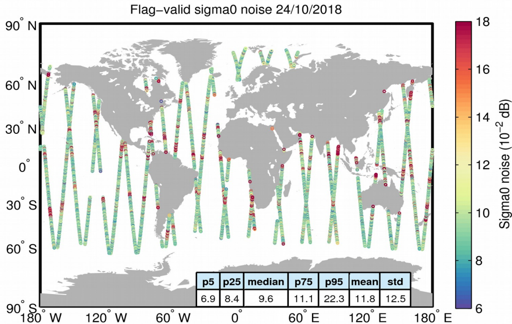
Figure 26. Geographical distribution of flag-valid 20-Hz sigma0 measurement noise over oceans and lakes for 24/10/2018. The statistical values shown in the table refer to the sigma0 noise and are calculated over all measurements shown in the figure.
