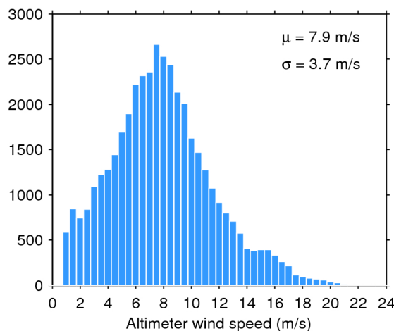
Figure 35. Histogram of science-valid wind over oceans and lakes for 24/10/2018. The mean ( \mu ) and standard deviation ( \sigma ) are also shown. Note that values larger than 24 m/s are excluded from the histogram for the sake of readability but not from the computation of \mu and \sigma .
