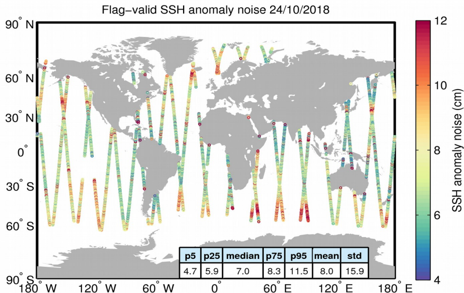
Figure 8. Geographical distribution of flag-valid 20-Hz SSH anomaly measurement noise over oceans and lakes for 24/10/2018. The statistical values shown in the table refer to the SSH anomaly noise and are calculated over all measurements shown in the figure.
