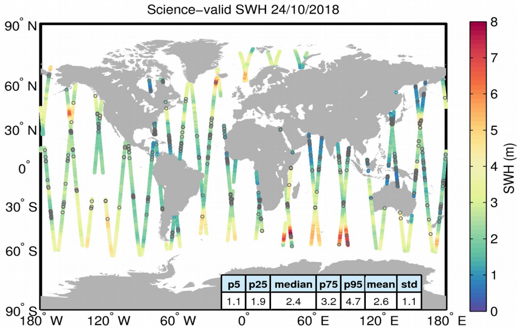
Figure 19. Geographical distribution of science-valid SWH data over oceans and lakes for 24/10/2018. The statistical values shown in the table refer to the SWH in m and are calculated over all measurements shown in the figure. Gray circles denote records that have been rejected based on the editing criteria described in Table 3.
