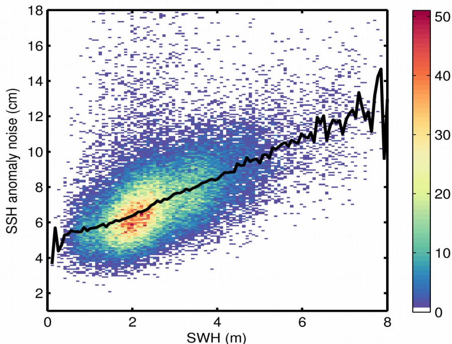
Figure 9. 2D histogram showing flag-valid SSH anomaly noise as a function of SWH for 24/10/2018. The black line denotes the median SSH anomaly noise as a function of SWH.
