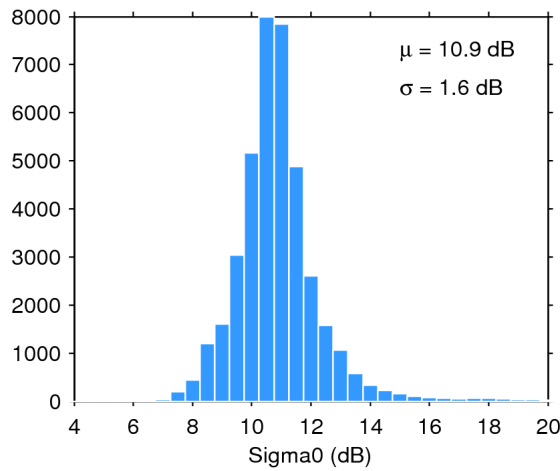
Figure 28. Histogram of science-valid sigma0 over oceans and lakes for 24/10/2018. The mean ( \mu ) and standard deviation ( \sigma ) are also shown. Note that values outside [4 20] dB are excluded from the histogram for the sake of readability but not from the computation of \mu and \sigma .
