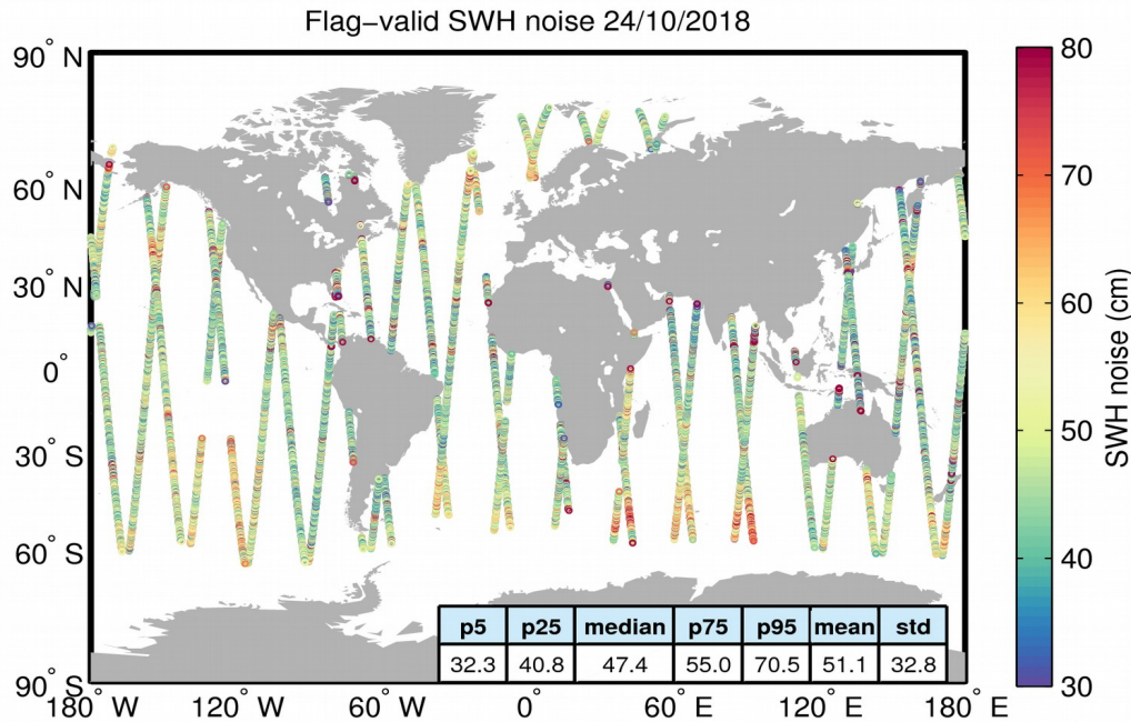
Figure 18. Geographical distribution of flag-valid 20-Hz SWH measurement noise over oceans and lakes for 24/10/2018. The statistical values shown in the figure refer to the SWH noise and are calculated over all measurements shown in the figure.
