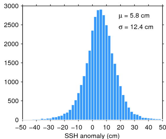
Figure 11. Histogram of science-valid SSH anomaly over oceans and lakes for 23/10/2018. The mean ( \mu ) and standard deviation ( \sigma ) are also shown. Note that values outside [-50 50] cm are excluded from the histogram for the sake of readability but not from the computation of \mu and \sigma .
