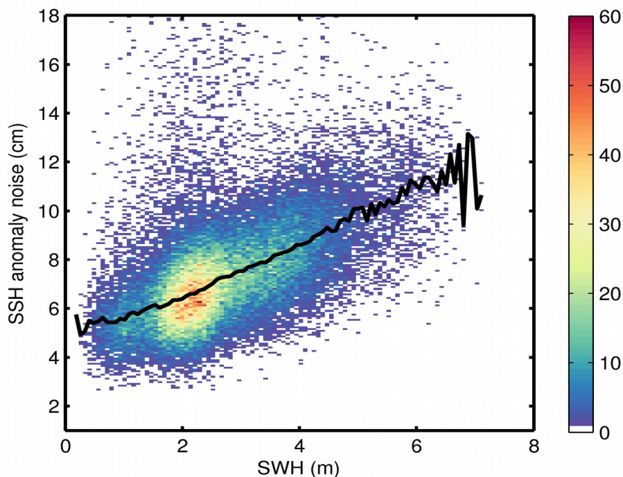
Figure 9. 2D histogram showing flag-valid SSH anomaly noise as a function of SWH for 23/10/2018. The black line denotes the median SSH anomaly noise as a function of SWH.
