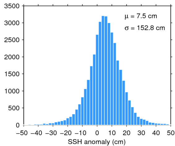
Figure 7. Histogram of flag-valid SSH anomaly over oceans and lakes for 23/10/2018. The mean ( \mu ) and standard deviation ( \sigma ) are also shown. Note that values outside [-50 50] cm are excluded from the histogram for the sake of readability but not from the computation of \mu and \sigma .
