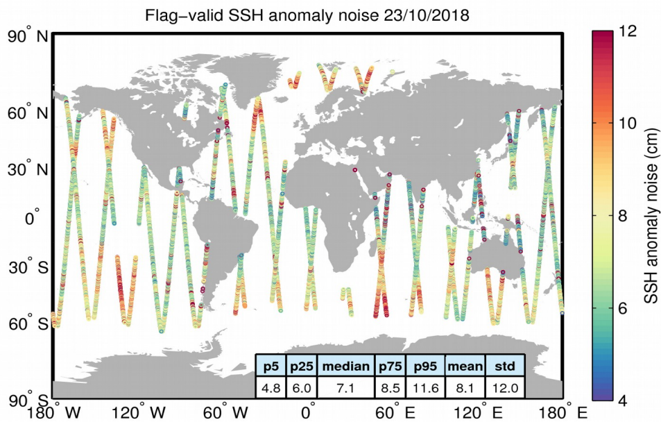
Figure 8. Geographical distribution of flag-valid 20-Hz SSH anomaly measurement noise over oceans and lakes for 23/10/2018. The statistical values shown in the table refer to the SSH anomaly noise and are calculated over all measurements shown in the figure.
