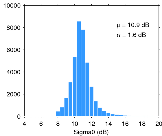
Figure 28. Histogram of science-valid sigma0 over oceans and lakes for 23/10/2018. The mean ( \mu ) and standard deviation ( \sigma ) are also shown. Note that values outside [4 20] dB are excluded from the histogram for the sake of readability but not from the computation of \mu and \sigma .
