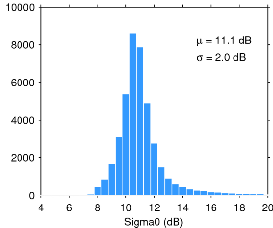
Figure 25. Histogram of flag-valid sigma0 over oceans and lakes for 23/10/2018. The mean ( \mu ) and standard deviation ( \sigma ) are also shown. Note that values outside [4 20] dB are excluded from the histogram for the sake of readability but not from the computation of \mu and \sigma .
