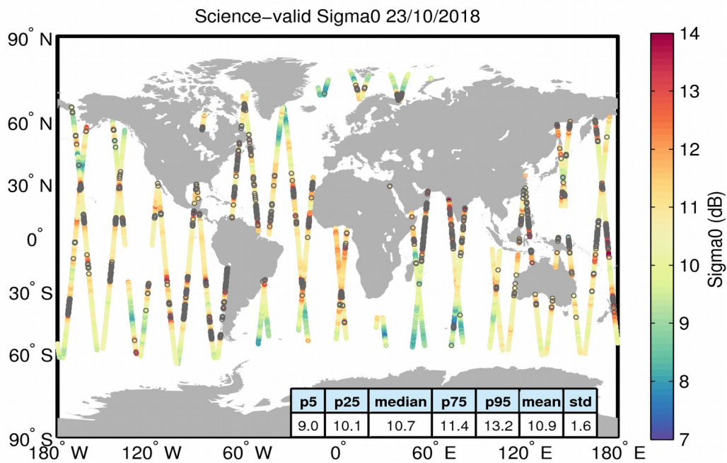
Figure 27. Geographical distribution of science-valid sigma0 data over oceans and lakes for 23/10/2018. The statistical values shown in the table refer to the sigma0 in dB and are calculated over all measurements shown in the figure. Gray circles denote records that have been rejected based on the editing criteria described in Table 4.
