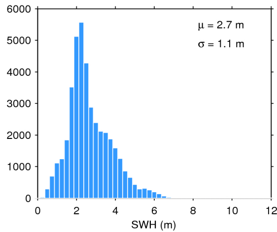
Figure 17. Histogram of flag-valid SWH over oceans and lakes for 23/10/2018. The mean ( \mu ) and standard deviation ( \sigma ) are also shown. Note that values larger than 12 m are excluded from the histogram for the sake of readability but not from the computation of \mu and \sigma .
