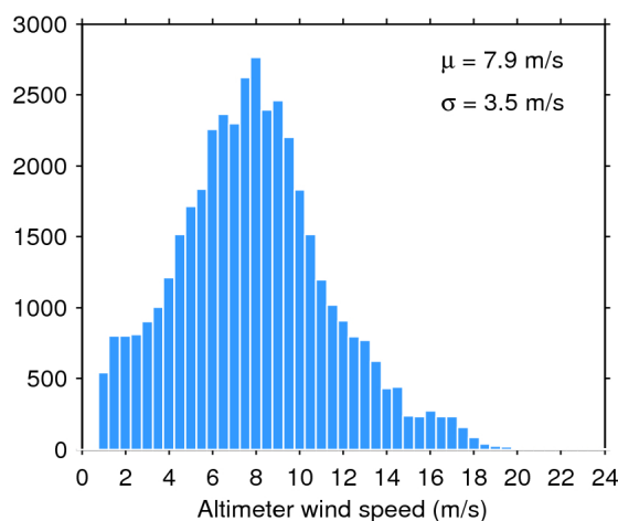
Figure 35. Histogram of science-valid wind over oceans and lakes for 23/10/2018. The mean ( \mu ) and standard deviation ( \sigma ) are also shown. Note that values larger than 24 m/s are excluded from the histogram for the sake of readability but not from the computation of \mu and \sigma .
