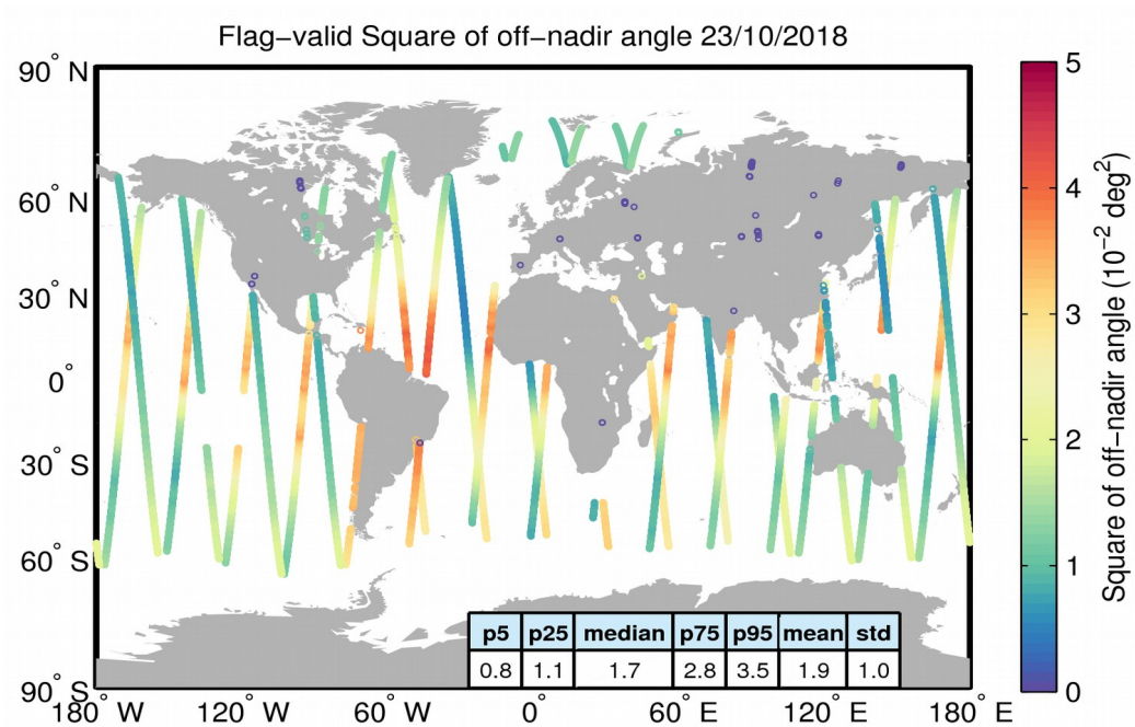
Figure 37. Geographical distribution of flag-valid mispointing data over oceans and lakes for 23/10/2018. The statistical values shown in the table refer to the mispointing in 10^{-2} \text{deg}^2 and are calculated over all measurements shown in the figure.
