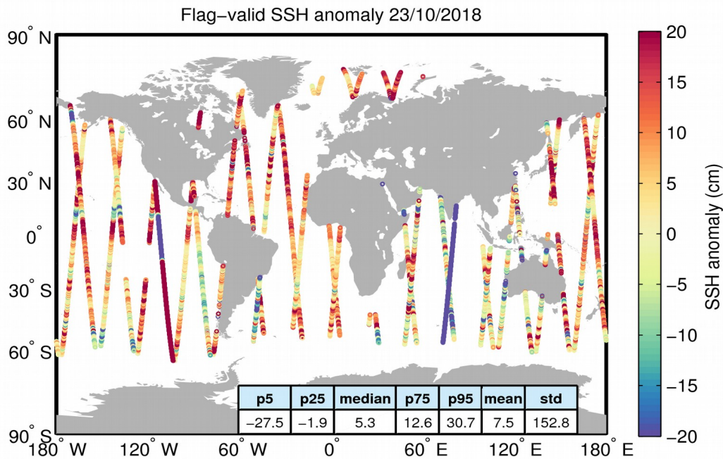
Figure 5. Geographical distribution of flag-valid 1-Hz SSH anomaly data over oceans and lakes for 23/10/2018. The statistical values shown in the table refer to the SSH anomaly in cm and are calculated over all measurements shown in the figure.
