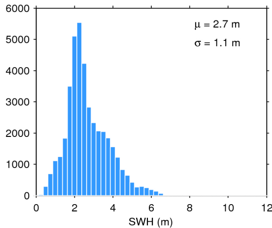
Figure 20. Histogram of science-valid SWH over oceans and lakes for 23/10/2018. The mean ( \mu ) and standard deviation ( \sigma ) are also shown. Note that values larger than 12 m are excluded from the histogram for the sake of readability but not from the computation of \mu and \sigma .
