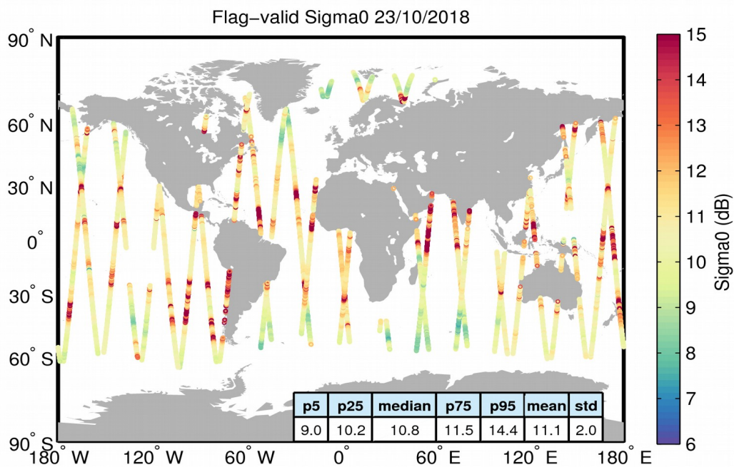
Figure 23. Geographical distribution of flag-valid sigma0 data over oceans and lakes for 23/10/2018. The statistical values shown in the table refer to the sigma0 in dB and are calculated over all measurements shown in the figure.
