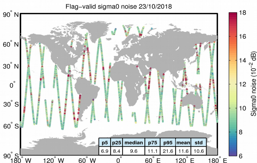
Figure 26. Geographical distribution of flag-valid 20-Hz sigma0 measurement noise over oceans and lakes for 23/10/2018. The statistical values shown in the table refer to the sigma0 noise and are calculated over all measurements shown in the figure.
