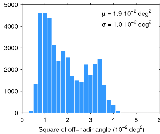
Figure 39. Histogram of flag-valid mispointing over oceans and lakes for 23/10/2018. The mean ( \mu ) and standard deviation ( \sigma ) are also shown. Note that values larger than 6 \cdot 10^{-2} \text{ deg}^2 are excluded from the histogram for the sake of readability but not from the computation of \mu and \sigma .
