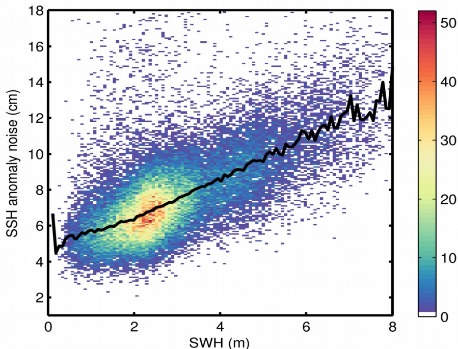
Figure 9. 2D histogram showing flag-valid SSH anomaly noise as a function of SWH for 21/10/2018. The black line denotes the median SSH anomaly noise as a function of SWH.
