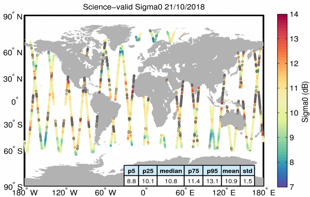
Figure 27. Geographical distribution of science-valid sigma0 data over oceans and lakes for 21/10/2018. The statistical values shown in the table refer to the sigma0 in dB and are calculated over all measurements shown in the figure. Gray circles denote records that have been rejected based on the editing criteria described in Table 4.
