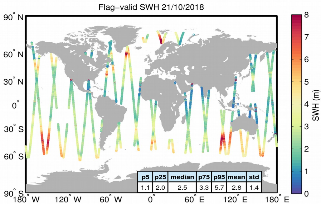
Figure 15. Geographical distribution of flag-valid SWH data over oceans and lakes for 21/10/2018. The statistical values shown in the table refer to the SWH in m and are calculated over all measurements shown in the figure.
