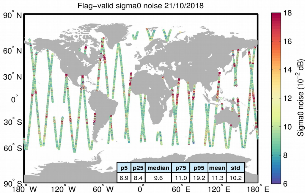
Figure 26. Geographical distribution of flag-valid 20-Hz sigma0 measurement noise over oceans and lakes for 21/10/2018. The statistical values shown in the table refer to the sigma0 noise and are calculated over all measurements shown in the figure.
