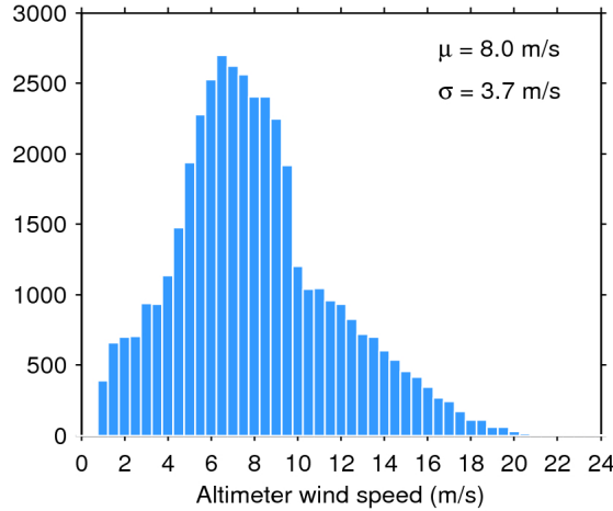
Figure 33. Histogram of flag-valid wind over oceans and lakes for 21/10/2018. The mean ( \mu ) and standard deviation ( \sigma ) are also shown. Note that values larger than 24 m/s are excluded from the histogram for the sake of readability but not from the computation of \mu and \sigma .
