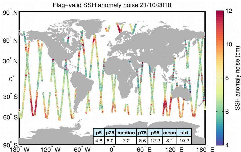
Figure 8. Geographical distribution of flag-valid 20-Hz SSH anomaly measurement noise over oceans and lakes for 21/10/2018. The statistical values shown in the table refer to the SSH anomaly noise and are calculated over all measurements shown in the figure.
