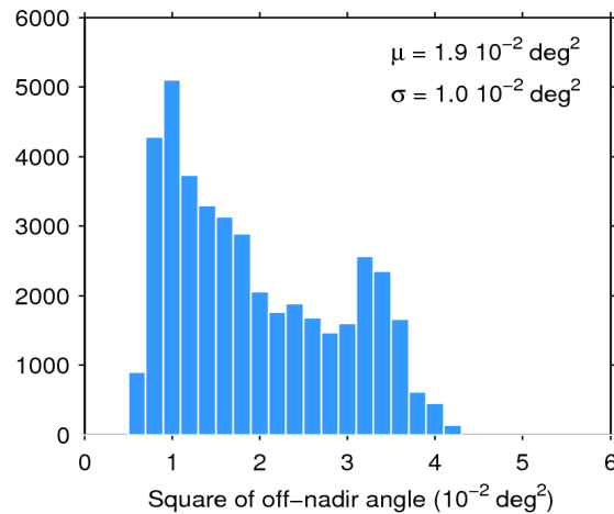
Figure 39. Histogram of flag-valid mispointing over oceans and lakes for 21/10/2018. The mean ( \mu ) and standard deviation ( \sigma ) are also shown. Note that values larger than 6 \cdot 10^{-2} \text{ deg}^2 are excluded from the histogram for the sake of readability but not from the computation of \mu and \sigma .
