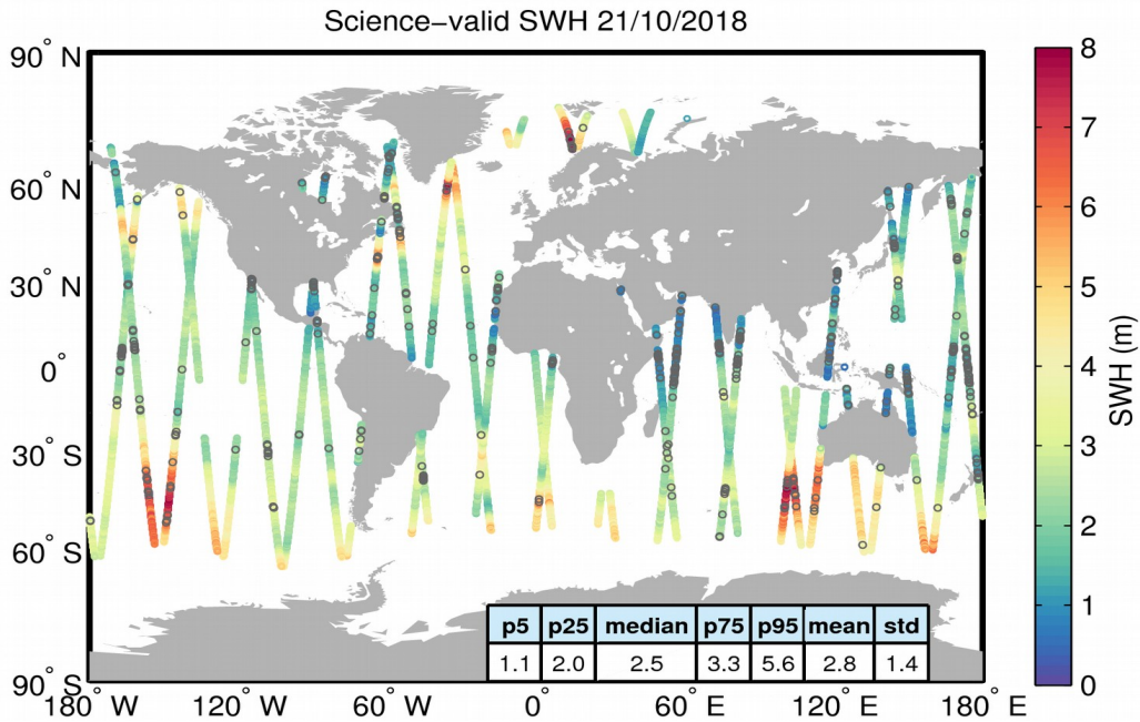
Figure 19. Geographical distribution of science-valid SWH data over oceans and lakes for 21/10/2018. The statistical values shown in the table refer to the SWH in m and are calculated over all measurements shown in the figure. Gray circles denote records that have been rejected based on the editing criteria described in Table 3.
