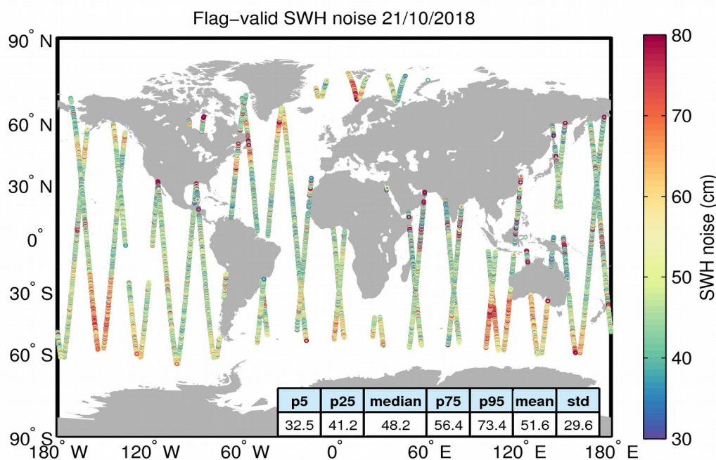
Figure 18. Geographical distribution of flag-valid 20-Hz SWH measurement noise over oceans and lakes for 21/10/2018. The statistical values shown in the figure refer to the SWH noise and are calculated over all measurements shown in the figure.
