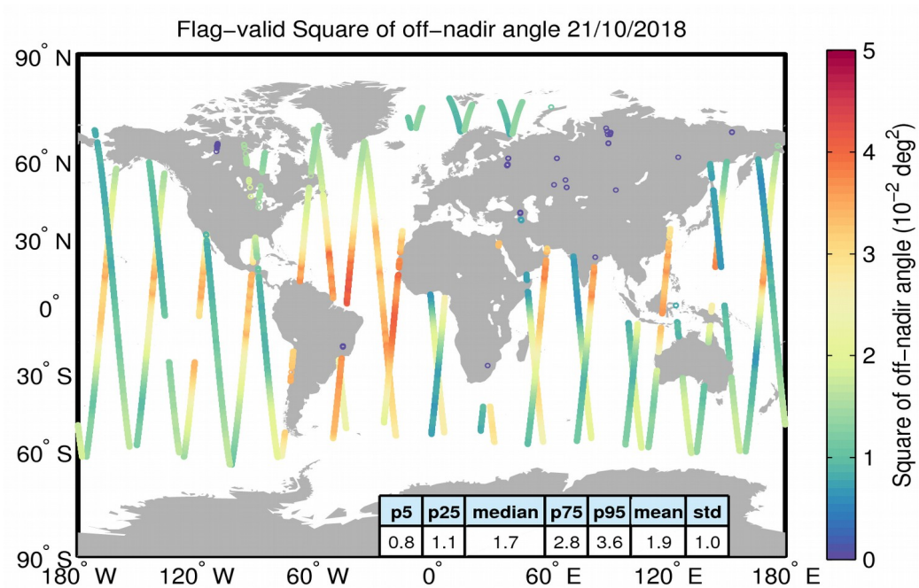
Figure 37. Geographical distribution of flag-valid mispointing data over oceans and lakes for 21/10/2018. The statistical values shown in the table refer to the mispointing in 10^{-2} \text{ deg}^2 and are calculated over all measurements shown in the figure.
