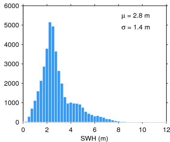
Figure 17. Histogram of flag-valid SWH over oceans and lakes for 21/10/2018. The mean ( \mu ) and standard deviation ( \sigma ) are also shown. Note that values larger than 12 m are excluded from the histogram for the sake of readability but not from the computation of \mu and \sigma .
