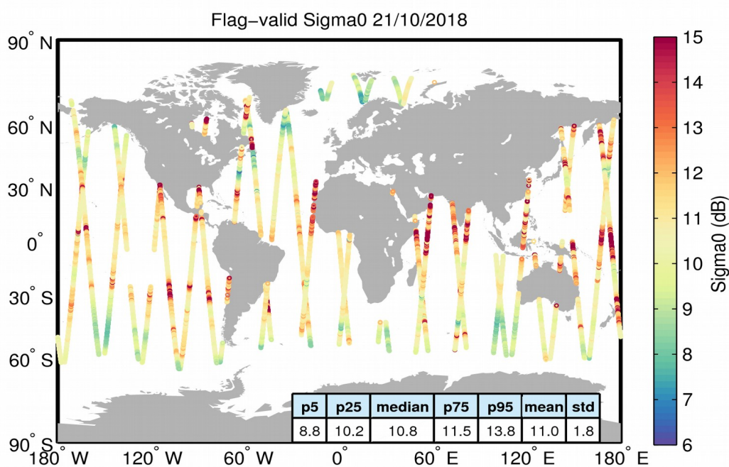
Figure 23. Geographical distribution of flag-valid sigma0 data over oceans and lakes for 21/10/2018. The statistical values shown in the table refer to the sigma0 in dB and are calculated over all measurements shown in the figure.
