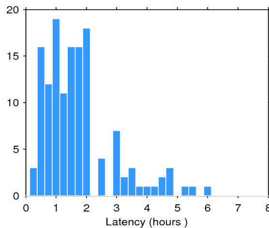
Figure 2. Histogram of the data latency for 21/10/2018. The y-axis denotes the number of files that are made available with a delay of x-hours with respect to the mean time of the records stored in the file.
