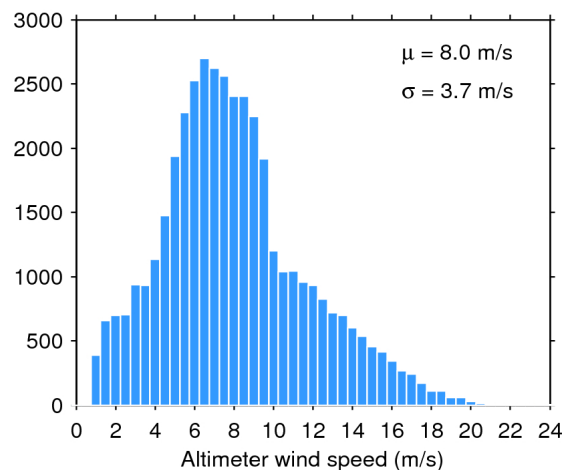
Figure 35. Histogram of science-valid wind over oceans and lakes for 21/10/2018. The mean ( \mu ) and standard deviation ( \sigma ) are also shown. Note that values larger than 24 m/s are excluded from the histogram for the sake of readability but not from the computation of \mu and \sigma .
