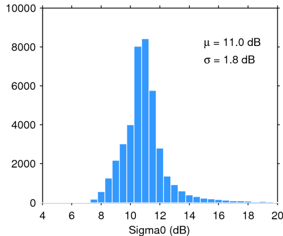
Figure 25. Histogram of flag-valid sigma0 over oceans and lakes for 21/10/2018. The mean ( \mu ) and standard deviation ( \sigma ) are also shown. Note that values outside [4 20] dB are excluded from the histogram for the sake of readability but not from the computation of \mu and \sigma .
