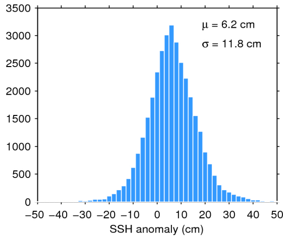
Figure 11. Histogram of science-valid SSH anomaly over oceans and lakes for 21/10/2018. The mean ( \mu ) and standard deviation ( \sigma ) are also shown. Note that values outside [-50 50] cm are excluded from the histogram for the sake of readability but not from the computation of \mu and \sigma .
