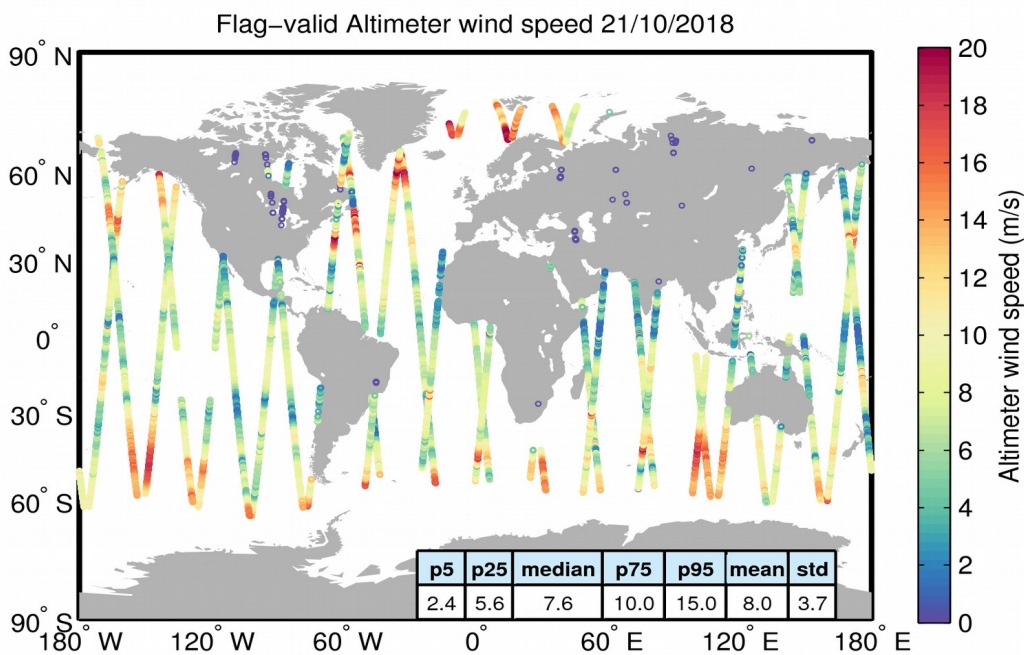
Figure 31. Geographical distribution of flag-valid wind data over oceans and lakes for 21/10/2018. The statistical values shown in the table refer to the wind in m/s and are calculated over all measurements shown in the figure.
