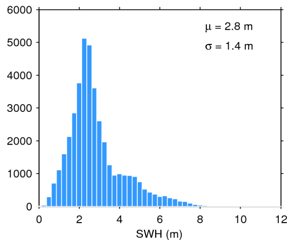
Figure 20. Histogram of science-valid SWH over oceans and lakes for 21/10/2018. The mean ( \mu ) and standard deviation ( \sigma ) are also shown. Note that values larger than 12 m are excluded from the histogram for the sake of readability but not from the computation of \mu and \sigma .
