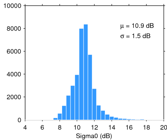
Figure 28. Histogram of science-valid sigma0 over oceans and lakes for 21/10/2018. The mean ( \mu ) and standard deviation ( \sigma ) are also shown. Note that values outside [4 20] dB are excluded from the histogram for the sake of readability but not from the computation of \mu and \sigma .
