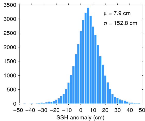
Figure 7. Histogram of flag-valid SSH anomaly over oceans and lakes for 21/10/2018. The mean ( \mu ) and standard deviation ( \sigma ) are also shown. Note that values outside [-50 50] cm are excluded from the histogram for the sake of readability but not from the computation of \mu and \sigma .
