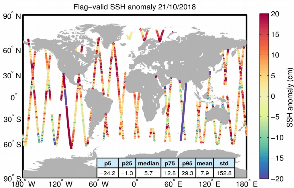
Figure 5. Geographical distribution of flag-valid 1-Hz SSH anomaly data over oceans and lakes for 21/10/2018. The statistical values shown in the table refer to the SSH anomaly in cm and are calculated over all measurements shown in the figure.
