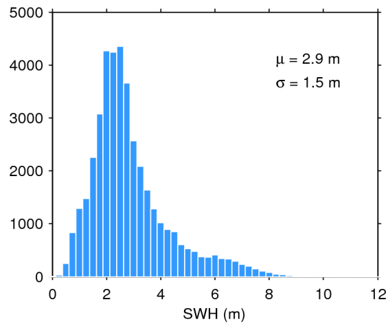
Figure 17. Histogram of flag-valid SWH over oceans and lakes for 20/10/2018. The mean ( \mu ) and standard deviation ( \sigma ) are also shown. Note that values larger than 12 m are excluded from the histogram for the sake of readability but not from the computation of \mu and \sigma .
