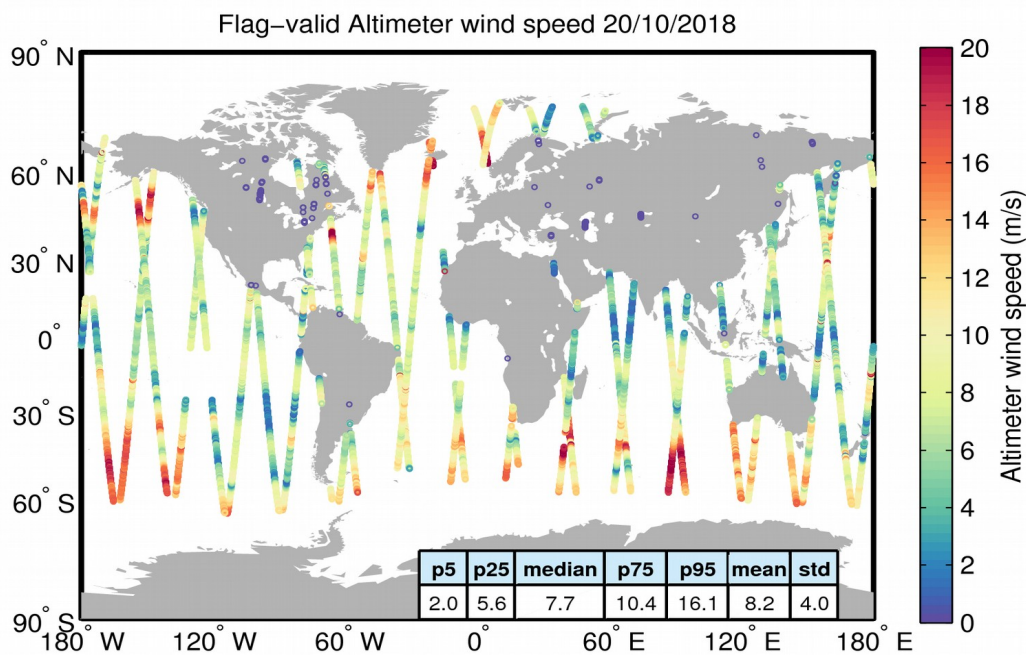
Figure 31. Geographical distribution of flag-valid wind data over oceans and lakes for 20/10/2018. The statistical values shown in the table refer to the wind in m/s and are calculated over all measurements shown in the figure.
