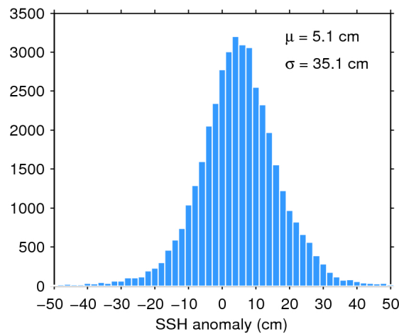
Figure 7. Histogram of flag-valid SSH anomaly over oceans and lakes for 20/10/2018. The mean ( \mu ) and standard deviation ( \sigma ) are also shown. Note that values outside [-50\ 50] cm are excluded from the histogram for the sake of readability but not from the computation of \mu and \sigma .
