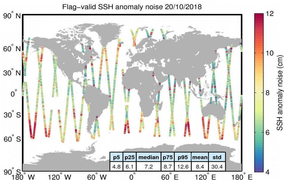
Figure 8. Geographical distribution of flag-valid 20-Hz SSH anomaly measurement noise over oceans and lakes for 20/10/2018. The statistical values shown in the table refer to the SSH anomaly noise and are calculated over all measurements shown in the figure.
