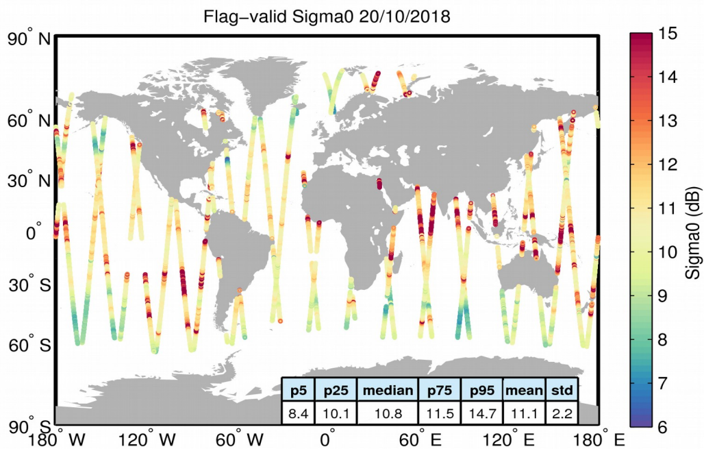
Figure 23. Geographical distribution of flag-valid sigma0 data over oceans and lakes for 20/10/2018. The statistical values shown in the table refer to the sigma0 in dB and are calculated over all measurements shown in the figure.
