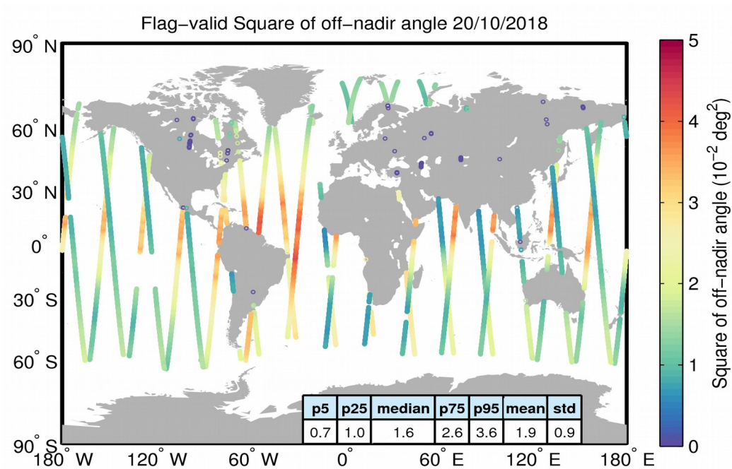
Figure 37. Geographical distribution of flag-valid mispointing data over oceans and lakes for 20/10/2018. The statistical values shown in the table refer to the mispointing in 10^{-2} deg 2 and are calculated over all measurements shown in the figure.
