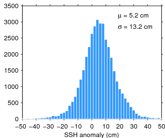
Figure 11. Histogram of science-valid SSH anomaly over oceans and lakes for 20/10/2018. The mean ( \mu ) and standard deviation ( \sigma ) are also shown. Note that values outside [-50 50] cm are excluded from the histogram for the sake of readability but not from the computation of \mu and \sigma .
