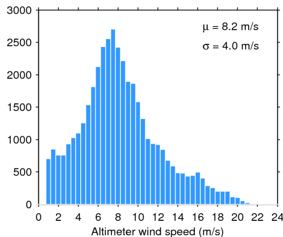
Figure 35. Histogram of science-valid wind over oceans and lakes for 20/10/2018. The mean ( \mu ) and standard deviation ( \sigma ) are also shown. Note that values larger than 24 m/s are excluded from the histogram for the sake of readability but not from the computation of \mu and \sigma .
