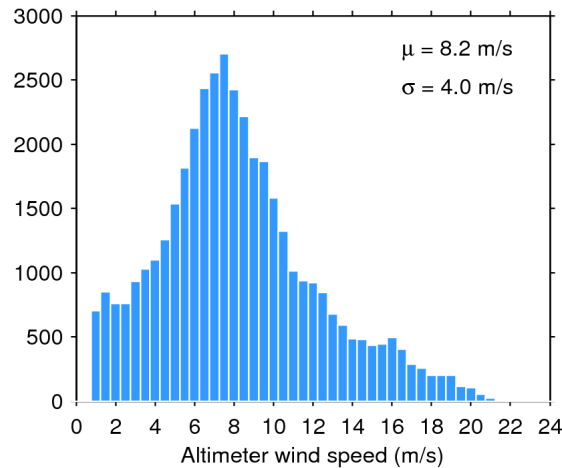
Figure 33. Histogram of flag-valid wind over oceans and lakes for 20/10/2018. The mean ( \mu ) and standard deviation ( \sigma ) are also shown. Note that values larger than 24 m/s are excluded from the histogram for the sake of readability but not from the computation of \mu and \sigma .
