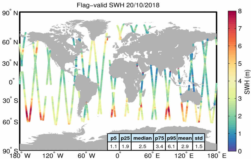
Figure 15. Geographical distribution of flag-valid SWH data over oceans and lakes for 20/10/2018. The statistical values shown in the table refer to the SWH in m and are calculated over all measurements shown in the figure.
