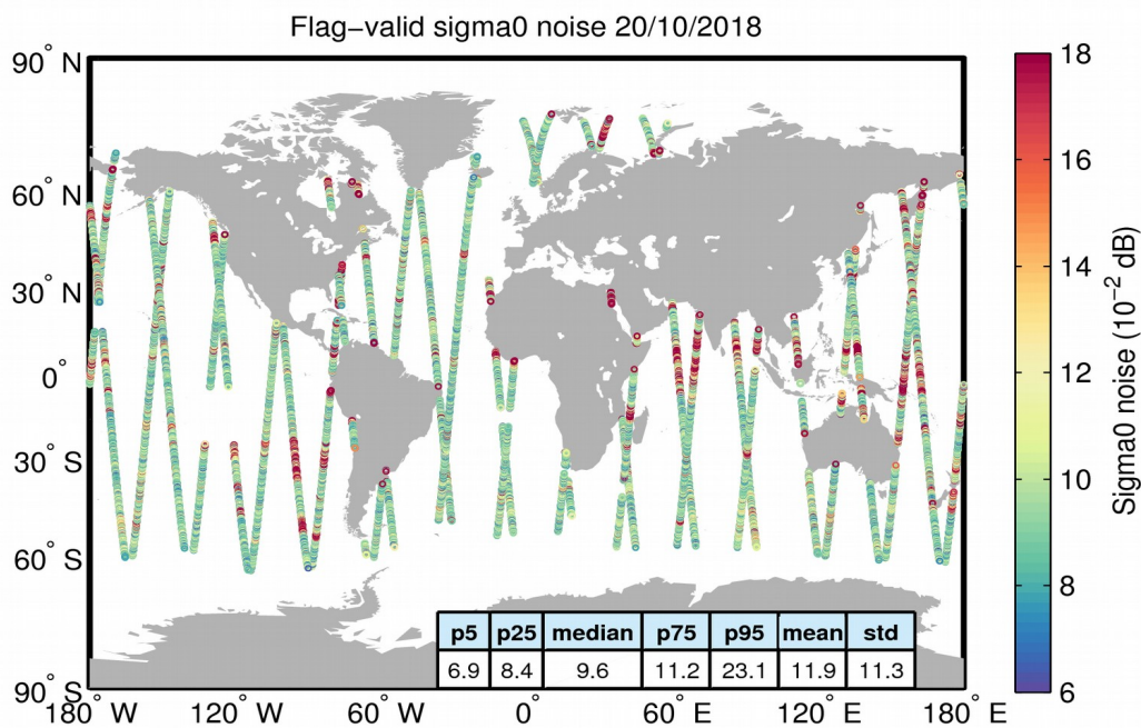
Figure 26. Geographical distribution of flag-valid 20-Hz sigma0 measurement noise over oceans and lakes for 20/10/2018. The statistical values shown in the table refer to the sigma0 noise and are calculated over all measurements shown in the figure.
