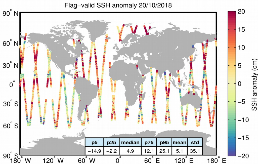
Figure 5. Geographical distribution of flag-valid 1-Hz SSH anomaly data over oceans and lakes for 20/10/2018. The statistical values shown in the table refer to the SSH anomaly in cm and are calculated over all measurements shown in the figure.
