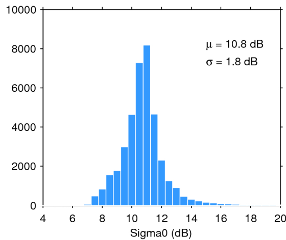
Figure 28. Histogram of science-valid sigma0 over oceans and lakes for 20/10/2018. The mean ( \mu ) and standard deviation ( \sigma ) are also shown. Note that values outside [4 20] dB are excluded from the histogram for the sake of readability but not from the computation of \mu and \sigma .
