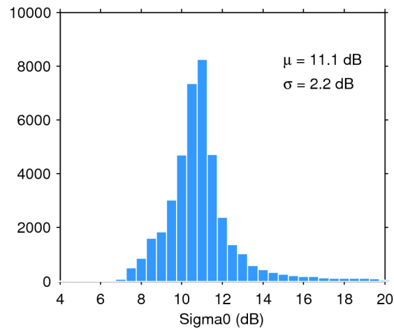
Figure 25. Histogram of flag-valid sigma0 over oceans and lakes for 20/10/2018. The mean ( \mu ) and standard deviation ( \sigma ) are also shown. Note that values outside [4 20] dB are excluded from the histogram for the sake of readability but not from the computation of \mu and \sigma .
