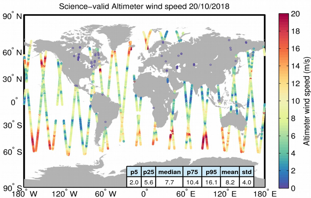
Figure 34. Geographical distribution of science-valid wind data over oceans and lakes for 20/10/2018. The statistical values shown in the table refer to the wind in m/s and are calculated over all measurements shown in the figure. Gray circles denote records that have been rejected based on the editing criteria described in Table 5.
