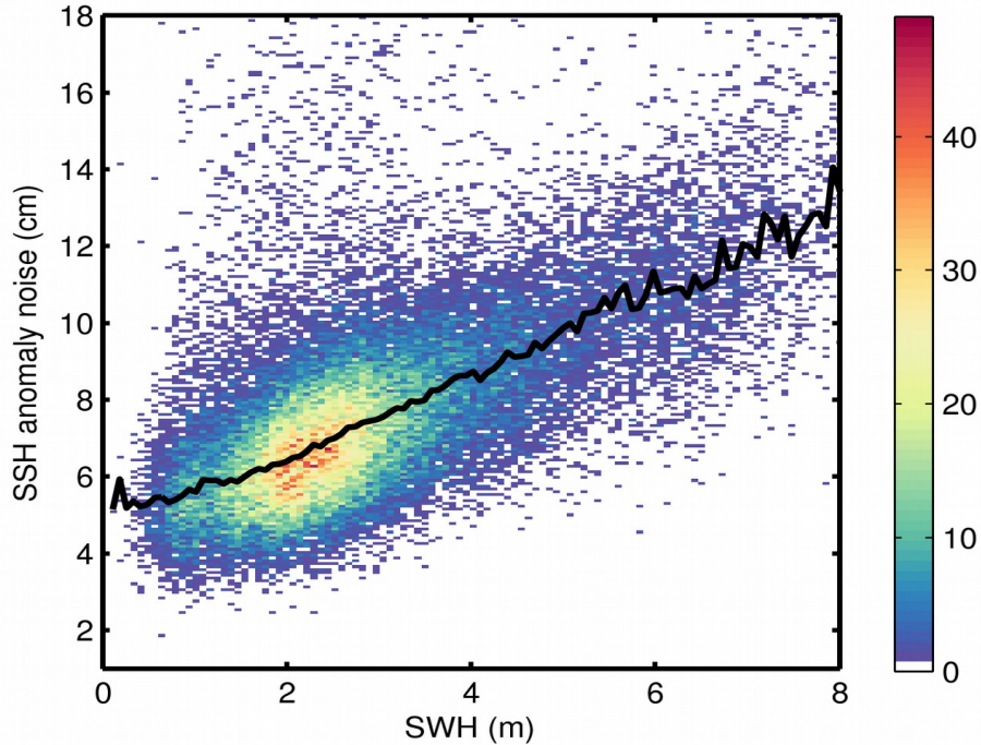
Figure 9. 2D histogram showing flag-valid SSH anomaly noise as a function of SWH for 20/10/2018. The black line denotes the median SSH anomaly noise as a function of SWH.
