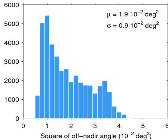
Figure 39. Histogram of flag-valid mispointing over oceans and lakes for 20/10/2018. The mean ( \mu ) and standard deviation ( \sigma ) are also shown. Note that values larger than 6 \cdot 10^{-2} \text{ deg}^2 are excluded from the histogram for the sake of readability but not from the computation of \mu and \sigma .
