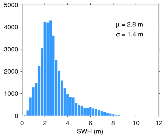
Figure 20. Histogram of science-valid SWH over oceans and lakes for 20/10/2018. The mean ( \mu ) and standard deviation ( \sigma ) are also shown. Note that values larger than 12 m are excluded from the histogram for the sake of readability but not from the computation of \mu and \sigma .
