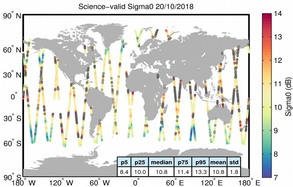
Figure 27. Geographical distribution of science-valid sigma0 data over oceans and lakes for 20/10/2018. The statistical values shown in the table refer to the sigma0 in dB and are calculated over all measurements shown in the figure. Gray circles denote records that have been rejected based on the editing criteria described in Table 4.
