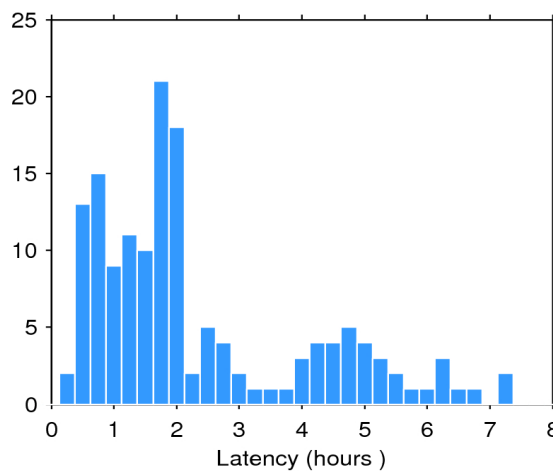
Figure 2. Histogram of the data latency for 20/10/2018. The y-axis denotes the number of files that are made available with a delay of x-hours with respect to the mean time of the records stored in the file.
