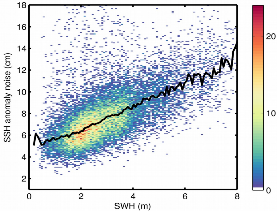
Figure 9. 2D histogram showing flag-valid SSH anomaly noise as a function of SWH for 19/10/2018. The black line denotes the median SSH anomaly noise as a function of SWH.
