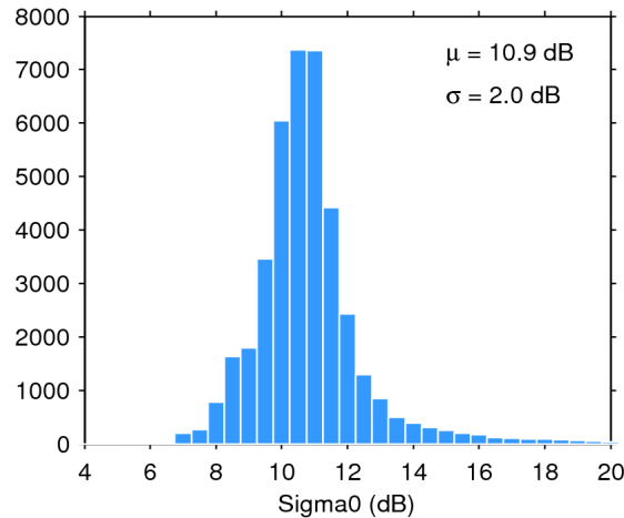
Figure 25. Histogram of flag-valid sigma0 over oceans and lakes for 19/10/2018. The mean ( \mu ) and standard deviation ( \sigma ) are also shown. Note that values outside [4 20] dB are excluded from the histogram for the sake of readability but not from the computation of \mu and \sigma .
