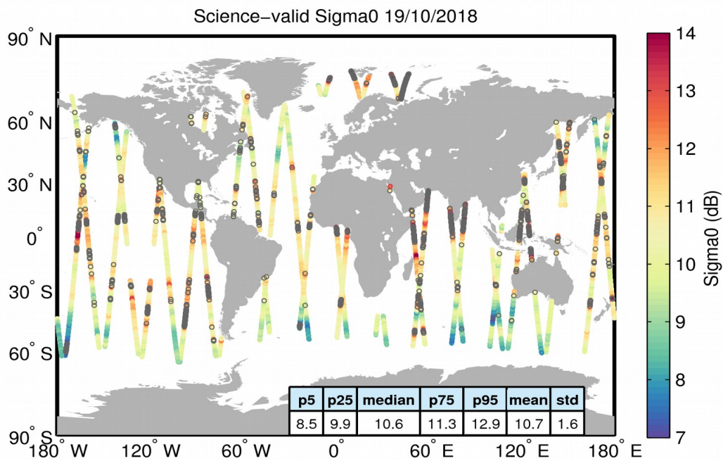
Figure 27. Geographical distribution of science-valid sigma0 data over oceans and lakes for 19/10/2018. The statistical values shown in the table refer to the sigma0 in dB and are calculated over all measurements shown in the figure. Gray circles denote records that have been rejected based on the editing criteria described in Table 4.
