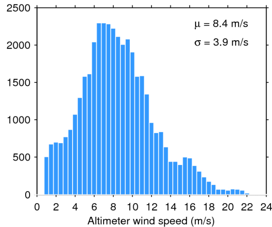
Figure 33. Histogram of flag-valid wind over oceans and lakes for 19/10/2018. The mean ( \mu ) and standard deviation ( \sigma ) are also shown. Note that values larger than 24 m/s are excluded from the histogram for the sake of readability but not from the computation of \mu and \sigma .
