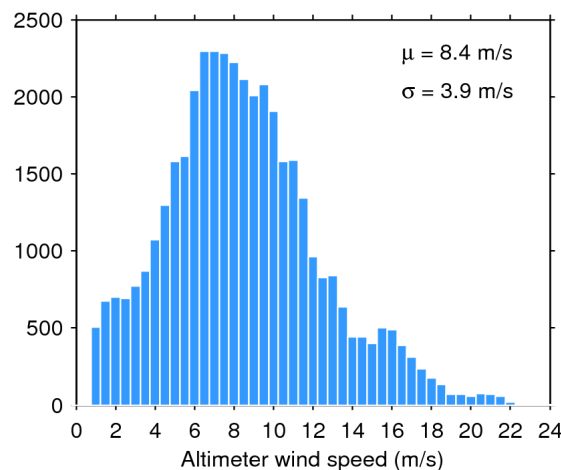
Figure 35. Histogram of science-valid wind over oceans and lakes for 19/10/2018. The mean ( \mu ) and standard deviation ( \sigma ) are also shown. Note that values larger than 24 m/s are excluded from the histogram for the sake of readability but not from the computation of \mu and \sigma .
