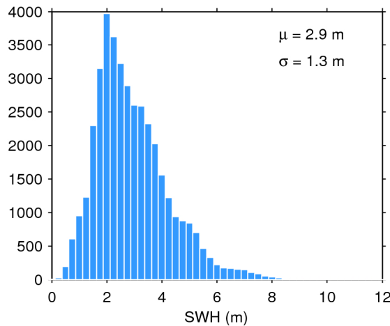
Figure 20. Histogram of science-valid SWH over oceans and lakes for 19/10/2018. The mean ( \mu ) and standard deviation ( \sigma ) are also shown. Note that values larger than 12 m are excluded from the histogram for the sake of readability but not from the computation of \mu and \sigma .
