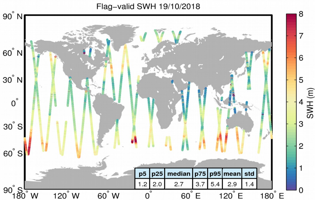
Figure 15. Geographical distribution of flag-valid SWH data over oceans and lakes for 19/10/2018. The statistical values shown in the table refer to the SWH in m and are calculated over all measurements shown in the figure.
