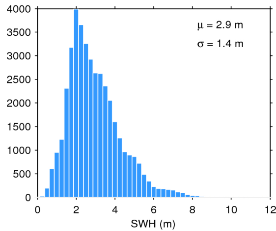
Figure 17. Histogram of flag-valid SWH over oceans and lakes for 19/10/2018. The mean ( \mu ) and standard deviation ( \sigma ) are also shown. Note that values larger than 12 m are excluded from the histogram for the sake of readability but not from the computation of \mu and \sigma .
