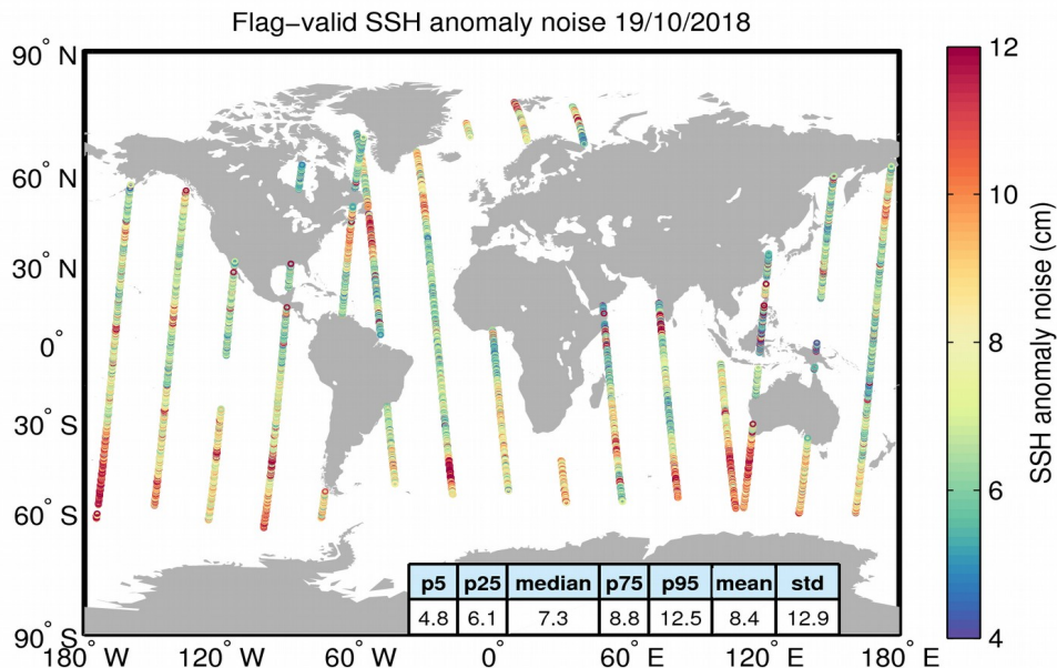
Figure 8. Geographical distribution of flag-valid 20-Hz SSH anomaly measurement noise over oceans and lakes for 19/10/2018. The statistical values shown in the table refer to the SSH anomaly noise and are calculated over all measurements shown in the figure.
