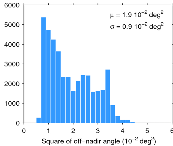
Figure 39. Histogram of flag-valid mispointing over oceans and lakes for 19/10/2018. The mean ( \mu ) and standard deviation ( \sigma ) are also shown. Note that values larger than 6 \cdot 10^{-2} \text{ deg}^2 are excluded from the histogram for the sake of readability but not from the computation of \mu and \sigma .
