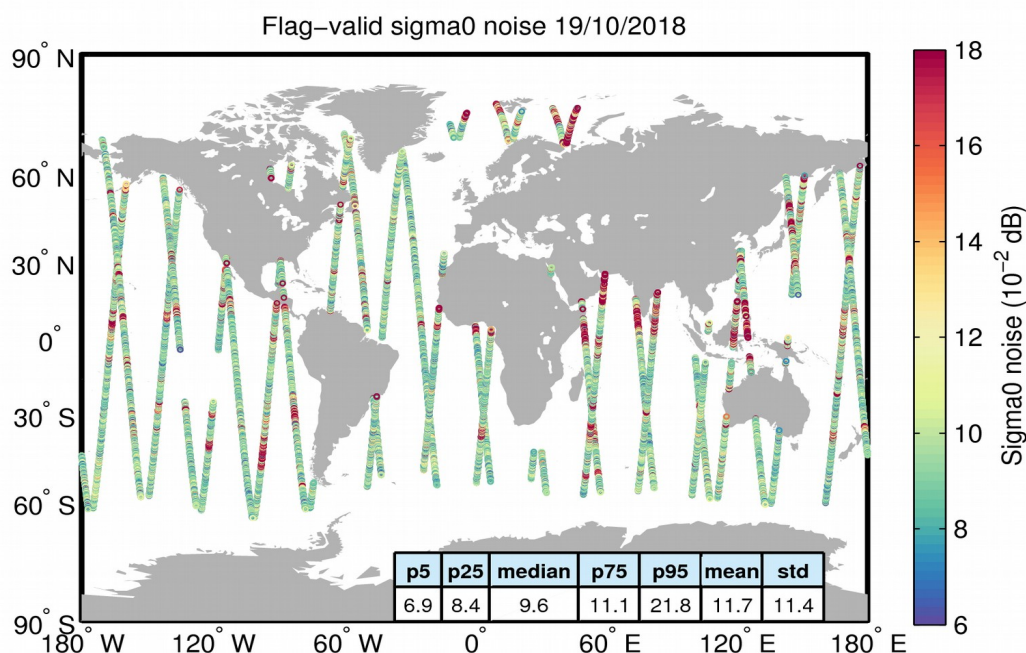
Figure 26. Geographical distribution of flag-valid 20-Hz sigma0 measurement noise over oceans and lakes for 19/10/2018. The statistical values shown in the table refer to the sigma0 noise and are calculated over all measurements shown in the figure.
