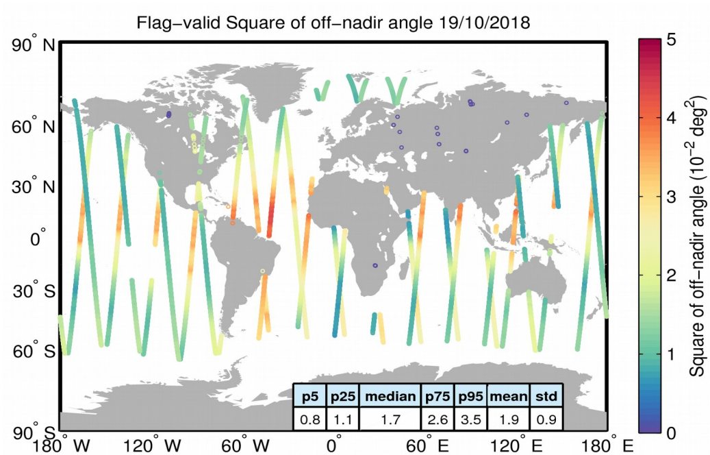
Figure 37. Geographical distribution of flag-valid mispointing data over oceans and lakes for 19/10/2018. The statistical values shown in the table refer to the mispointing in 10^{-2} \text{ deg}^2 and are calculated over all measurements shown in the figure.
