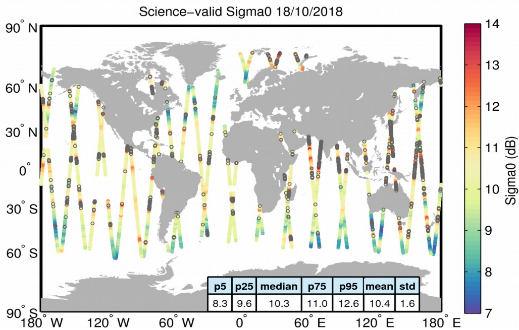
Figure 27. Geographical distribution of science-valid sigma0 data over oceans and lakes for 18/10/2018. The statistical values shown in the table refer to the sigma0 in dB and are calculated over all measurements shown in the figure. Gray circles denote records that have been rejected based on the editing criteria described in Table 4.
