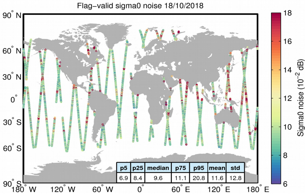
Figure 26. Geographical distribution of flag-valid 20-Hz sigma0 measurement noise over oceans and lakes for 18/10/2018. The statistical values shown in the table refer to the sigma0 noise and are calculated over all measurements shown in the figure.
