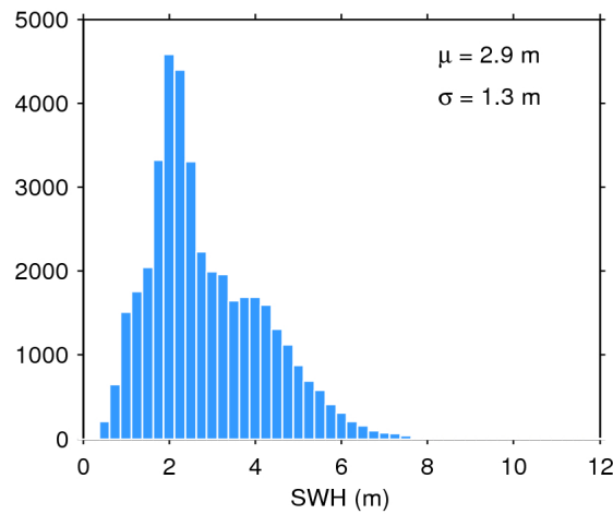
Figure 17. Histogram of flag-valid SWH over oceans and lakes for 18/10/2018. The mean ( \mu ) and standard deviation ( \sigma ) are also shown. Note that values larger than 12 m are excluded from the histogram for the sake of readability but not from the computation of \mu and \sigma .
