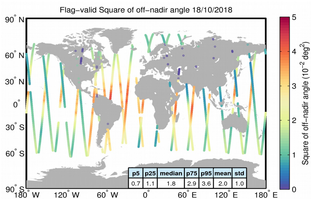
Figure 37. Geographical distribution of flag-valid mispointing data over oceans and lakes for 18/10/2018. The statistical values shown in the table refer to the mispointing in 10^{-2} deg 2 and are calculated over all measurements shown in the figure.
