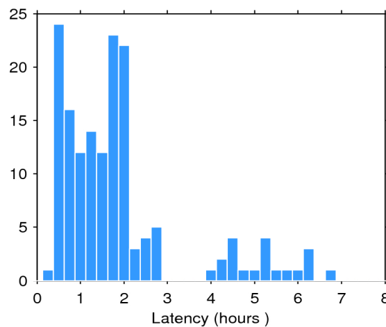
Figure 2. Histogram of the data latency for 18/10/2018. The y-axis denotes the number of files that are made available with a delay of x-hours with respect to the mean time of the records stored in the file.
