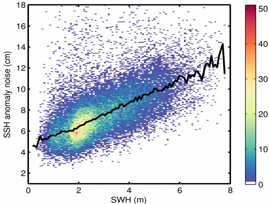
Figure 9. 2D histogram showing flag-valid SSH anomaly noise as a function of SWH for 18/10/2018. The black line denotes the median SSH anomaly noise as a function of SWH.
