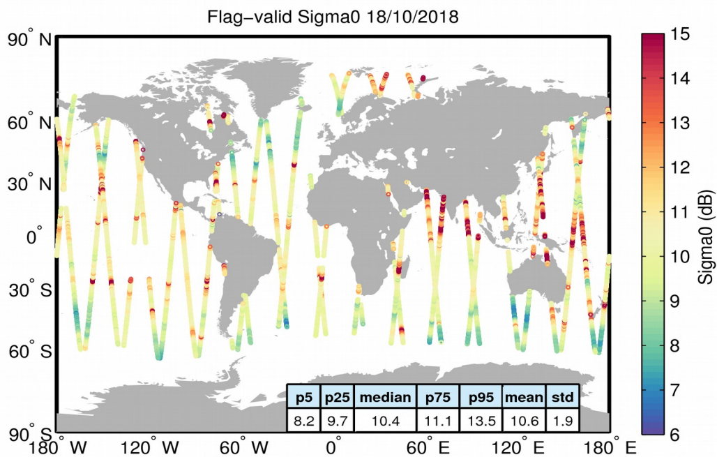
Figure 23. Geographical distribution of flag-valid sigma0 data over oceans and lakes for 18/10/2018. The statistical values shown in the table refer to the sigma0 in dB and are calculated over all measurements shown in the figure.
