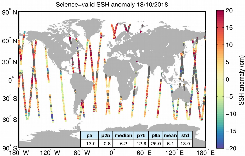
Figure 10. Geographical distribution of science-valid SSH anomaly data over oceans and lakes for 18/10/2018. The statistical values shown in the table refer to the SSH anomaly in cm and are calculated over all measurements shown in the figure. Gray circles denote records that have been rejected based on the editing criteria described in Table 2.
