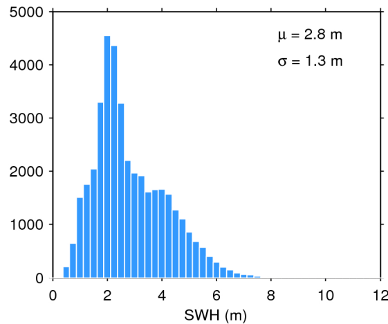
Figure 20. Histogram of science-valid SWH over oceans and lakes for 18/10/2018. The mean ( \mu ) and standard deviation ( \sigma ) are also shown. Note that values larger than 12 m are excluded from the histogram for the sake of readability but not from the computation of \mu and \sigma .
