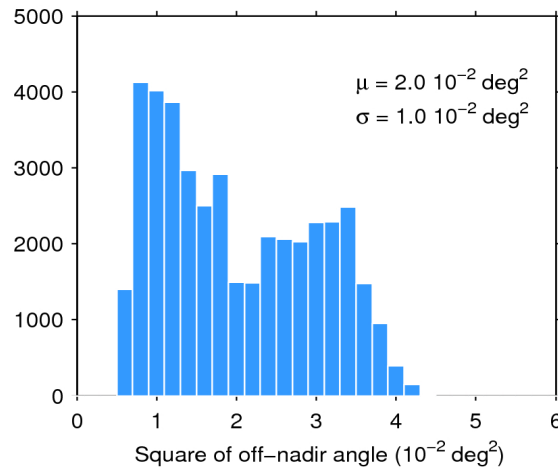
Figure 39. Histogram of flag-valid mispointing over oceans and lakes for 18/10/2018. The mean ( \mu ) and standard deviation ( \sigma ) are also shown. Note that values larger than 6 \cdot 10^{-2} \text{ deg}^2 are excluded from the histogram for the sake of readability but not from the computation of \mu and \sigma .
