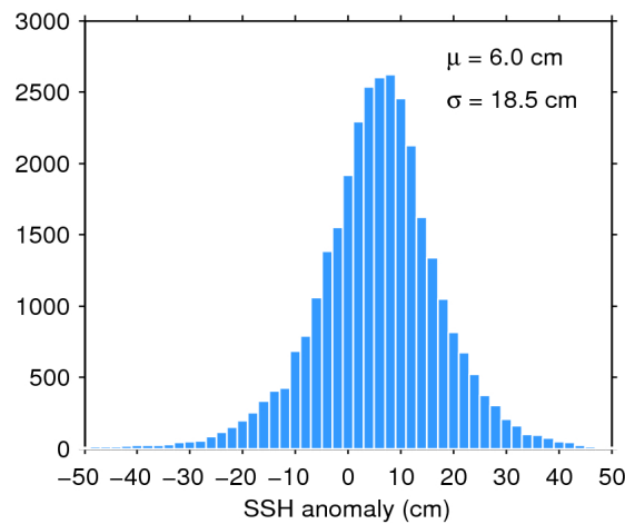
Figure 7. Histogram of flag-valid SSH anomaly over oceans and lakes for 18/10/2018. The mean ( \mu ) and standard deviation ( \sigma ) are also shown. Note that values outside [-50 50] cm are excluded from the histogram for the sake of readability but not from the computation of \mu and \sigma .
