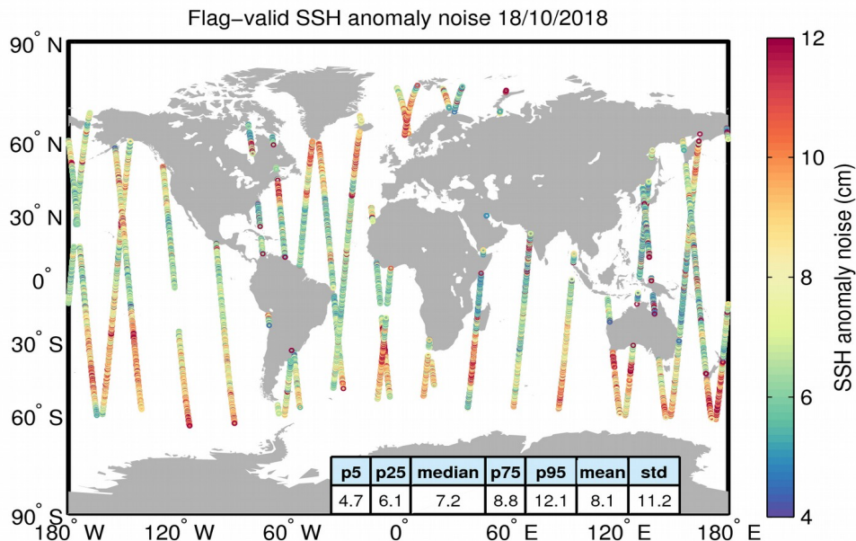
Figure 8. Geographical distribution of flag-valid 20-Hz SSH anomaly measurement noise over oceans and lakes for 18/10/2018. The statistical values shown in the table refer to the SSH anomaly noise and are calculated over all measurements shown in the figure.
