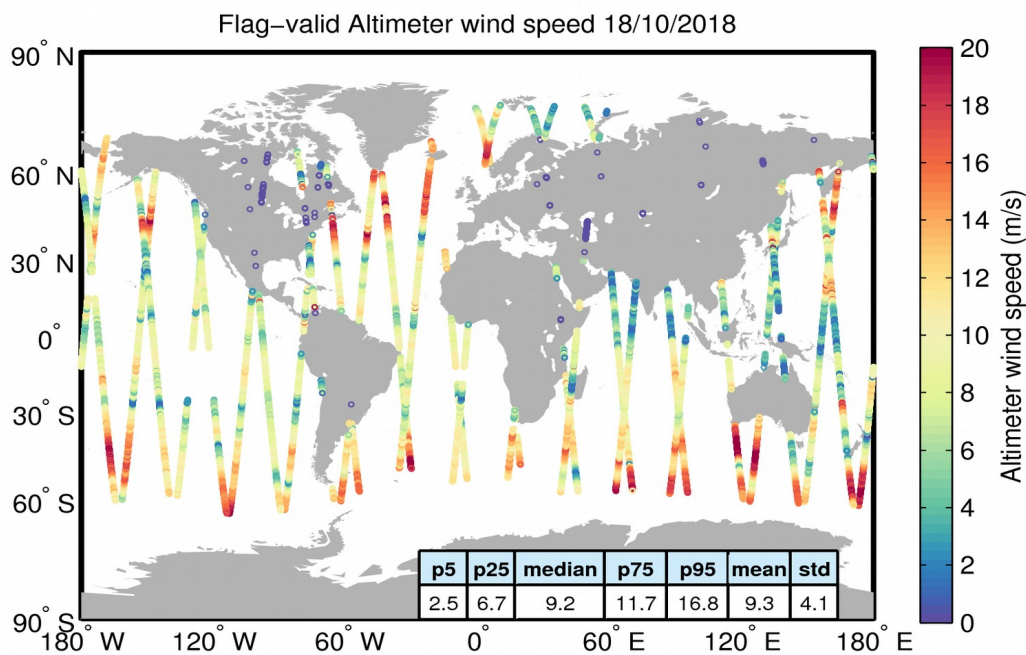
Figure 31. Geographical distribution of flag-valid wind data over oceans and lakes for 18/10/2018. The statistical values shown in the table refer to the wind in m/s and are calculated over all measurements shown in the figure.
