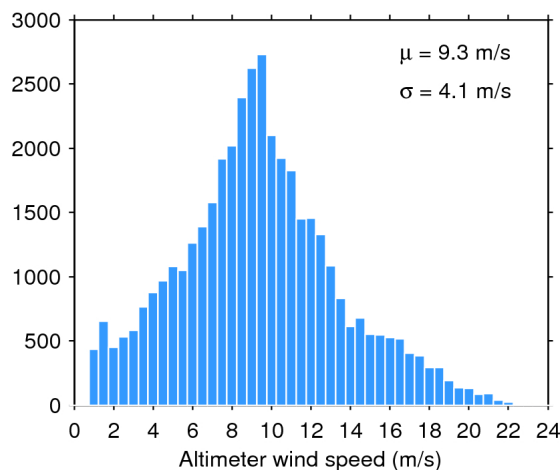
Figure 35. Histogram of science-valid wind over oceans and lakes for 18/10/2018. The mean ( \mu ) and standard deviation ( \sigma ) are also shown. Note that values larger than 24 m/s are excluded from the histogram for the sake of readability but not from the computation of \mu and \sigma .
