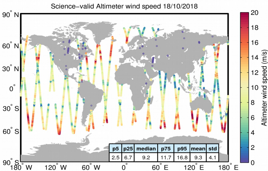
Figure 34. Geographical distribution of science-valid wind data over oceans and lakes for 18/10/2018. The statistical values shown in the table refer to the wind in m/s and are calculated over all measurements shown in the figure. Gray circles denote records that have been rejected based on the editing criteria described in Table 5.
