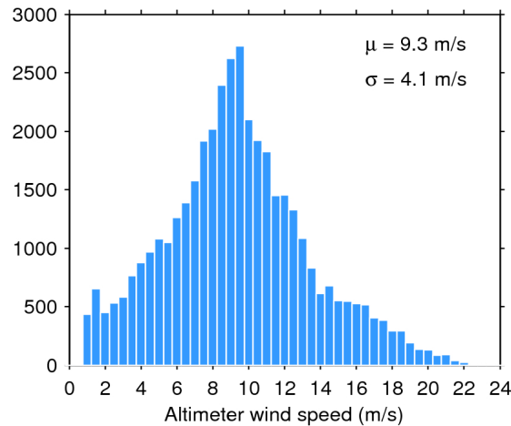
Figure 33. Histogram of flag-valid wind over oceans and lakes for 18/10/2018. The mean ( \mu ) and standard deviation ( \sigma ) are also shown. Note that values larger than 24 m/s are excluded from the histogram for the sake of readability but not from the computation of \mu and \sigma .
