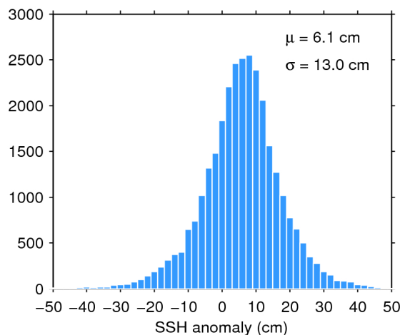
Figure 11. Histogram of science-valid SSH anomaly over oceans and lakes for 18/10/2018. The mean ( \mu ) and standard deviation ( \sigma ) are also shown. Note that values outside [-50 50] cm are excluded from the histogram for the sake of readability but not from the computation of \mu and \sigma .
