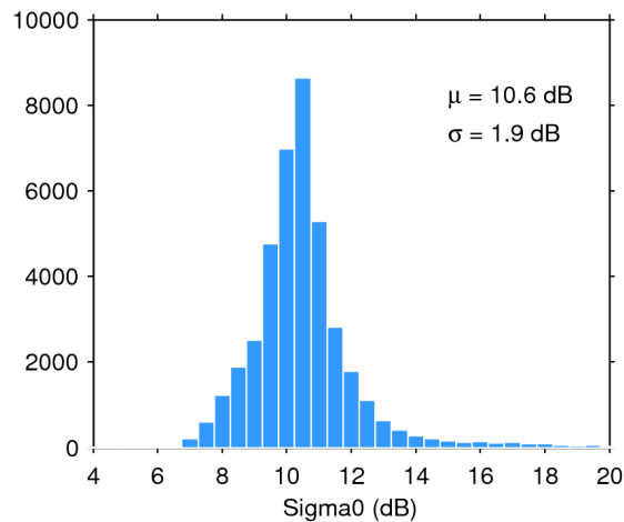
Figure 25. Histogram of flag-valid sigma0 over oceans and lakes for 18/10/2018. The mean ( \mu ) and standard deviation ( \sigma ) are also shown. Note that values outside [4 20] dB are excluded from the histogram for the sake of readability but not from the computation of \mu and \sigma .
