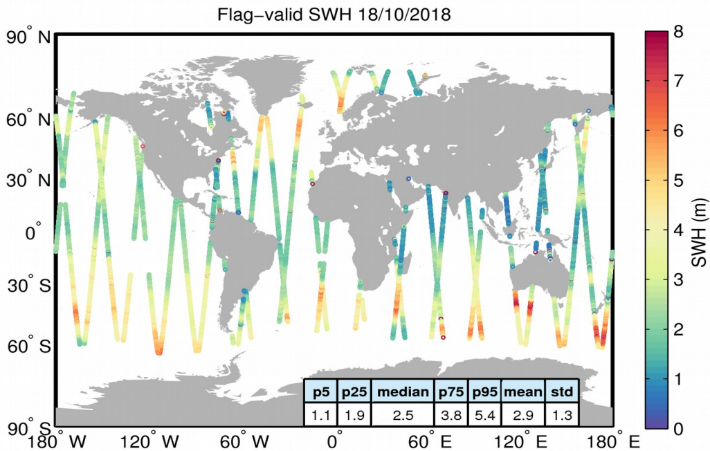
Figure 15. Geographical distribution of flag-valid SWH data over oceans and lakes for 18/10/2018. The statistical values shown in the table refer to the SWH in m and are calculated over all measurements shown in the figure.
