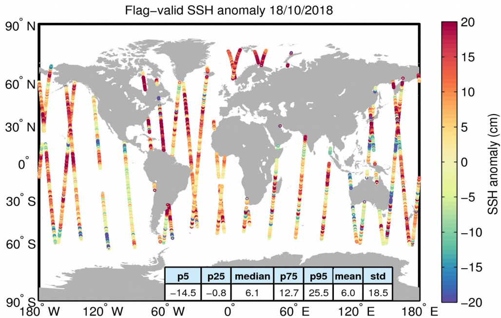
Figure 5. Geographical distribution of flag-valid 1-Hz SSH anomaly data over oceans and lakes for 18/10/2018. The statistical values shown in the table refer to the SSH anomaly in cm and are calculated over all measurements shown in the figure.
