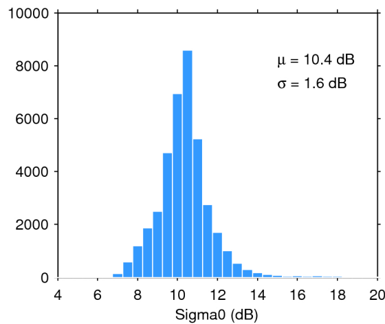
Figure 28. Histogram of science-valid sigma0 over oceans and lakes for 18/10/2018. The mean ( \mu ) and standard deviation ( \sigma ) are also shown. Note that values outside [4 20] dB are excluded from the histogram for the sake of readability but not from the computation of \mu and \sigma .
