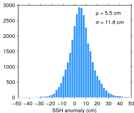
Figure 11. Histogram of science-valid SSH anomaly over oceans and lakes for 17/10/2018. The mean ( \mu ) and standard deviation ( \sigma ) are also shown. Note that values outside [-50 50] cm are excluded from the histogram for the sake of readability but not from the computation of \mu and \sigma .
