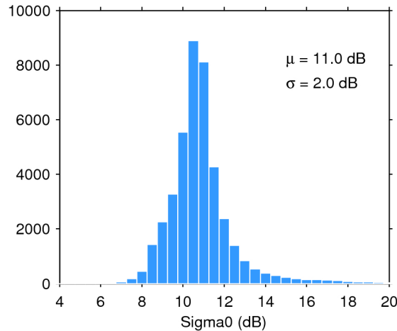
Figure 25. Histogram of flag-valid sigma0 over oceans and lakes for 17/10/2018. The mean ( \mu ) and standard deviation ( \sigma ) are also shown. Note that values outside [4 20] dB are excluded from the histogram for the sake of readability but not from the computation of \mu and \sigma .
