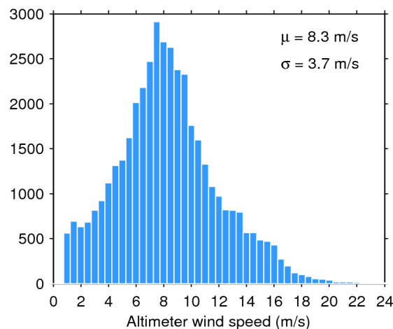
Figure 35. Histogram of science-valid wind over oceans and lakes for 17/10/2018. The mean ( \mu ) and standard deviation ( \sigma ) are also shown. Note that values larger than 24 m/s are excluded from the histogram for the sake of readability but not from the computation of \mu and \sigma .
