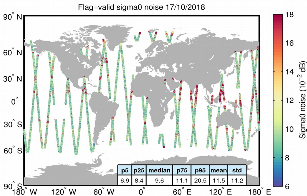
Figure 26. Geographical distribution of flag-valid 20-Hz sigma0 measurement noise over oceans and lakes for 17/10/2018. The statistical values shown in the table refer to the sigma0 noise and are calculated over all measurements shown in the figure.
