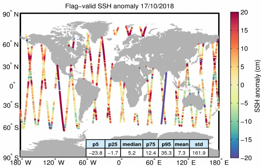
Figure 5. Geographical distribution of flag-valid 1-Hz SSH anomaly data over oceans and lakes for 17/10/2018. The statistical values shown in the table refer to the SSH anomaly in cm and are calculated over all measurements shown in the figure.
