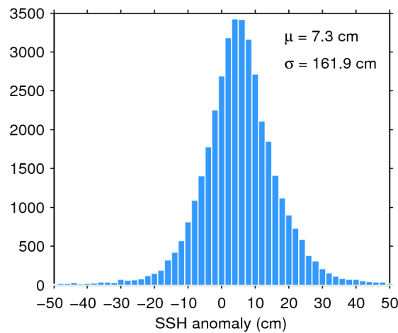
Figure 7. Histogram of flag-valid SSH anomaly over oceans and lakes for 17/10/2018. The mean ( \mu ) and standard deviation ( \sigma ) are also shown. Note that values outside [-50 50] cm are excluded from the histogram for the sake of readability but not from the computation of \mu and \sigma .
