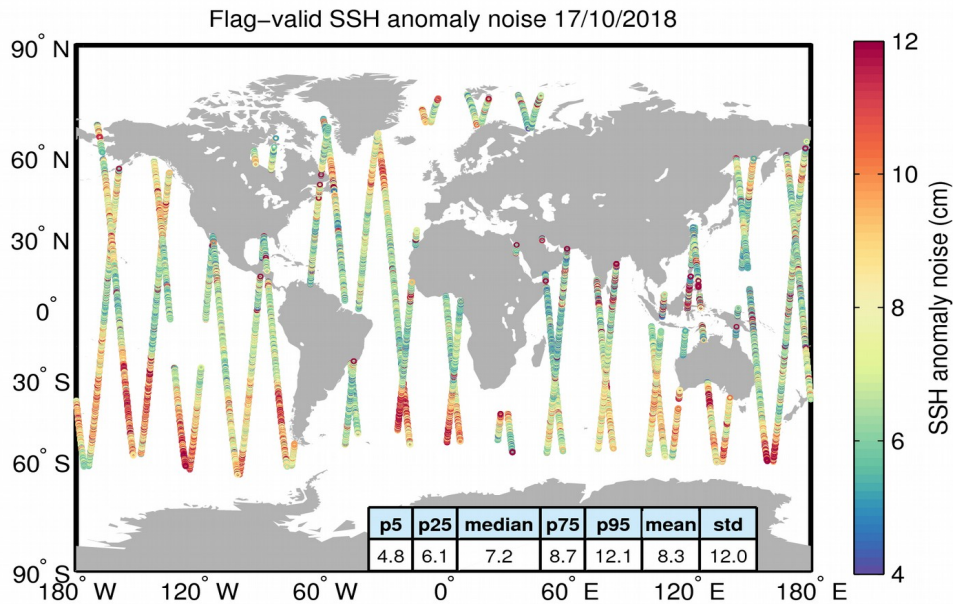
Figure 8. Geographical distribution of flag-valid 20-Hz SSH anomaly measurement noise over oceans and lakes for 17/10/2018. The statistical values shown in the table refer to the SSH anomaly noise and are calculated over all measurements shown in the figure.
