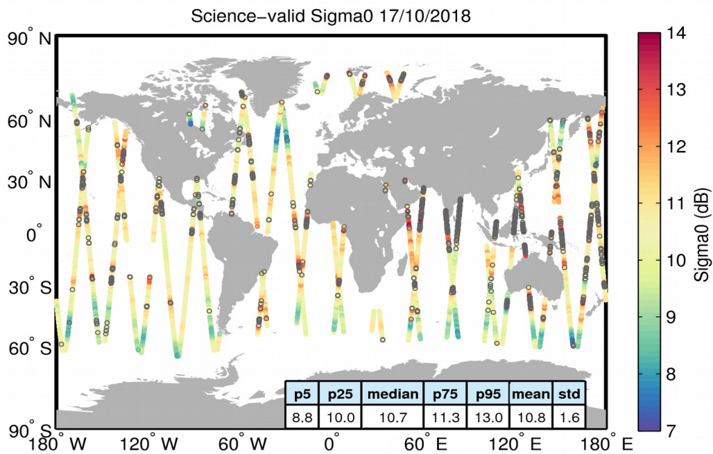
Figure 27. Geographical distribution of science-valid sigma0 data over oceans and lakes for 17/10/2018. The statistical values shown in the table refer to the sigma0 in dB and are calculated over all measurements shown in the figure. Gray circles denote records that have been rejected based on the editing criteria described in Table 4.
