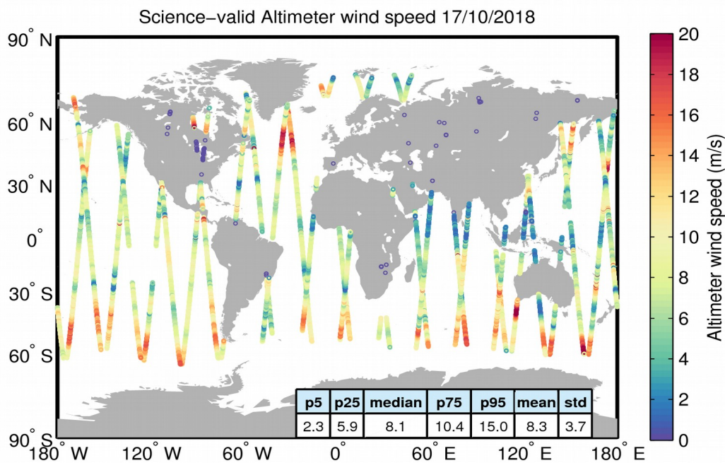
Figure 34. Geographical distribution of science-valid wind data over oceans and lakes for 17/10/2018. The statistical values shown in the table refer to the wind in m/s and are calculated over all measurements shown in the figure. Gray circles denote records that have been rejected based on the editing criteria described in Table 5.
