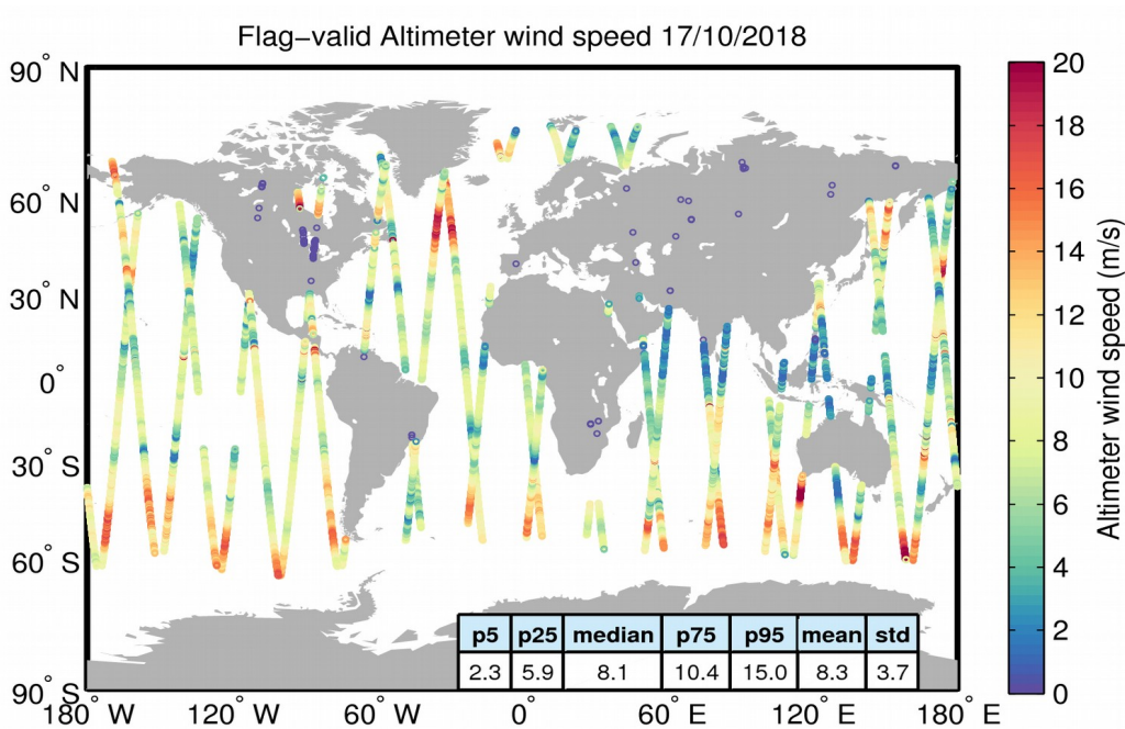
Figure 31. Geographical distribution of flag-valid wind data over oceans and lakes for 17/10/2018. The statistical values shown in the table refer to the wind in m/s and are calculated over all measurements shown in the figure.
