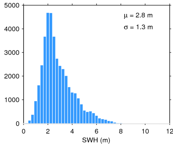
Figure 20. Histogram of science-valid SWH over oceans and lakes for 17/10/2018. The mean ( \mu ) and standard deviation ( \sigma ) are also shown. Note that values larger than 12 m are excluded from the histogram for the sake of readability but not from the computation of \mu and \sigma .
