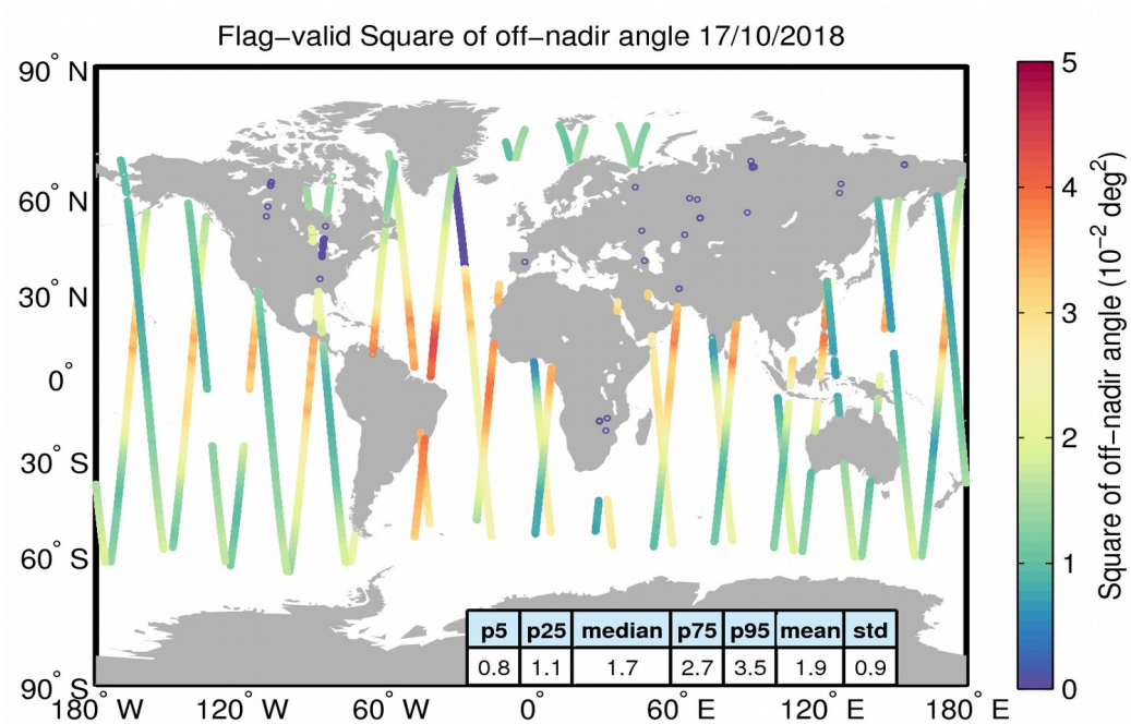
Figure 37. Geographical distribution of flag-valid mispointing data over oceans and lakes for 17/10/2018. The statistical values shown in the table refer to the mispointing in 10^{-2} \text{ deg}^2 and are calculated over all measurements shown in the figure.
