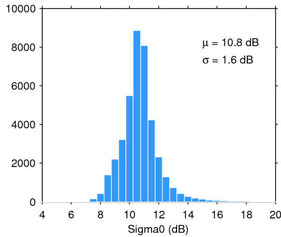
Figure 28. Histogram of science-valid sigma0 over oceans and lakes for 17/10/2018. The mean ( \mu ) and standard deviation ( \sigma ) are also shown. Note that values outside [4 20] dB are excluded from the histogram for the sake of readability but not from the computation of \mu and \sigma .
