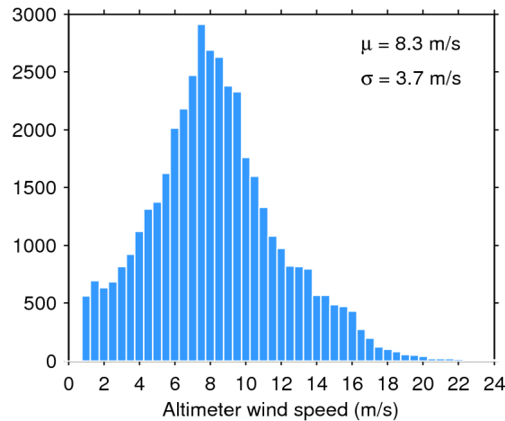
Figure 33. Histogram of flag-valid wind over oceans and lakes for 17/10/2018. The mean ( \mu ) and standard deviation ( \sigma ) are also shown. Note that values larger than 24 m/s are excluded from the histogram for the sake of readability but not from the computation of \mu and \sigma .
