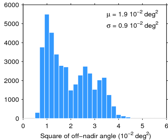
Figure 39. Histogram of flag-valid mispointing over oceans and lakes for 17/10/2018. The mean ( \mu ) and standard deviation ( \sigma ) are also shown. Note that values larger than 6 \cdot 10^{-2} \text{ deg}^2 are excluded from the histogram for the sake of readability but not from the computation of \mu and \sigma .
