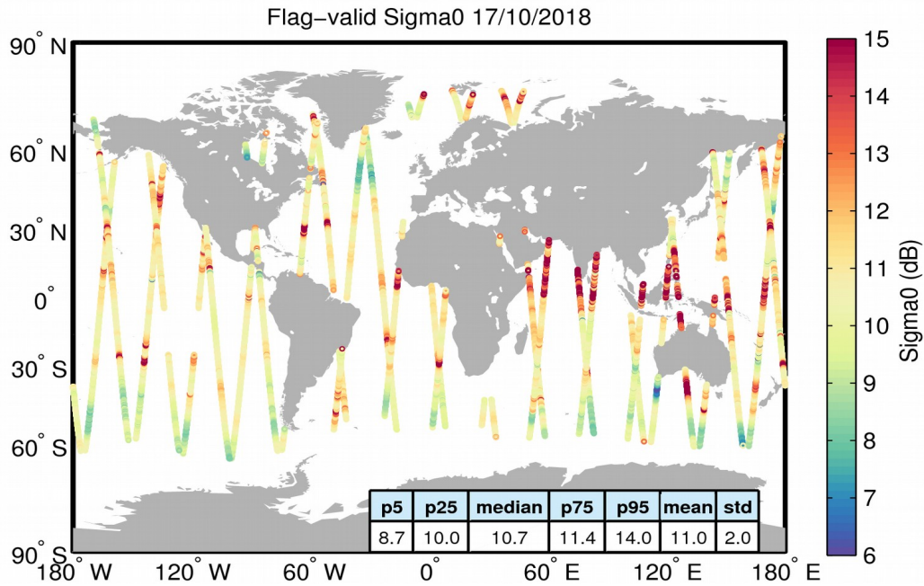
Figure 23. Geographical distribution of flag-valid sigma0 data over oceans and lakes for 17/10/2018. The statistical values shown in the table refer to the sigma0 in dB and are calculated over all measurements shown in the figure.
