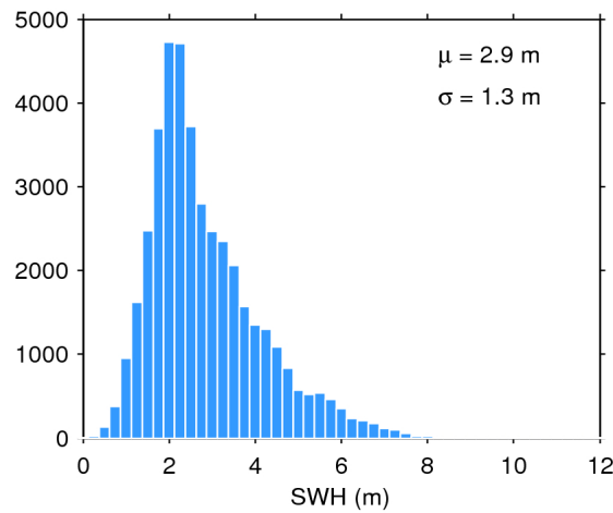
Figure 17. Histogram of flag-valid SWH over oceans and lakes for 17/10/2018. The mean ( \mu ) and standard deviation ( \sigma ) are also shown. Note that values larger than 12 m are excluded from the histogram for the sake of readability but not from the computation of \mu and \sigma .
