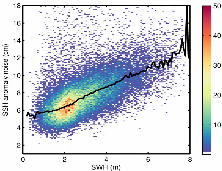
Figure 9. 2D histogram showing flag-valid SSH anomaly noise as a function of SWH for 17/10/2018. The black line denotes the median SSH anomaly noise as a function of SWH.
