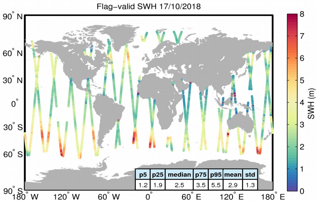
Figure 15. Geographical distribution of flag-valid SWH data over oceans and lakes for 17/10/2018. The statistical values shown in the table refer to the SWH in m and are calculated over all measurements shown in the figure.
