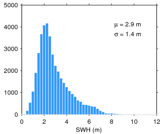
Figure 17. Histogram of flag-valid SWH over oceans and lakes for 16/10/2018. The mean ( \mu ) and standard deviation ( \sigma ) are also shown. Note that values larger than 12 m are excluded from the histogram for the sake of readability but not from the computation of \mu and \sigma .
