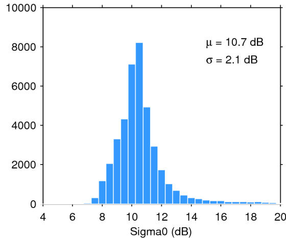
Figure 25. Histogram of flag-valid sigma0 over oceans and lakes for 16/10/2018. The mean ( \mu ) and standard deviation ( \sigma ) are also shown. Note that values outside [4 20] dB are excluded from the histogram for the sake of readability but not from the computation of \mu and \sigma .
