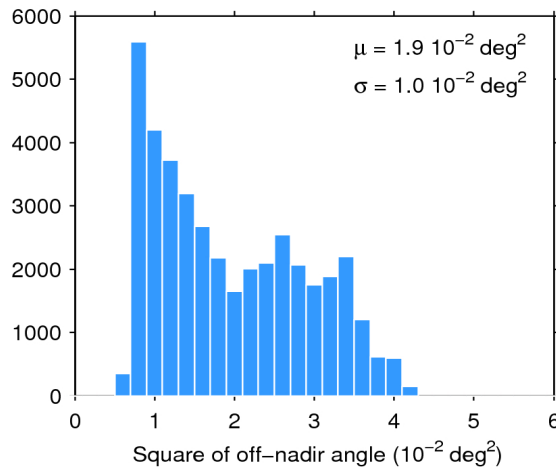
Figure 39. Histogram of flag-valid mispointing over oceans and lakes for 16/10/2018. The mean ( \mu ) and standard deviation ( \sigma ) are also shown. Note that values larger than 6 \cdot 10^{-2} \text{ deg}^2 are excluded from the histogram for the sake of readability but not from the computation of \mu and \sigma .
