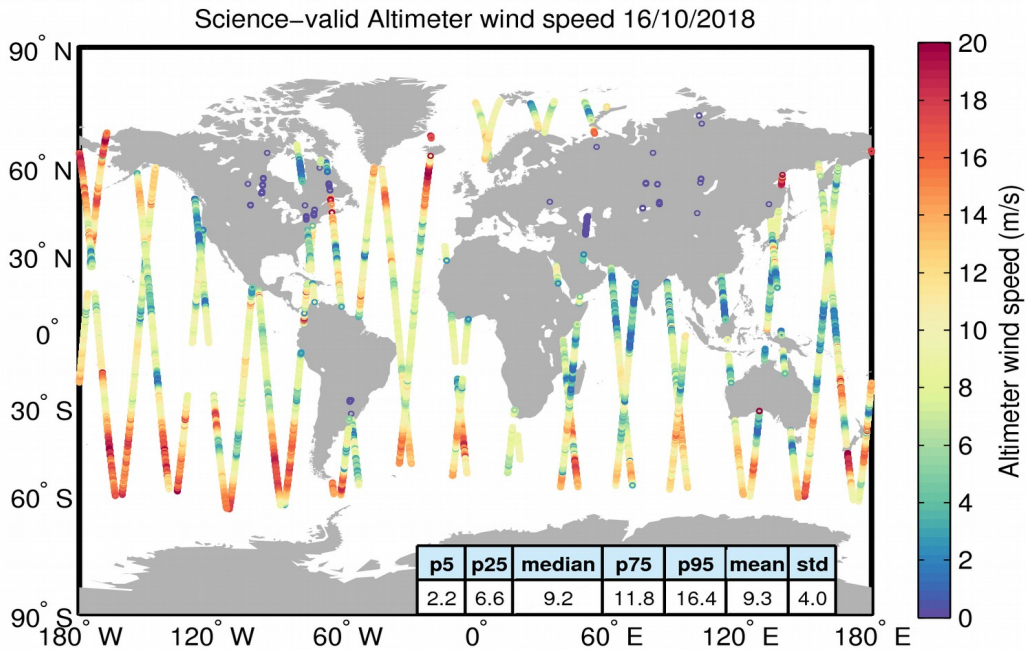
Figure 34. Geographical distribution of science-valid wind data over oceans and lakes for 16/10/2018. The statistical values shown in the table refer to the wind in m/s and are calculated over all measurements shown in the figure. Gray circles denote records that have been rejected based on the editing criteria described in Table 5.
