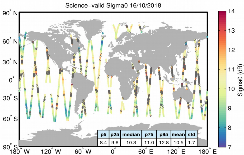
Figure 27. Geographical distribution of science-valid sigma0 data over oceans and lakes for 16/10/2018. The statistical values shown in the table refer to the sigma0 in dB and are calculated over all measurements shown in the figure. Gray circles denote records that have been rejected based on the editing criteria described in Table 4.
