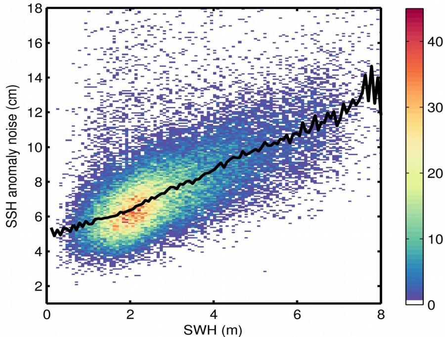
Figure 9. 2D histogram showing flag-valid SSH anomaly noise as a function of SWH for 16/10/2018. The black line denotes the median SSH anomaly noise as a function of SWH.
