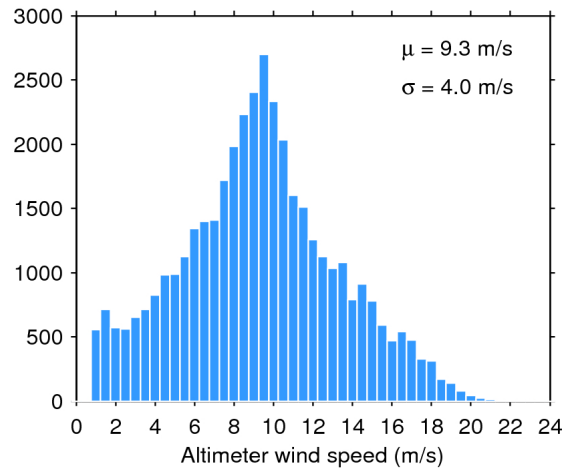
Figure 33. Histogram of flag-valid wind over oceans and lakes for 16/10/2018. The mean ( \mu ) and standard deviation ( \sigma ) are also shown. Note that values larger than 24 m/s are excluded from the histogram for the sake of readability but not from the computation of \mu and \sigma .
