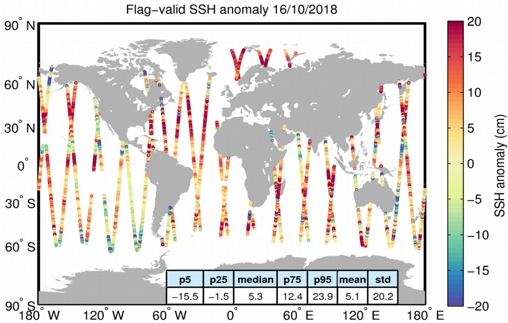
Figure 5. Geographical distribution of flag-valid 1-Hz SSH anomaly data over oceans and lakes for 16/10/2018. The statistical values shown in the table refer to the SSH anomaly in cm and are calculated over all measurements shown in the figure.
