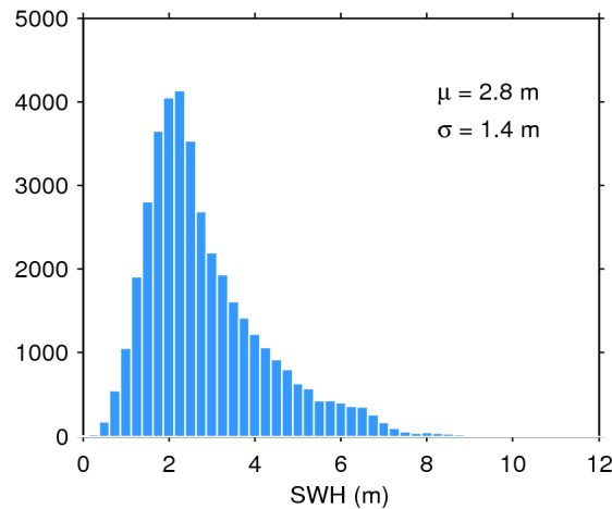
Figure 20. Histogram of science-valid SWH over oceans and lakes for 16/10/2018. The mean ( \mu ) and standard deviation ( \sigma ) are also shown. Note that values larger than 12 m are excluded from the histogram for the sake of readability but not from the computation of \mu and \sigma .
