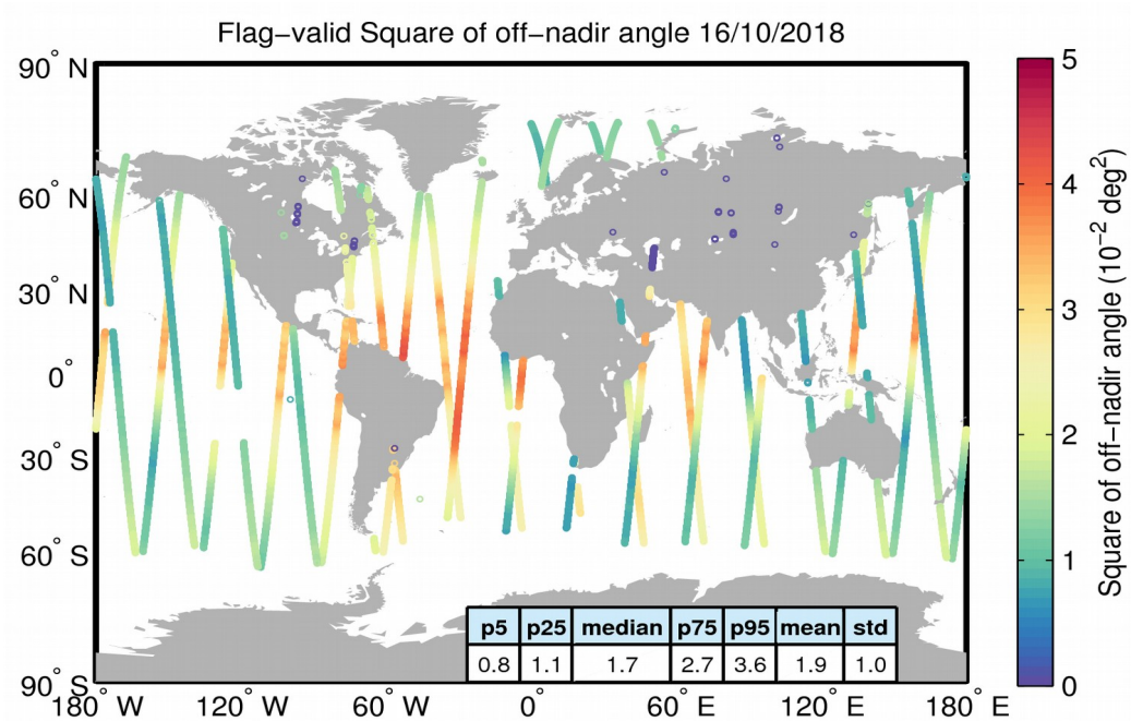
Figure 37. Geographical distribution of flag-valid mispointing data over oceans and lakes for 16/10/2018. The statistical values shown in the table refer to the mispointing in 10^{-2} deg 2 and are calculated over all measurements shown in the figure.
