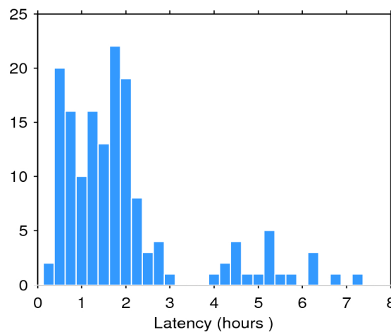
Figure 2. Histogram of the data latency for 16/10/2018. The y-axis denotes the number of files that are made available with a delay of x-hours with respect to the mean time of the records stored in the file.
