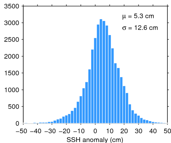
Figure 11. Histogram of science-valid SSH anomaly over oceans and lakes for 16/10/2018. The mean ( \mu ) and standard deviation ( \sigma ) are also shown. Note that values outside [-50 50] cm are excluded from the histogram for the sake of readability but not from the computation of \mu and \sigma .
