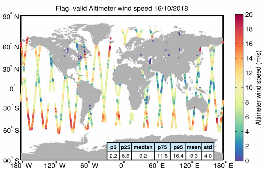
Figure 31. Geographical distribution of flag-valid wind data over oceans and lakes for 16/10/2018. The statistical values shown in the table refer to the wind in m/s and are calculated over all measurements shown in the figure.
