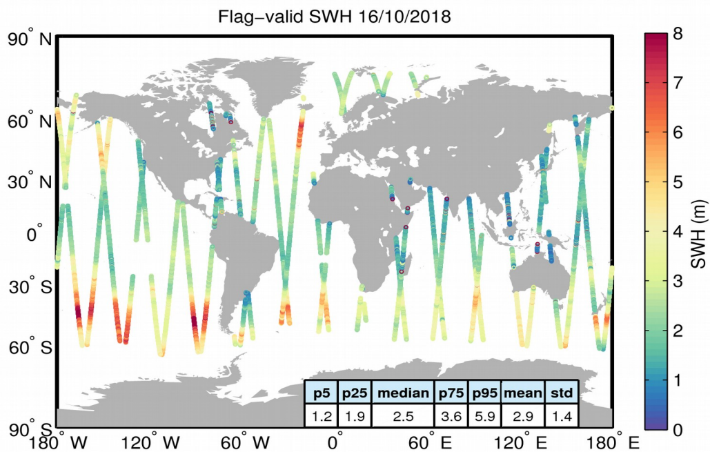
Figure 15. Geographical distribution of flag-valid SWH data over oceans and lakes for 16/10/2018. The statistical values shown in the table refer to the SWH in m and are calculated over all measurements shown in the figure.
