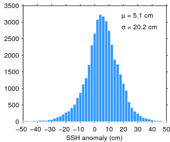
Figure 7. Histogram of flag-valid SSH anomaly over oceans and lakes for 16/10/2018. The mean ( \mu ) and standard deviation ( \sigma ) are also shown. Note that values outside [-50\ 50] cm are excluded from the histogram for the sake of readability but not from the computation of \mu and \sigma .
