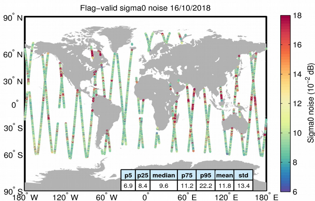
Figure 26. Geographical distribution of flag-valid 20-Hz sigma0 measurement noise over oceans and lakes for 16/10/2018. The statistical values shown in the table refer to the sigma0 noise and are calculated over all measurements shown in the figure.
