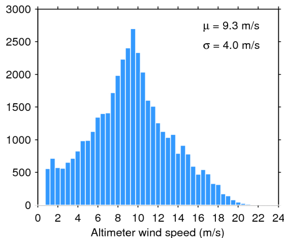
Figure 35. Histogram of science-valid wind over oceans and lakes for 16/10/2018. The mean ( \mu ) and standard deviation ( \sigma ) are also shown. Note that values larger than 24 m/s are excluded from the histogram for the sake of readability but not from the computation of \mu and \sigma .
