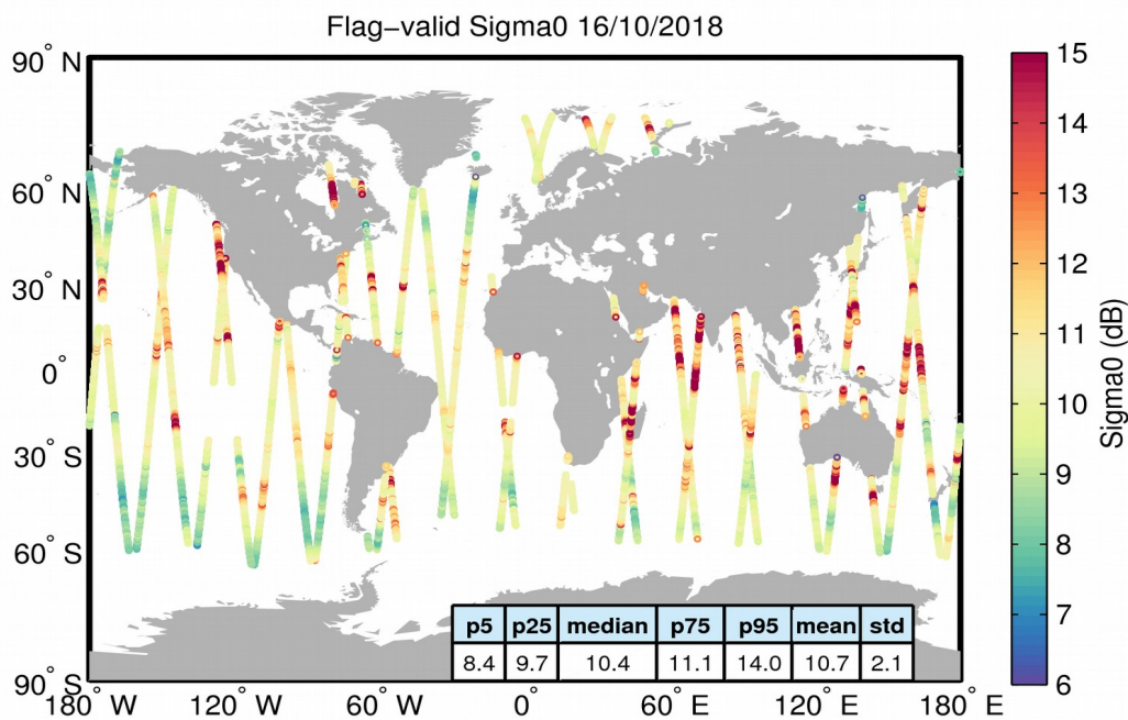
Figure 23. Geographical distribution of flag-valid sigma0 data over oceans and lakes for 16/10/2018. The statistical values shown in the table refer to the sigma0 in dB and are calculated over all measurements shown in the figure.
