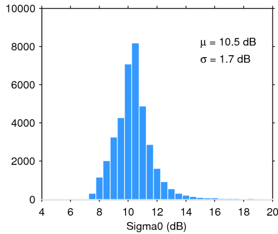
Figure 28. Histogram of science-valid sigma0 over oceans and lakes for 16/10/2018. The mean ( \mu ) and standard deviation ( \sigma ) are also shown. Note that values outside [4 20] dB are excluded from the histogram for the sake of readability but not from the computation of \mu and \sigma .
