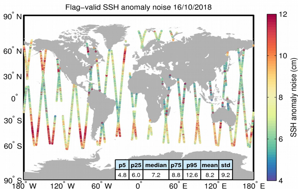
Figure 8. Geographical distribution of flag-valid 20-Hz SSH anomaly measurement noise over oceans and lakes for 16/10/2018. The statistical values shown in the table refer to the SSH anomaly noise and are calculated over all measurements shown in the figure.
