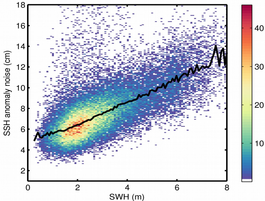
Figure 9. 2D histogram showing flag-valid SSH anomaly noise as a function of SWH for 15/10/2018. The black line denotes the median SSH anomaly noise as a function of SWH.
