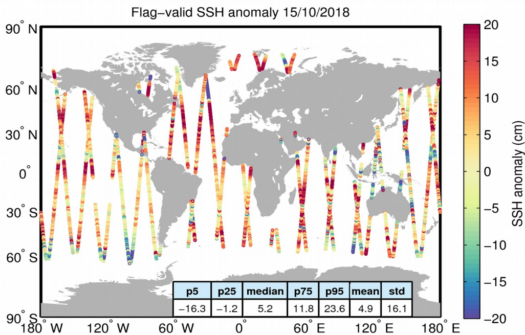
Figure 5. Geographical distribution of flag-valid 1-Hz SSH anomaly data over oceans and lakes for 15/10/2018. The statistical values shown in the table refer to the SSH anomaly in cm and are calculated over all measurements shown in the figure.
