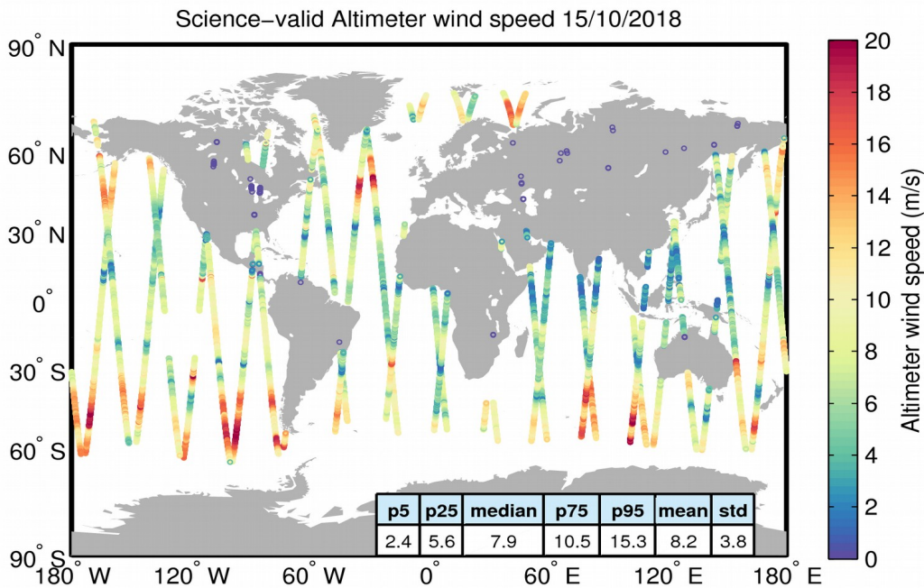
Figure 34. Geographical distribution of science-valid wind data over oceans and lakes for 15/10/2018. The statistical values shown in the table refer to the wind in m/s and are calculated over all measurements shown in the figure. Gray circles denote records that have been rejected based on the editing criteria described in Table 5.
