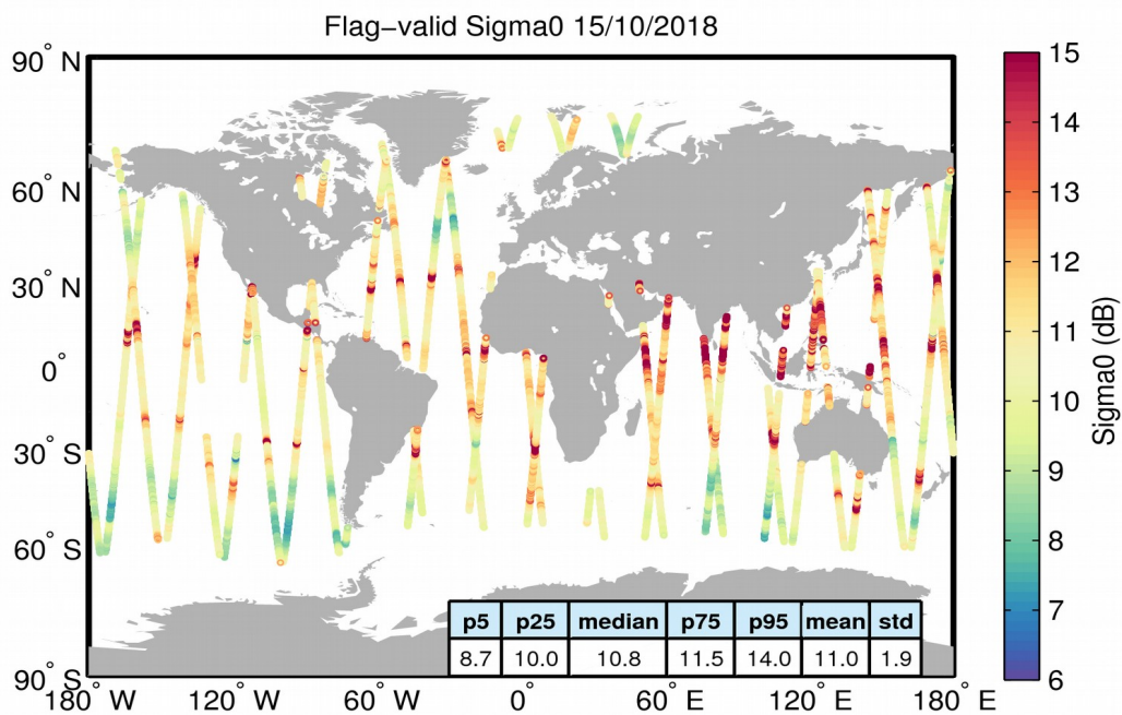
Figure 23. Geographical distribution of flag-valid sigma0 data over oceans and lakes for 15/10/2018. The statistical values shown in the table refer to the sigma0 in dB and are calculated over all measurements shown in the figure.
