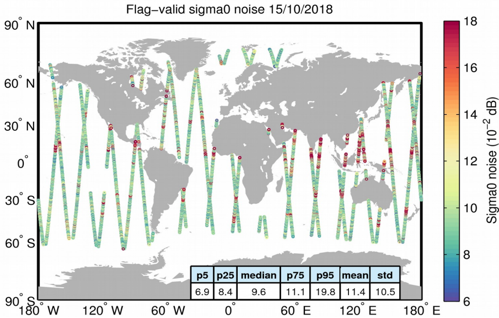
Figure 26. Geographical distribution of flag-valid 20-Hz sigma0 measurement noise over oceans and lakes for 15/10/2018. The statistical values shown in the table refer to the sigma0 noise and are calculated over all measurements shown in the figure.
