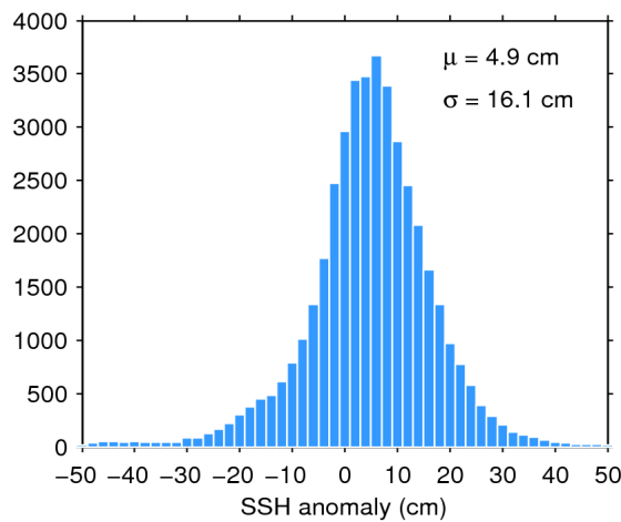
Figure 7. Histogram of flag-valid SSH anomaly over oceans and lakes for 15/10/2018. The mean ( \mu ) and standard deviation ( \sigma ) are also shown. Note that values outside [-50\ 50] cm are excluded from the histogram for the sake of readability but not from the computation of \mu and \sigma .
