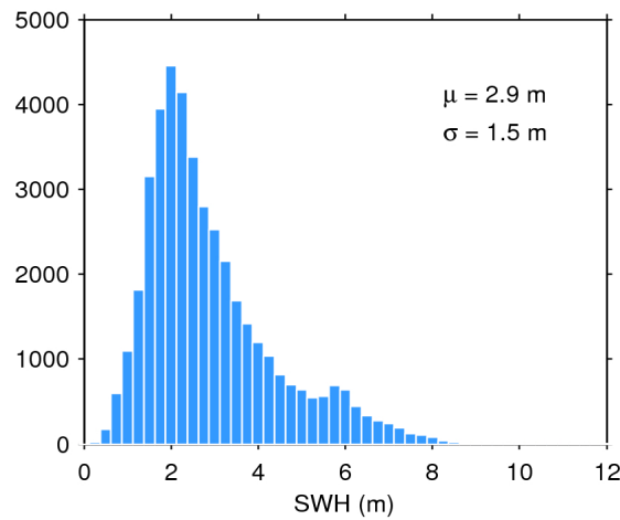
Figure 17. Histogram of flag-valid SWH over oceans and lakes for 15/10/2018. The mean ( \mu ) and standard deviation ( \sigma ) are also shown. Note that values larger than 12 m are excluded from the histogram for the sake of readability but not from the computation of \mu and \sigma .
