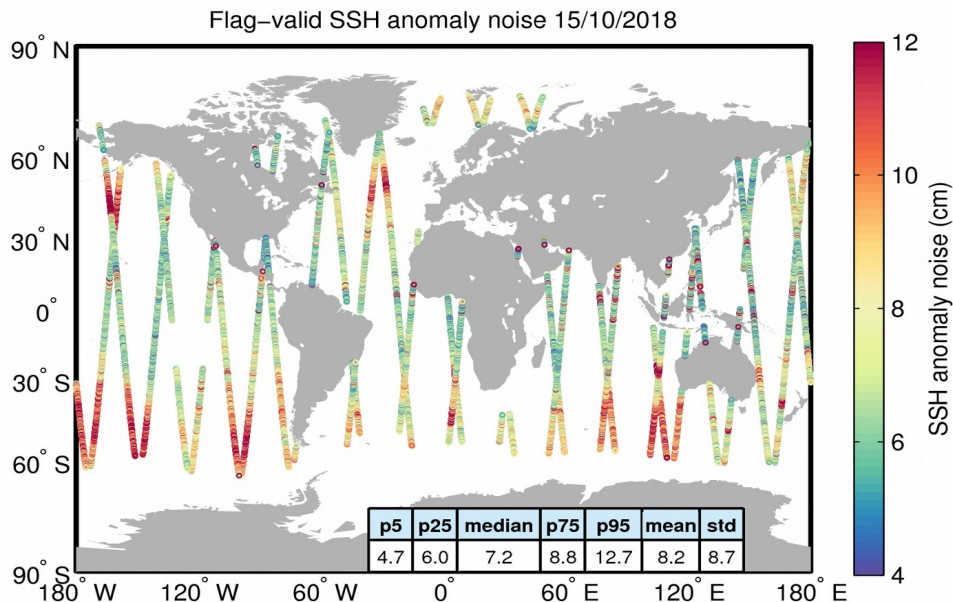
Figure 8. Geographical distribution of flag-valid 20-Hz SSH anomaly measurement noise over oceans and lakes for 15/10/2018. The statistical values shown in the table refer to the SSH anomaly noise and are calculated over all measurements shown in the figure.
