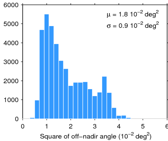
Figure 39. Histogram of flag-valid mispointing over oceans and lakes for 15/10/2018. The mean ( \mu ) and standard deviation ( \sigma ) are also shown. Note that values larger than 6 \cdot 10^{-2} \text{ deg}^2 are excluded from the histogram for the sake of readability but not from the computation of \mu and \sigma .
