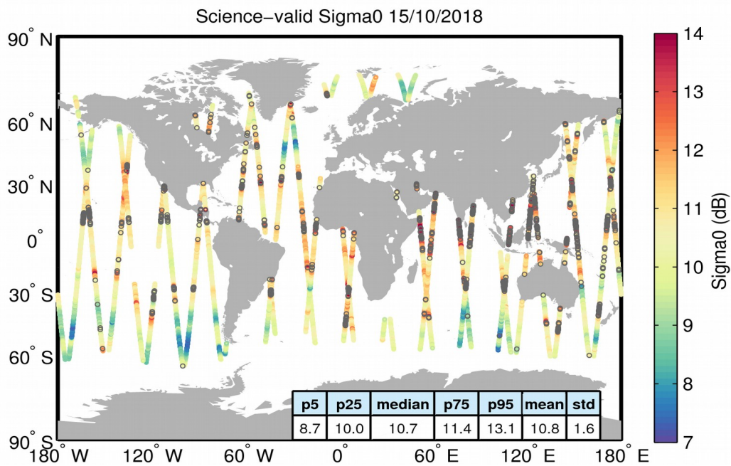
Figure 27. Geographical distribution of science-valid sigma0 data over oceans and lakes for 15/10/2018. The statistical values shown in the table refer to the sigma0 in dB and are calculated over all measurements shown in the figure. Gray circles denote records that have been rejected based on the editing criteria described in Table 4.
