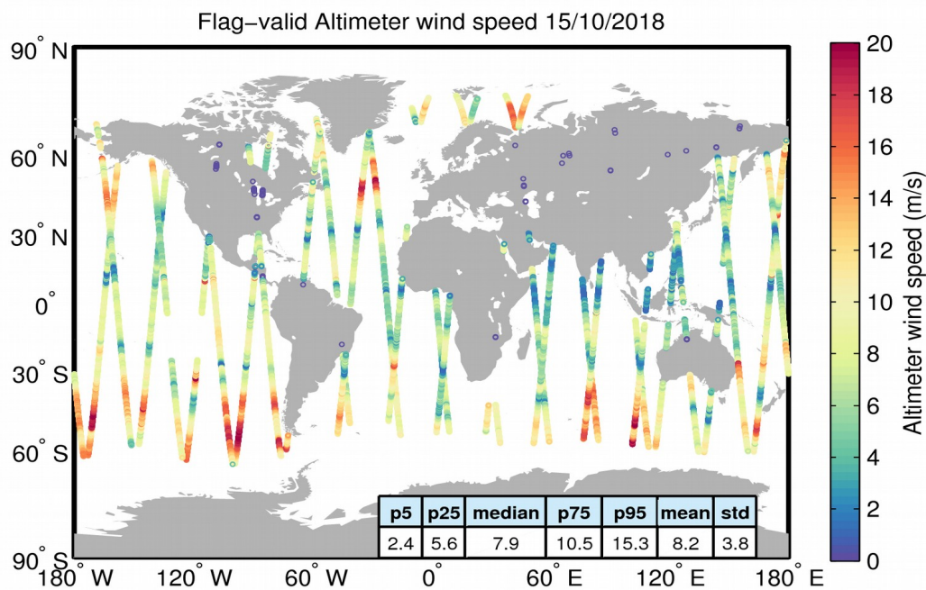
Figure 31. Geographical distribution of flag-valid wind data over oceans and lakes for 15/10/2018. The statistical values shown in the table refer to the wind in m/s and are calculated over all measurements shown in the figure.
