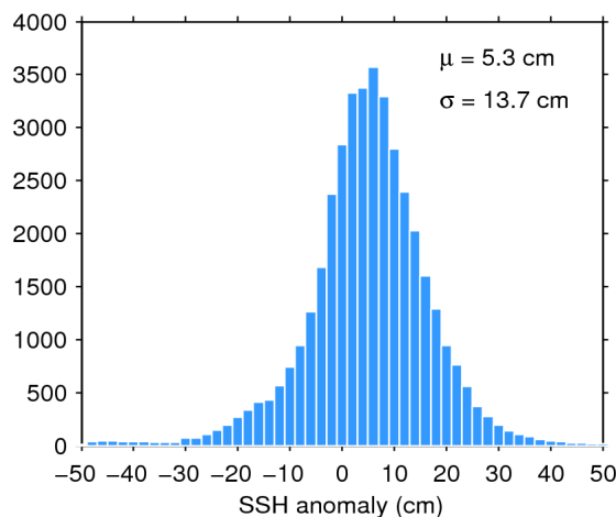
Figure 11. Histogram of science-valid SSH anomaly over oceans and lakes for 15/10/2018. The mean ( \mu ) and standard deviation ( \sigma ) are also shown. Note that values outside [-50 50] cm are excluded from the histogram for the sake of readability but not from the computation of \mu and \sigma .
