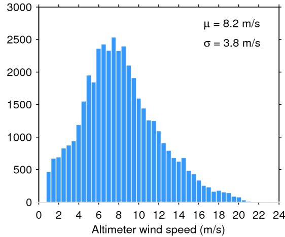
Figure 33. Histogram of flag-valid wind over oceans and lakes for 15/10/2018. The mean ( \mu ) and standard deviation ( \sigma ) are also shown. Note that values larger than 24 m/s are excluded from the histogram for the sake of readability but not from the computation of \mu and \sigma .
