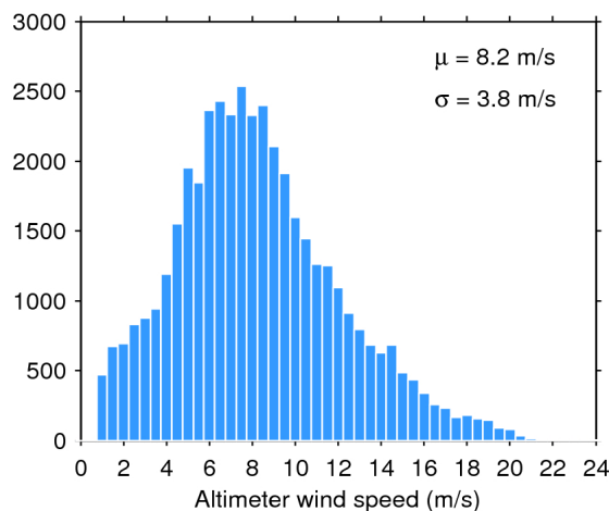
Figure 35. Histogram of science-valid wind over oceans and lakes for 15/10/2018. The mean ( \mu ) and standard deviation ( \sigma ) are also shown. Note that values larger than 24 m/s are excluded from the histogram for the sake of readability but not from the computation of \mu and \sigma .
