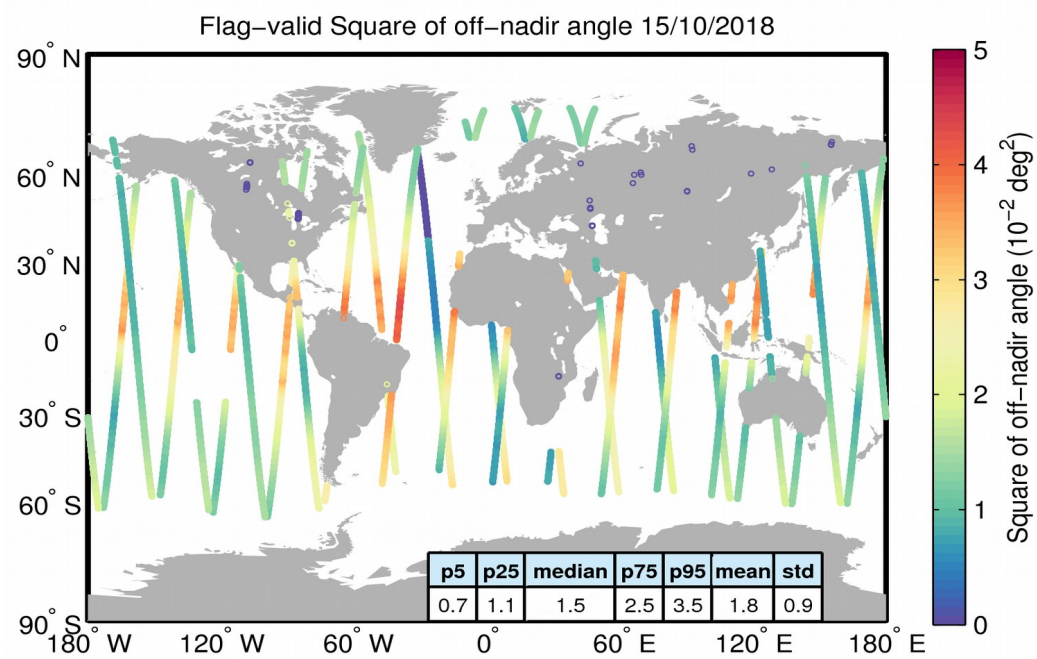
Figure 37. Geographical distribution of flag-valid mispointing data over oceans and lakes for 15/10/2018. The statistical values shown in the table refer to the mispointing in 10^{-2} \text{ deg}^2 and are calculated over all measurements shown in the figure.
