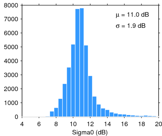
Figure 25. Histogram of flag-valid sigma0 over oceans and lakes for 15/10/2018. The mean ( \mu ) and standard deviation ( \sigma ) are also shown. Note that values outside [4 20] dB are excluded from the histogram for the sake of readability but not from the computation of \mu and \sigma .
