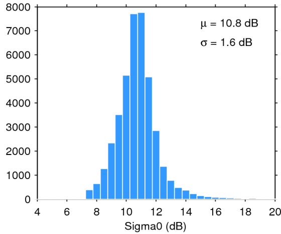
Figure 28. Histogram of science-valid sigma0 over oceans and lakes for 15/10/2018. The mean ( \mu ) and standard deviation ( \sigma ) are also shown. Note that values outside [4 20] dB are excluded from the histogram for the sake of readability but not from the computation of \mu and \sigma .
