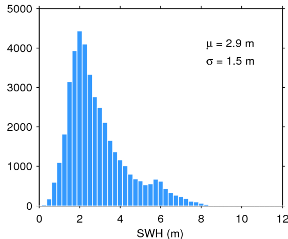
Figure 20. Histogram of science-valid SWH over oceans and lakes for 15/10/2018. The mean ( \mu ) and standard deviation ( \sigma ) are also shown. Note that values larger than 12 m are excluded from the histogram for the sake of readability but not from the computation of \mu and \sigma .
