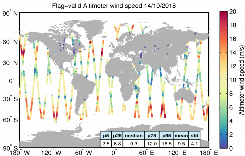
Figure 31. Geographical distribution of flag-valid wind data over oceans and lakes for 14/10/2018. The statistical values shown in the table refer to the wind in m/s and are calculated over all measurements shown in the figure.
