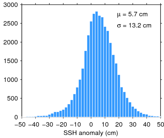
Figure 11. Histogram of science-valid SSH anomaly over oceans and lakes for 14/10/2018. The mean ( \mu ) and standard deviation ( \sigma ) are also shown. Note that values outside [-50 50] cm are excluded from the histogram for the sake of readability but not from the computation of \mu and \sigma .
