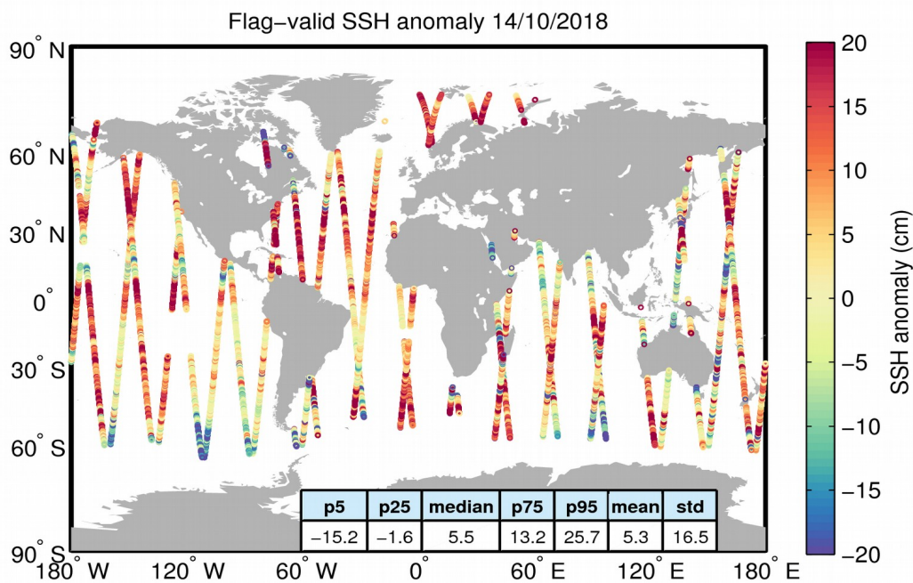
Figure 5. Geographical distribution of flag-valid 1-Hz SSH anomaly data over oceans and lakes for 14/10/2018. The statistical values shown in the table refer to the SSH anomaly in cm and are calculated over all measurements shown in the figure.
