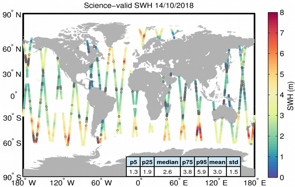
Figure 19. Geographical distribution of science-valid SWH data over oceans and lakes for 14/10/2018. The statistical values shown in the table refer to the SWH in m and are calculated over all measurements shown in the figure. Gray circles denote records that have been rejected based on the editing criteria described in Table 3.
