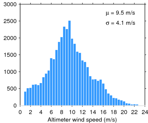
Figure 33. Histogram of flag-valid wind over oceans and lakes for 14/10/2018. The mean ( \mu ) and standard deviation ( \sigma ) are also shown. Note that values larger than 24 m/s are excluded from the histogram for the sake of readability but not from the computation of \mu and \sigma .
