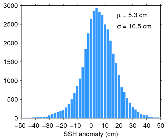
Figure 7. Histogram of flag-valid SSH anomaly over oceans and lakes for 14/10/2018. The mean ( \mu ) and standard deviation ( \sigma ) are also shown. Note that values outside [-50 50] cm are excluded from the histogram for the sake of readability but not from the computation of \mu and \sigma .
