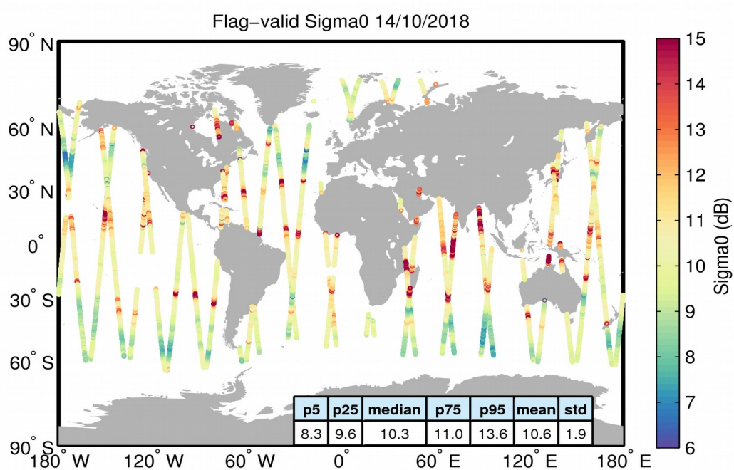
Figure 23. Geographical distribution of flag-valid sigma0 data over oceans and lakes for 14/10/2018. The statistical values shown in the table refer to the sigma0 in dB and are calculated over all measurements shown in the figure.
