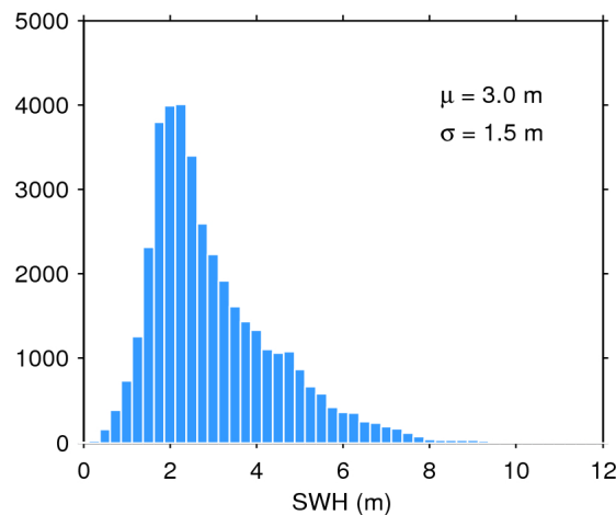
Figure 20. Histogram of science-valid SWH over oceans and lakes for 14/10/2018. The mean ( \mu ) and standard deviation ( \sigma ) are also shown. Note that values larger than 12 m are excluded from the histogram for the sake of readability but not from the computation of \mu and \sigma .
