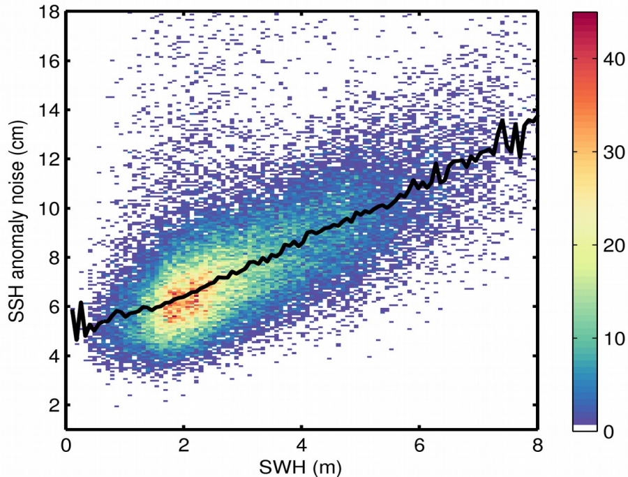
Figure 9. 2D histogram showing flag-valid SSH anomaly noise as a function of SWH for 14/10/2018. The black line denotes the median SSH anomaly noise as a function of SWH.
