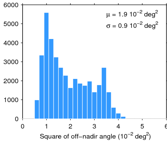
Figure 39. Histogram of flag-valid mispointing over oceans and lakes for 14/10/2018. The mean ( \mu ) and standard deviation ( \sigma ) are also shown. Note that values larger than 6 \cdot 10^{-2} \text{ deg}^2 are excluded from the histogram for the sake of readability but not from the computation of \mu and \sigma .
