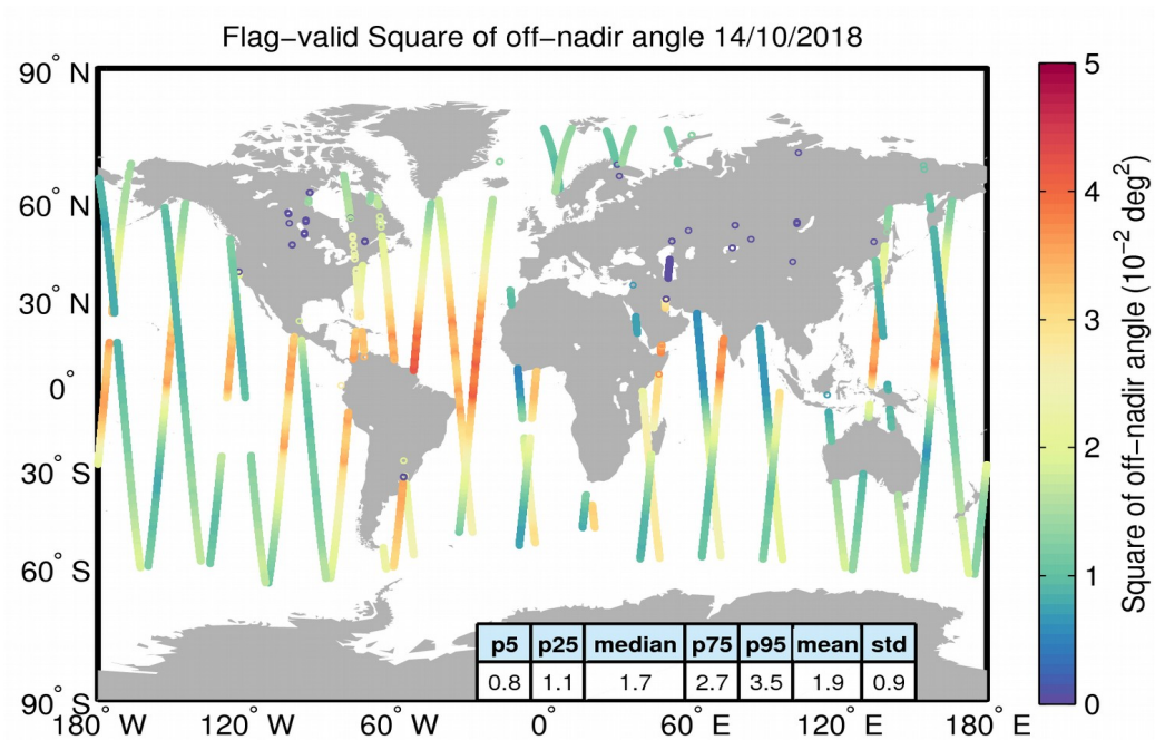
Figure 37. Geographical distribution of flag-valid mispointing data over oceans and lakes for 14/10/2018. The statistical values shown in the table refer to the mispointing in 10^{-2} deg 2 and are calculated over all measurements shown in the figure.
