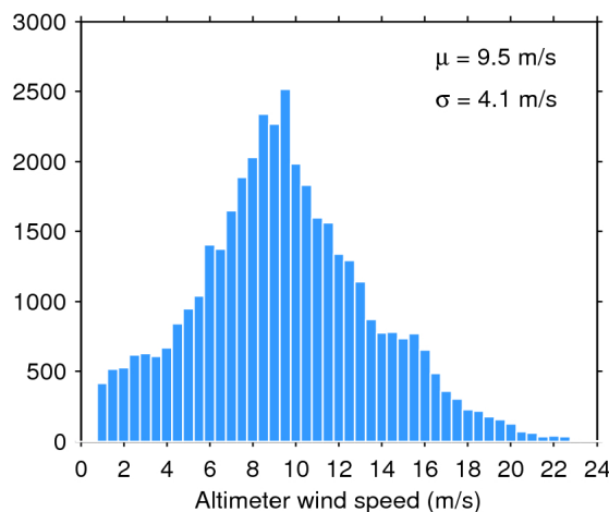
Figure 35. Histogram of science-valid wind over oceans and lakes for 14/10/2018. The mean ( \mu ) and standard deviation ( \sigma ) are also shown. Note that values larger than 24 m/s are excluded from the histogram for the sake of readability but not from the computation of \mu and \sigma .
