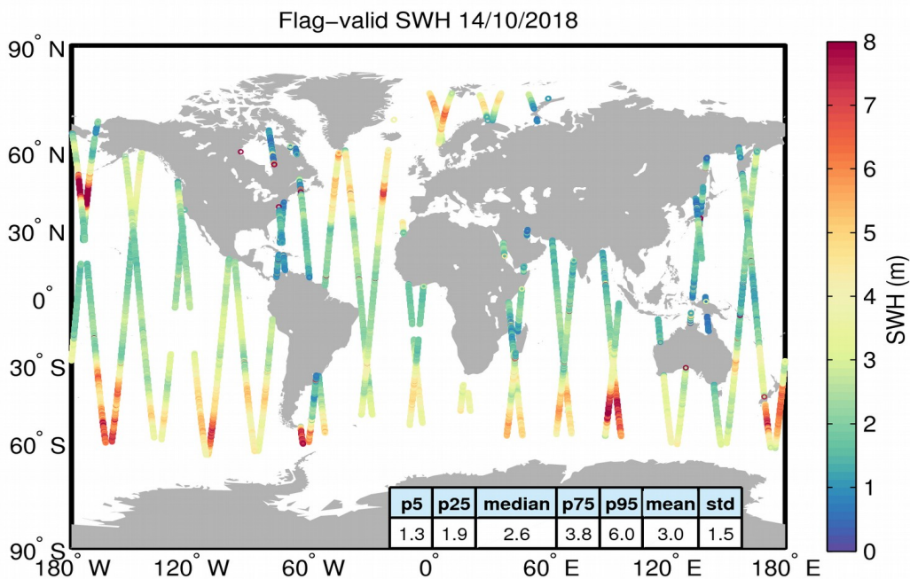
Figure 15. Geographical distribution of flag-valid SWH data over oceans and lakes for 14/10/2018. The statistical values shown in the table refer to the SWH in m and are calculated over all measurements shown in the figure.
