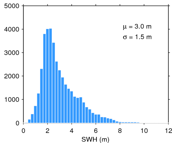
Figure 17. Histogram of flag-valid SWH over oceans and lakes for 14/10/2018. The mean ( \mu ) and standard deviation ( \sigma ) are also shown. Note that values larger than 12 m are excluded from the histogram for the sake of readability but not from the computation of \mu and \sigma .
