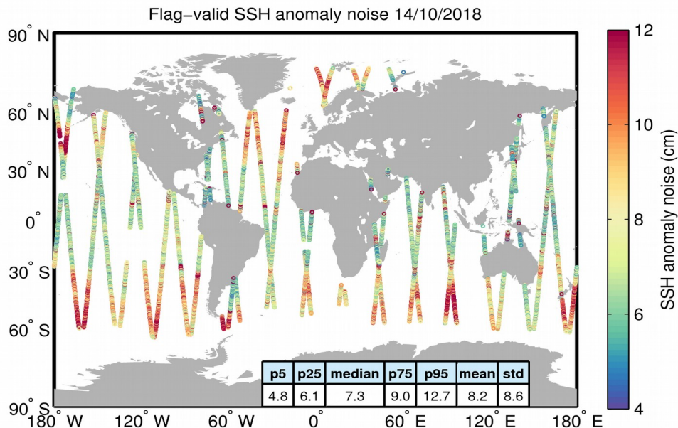
Figure 8. Geographical distribution of flag-valid 20-Hz SSH anomaly measurement noise over oceans and lakes for 14/10/2018. The statistical values shown in the table refer to the SSH anomaly noise and are calculated over all measurements shown in the figure.
