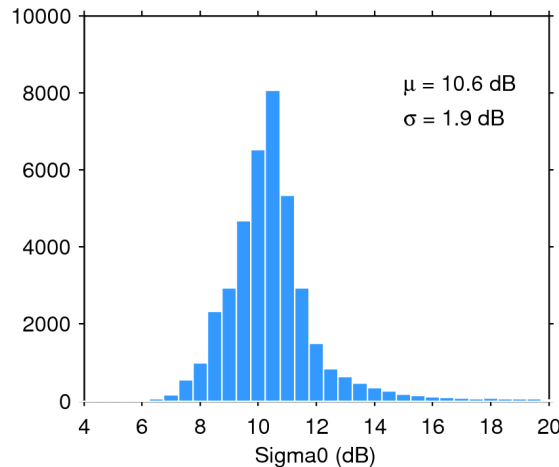
Figure 25. Histogram of flag-valid sigma0 over oceans and lakes for 14/10/2018. The mean ( \mu ) and standard deviation ( \sigma ) are also shown. Note that values outside [4 20] dB are excluded from the histogram for the sake of readability but not from the computation of \mu and \sigma .
