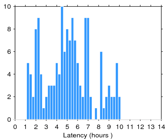
Figure 2. Histogram of the data latency for 14/10/2018. The y-axis denotes the number of files that are made available with a delay of x-hours with respect to the mean time of the records stored in the file.
