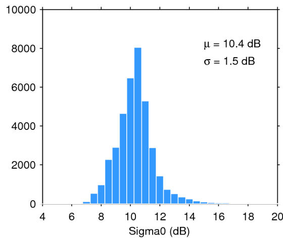
Figure 28. Histogram of science-valid sigma0 over oceans and lakes for 14/10/2018. The mean ( \mu ) and standard deviation ( \sigma ) are also shown. Note that values outside [4 20] dB are excluded from the histogram for the sake of readability but not from the computation of \mu and \sigma .
