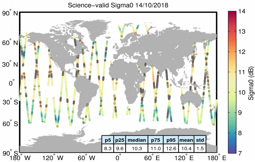
Figure 27. Geographical distribution of science-valid sigma0 data over oceans and lakes for 14/10/2018. The statistical values shown in the table refer to the sigma0 in dB and are calculated over all measurements shown in the figure. Gray circles denote records that have been rejected based on the editing criteria described in Table 4.
