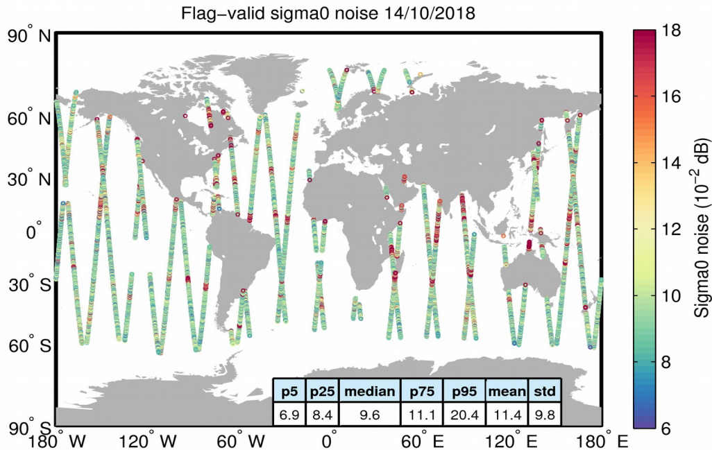
Figure 26. Geographical distribution of flag-valid 20-Hz sigma0 measurement noise over oceans and lakes for 14/10/2018. The statistical values shown in the table refer to the sigma0 noise and are calculated over all measurements shown in the figure.
