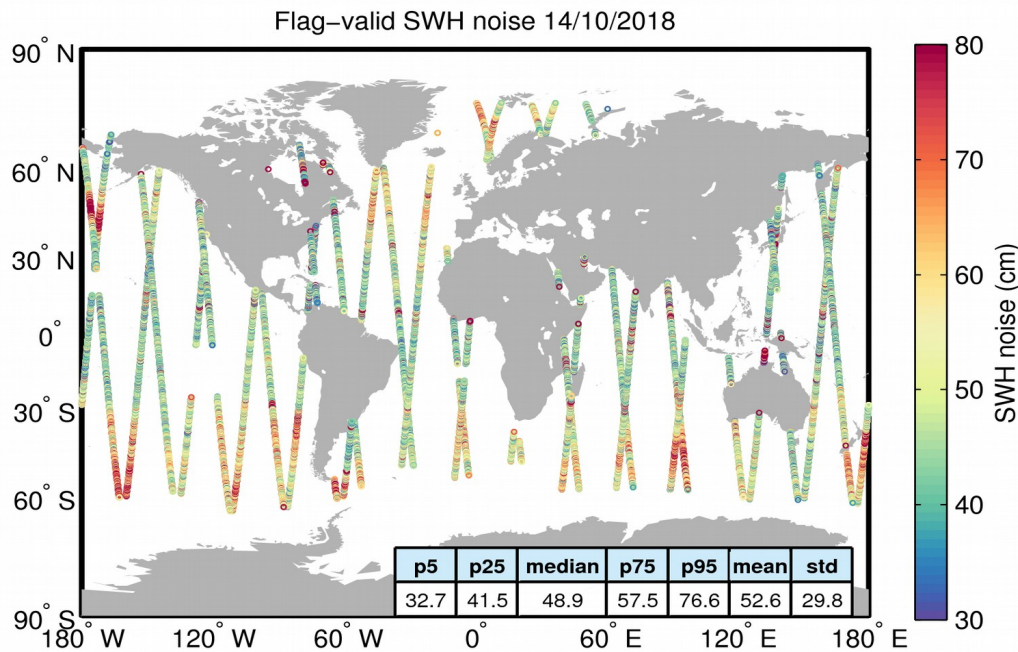
Figure 18. Geographical distribution of flag-valid 20-Hz SWH measurement noise over oceans and lakes for 14/10/2018. The statistical values shown in the figure refer to the SWH noise and are calculated over all measurements shown in the figure.
