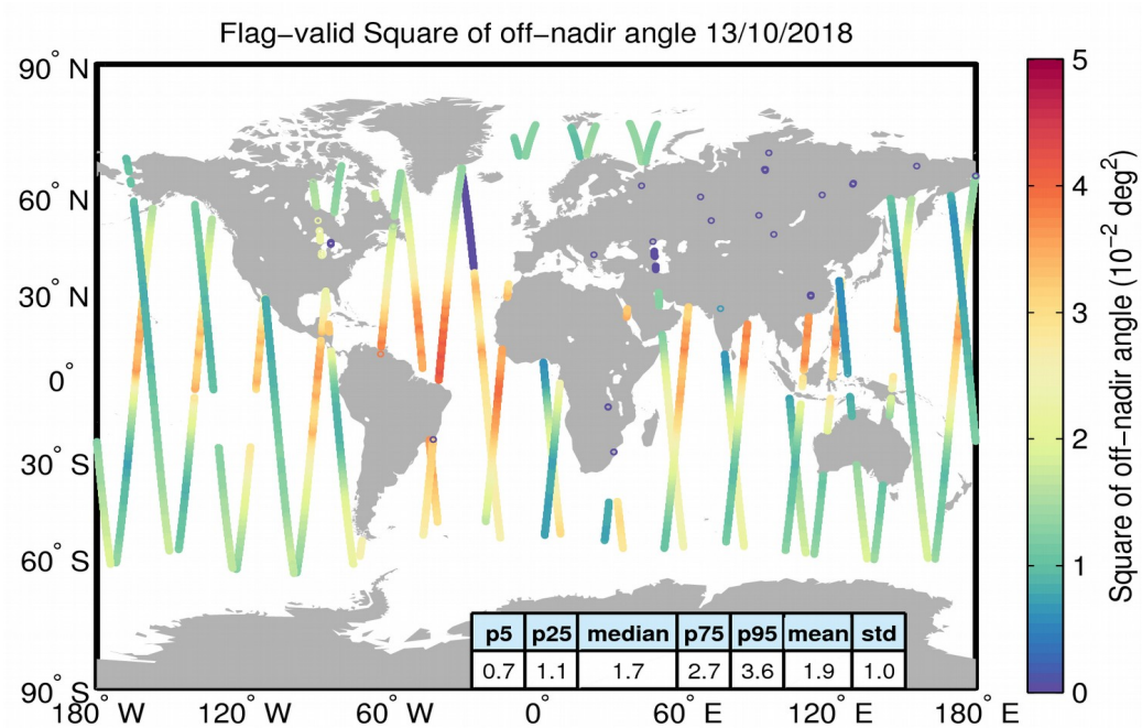
Figure 37. Geographical distribution of flag-valid mispointing data over oceans and lakes for 13/10/2018. The statistical values shown in the table refer to the mispointing in 10^{-2} \text{ deg}^2 and are calculated over all measurements shown in the figure.
