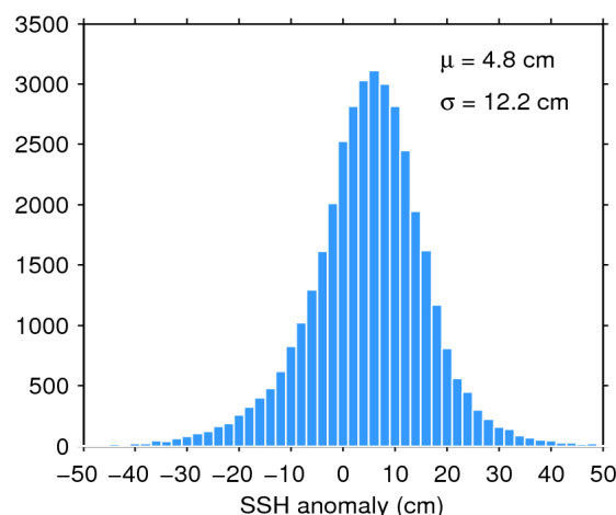
Figure 11. Histogram of science-valid SSH anomaly over oceans and lakes for 13/10/2018. The mean ( \mu ) and standard deviation ( \sigma ) are also shown. Note that values outside [-50 50] cm are excluded from the histogram for the sake of readability but not from the computation of \mu and \sigma .
