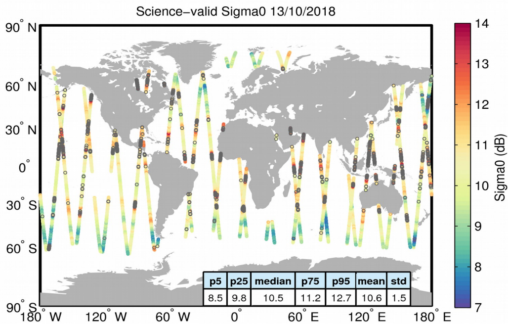
Figure 27. Geographical distribution of science-valid sigma0 data over oceans and lakes for 13/10/2018. The statistical values shown in the table refer to the sigma0 in dB and are calculated over all measurements shown in the figure. Gray circles denote records that have been rejected based on the editing criteria described in Table 4.
