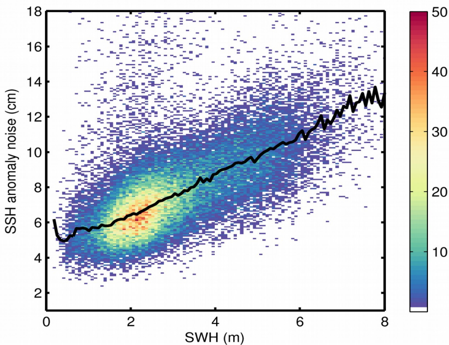
Figure 9. 2D histogram showing flag-valid SSH anomaly noise as a function of SWH for 13/10/2018. The black line denotes the median SSH anomaly noise as a function of SWH.
