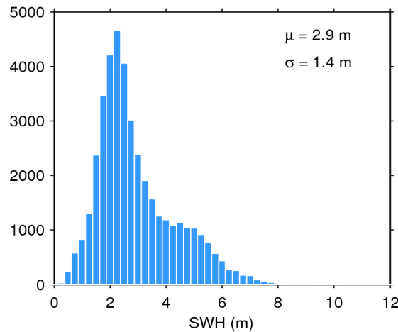
Figure 20. Histogram of science-valid SWH over oceans and lakes for 13/10/2018. The mean ( \mu ) and standard deviation ( \sigma ) are also shown. Note that values larger than 12 m are excluded from the histogram for the sake of readability but not from the computation of \mu and \sigma .
