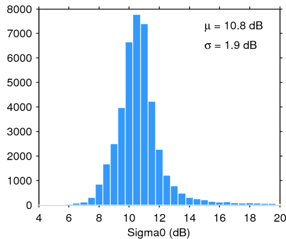
Figure 25. Histogram of flag-valid sigma0 over oceans and lakes for 13/10/2018. The mean ( \mu ) and standard deviation ( \sigma ) are also shown. Note that values outside [4 20] dB are excluded from the histogram for the sake of readability but not from the computation of \mu and \sigma .
