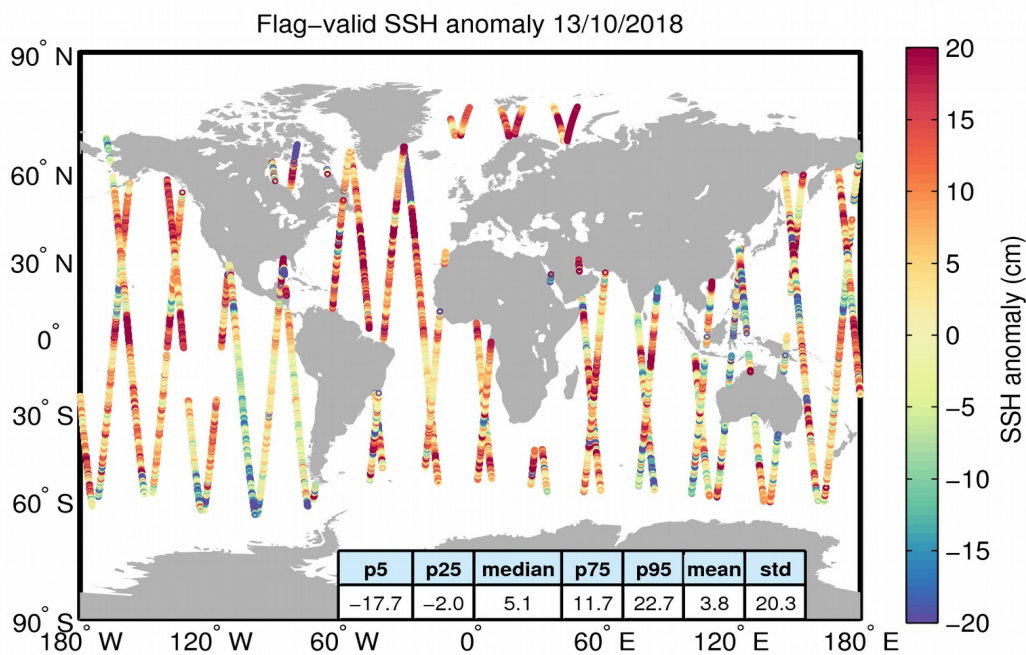
Figure 5. Geographical distribution of flag-valid 1-Hz SSH anomaly data over oceans and lakes for 13/10/2018. The statistical values shown in the table refer to the SSH anomaly in cm and are calculated over all measurements shown in the figure.
