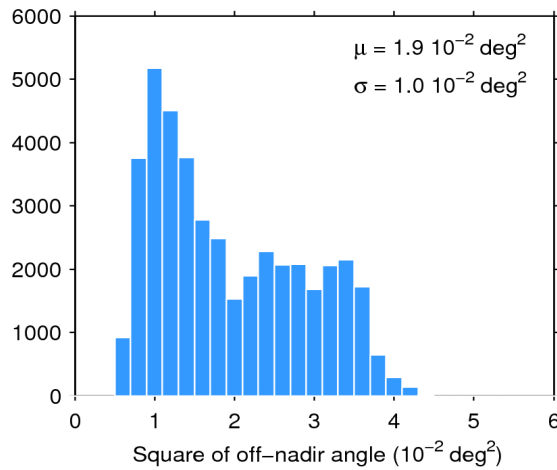
Figure 39. Histogram of flag-valid mispointing over oceans and lakes for 13/10/2018. The mean ( \mu ) and standard deviation ( \sigma ) are also shown. Note that values larger than 6 \cdot 10^{-2} \text{ deg}^2 are excluded from the histogram for the sake of readability but not from the computation of \mu and \sigma .
