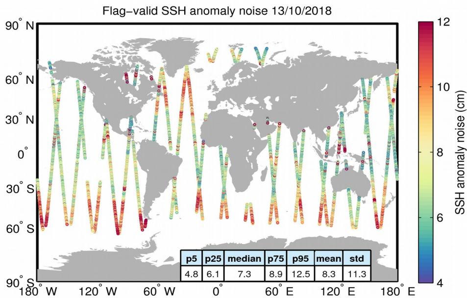
Figure 8. Geographical distribution of flag-valid 20-Hz SSH anomaly measurement noise over oceans and lakes for 13/10/2018. The statistical values shown in the table refer to the SSH anomaly noise and are calculated over all measurements shown in the figure.
