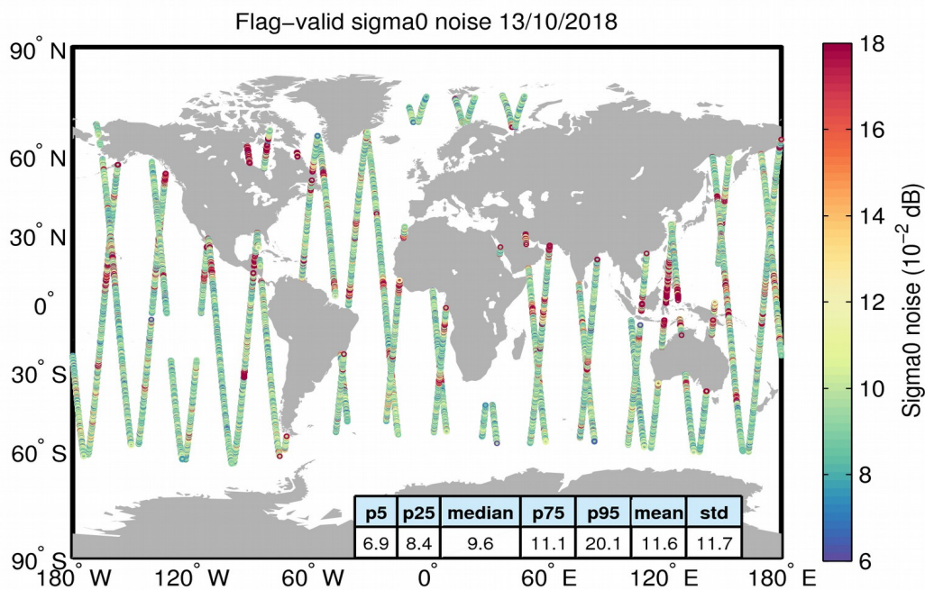
Figure 26. Geographical distribution of flag-valid 20-Hz sigma0 measurement noise over oceans and lakes for 13/10/2018. The statistical values shown in the table refer to the sigma0 noise and are calculated over all measurements shown in the figure.
