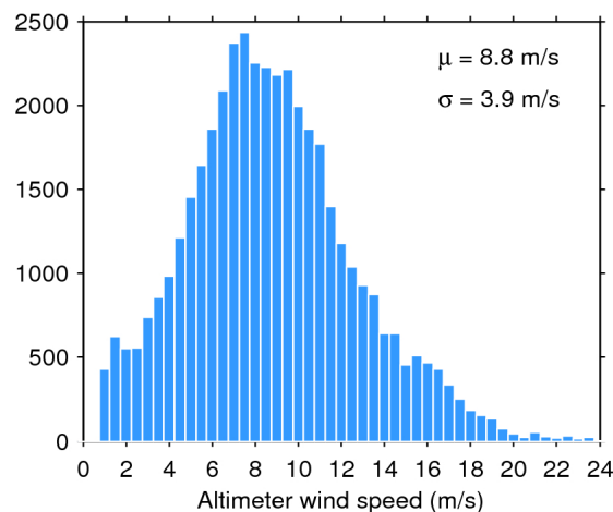
Figure 35. Histogram of science-valid wind over oceans and lakes for 13/10/2018. The mean ( \mu ) and standard deviation ( \sigma ) are also shown. Note that values larger than 24 m/s are excluded from the histogram for the sake of readability but not from the computation of \mu and \sigma .
