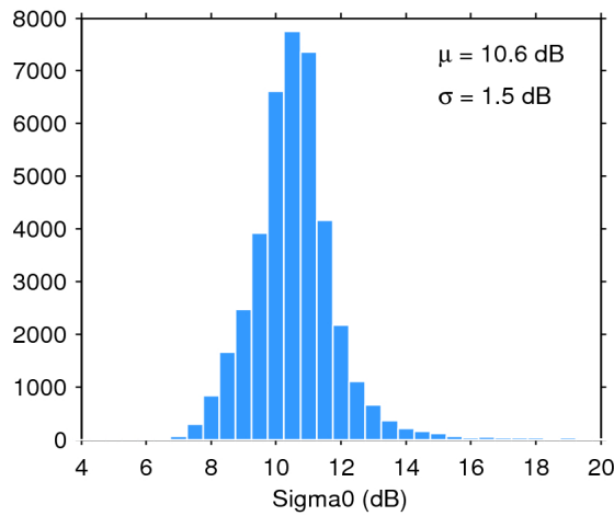
Figure 28. Histogram of science-valid sigma0 over oceans and lakes for 13/10/2018. The mean ( \mu ) and standard deviation ( \sigma ) are also shown. Note that values outside [4 20] dB are excluded from the histogram for the sake of readability but not from the computation of \mu and \sigma .
