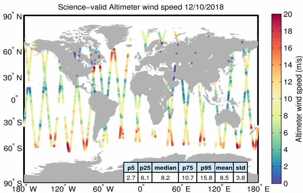
Figure 34. Geographical distribution of science-valid wind data over oceans and lakes for 12/10/2018. The statistical values shown in the table refer to the wind in m/s and are calculated over all measurements shown in the figure. Gray circles denote records that have been rejected based on the editing criteria described in Table 5.
