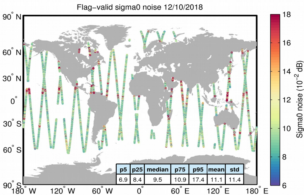
Figure 26. Geographical distribution of flag-valid 20-Hz sigma0 measurement noise over oceans and lakes for 12/10/2018. The statistical values shown in the table refer to the sigma0 noise and are calculated over all measurements shown in the figure.
