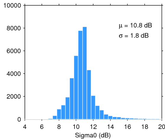
Figure 25. Histogram of flag-valid sigma0 over oceans and lakes for 12/10/2018. The mean ( \mu ) and standard deviation ( \sigma ) are also shown. Note that values outside [4 20] dB are excluded from the histogram for the sake of readability but not from the computation of \mu and \sigma .
