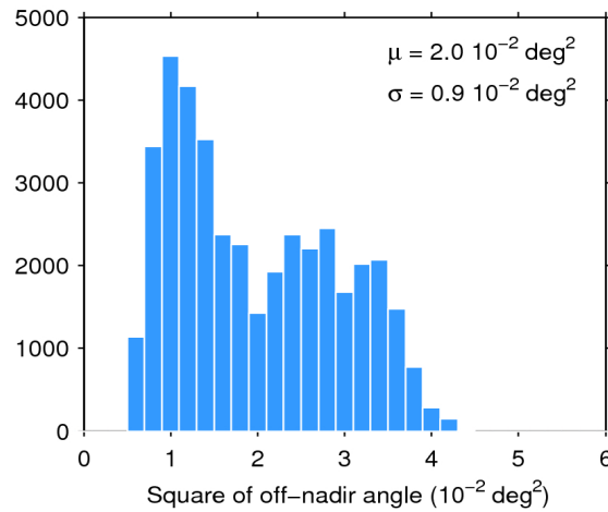
Figure 39. Histogram of flag-valid mispointing over oceans and lakes for 12/10/2018. The mean ( \mu ) and standard deviation ( \sigma ) are also shown. Note that values larger than 6 \cdot 10^{-2} \text{ deg}^2 are excluded from the histogram for the sake of readability but not from the computation of \mu and \sigma .
