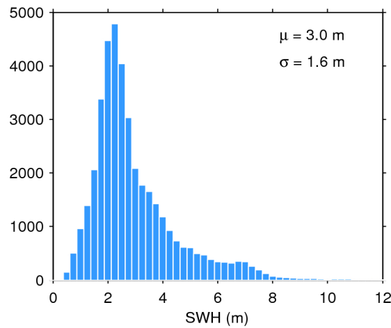
Figure 17. Histogram of flag-valid SWH over oceans and lakes for 12/10/2018. The mean ( \mu ) and standard deviation ( \sigma ) are also shown. Note that values larger than 12 m are excluded from the histogram for the sake of readability but not from the computation of \mu and \sigma .
