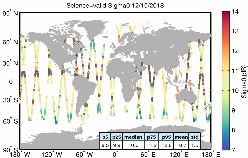
Figure 27. Geographical distribution of science-valid sigma0 data over oceans and lakes for 12/10/2018. The statistical values shown in the table refer to the sigma0 in dB and are calculated over all measurements shown in the figure. Gray circles denote records that have been rejected based on the editing criteria described in Table 4.
