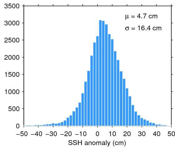
Figure 7. Histogram of flag-valid SSH anomaly over oceans and lakes for 12/10/2018. The mean ( \mu ) and standard deviation ( \sigma ) are also shown. Note that values outside [-50\ 50] cm are excluded from the histogram for the sake of readability but not from the computation of \mu and \sigma .
