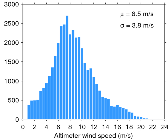
Figure 33. Histogram of flag-valid wind over oceans and lakes for 12/10/2018. The mean ( \mu ) and standard deviation ( \sigma ) are also shown. Note that values larger than 24 m/s are excluded from the histogram for the sake of readability but not from the computation of \mu and \sigma .
