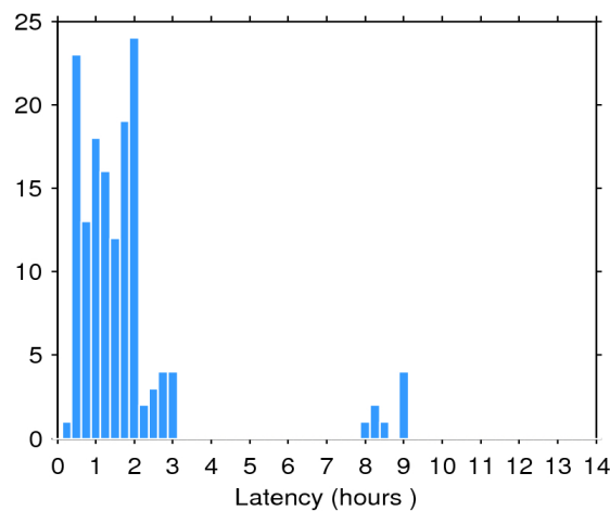
Figure 2. Histogram of the data latency for 12/10/2018. The y-axis denotes the number of files that are made available with a delay of x-hours with respect to the mean time of the records stored in the file.
