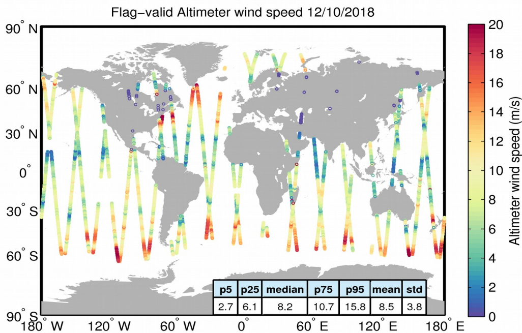
Figure 31. Geographical distribution of flag-valid wind data over oceans and lakes for 12/10/2018. The statistical values shown in the table refer to the wind in m/s and are calculated over all measurements shown in the figure.
