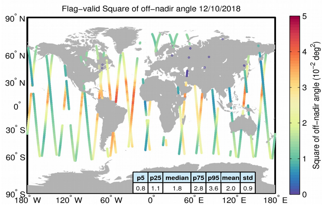
Figure 37. Geographical distribution of flag-valid mispointing data over oceans and lakes for 12/10/2018. The statistical values shown in the table refer to the mispointing in 10^{-2} \text{deg}^2 and are calculated over all measurements shown in the figure.
