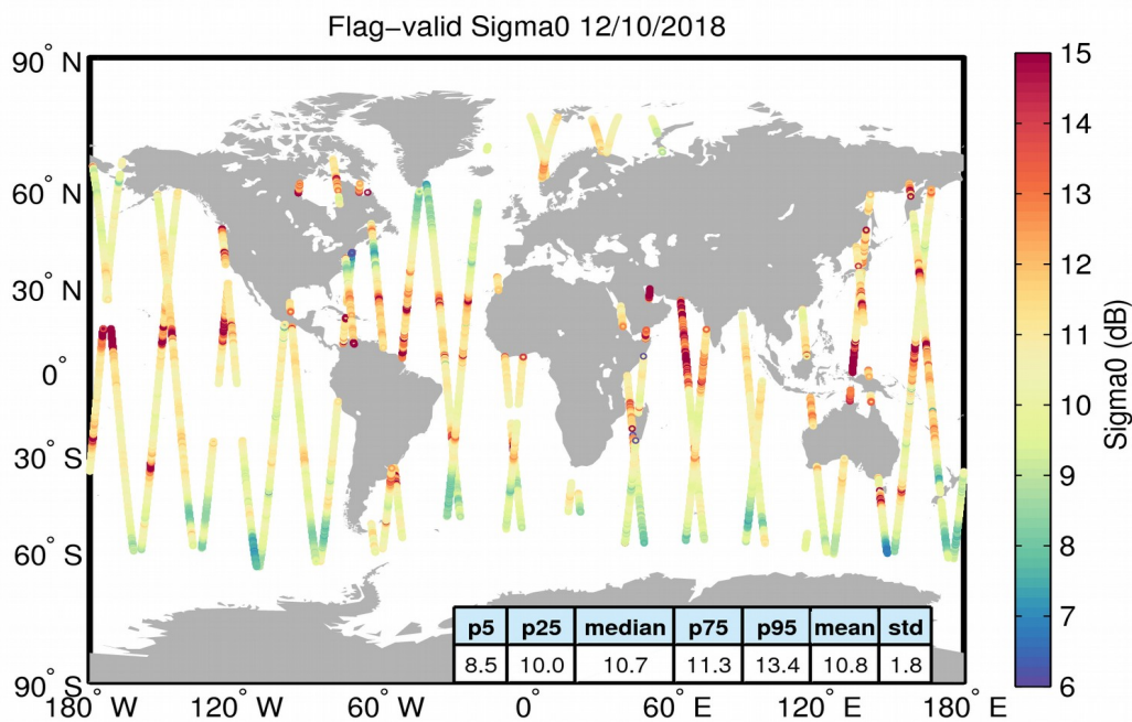
Figure 23. Geographical distribution of flag-valid sigma0 data over oceans and lakes for 12/10/2018. The statistical values shown in the table refer to the sigma0 in dB and are calculated over all measurements shown in the figure.
