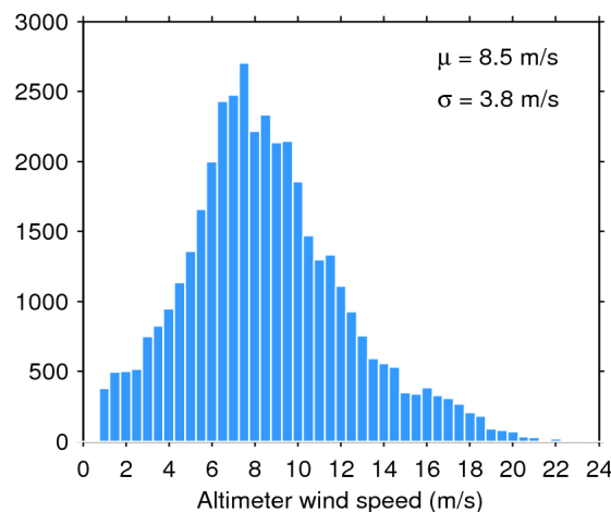
Figure 35. Histogram of science-valid wind over oceans and lakes for 12/10/2018. The mean ( \mu ) and standard deviation ( \sigma ) are also shown. Note that values larger than 24 m/s are excluded from the histogram for the sake of readability but not from the computation of \mu and \sigma .
