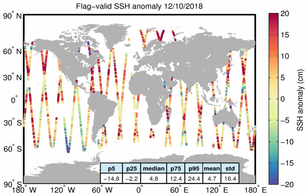
Figure 5. Geographical distribution of flag-valid 1-Hz SSH anomaly data over oceans and lakes for 12/10/2018. The statistical values shown in the table refer to the SSH anomaly in cm and are calculated over all measurements shown in the figure.
