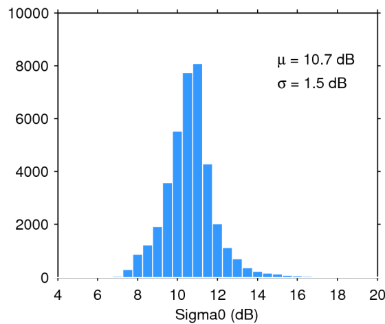
Figure 28. Histogram of science-valid sigma0 over oceans and lakes for 12/10/2018. The mean ( \mu ) and standard deviation ( \sigma ) are also shown. Note that values outside [4 20] dB are excluded from the histogram for the sake of readability but not from the computation of \mu and \sigma .
