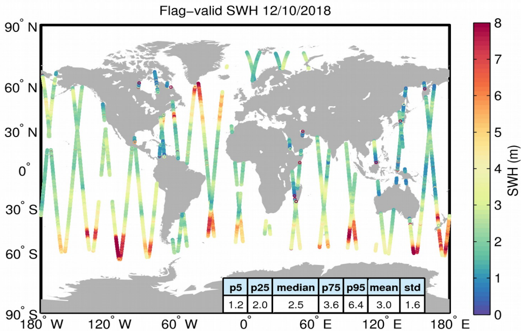
Figure 15. Geographical distribution of flag-valid SWH data over oceans and lakes for 12/10/2018. The statistical values shown in the table refer to the SWH in m and are calculated over all measurements shown in the figure.
