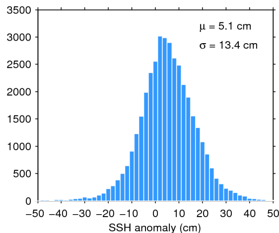
Figure 11. Histogram of science-valid SSH anomaly over oceans and lakes for 12/10/2018. The mean ( \mu ) and standard deviation ( \sigma ) are also shown. Note that values outside [-50 50] cm are excluded from the histogram for the sake of readability but not from the computation of \mu and \sigma .
