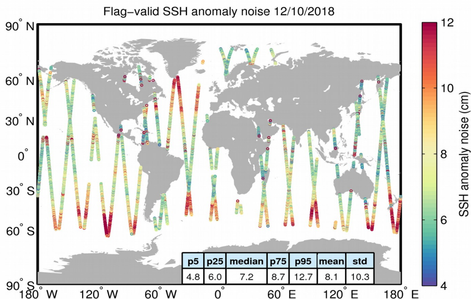
Figure 8. Geographical distribution of flag-valid 20-Hz SSH anomaly measurement noise over oceans and lakes for 12/10/2018. The statistical values shown in the table refer to the SSH anomaly noise and are calculated over all measurements shown in the figure.
