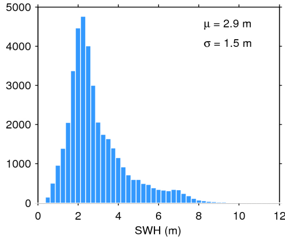
Figure 20. Histogram of science-valid SWH over oceans and lakes for 12/10/2018. The mean ( \mu ) and standard deviation ( \sigma ) are also shown. Note that values larger than 12 m are excluded from the histogram for the sake of readability but not from the computation of \mu and \sigma .
