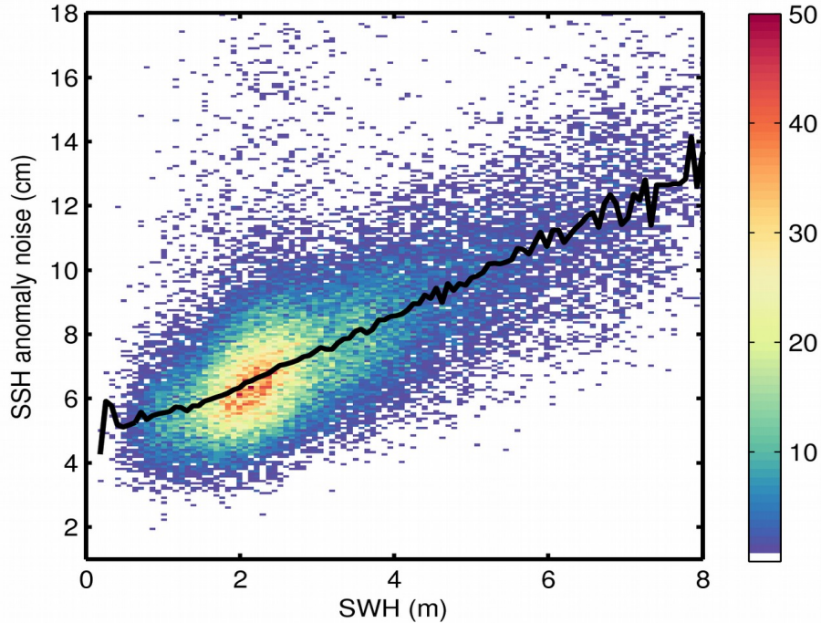
Figure 9. 2D histogram showing flag-valid SSH anomaly noise as a function of SWH for 12/10/2018. The black line denotes the median SSH anomaly noise as a function of SWH.
