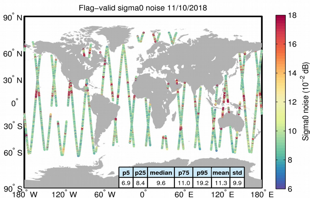
Figure 26. Geographical distribution of flag-valid 20-Hz sigma0 measurement noise over oceans and lakes for 11/10/2018. The statistical values shown in the table refer to the sigma0 noise and are calculated over all measurements shown in the figure.
