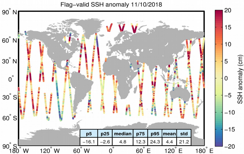
Figure 5. Geographical distribution of flag-valid 1-Hz SSH anomaly data over oceans and lakes for 11/10/2018. The statistical values shown in the table refer to the SSH anomaly in cm and are calculated over all measurements shown in the figure.
