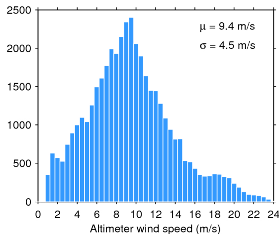
Figure 35. Histogram of science-valid wind over oceans and lakes for 11/10/2018. The mean ( \mu ) and standard deviation ( \sigma ) are also shown. Note that values larger than 24 m/s are excluded from the histogram for the sake of readability but not from the computation of \mu and \sigma .
