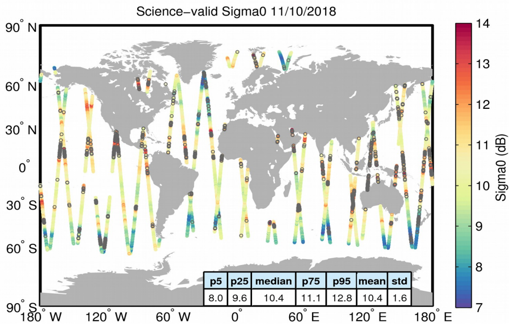
Figure 27. Geographical distribution of science-valid sigma0 data over oceans and lakes for 11/10/2018. The statistical values shown in the table refer to the sigma0 in dB and are calculated over all measurements shown in the figure. Gray circles denote records that have been rejected based on the editing criteria described in Table 4.
