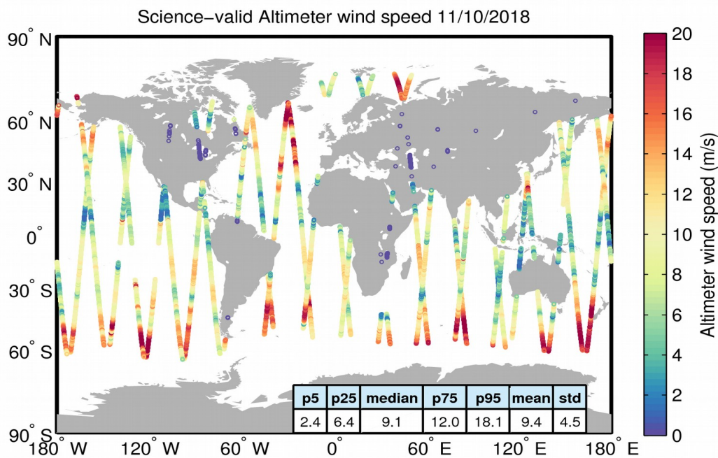
Figure 34. Geographical distribution of science-valid wind data over oceans and lakes for 11/10/2018. The statistical values shown in the table refer to the wind in m/s and are calculated over all measurements shown in the figure. Gray circles denote records that have been rejected based on the editing criteria described in Table 5.
