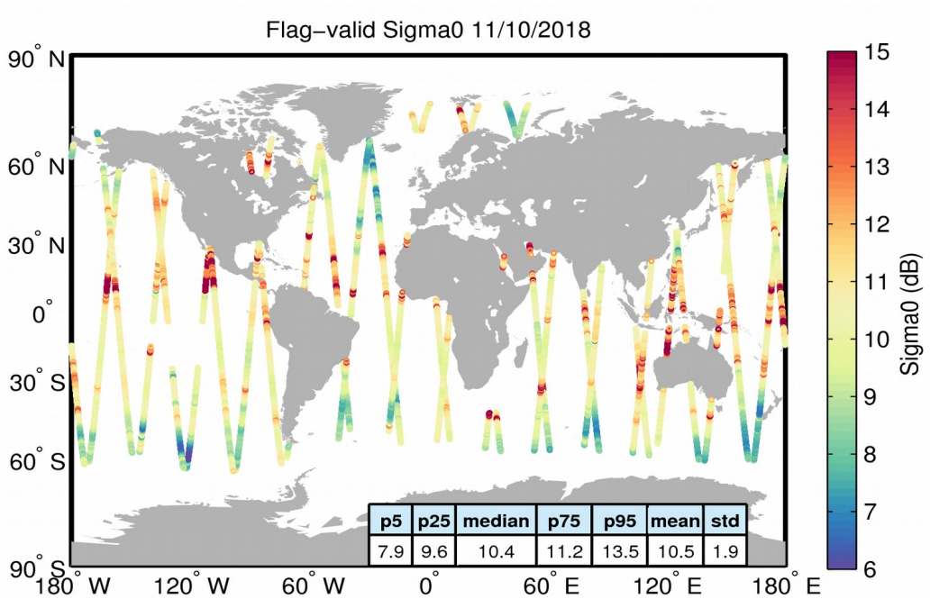
Figure 23. Geographical distribution of flag-valid sigma0 data over oceans and lakes for 11/10/2018. The statistical values shown in the table refer to the sigma0 in dB and are calculated over all measurements shown in the figure.
