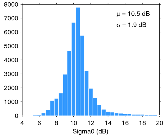
Figure 25. Histogram of flag-valid sigma0 over oceans and lakes for 11/10/2018. The mean ( \mu ) and standard deviation ( \sigma ) are also shown. Note that values outside [4 20] dB are excluded from the histogram for the sake of readability but not from the computation of \mu and \sigma .
