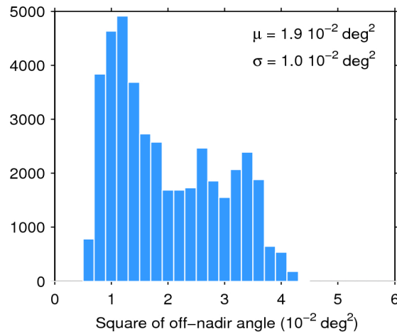
Figure 39. Histogram of flag-valid mispointing over oceans and lakes for 11/10/2018. The mean ( \mu ) and standard deviation ( \sigma ) are also shown. Note that values larger than 6 \cdot 10^{-2} \text{ deg}^2 are excluded from the histogram for the sake of readability but not from the computation of \mu and \sigma .
