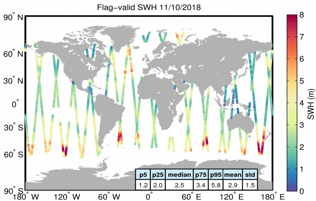
Figure 15. Geographical distribution of flag-valid SWH data over oceans and lakes for 11/10/2018. The statistical values shown in the table refer to the SWH in m and are calculated over all measurements shown in the figure.
