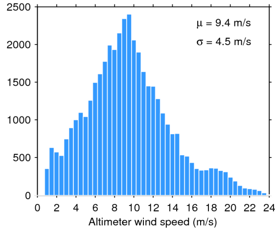
Figure 33. Histogram of flag-valid wind over oceans and lakes for 11/10/2018. The mean ( \mu ) and standard deviation ( \sigma ) are also shown. Note that values larger than 24 m/s are excluded from the histogram for the sake of readability but not from the computation of \mu and \sigma .
