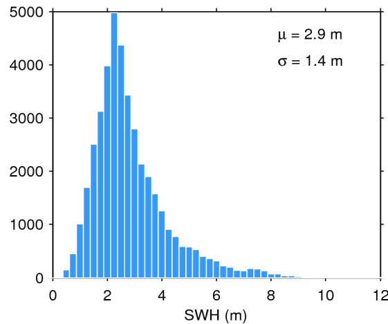
Figure 20. Histogram of science-valid SWH over oceans and lakes for 11/10/2018. The mean ( \mu ) and standard deviation ( \sigma ) are also shown. Note that values larger than 12 m are excluded from the histogram for the sake of readability but not from the computation of \mu and \sigma .
