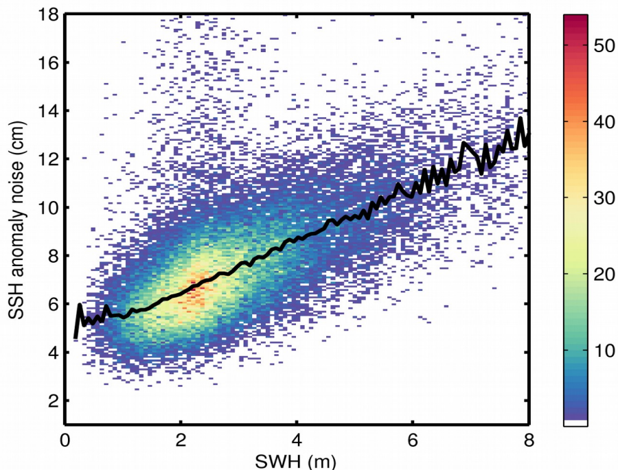
Figure 9. 2D histogram showing flag-valid SSH anomaly noise as a function of SWH for 11/10/2018. The black line denotes the median SSH anomaly noise as a function of SWH.
