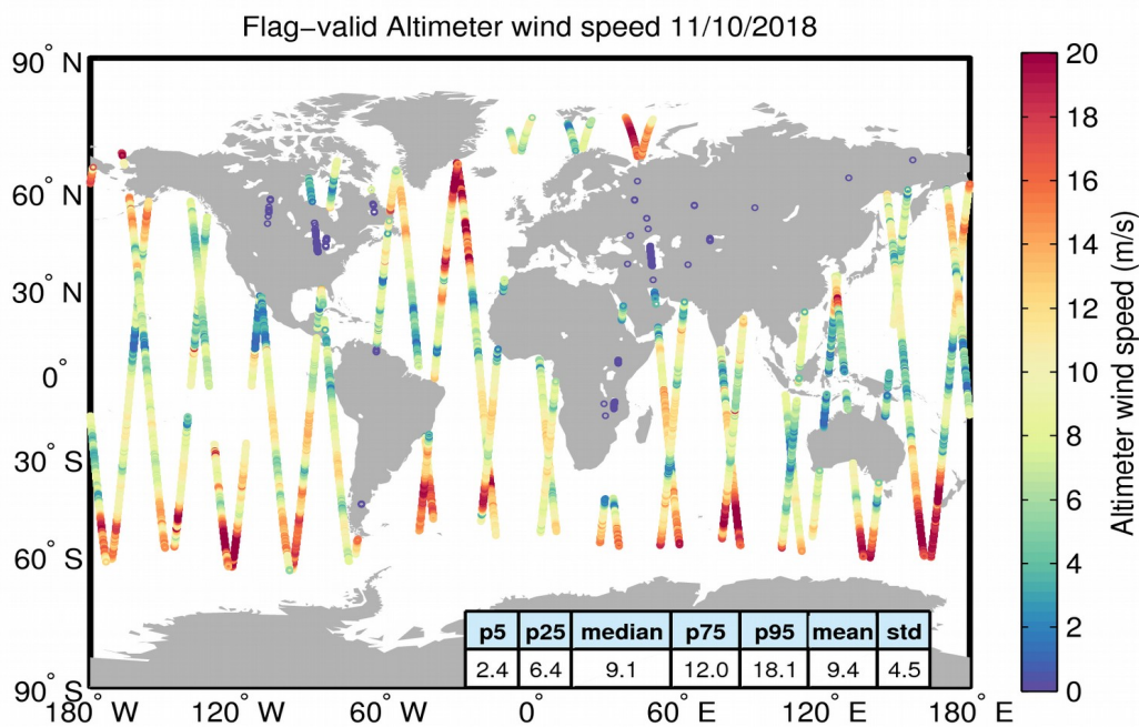
Figure 31. Geographical distribution of flag-valid wind data over oceans and lakes for 11/10/2018. The statistical values shown in the table refer to the wind in m/s and are calculated over all measurements shown in the figure.
