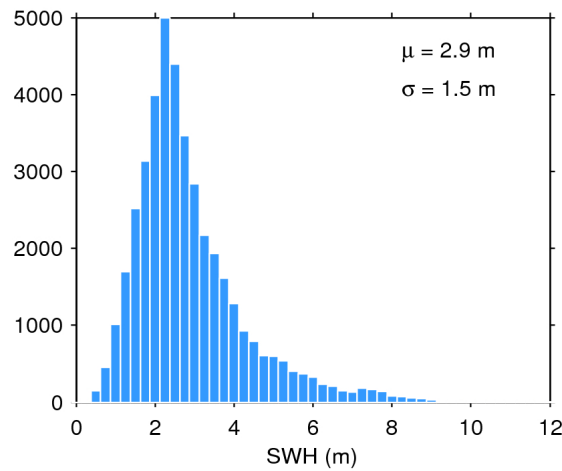
Figure 17. Histogram of flag-valid SWH over oceans and lakes for 11/10/2018. The mean ( \mu ) and standard deviation ( \sigma ) are also shown. Note that values larger than 12 m are excluded from the histogram for the sake of readability but not from the computation of \mu and \sigma .
