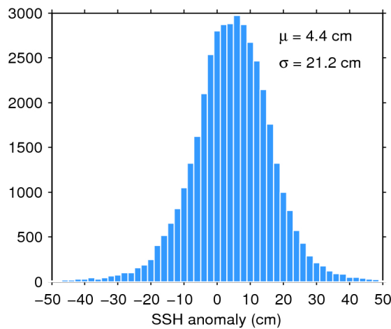
Figure 7. Histogram of flag-valid SSH anomaly over oceans and lakes for 11/10/2018. The mean ( \mu ) and standard deviation ( \sigma ) are also shown. Note that values outside [-50\ 50] cm are excluded from the histogram for the sake of readability but not from the computation of \mu and \sigma .
