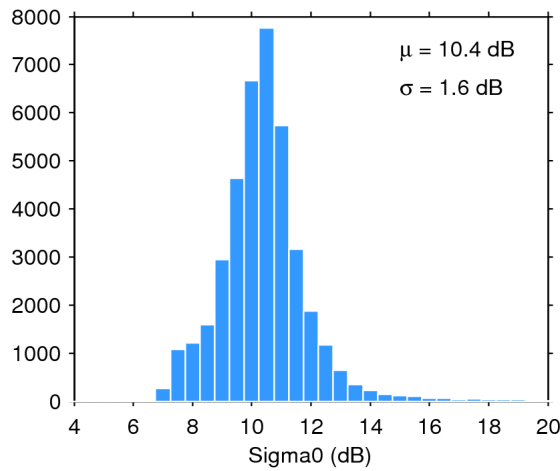
Figure 28. Histogram of science-valid sigma0 over oceans and lakes for 11/10/2018. The mean ( \mu ) and standard deviation ( \sigma ) are also shown. Note that values outside [4 20] dB are excluded from the histogram for the sake of readability but not from the computation of \mu and \sigma .
