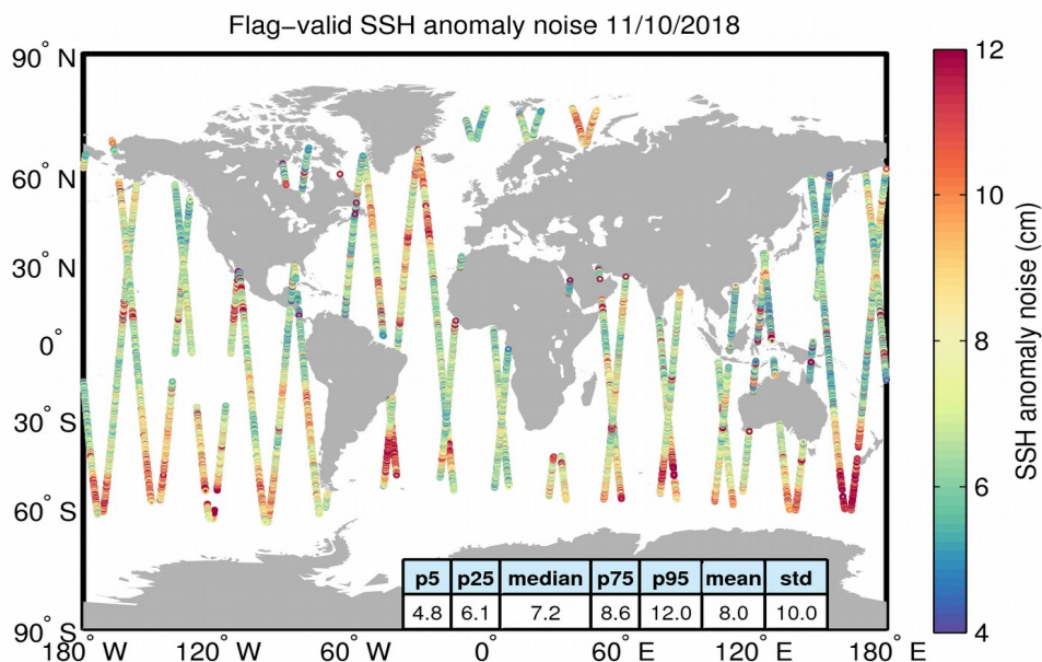
Figure 8. Geographical distribution of flag-valid 20-Hz SSH anomaly measurement noise over oceans and lakes for 11/10/2018. The statistical values shown in the table refer to the SSH anomaly noise and are calculated over all measurements shown in the figure.
