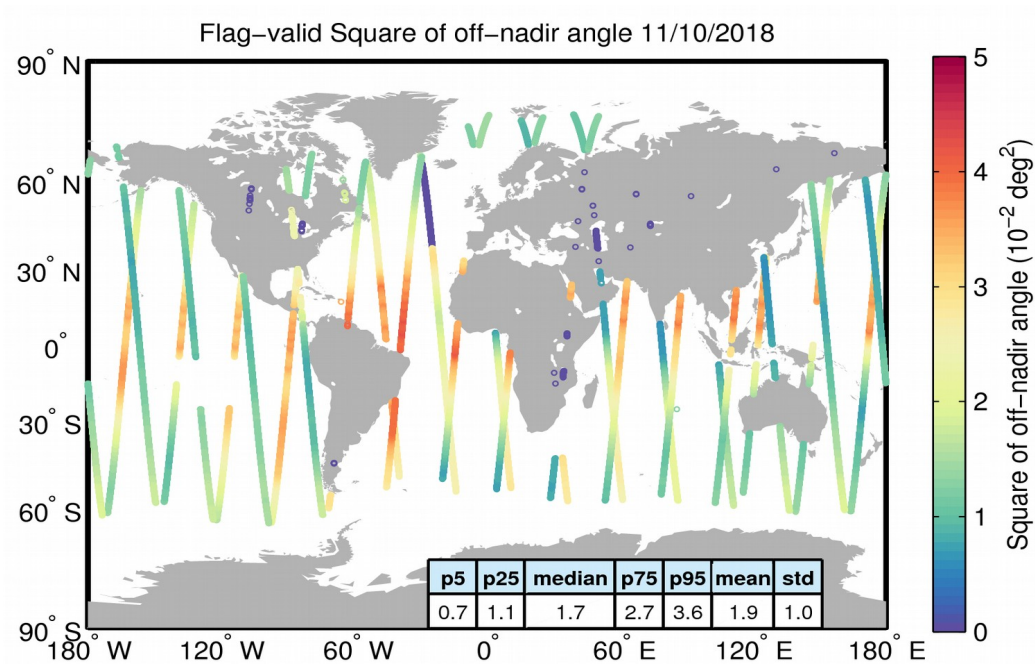
Figure 37. Geographical distribution of flag-valid mispointing data over oceans and lakes for 11/10/2018. The statistical values shown in the table refer to the mispointing in 10^{-2} \text{deg}^2 and are calculated over all measurements shown in the figure.
