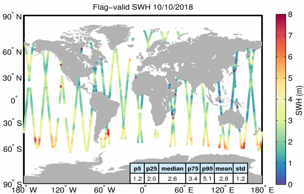
Figure 15. Geographical distribution of flag-valid SWH data over oceans and lakes for 10/10/2018. The statistical values shown in the table refer to the SWH in m and are calculated over all measurements shown in the figure.
