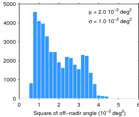
Figure 39. Histogram of flag-valid mispointing over oceans and lakes for 10/10/2018. The mean ( \mu ) and standard deviation ( \sigma ) are also shown. Note that values larger than 6 \cdot 10^{-2} \text{ deg}^2 are excluded from the histogram for the sake of readability but not from the computation of \mu and \sigma .
