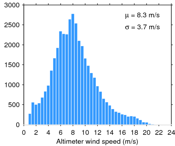
Figure 33. Histogram of flag-valid wind over oceans and lakes for 10/10/2018. The mean ( \mu ) and standard deviation ( \sigma ) are also shown. Note that values larger than 24 m/s are excluded from the histogram for the sake of readability but not from the computation of \mu and \sigma .
