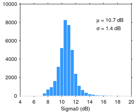
Figure 28. Histogram of science-valid sigma0 over oceans and lakes for 10/10/2018. The mean ( \mu ) and standard deviation ( \sigma ) are also shown. Note that values outside [4 20] dB are excluded from the histogram for the sake of readability but not from the computation of \mu and \sigma .
