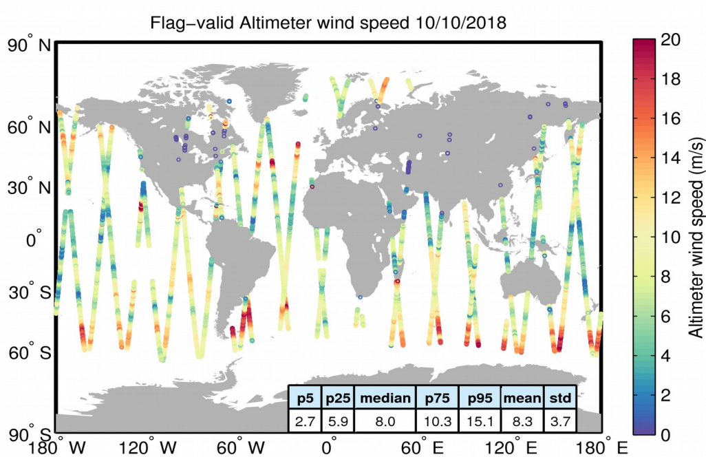
Figure 31. Geographical distribution of flag-valid wind data over oceans and lakes for 10/10/2018. The statistical values shown in the table refer to the wind in m/s and are calculated over all measurements shown in the figure.
