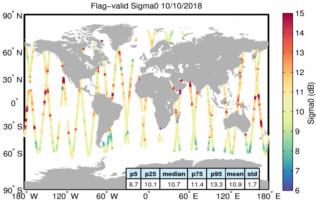
Figure 23. Geographical distribution of flag-valid sigma0 data over oceans and lakes for 10/10/2018. The statistical values shown in the table refer to the sigma0 in dB and are calculated over all measurements shown in the figure.
