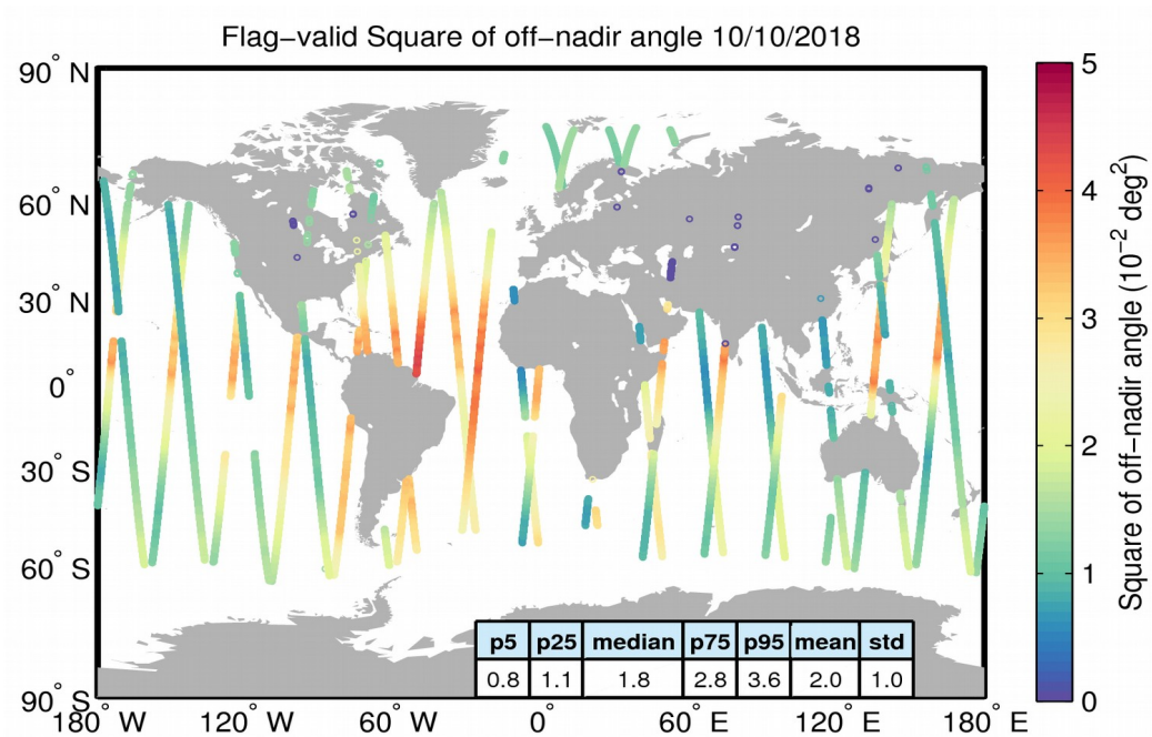
Figure 37. Geographical distribution of flag-valid mispointing data over oceans and lakes for 10/10/2018. The statistical values shown in the table refer to the mispointing in 10^{-2} deg 2 and are calculated over all measurements shown in the figure.
