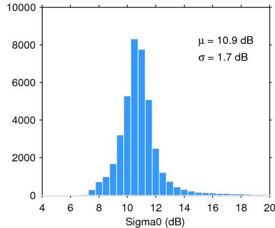
Figure 25. Histogram of flag-valid sigma0 over oceans and lakes for 10/10/2018. The mean ( \mu ) and standard deviation ( \sigma ) are also shown. Note that values outside [4 20] dB are excluded from the histogram for the sake of readability but not from the computation of \mu and \sigma .
