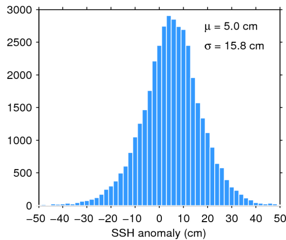
Figure 7. Histogram of flag-valid SSH anomaly over oceans and lakes for 10/10/2018. The mean ( \mu ) and standard deviation ( \sigma ) are also shown. Note that values outside [-50\ 50] cm are excluded from the histogram for the sake of readability but not from the computation of \mu and \sigma .
