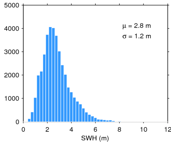
Figure 20. Histogram of science-valid SWH over oceans and lakes for 10/10/2018. The mean ( \mu ) and standard deviation ( \sigma ) are also shown. Note that values larger than 12 m are excluded from the histogram for the sake of readability but not from the computation of \mu and \sigma .
