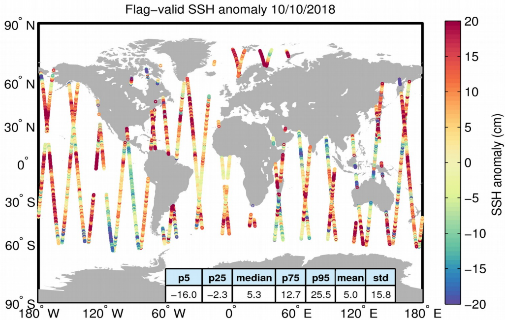
Figure 5. Geographical distribution of flag-valid 1-Hz SSH anomaly data over oceans and lakes for 10/10/2018. The statistical values shown in the table refer to the SSH anomaly in cm and are calculated over all measurements shown in the figure.
