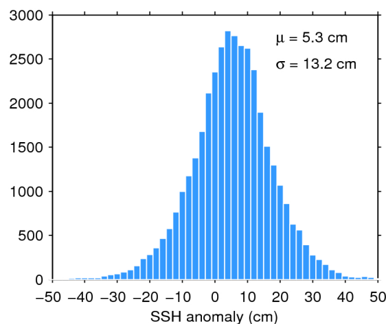
Figure 11. Histogram of science-valid SSH anomaly over oceans and lakes for 10/10/2018. The mean ( \mu ) and standard deviation ( \sigma ) are also shown. Note that values outside [-50 50] cm are excluded from the histogram for the sake of readability but not from the computation of \mu and \sigma .
