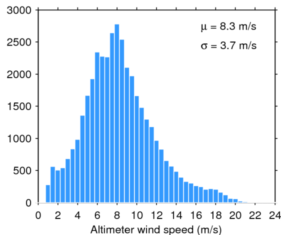
Figure 35. Histogram of science-valid wind over oceans and lakes for 10/10/2018. The mean ( \mu ) and standard deviation ( \sigma ) are also shown. Note that values larger than 24 m/s are excluded from the histogram for the sake of readability but not from the computation of \mu and \sigma .
