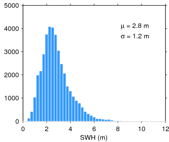
Figure 17. Histogram of flag-valid SWH over oceans and lakes for 10/10/2018. The mean ( \mu ) and standard deviation ( \sigma ) are also shown. Note that values larger than 12 m are excluded from the histogram for the sake of readability but not from the computation of \mu and \sigma .
