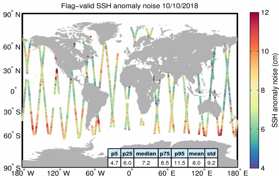
Figure 8. Geographical distribution of flag-valid 20-Hz SSH anomaly measurement noise over oceans and lakes for 10/10/2018. The statistical values shown in the table refer to the SSH anomaly noise and are calculated over all measurements shown in the figure.
