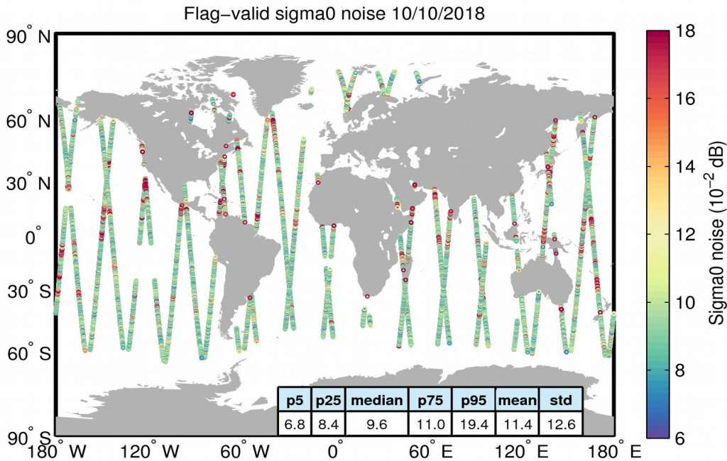
Figure 26. Geographical distribution of flag-valid 20-Hz sigma0 measurement noise over oceans and lakes for 10/10/2018. The statistical values shown in the table refer to the sigma0 noise and are calculated over all measurements shown in the figure.
