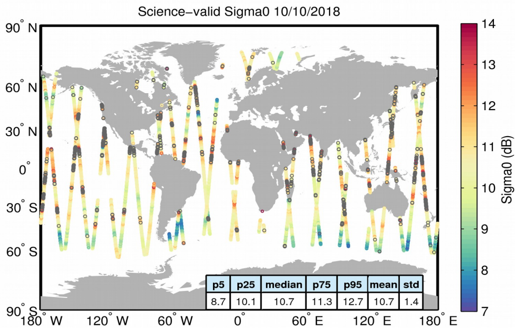
Figure 27. Geographical distribution of science-valid sigma0 data over oceans and lakes for 10/10/2018. The statistical values shown in the table refer to the sigma0 in dB and are calculated over all measurements shown in the figure. Gray circles denote records that have been rejected based on the editing criteria described in Table 4.
