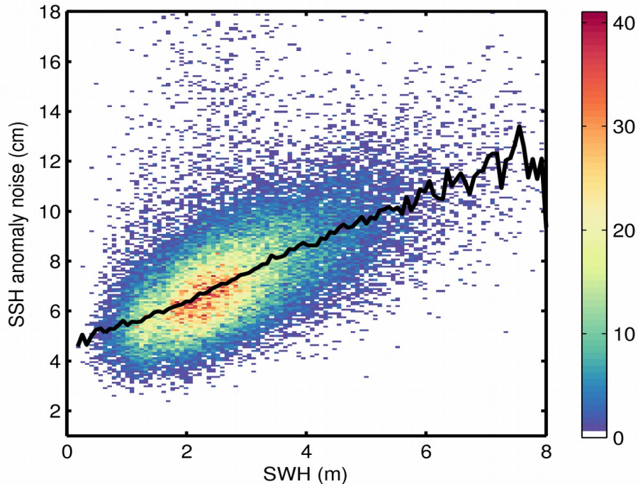
Figure 9. 2D histogram showing flag-valid SSH anomaly noise as a function of SWH for 10/10/2018. The black line denotes the median SSH anomaly noise as a function of SWH.
