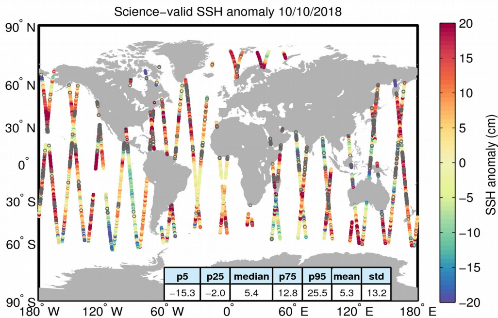
Figure 10. Geographical distribution of science-valid SSH anomaly data over oceans and lakes for 10/10/2018. The statistical values shown in the table refer to the SSH anomaly in cm and are calculated over all measurements shown in the figure. Gray circles denote records that have been rejected based on the editing criteria described in Table 2.
