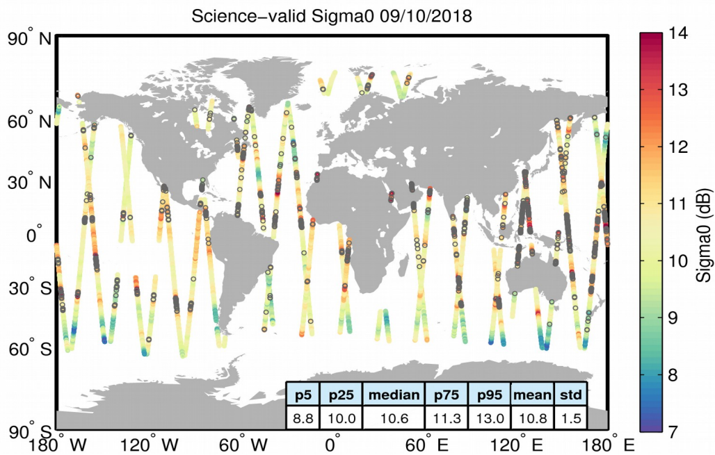
Figure 27. Geographical distribution of science-valid sigma0 data over oceans and lakes for 09/10/2018. The statistical values shown in the table refer to the sigma0 in dB and are calculated over all measurements shown in the figure. Gray circles denote records that have been rejected based on the editing criteria described in Table 4.
