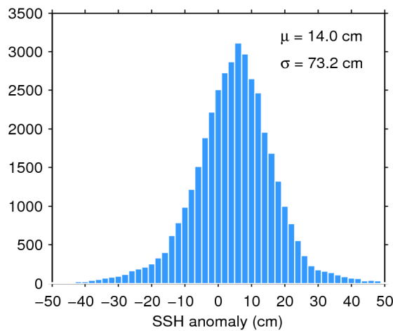
Figure 7. Histogram of flag-valid SSH anomaly over oceans and lakes for 09/10/2018. The mean ( \mu ) and standard deviation ( \sigma ) are also shown. Note that values outside [-50\ 50] cm are excluded from the histogram for the sake of readability but not from the computation of \mu and \sigma .
