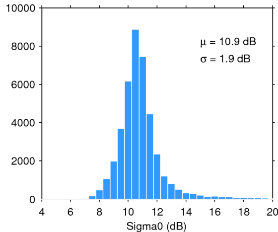
Figure 25. Histogram of flag-valid sigma0 over oceans and lakes for 09/10/2018. The mean ( \mu ) and standard deviation ( \sigma ) are also shown. Note that values outside [4 20] dB are excluded from the histogram for the sake of readability but not from the computation of \mu and \sigma .
