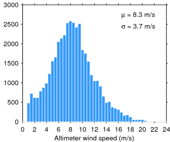
Figure 33. Histogram of flag-valid wind over oceans and lakes for 09/10/2018. The mean ( \mu ) and standard deviation ( \sigma ) are also shown. Note that values larger than 24 m/s are excluded from the histogram for the sake of readability but not from the computation of \mu and \sigma .
