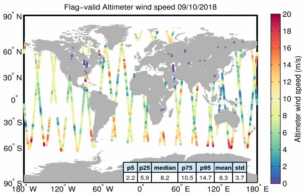
Figure 31. Geographical distribution of flag-valid wind data over oceans and lakes for 09/10/2018. The statistical values shown in the table refer to the wind in m/s and are calculated over all measurements shown in the figure.
