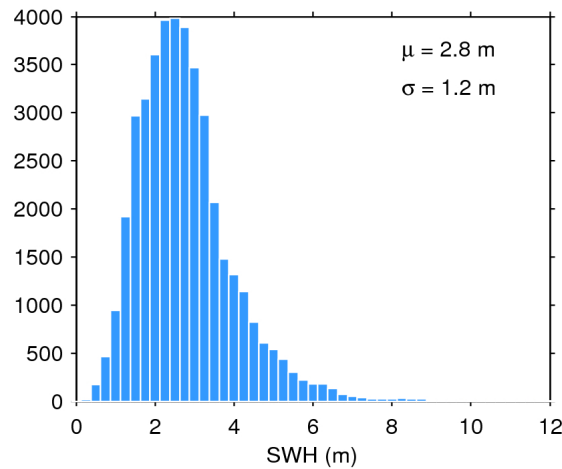
Figure 17. Histogram of flag-valid SWH over oceans and lakes for 09/10/2018. The mean ( \mu ) and standard deviation ( \sigma ) are also shown. Note that values larger than 12 m are excluded from the histogram for the sake of readability but not from the computation of \mu and \sigma .
