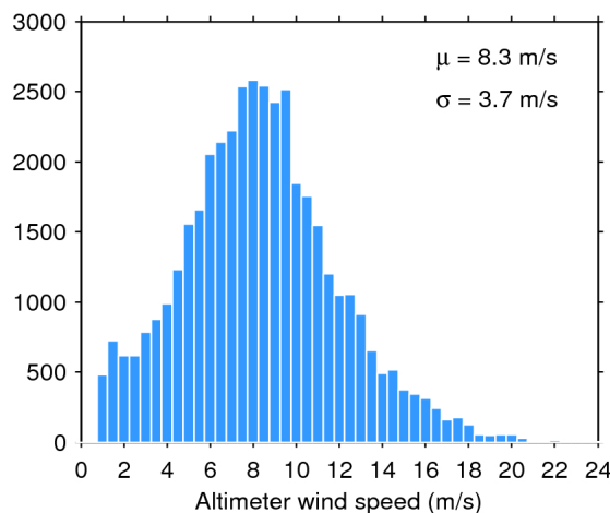
Figure 35. Histogram of science-valid wind over oceans and lakes for 09/10/2018. The mean ( \mu ) and standard deviation ( \sigma ) are also shown. Note that values larger than 24 m/s are excluded from the histogram for the sake of readability but not from the computation of \mu and \sigma .
