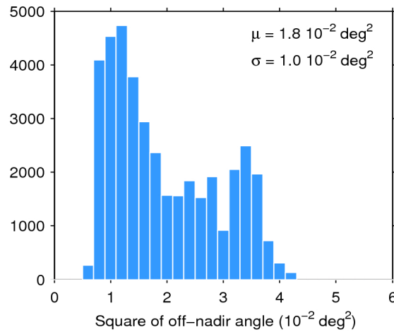
Figure 39. Histogram of flag-valid mispointing over oceans and lakes for 09/10/2018. The mean ( \mu ) and standard deviation ( \sigma ) are also shown. Note that values larger than 6 \cdot 10^{-2} \text{ deg}^2 are excluded from the histogram for the sake of readability but not from the computation of \mu and \sigma .
