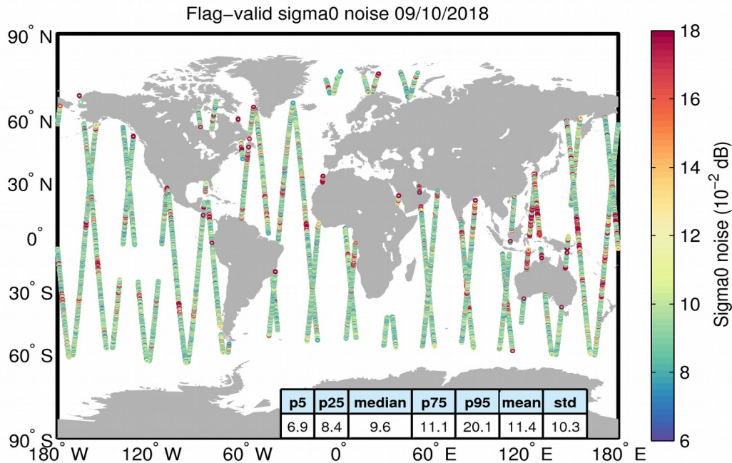
Figure 26. Geographical distribution of flag-valid 20-Hz sigma0 measurement noise over oceans and lakes for 09/10/2018. The statistical values shown in the table refer to the sigma0 noise and are calculated over all measurements shown in the figure.
