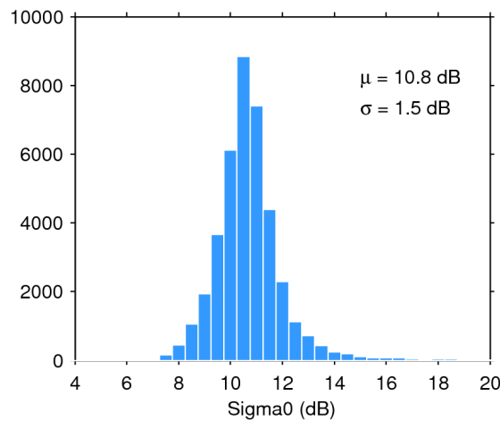
Figure 28. Histogram of science-valid sigma0 over oceans and lakes for 09/10/2018. The mean ( \mu ) and standard deviation ( \sigma ) are also shown. Note that values outside [4 20] dB are excluded from the histogram for the sake of readability but not from the computation of \mu and \sigma .
