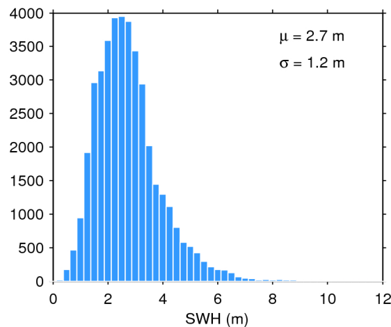
Figure 20. Histogram of science-valid SWH over oceans and lakes for 09/10/2018. The mean ( \mu ) and standard deviation ( \sigma ) are also shown. Note that values larger than 12 m are excluded from the histogram for the sake of readability but not from the computation of \mu and \sigma .
