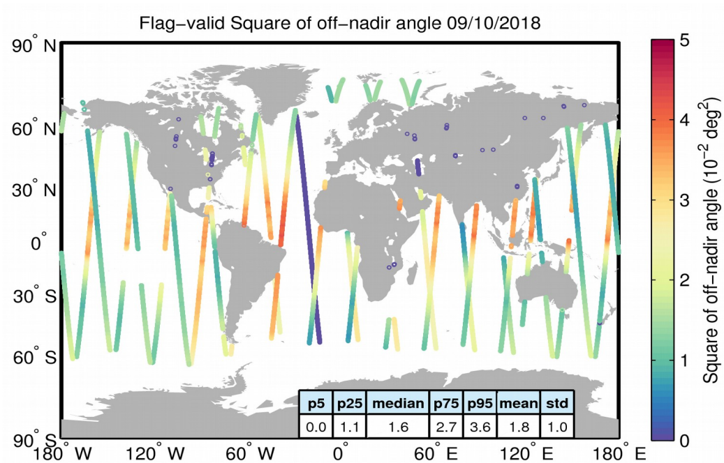
Figure 37. Geographical distribution of flag-valid mispointing data over oceans and lakes for 09/10/2018. The statistical values shown in the table refer to the mispointing in 10^{-2} deg 2 and are calculated over all measurements shown in the figure.
