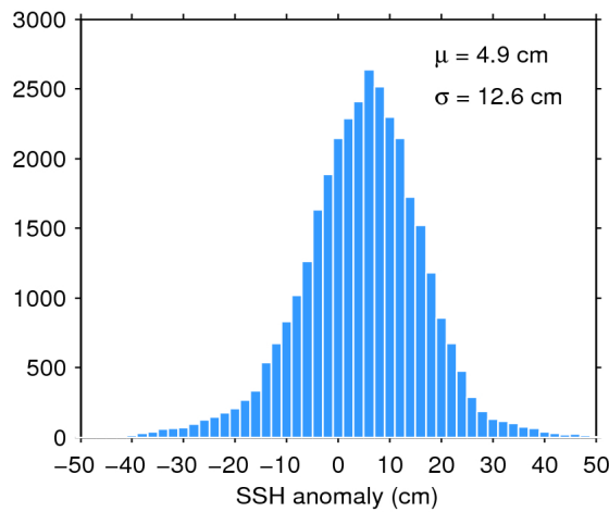
Figure 11. Histogram of science-valid SSH anomaly over oceans and lakes for 09/10/2018. The mean ( \mu ) and standard deviation ( \sigma ) are also shown. Note that values outside [-50 50] cm are excluded from the histogram for the sake of readability but not from the computation of \mu and \sigma .
