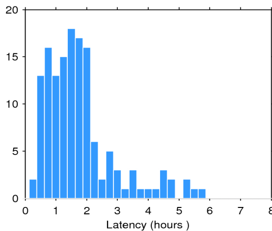
Figure 2. Histogram of the data latency for 09/10/2018. The y-axis denotes the number of files that are made available with a delay of x-hours with respect to the mean time of the records stored in the file.
