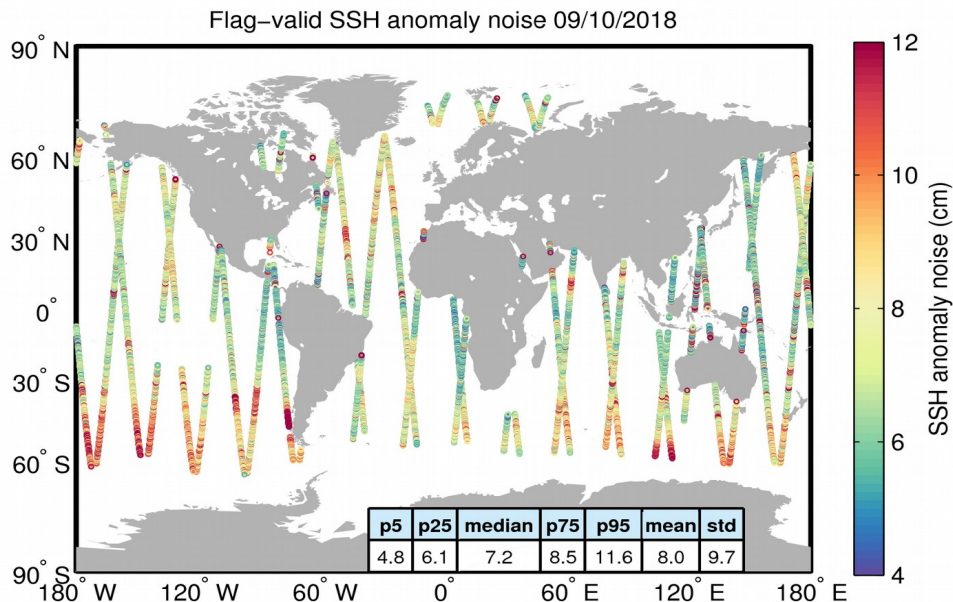
Figure 8. Geographical distribution of flag-valid 20-Hz SSH anomaly measurement noise over oceans and lakes for 09/10/2018. The statistical values shown in the table refer to the SSH anomaly noise and are calculated over all measurements shown in the figure.
