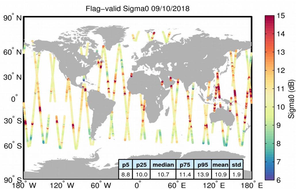
Figure 23. Geographical distribution of flag-valid sigma0 data over oceans and lakes for 09/10/2018. The statistical values shown in the table refer to the sigma0 in dB and are calculated over all measurements shown in the figure.
