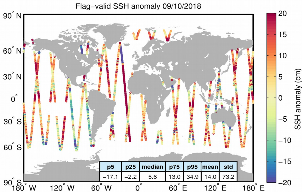
Figure 5. Geographical distribution of flag-valid 1-Hz SSH anomaly data over oceans and lakes for 09/10/2018. The statistical values shown in the table refer to the SSH anomaly in cm and are calculated over all measurements shown in the figure.
