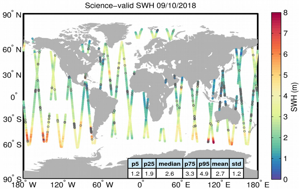
Figure 19. Geographical distribution of science-valid SWH data over oceans and lakes for 09/10/2018. The statistical values shown in the table refer to the SWH in m and are calculated over all measurements shown in the figure. Gray circles denote records that have been rejected based on the editing criteria described in Table 3.
