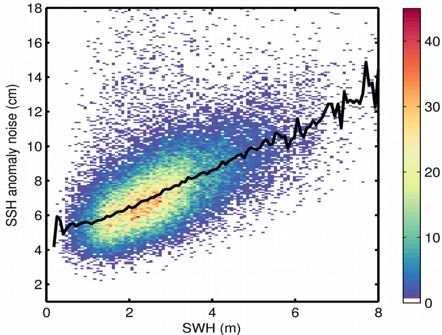
Figure 9. 2D histogram showing flag-valid SSH anomaly noise as a function of SWH for 09/10/2018. The black line denotes the median SSH anomaly noise as a function of SWH.
