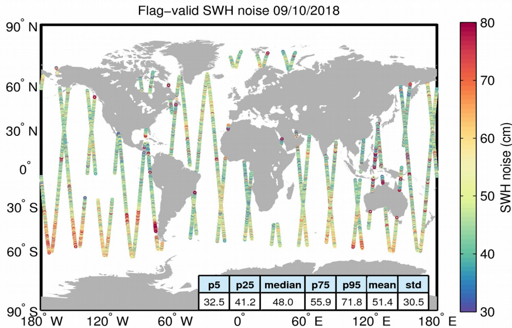
Figure 18. Geographical distribution of flag-valid 20-Hz SWH measurement noise over oceans and lakes for 09/10/2018. The statistical values shown in the table refer to the SWH noise and are calculated over all measurements shown in the figure.
