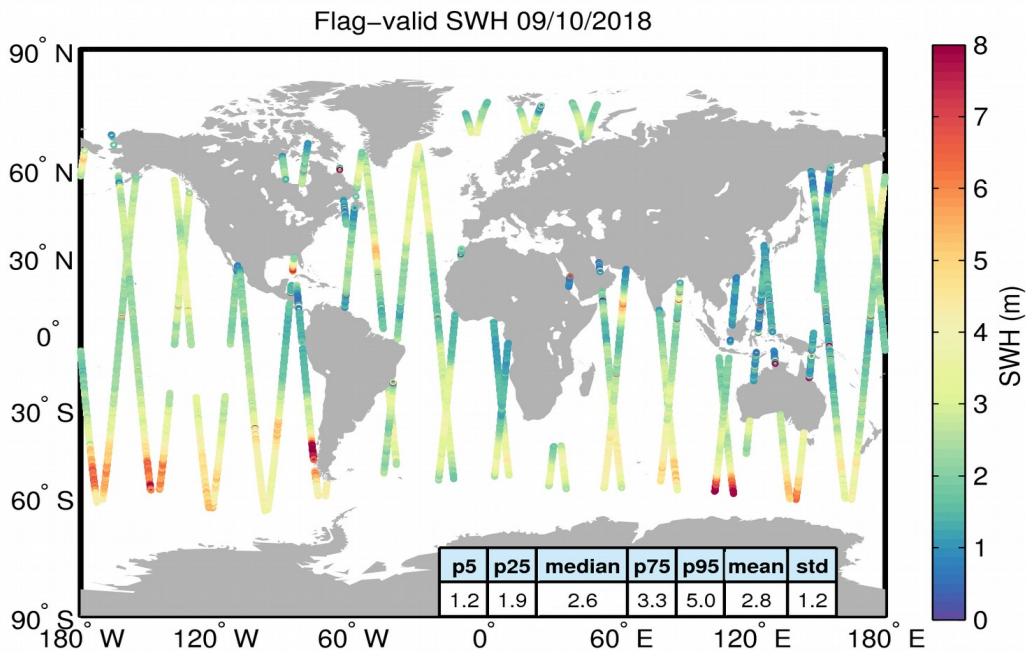
Figure 15. Geographical distribution of flag-valid SWH data over oceans and lakes for 09/10/2018. The statistical values shown in the table refer to the SWH in m and are calculated over all measurements shown in the figure.
