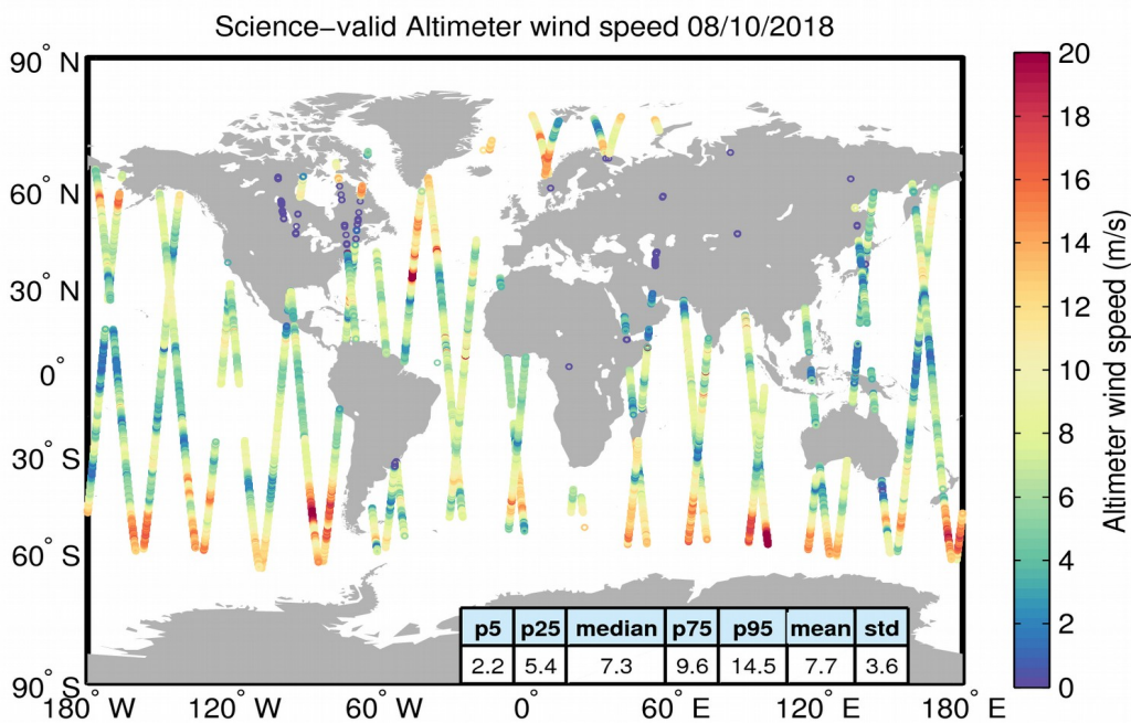
Figure 34. Geographical distribution of science-valid wind data over oceans and lakes for 08/10/2018. The statistical values shown in the table refer to the wind in m/s and are calculated over all measurements shown in the figure. Gray circles denote records that have been rejected based on the editing criteria described in Table 5.
