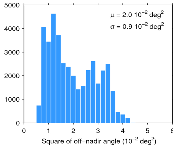
Figure 39. Histogram of flag-valid mispointing over oceans and lakes for 08/10/2018. The mean ( \mu ) and standard deviation ( \sigma ) are also shown. Note that values larger than 6 \cdot 10^{-2} \text{ deg}^2 are excluded from the histogram for the sake of readability but not from the computation of \mu and \sigma .
