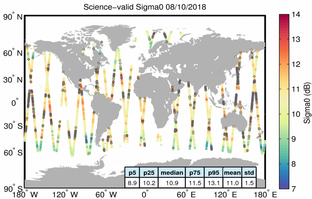
Figure 27. Geographical distribution of science-valid sigma0 data over oceans and lakes for 08/10/2018. The statistical values shown in the table refer to the sigma0 in dB and are calculated over all measurements shown in the figure. Gray circles denote records that have been rejected based on the editing criteria described in Table 4.
