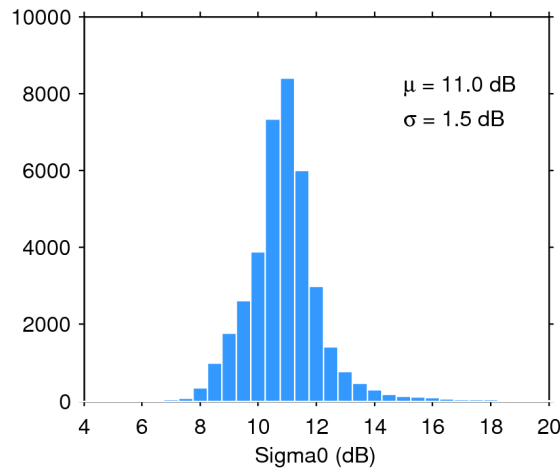
Figure 28. Histogram of science-valid sigma0 over oceans and lakes for 08/10/2018. The mean ( \mu ) and standard deviation ( \sigma ) are also shown. Note that values outside [4 20] dB are excluded from the histogram for the sake of readability but not from the computation of \mu and \sigma .
