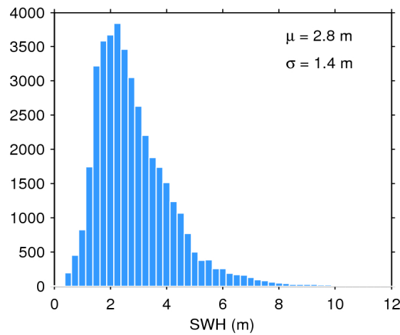
Figure 17. Histogram of flag-valid SWH over oceans and lakes for 08/10/2018. The mean ( \mu ) and standard deviation ( \sigma ) are also shown. Note that values larger than 12 m are excluded from the histogram for the sake of readability but not from the computation of \mu and \sigma .
