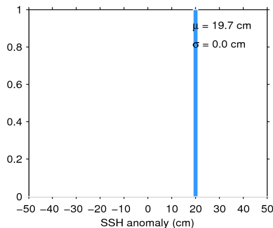
Figure 11. Histogram of science-valid SSH anomaly over oceans and lakes for 08/10/2018. The mean ( \mu ) and standard deviation ( \sigma ) are also shown. Note that values outside [-50 50] cm are excluded from the histogram for the sake of readability but not from the computation of \mu and \sigma .
