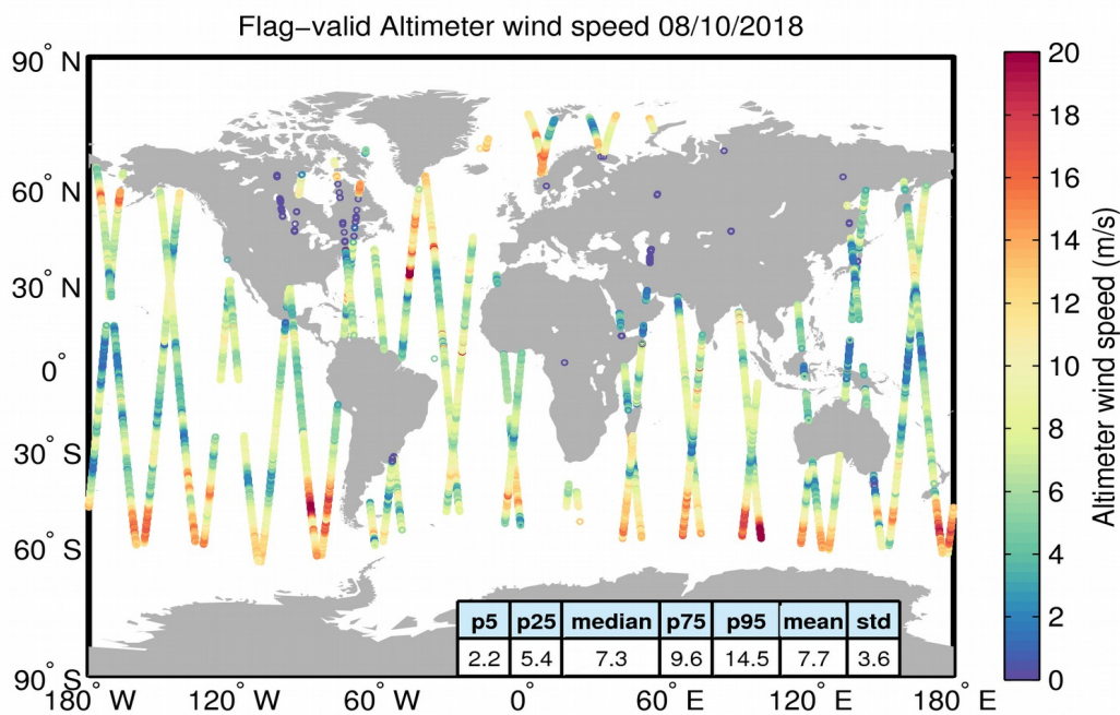
Figure 31. Geographical distribution of flag-valid wind data over oceans and lakes for 08/10/2018. The statistical values shown in the table refer to the wind in m/s and are calculated over all measurements shown in the figure.
