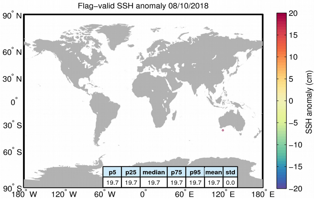
Figure 5. Geographical distribution of flag-valid 1-Hz SSH anomaly data over oceans and lakes for 08/10/2018. The statistical values shown in the table refer to the SSH anomaly in cm and are calculated over all measurements shown in the figure.
