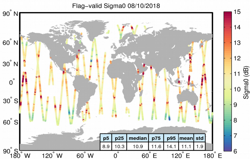
Figure 23. Geographical distribution of flag-valid sigma0 data over oceans and lakes for 08/10/2018. The statistical values shown in the table refer to the sigma0 in dB and are calculated over all measurements shown in the figure.
