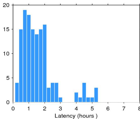
Figure 2. Histogram of the data latency for 08/10/2018. The y-axis denotes the number of files that are made available with a delay of x-hours with respect to the mean time of the records stored in the file.
