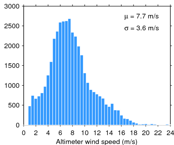
Figure 35. Histogram of science-valid wind over oceans and lakes for 08/10/2018. The mean ( \mu ) and standard deviation ( \sigma ) are also shown. Note that values larger than 24 m/s are excluded from the histogram for the sake of readability but not from the computation of \mu and \sigma .
