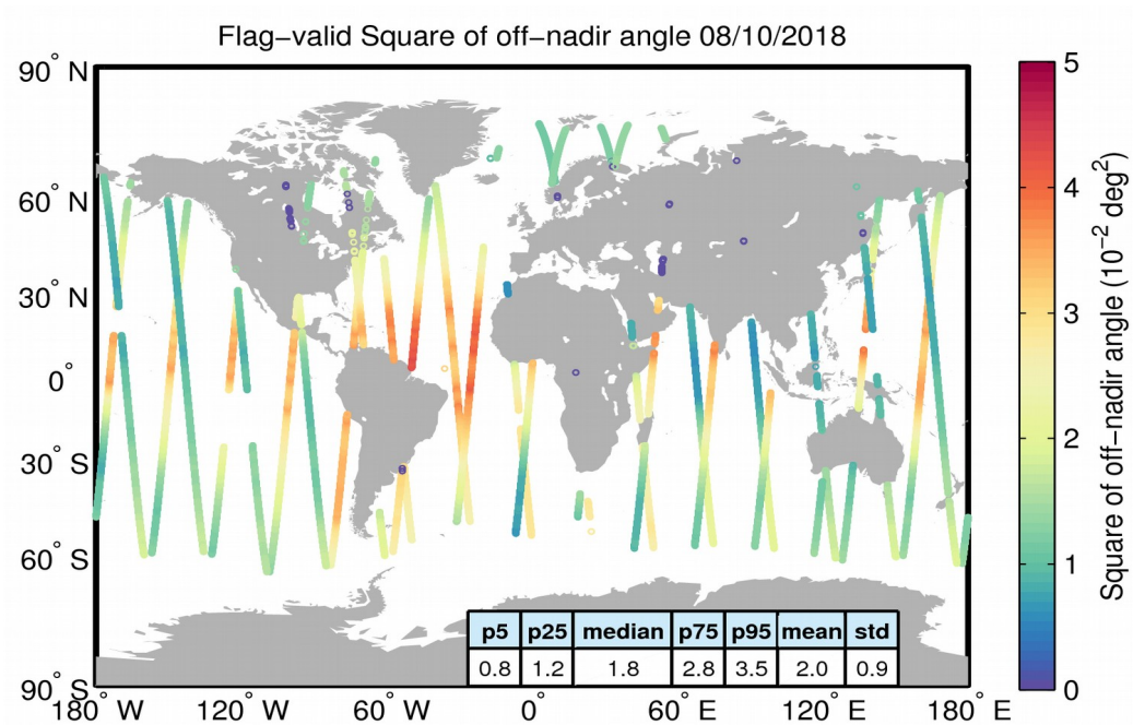
Figure 37. Geographical distribution of flag-valid mispointing data over oceans and lakes for 08/10/2018. The statistical values shown in the table refer to the mispointing in 10^{-2} \text{ deg}^2 and are calculated over all measurements shown in the figure.
