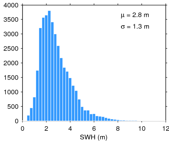
Figure 20. Histogram of science-valid SWH over oceans and lakes for 08/10/2018. The mean ( \mu ) and standard deviation ( \sigma ) are also shown. Note that values larger than 12 m are excluded from the histogram for the sake of readability but not from the computation of \mu and \sigma .
