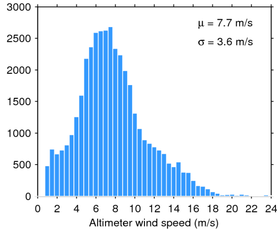
Figure 33. Histogram of flag-valid wind over oceans and lakes for 08/10/2018. The mean ( \mu ) and standard deviation ( \sigma ) are also shown. Note that values larger than 24 m/s are excluded from the histogram for the sake of readability but not from the computation of \mu and \sigma .
