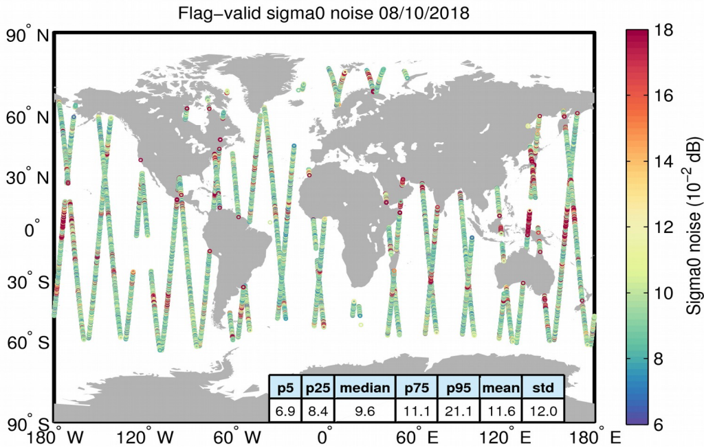
Figure 26. Geographical distribution of flag-valid 20-Hz sigma0 measurement noise over oceans and lakes for 08/10/2018. The statistical values shown in the table refer to the sigma0 noise and are calculated over all measurements shown in the figure.
