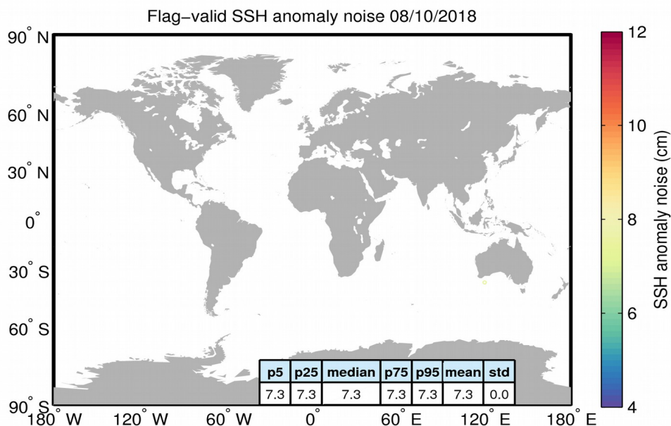
Figure 8. Geographical distribution of flag-valid 20-Hz SSH anomaly measurement noise over oceans and lakes for 08/10/2018. The statistical values shown in the table refer to the SSH anomaly noise and are calculated over all measurements shown in the figure.
