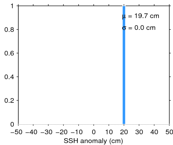
Figure 7. Histogram of flag-valid SSH anomaly over oceans and lakes for 08/10/2018. The mean ( \mu ) and standard deviation ( \sigma ) are also shown. Note that values outside [-50\ 50] cm are excluded from the histogram for the sake of readability but not from the computation of \mu and \sigma .
