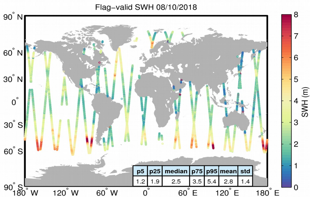
Figure 15. Geographical distribution of flag-valid SWH data over oceans and lakes for 08/10/2018. The statistical values shown in the table refer to the SWH in m and are calculated over all measurements shown in the figure.
