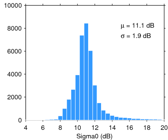
Figure 25. Histogram of flag-valid sigma0 over oceans and lakes for 08/10/2018. The mean ( \mu ) and standard deviation ( \sigma ) are also shown. Note that values outside [4 20] dB are excluded from the histogram for the sake of readability but not from the computation of \mu and \sigma .
