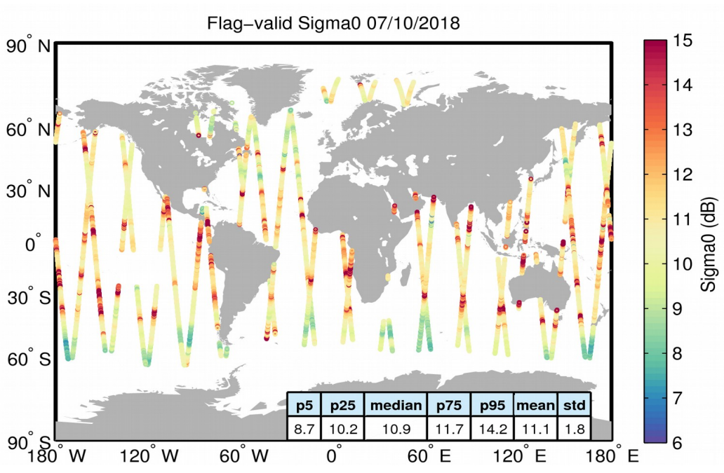
Figure 23. Geographical distribution of flag-valid sigma0 data over oceans and lakes for 07/10/2018. The statistical values shown in the table refer to the sigma0 in dB and are calculated over all measurements shown in the figure.
