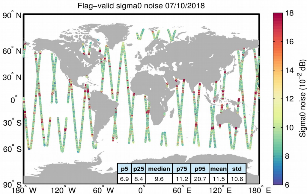
Figure 26. Geographical distribution of flag-valid 20-Hz sigma0 measurement noise over oceans and lakes for 07/10/2018. The statistical values shown in the table refer to the sigma0 noise and are calculated over all measurements shown in the figure.
