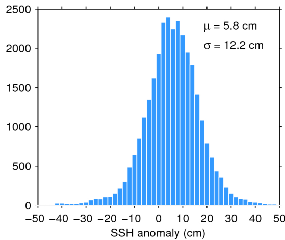
Figure 11. Histogram of science-valid SSH anomaly over oceans and lakes for 07/10/2018. The mean ( \mu ) and standard deviation ( \sigma ) are also shown. Note that values outside [-50 50] cm are excluded from the histogram for the sake of readability but not from the computation of \mu and \sigma .
