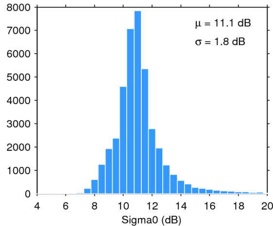
Figure 25. Histogram of flag-valid sigma0 over oceans and lakes for 07/10/2018. The mean ( \mu ) and standard deviation ( \sigma ) are also shown. Note that values outside [4 20] dB are excluded from the histogram for the sake of readability but not from the computation of \mu and \sigma .
