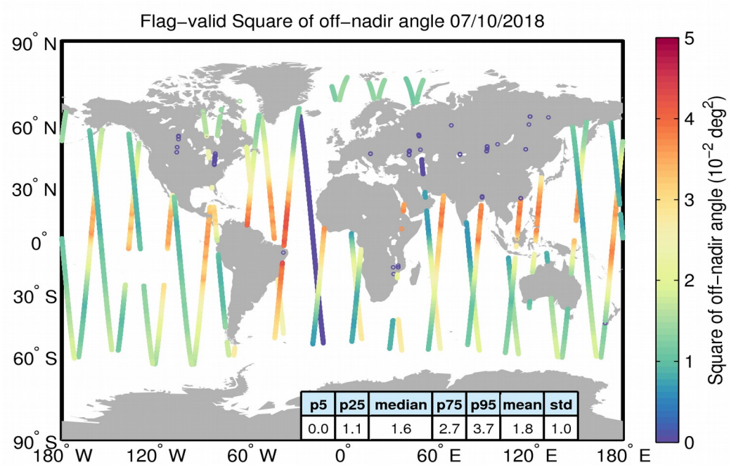
Figure 37. Geographical distribution of flag-valid mispointing data over oceans and lakes for 07/10/2018. The statistical values shown in the table refer to the mispointing in 10^{-2} \text{ deg}^2 and are calculated over all measurements shown in the figure.
