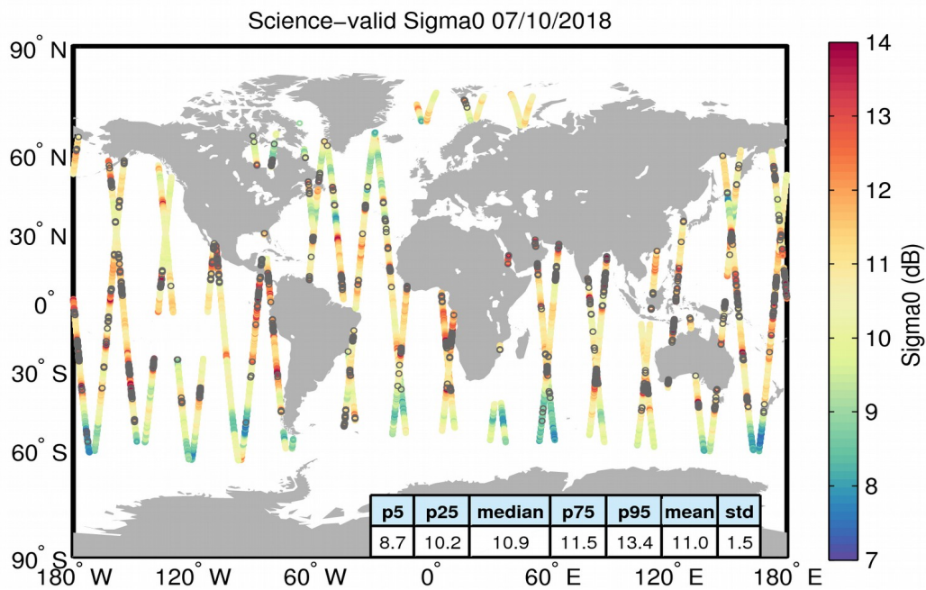
Figure 27. Geographical distribution of science-valid sigma0 data over oceans and lakes for 07/10/2018. The statistical values shown in the table refer to the sigma0 in dB and are calculated over all measurements shown in the figure. Gray circles denote records that have been rejected based on the editing criteria described in Table 4.
