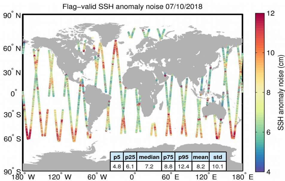
Figure 8. Geographical distribution of flag-valid 20-Hz SSH anomaly measurement noise over oceans and lakes for 07/10/2018. The statistical values shown in the table refer to the SSH anomaly noise and are calculated over all measurements shown in the figure.
