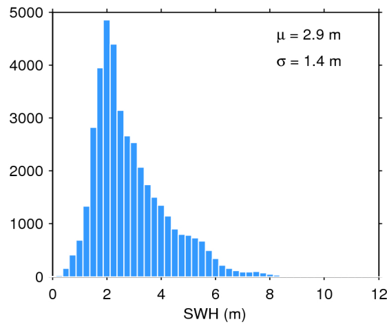
Figure 17. Histogram of flag-valid SWH over oceans and lakes for 07/10/2018. The mean ( \mu ) and standard deviation ( \sigma ) are also shown. Note that values larger than 12 m are excluded from the histogram for the sake of readability but not from the computation of \mu and \sigma .
