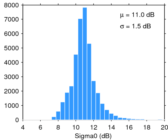
Figure 28. Histogram of science-valid sigma0 over oceans and lakes for 07/10/2018. The mean ( \mu ) and standard deviation ( \sigma ) are also shown. Note that values outside [4 20] dB are excluded from the histogram for the sake of readability but not from the computation of \mu and \sigma .
