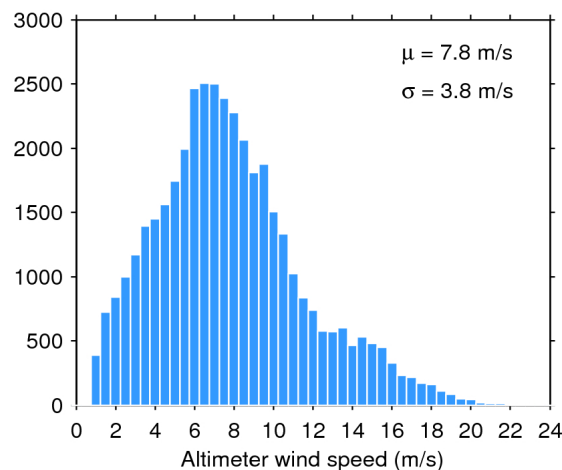
Figure 35. Histogram of science-valid wind over oceans and lakes for 07/10/2018. The mean ( \mu ) and standard deviation ( \sigma ) are also shown. Note that values larger than 24 m/s are excluded from the histogram for the sake of readability but not from the computation of \mu and \sigma .
