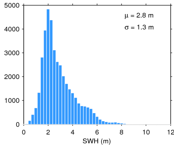
Figure 20. Histogram of science-valid SWH over oceans and lakes for 07/10/2018. The mean ( \mu ) and standard deviation ( \sigma ) are also shown. Note that values larger than 12 m are excluded from the histogram for the sake of readability but not from the computation of \mu and \sigma .
