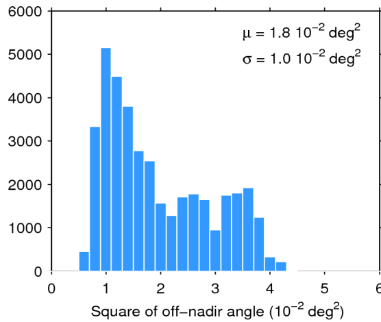
Figure 39. Histogram of flag-valid mispointing over oceans and lakes for 07/10/2018. The mean ( \mu ) and standard deviation ( \sigma ) are also shown. Note that values larger than 6 \cdot 10^{-2} \text{ deg}^2 are excluded from the histogram for the sake of readability but not from the computation of \mu and \sigma .
