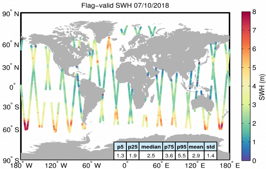
Figure 15. Geographical distribution of flag-valid SWH data over oceans and lakes for 07/10/2018. The statistical values shown in the table refer to the SWH in m and are calculated over all measurements shown in the figure.
