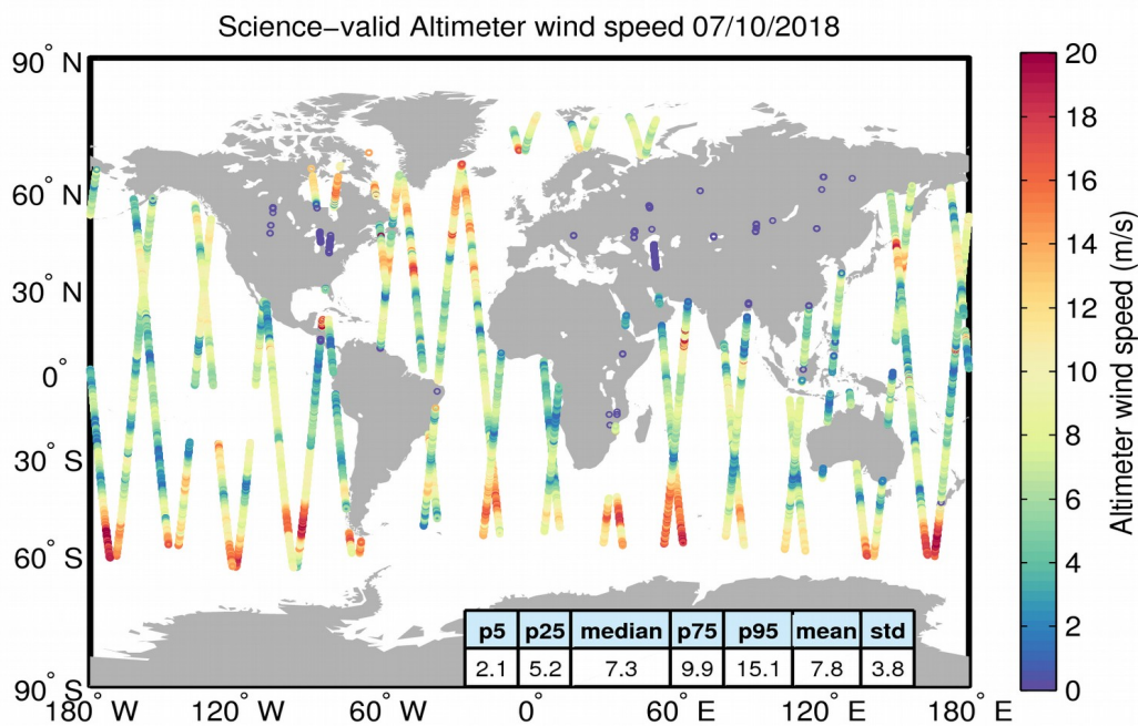
Figure 34. Geographical distribution of science-valid wind data over oceans and lakes for 07/10/2018. The statistical values shown in the table refer to the wind in m/s and are calculated over all measurements shown in the figure. Gray circles denote records that have been rejected based on the editing criteria described in Table 5.
