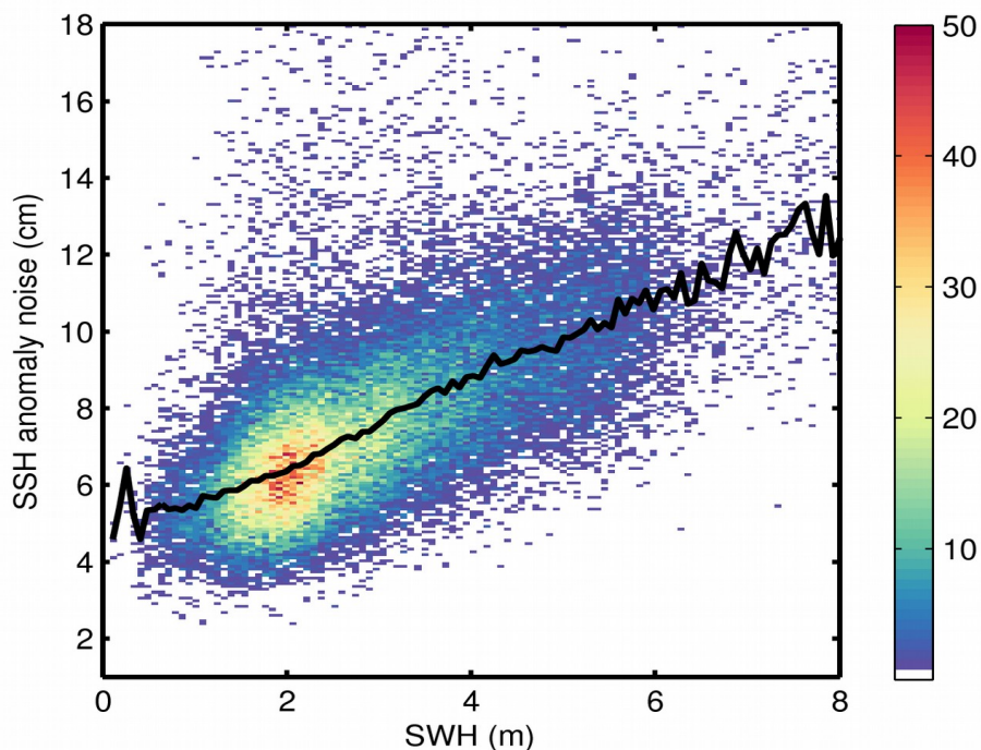
Figure 9. 2D histogram showing flag-valid SSH anomaly noise as a function of SWH for 07/10/2018. The black line denotes the median SSH anomaly noise as a function of SWH.
